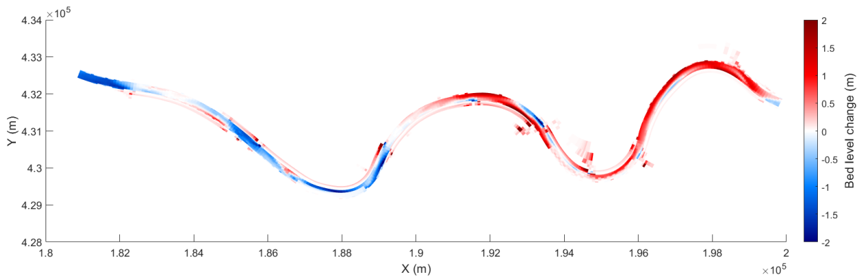
FIGURE F.5: Bed level change after 20 years for \text{Sim}_{SC-LTD}
