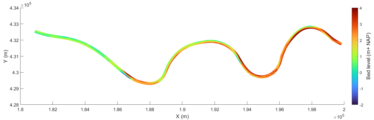
FIGURE 4.8: Bed level at the start of the simulation for Sim REF in the Boven-Waal. This includes the 2 years of morphological spin-up described in Section 3.5.
