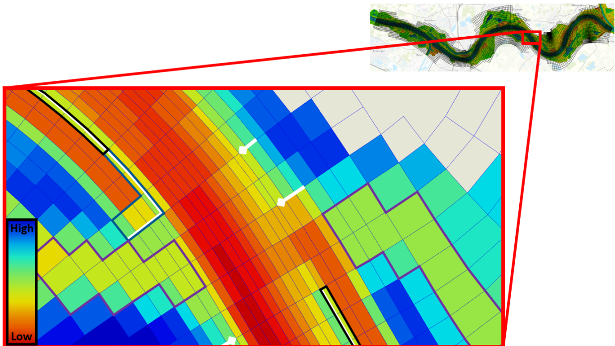
FIGURE D.8: An example of how \text{Sim}_{SC-GL-LTD} is schematized between rkm 876 and 877. The colours indicate the elevation of the grid cells. The black polygons represent the crest of an LTD, the dark blue polygon represents the sill of the LTD, the purple polygons represent side channels and the white lines represent weirs. The white lines with a square at the tip are also weirs in the model schematization, but specifically represent groynes in this figure.
