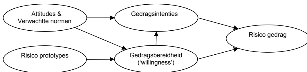
Figuur 2 Prototype-Willingness model (Gerrard, Gibbons, Stock, Vande Lune, & Cleveland, 2005, p 306)
