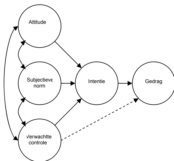
Figuur 1 Theory of Planned Behavior (Ajzen, 1991, p 182)
