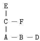
Figure 3.12: The AST for the rule “A B C ^^ D E ^^ F G!”, given the sentence “A B C D E F G”
