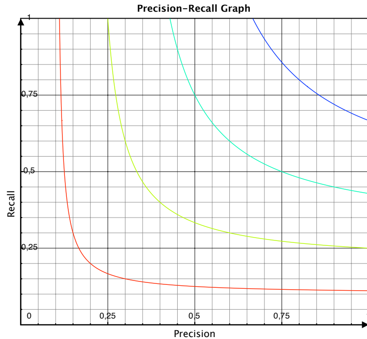
Figure 13: Precision-Recall graph
