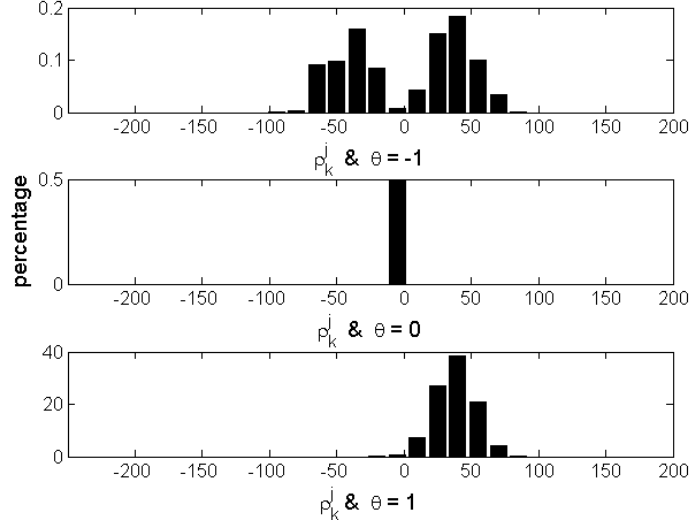
Figure 33: Example of an acceleration histogram based on an empirical density of the particles in one MC simulation run with HPF M=3 at time t=60 , N_p = 5 \cdot 10^4
