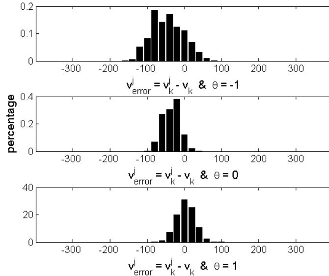
Figure 31: Example of a velocity histogram based on an empirical density of the particles in one MC simulation run with HPF M=3 at time t=46 , N_p = 5 \cdot 10^4
