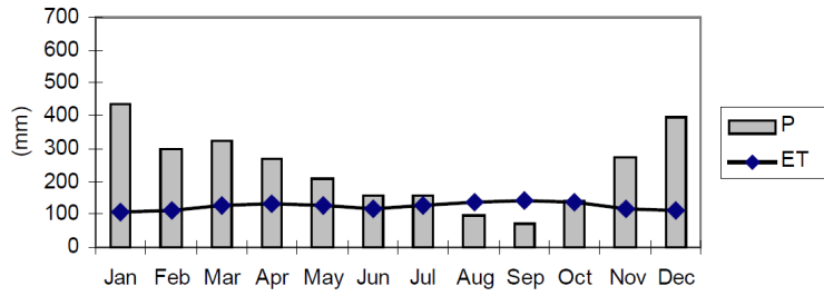
Figure 2.2: Precipitation ( P ) and evapotranspiration ( ET ) measured from Banjarmasin, on the southwest boundary of the EMRP-area. During the dry period, evapotranspiration exceeds the rainfall. Data obtained from Ritzema and Wösten (2002).
