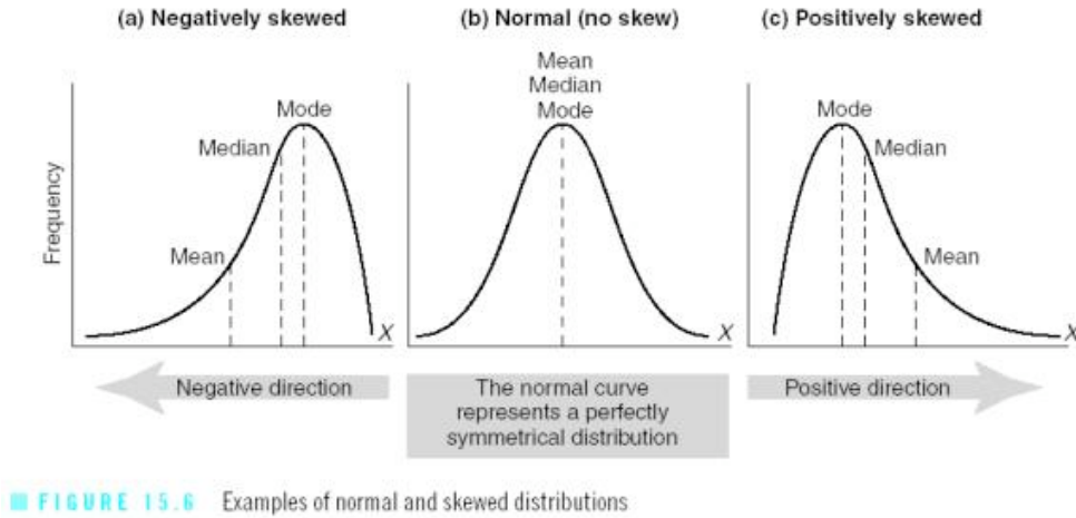
Figure 5: A plot of a (skew) normal distribution [9]
