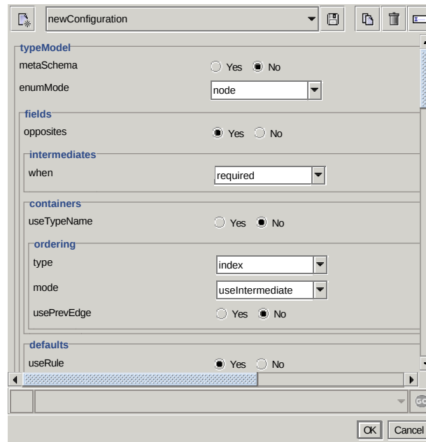
Figure 6.3: A generated configuration GUI.
