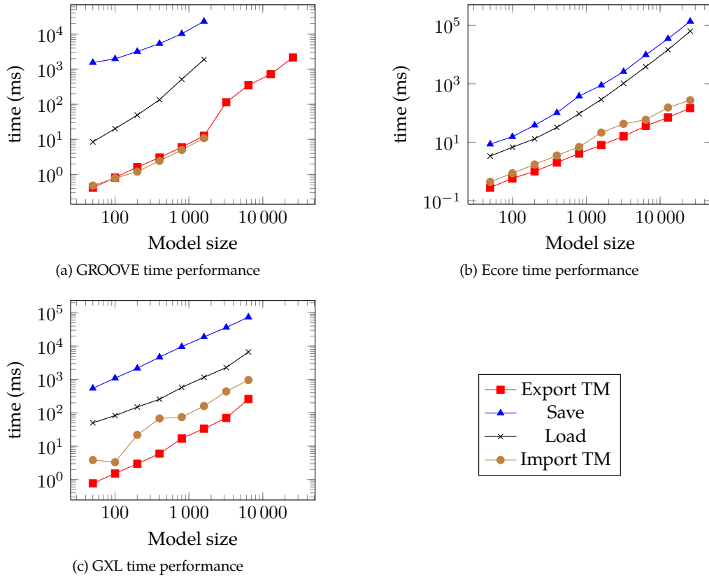
Figure 6.5: Time performance of GROOVE, Ecore and GXL mappings.
