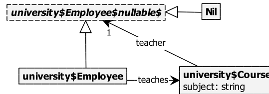
Figure 4.2: Example typegraph with nullable classes.
