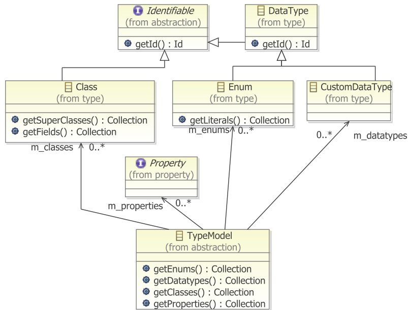
Figure A.3: The Java classes for the type model.
