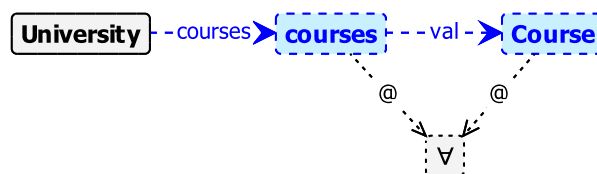
Figure 2.5: Example rule graph with quantifier node. This rule matches a University node and all course edges and Course nodes connected to this University node. These edges and Course nodes are then deleted.
