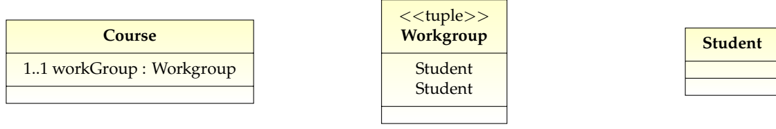
(a) Graphical representation of a type model with a tuple.
