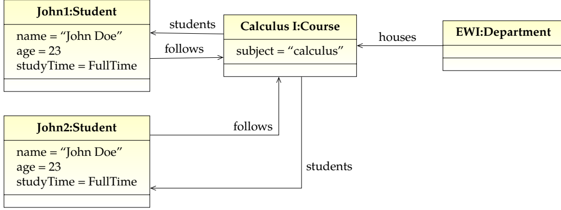
Figure 3.7: Model not satisfying the identity property.
