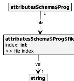
Figure 5.7: Simple GXL type graph with attributed nodes.
