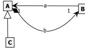
Figure 4.5: The containment property in GROOVE. In this example, the field b of class A is declared to be a containment relation.
