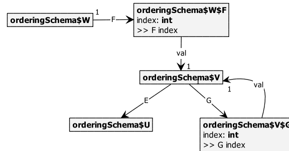
Figure 5.6: Simple GXL type graph with ordered edges.
