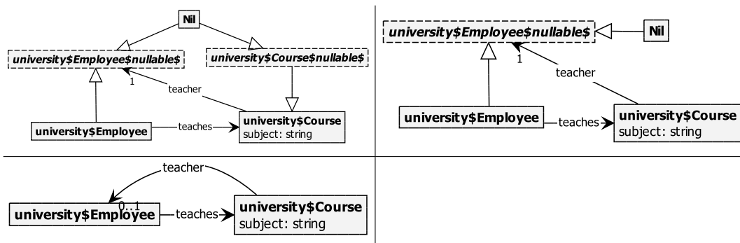
Figure 4.21: Effect of the NullableClasses option on type graphs.
