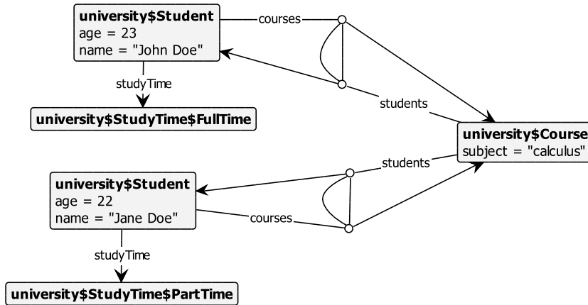
Figure 4.16: An instance graph representation of the example University instance model.
