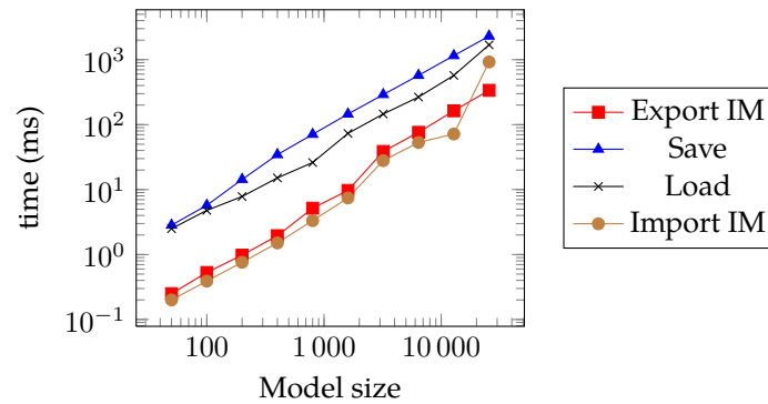
Figure 6.6: Time performance of the DOT mapping.
