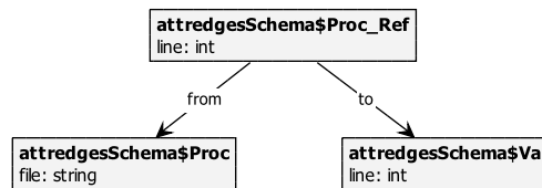
Figure 5.8: Complex GXL type graph with an attributed edge.
