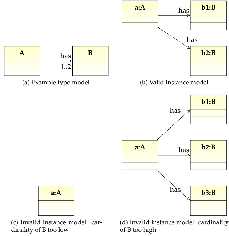
Figure 3.5: Examples of valid and invalid multiplicities.
