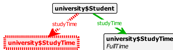
Figure 4.10: A rule graph for the defaultValue property.
