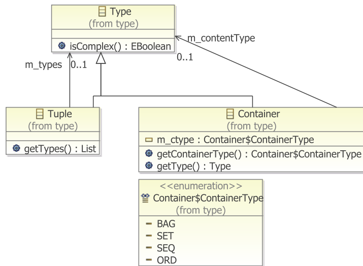
Figure A.5: The complex types.
