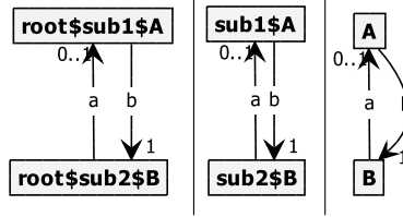
Figure 4.20: Effect of the Namespaces option on identifiers in graphs. The figure shows the Full, NonAmbiguous and Flat alternatives respectively.
