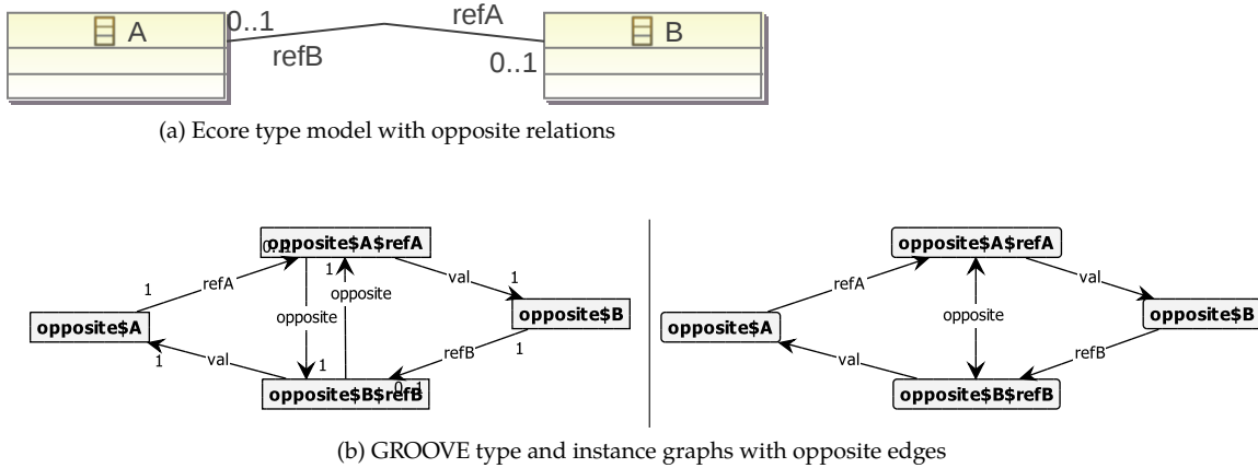
Figure 5.4: Imported Ecore model showing opposite relations, and corresponding GROOVE graphs.
