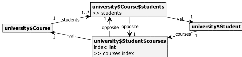
Figure 4.8: Example type graph for opposite edges.
