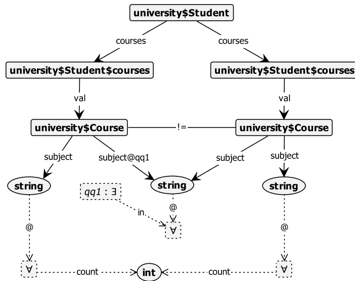
Figure 4.7: Example of a keyset constraint rule. This rule checks that no instance of the Student class has two Course instances with the same subject in the courses relation.
