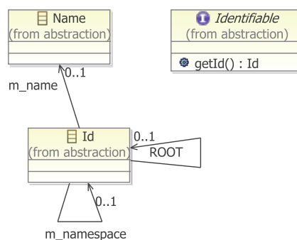
Figure A.1: Names and identifiers.
