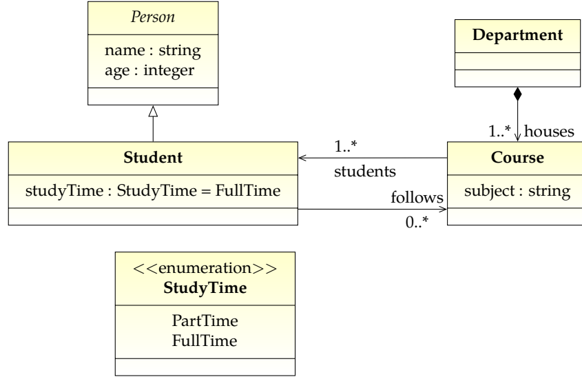
(a) Graphical representation of a type model
