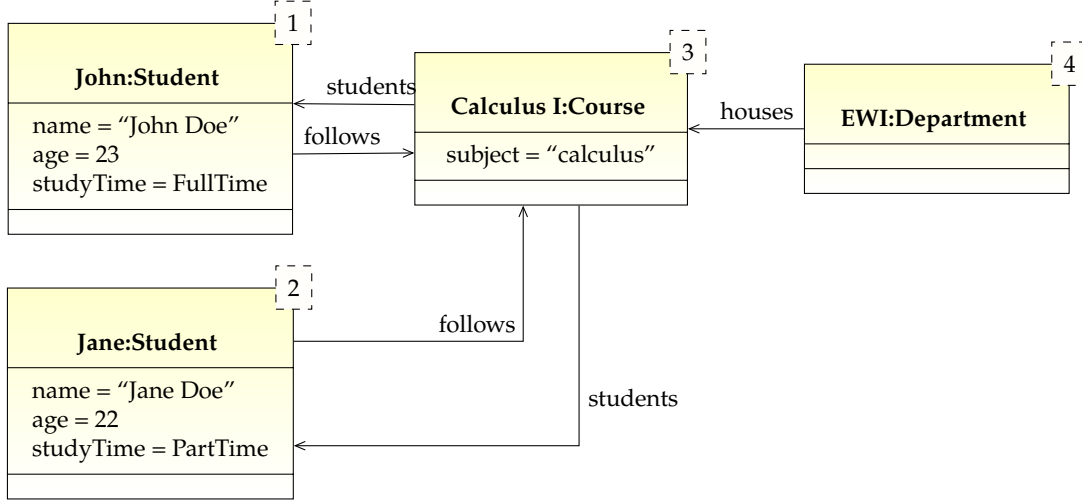
(a) Graphical representation of an instance model.
