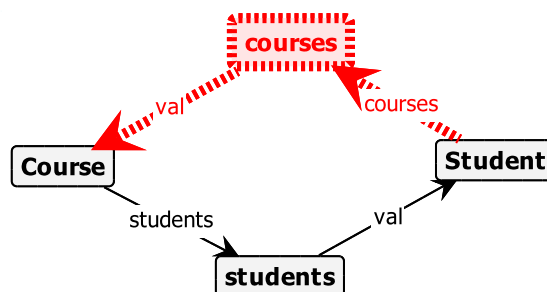
Figure 2.4: Example rule graph with NAC node. This rule matches only if a Course and Student node exist, which are connected by an intermediate students node, but not by an intermediate courses node.
