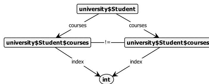
Figure C.3: Example ordered rule graph.
