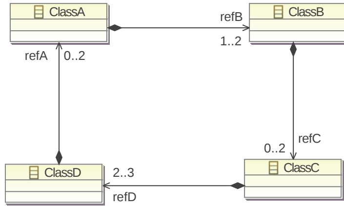
(a) Ecore type model with various relations
