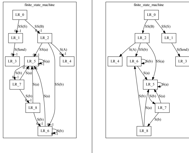
Figure 5.14: Exported type graph (left) and instance graph (right), rendered by DOT.
