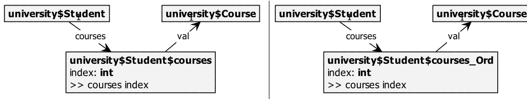
Figure 4.24: Effect of the IntermediatePostfix option. On the left the option is turned off, on the right it is turned on.
