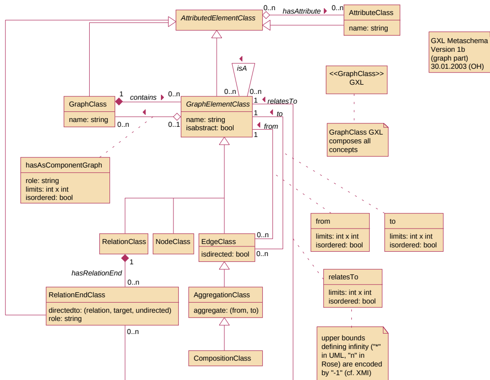
Figure B.1: Graph part of the GXL meta schema.
