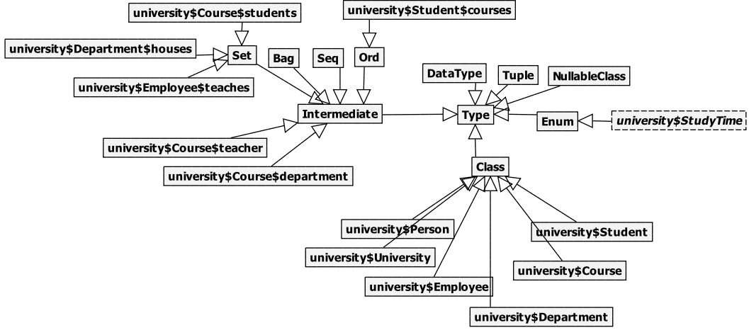
Figure 4.15: Meta graph of University example.
