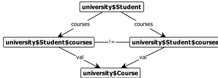
Figure 4.14: Example constraint rule for unique values.
