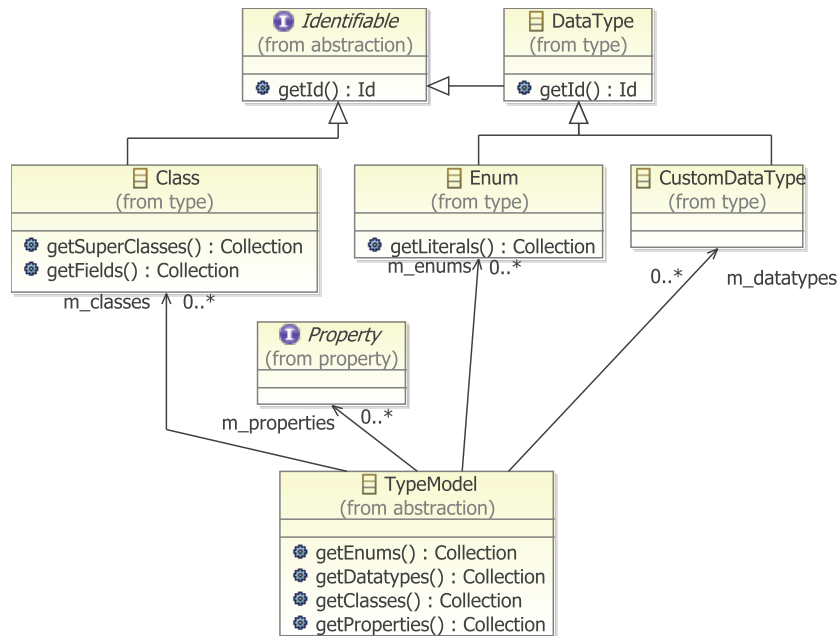
Figure 6.1: Part of the implementation of the type model.
