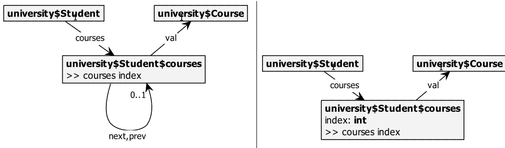
Figure 4.25: Effect of the Ordering option on intermediate nodes of ordered container types in type graphs. Note that the index of the values is hidden in the right graph, but internally still present.
