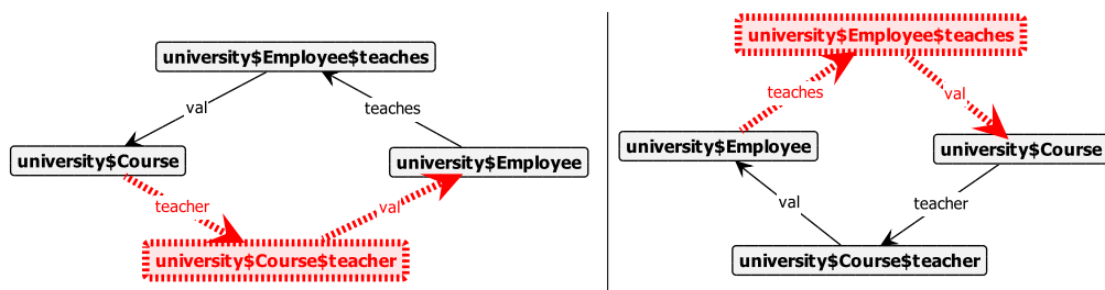
Figure 4.9: Example constraint rules for opposite fields.
