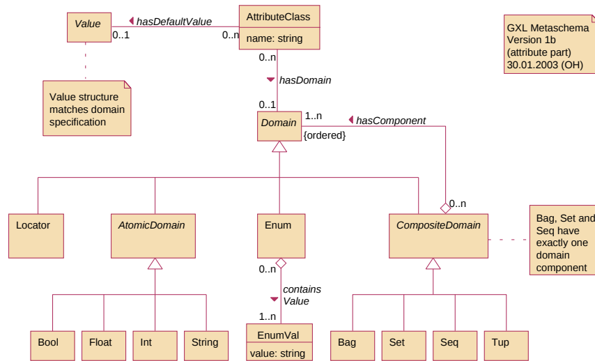
Figure B.2: Attribute part of the GXL meta schema.
