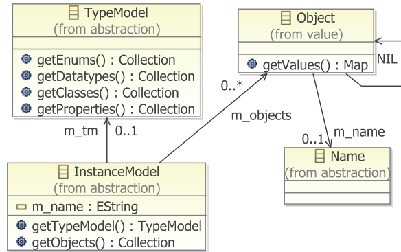
Figure A.7: The instance model.
