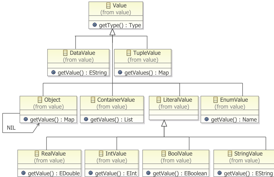
Figure A.8: Value types used within the instance model.
