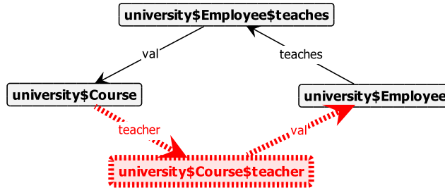
Figure C.1: Example opposite rule graph.
