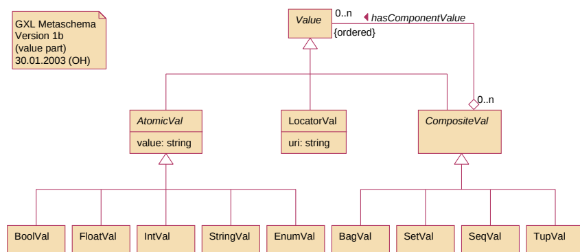
Figure B.3: Value part of the GXL meta schema.
