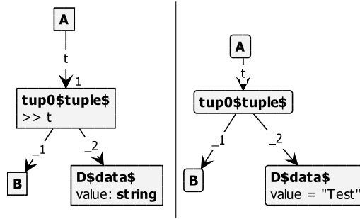
Figure 4.12: Example of a tuple in a type graph (left) and an instance graph (right).
