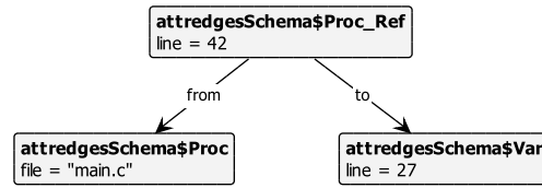
Figure 5.11: Complex GXL instance graph with an attributed edge.
