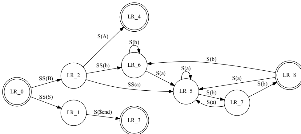
(b) Rendering of a DOT graph
