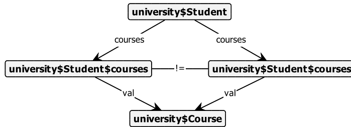
Figure C.2: Example unique rule graph.
