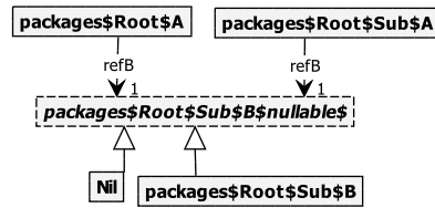
(b) GROOVE type graph with namespaces
