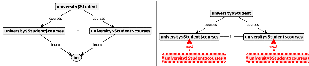
Figure 4.13: Example constraint rule for ordered containers using an index and a next edge respectively.
