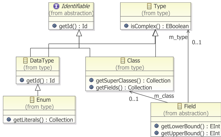
Figure A.4: The class and enum types.
