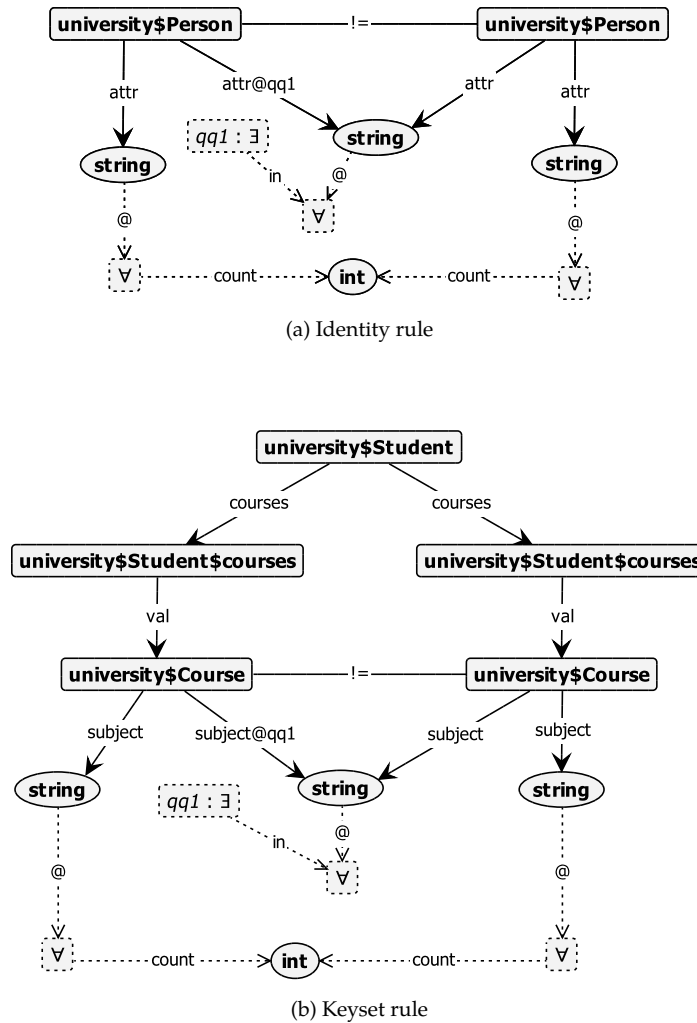
Figure C.5: Example identity and keyset rule graphs.
