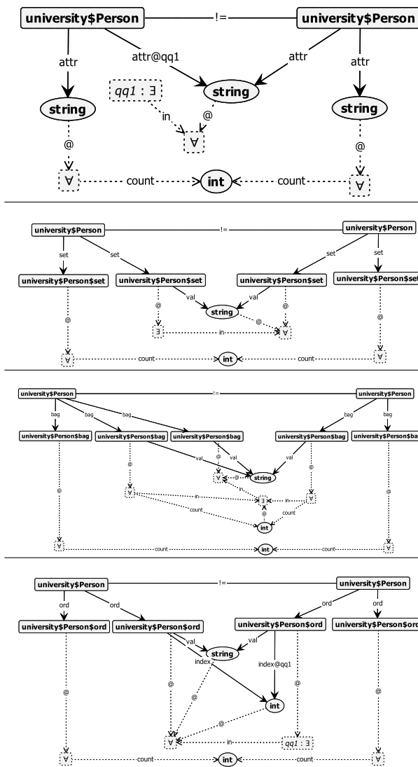
Figure 4.11: Example constraint rules for opposite fields.
