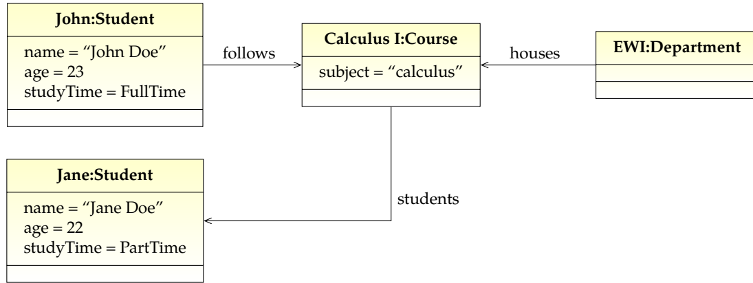
Figure 3.10: Model not satisfying the opposite property.
