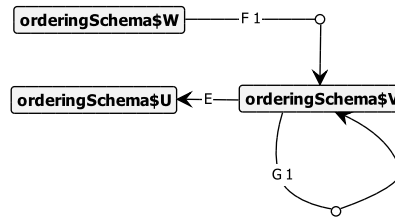
Figure 5.9: Simple GXL instance graph with ordered edges.
