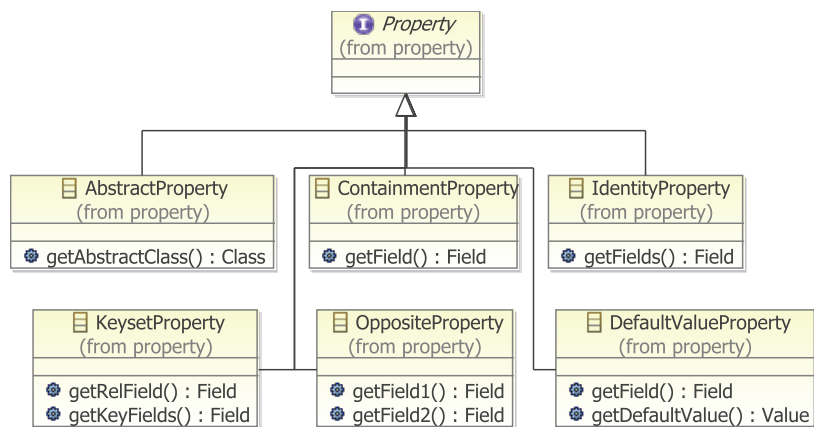
Figure A.6: The properties.
