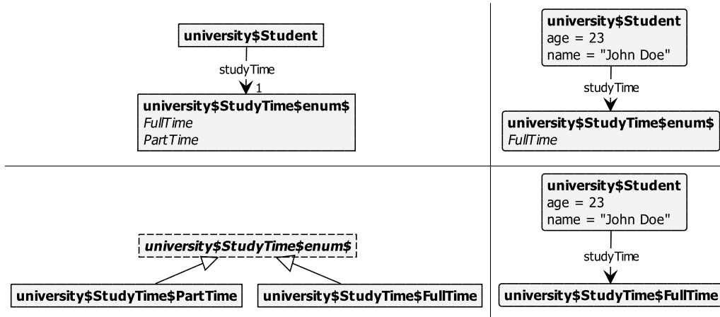
Figure 4.22: Type and instance graphs generated for enumerations using flags or nodes.
