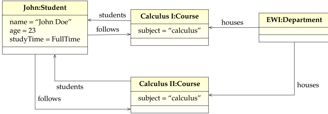
Figure 3.8: Model not satisfying the keyset property.
