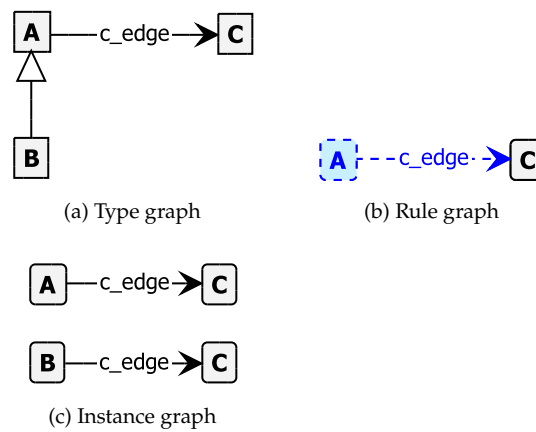
Figure 1.1: Example GROOVE graphs.
