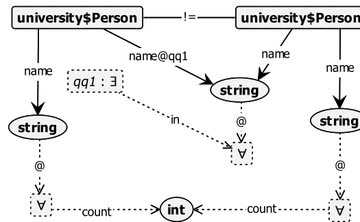
Figure 4.6: Example of an identity constraint rule. This rule checks that no two instances of the Person class have the same value of the name field.
