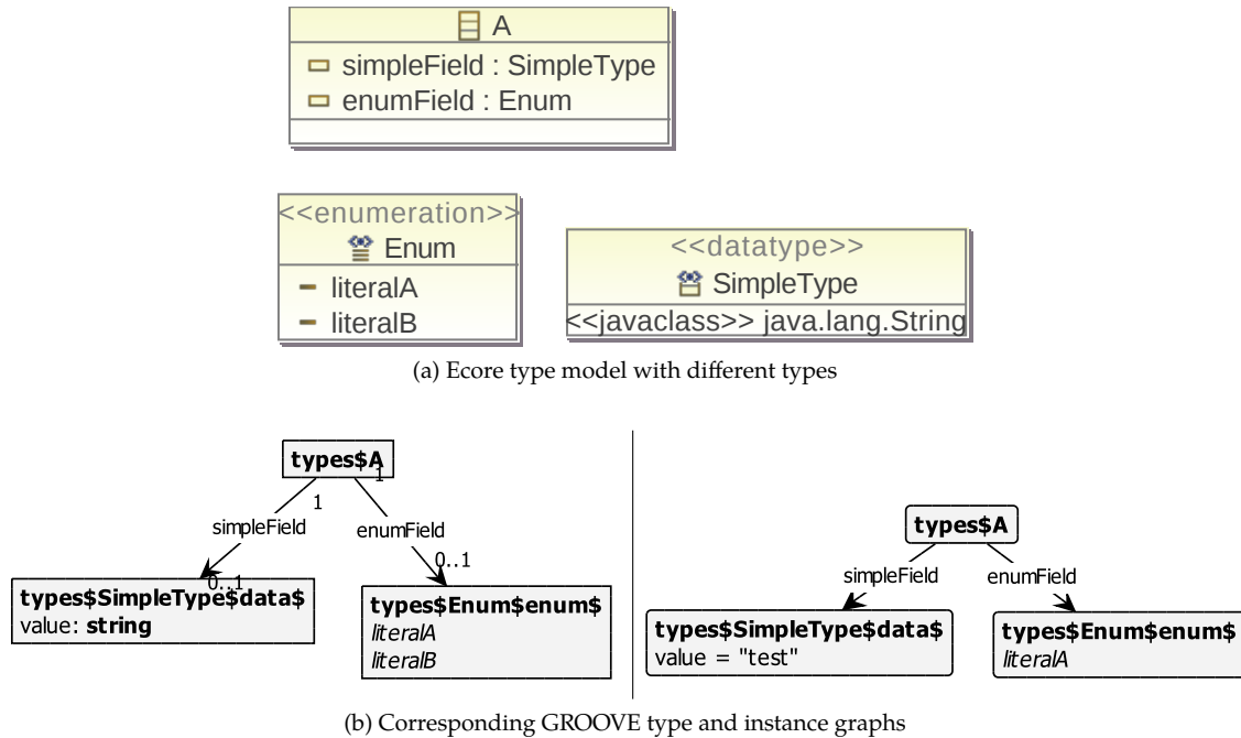
Figure 5.3: Imported Ecore class, enum and data type, and corresponding GROOVE graphs.
