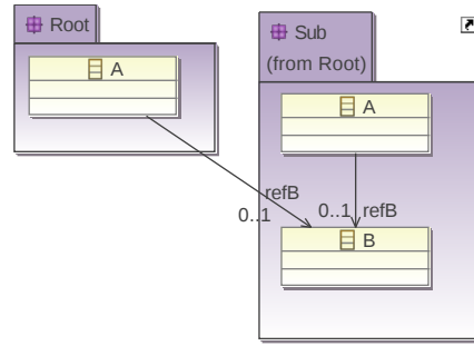
(a) Ecore model with packages
