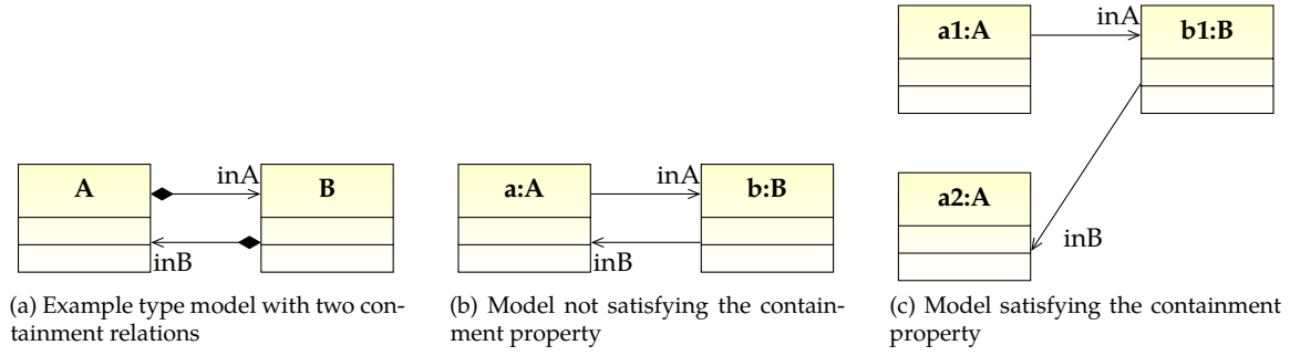
Figure 3.9: Examples of the containment property.
