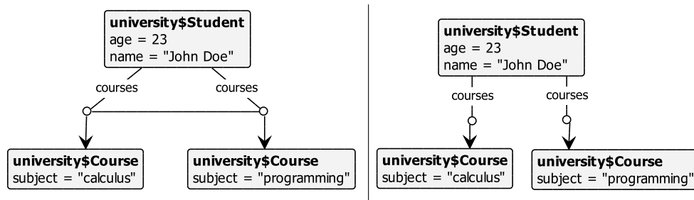
Figure 4.27: Effect of the Ordering option on intermediate nodes of ordered container types in instance graphs.
