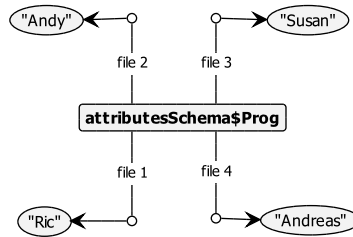
Figure 5.10: Simple GXL instance graph with attributed nodes.
