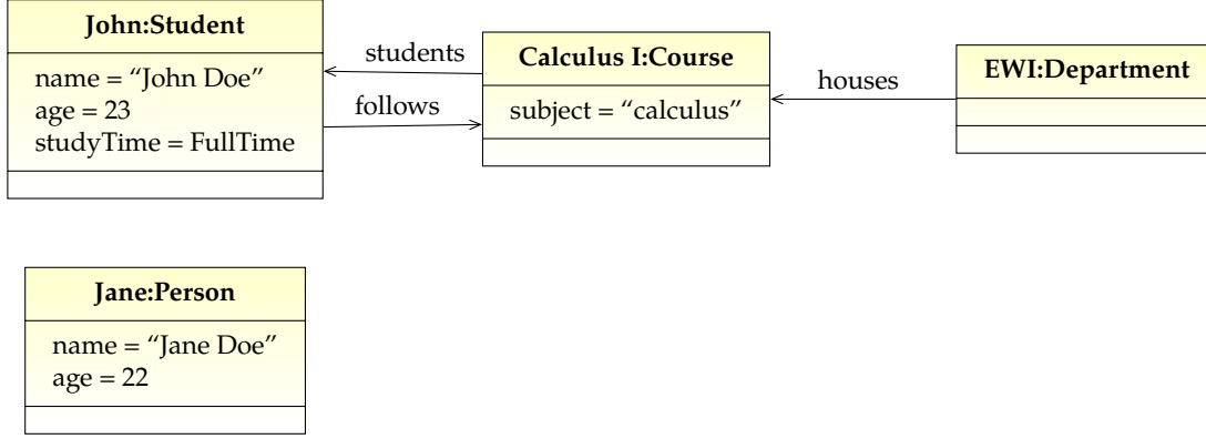
Figure 3.6: Model not satisfying the abstract property.
