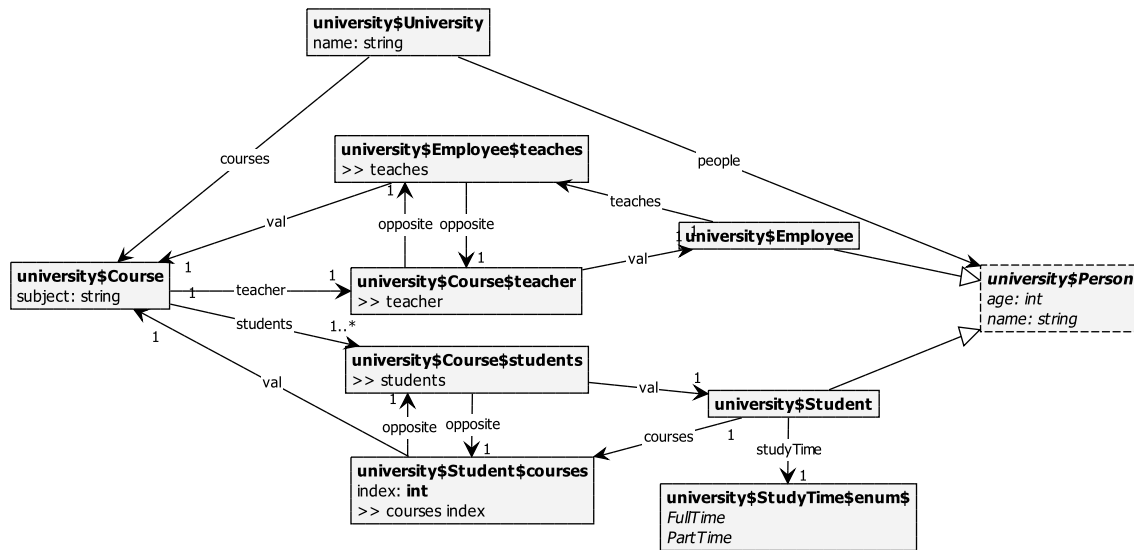
Figure 4.1: Example graph representation in GROOVE for the University type model example.
