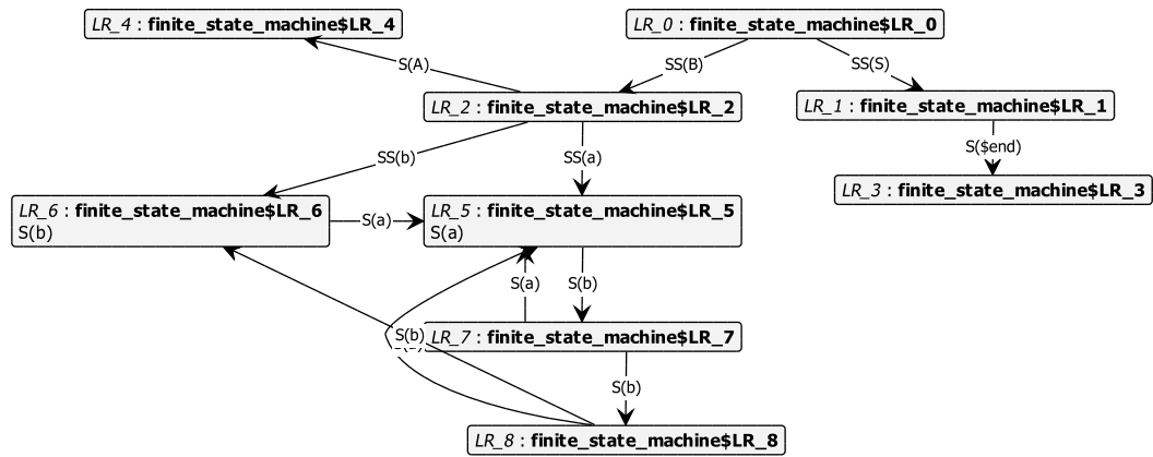
(a) Instance graph
