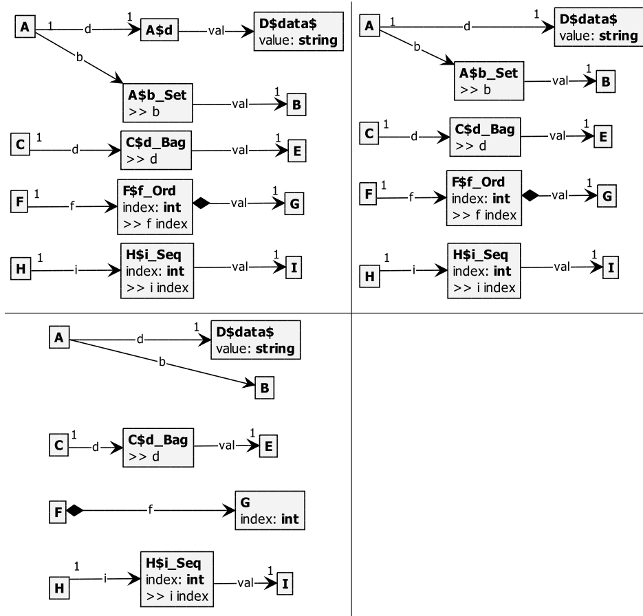
Figure 4.28: Effect of the IntermediateNodes option on intermediate nodes in type graphs. The effects of the Always , Container and Required alternatives are shown respectively.
