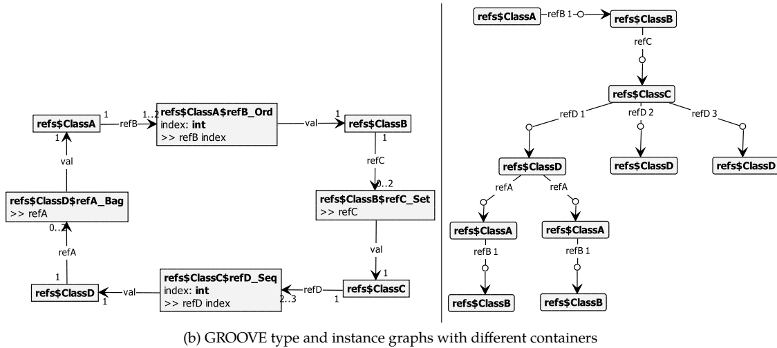
Figure 5.5: Imported Ecore model showing various relation types. On the left the resulting type graph, on the right an example instance graph.
