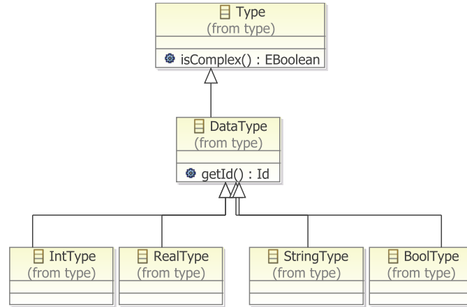
Figure A.2: Java classes for various (data) types.
