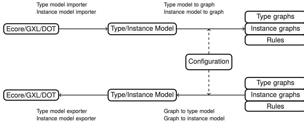
Figure 6.2: Overview of conversion process.
