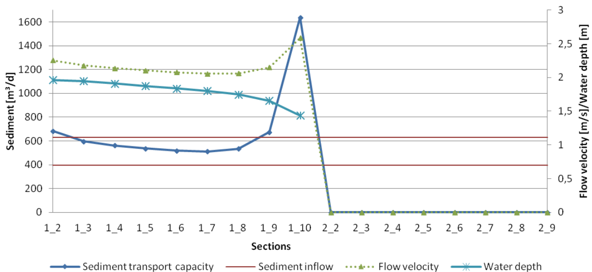
FIGURE 25: SEDIMENT TRANSPORT PROCESSES - WETLAND ALTERNATIVE ( Q=25 \text{ M}^3/\text{S} )
