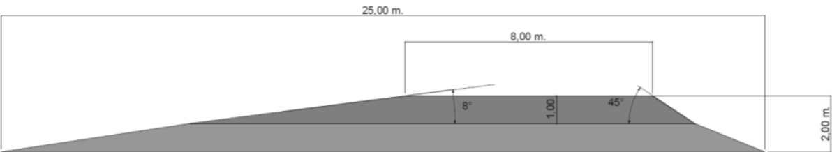
APPENDIX FIGURE 9: DIKE DIMENSIONS
