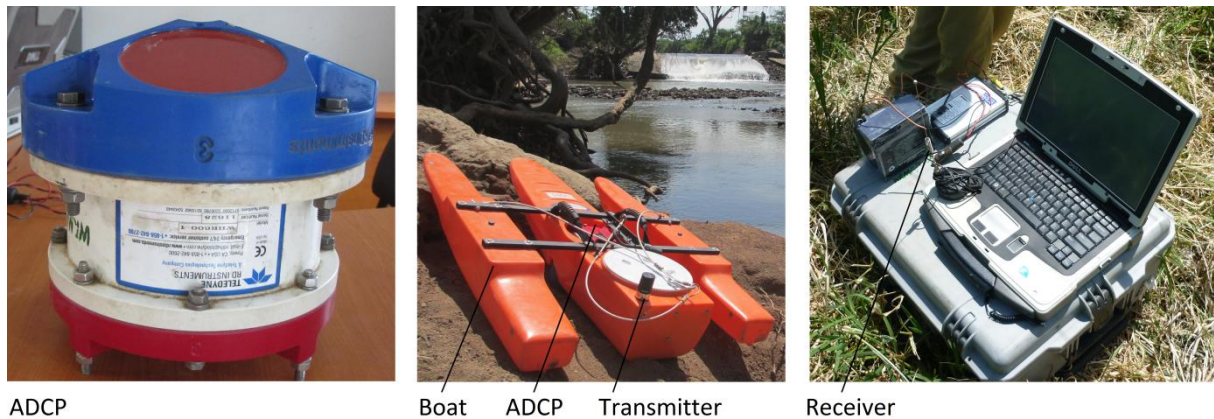
APPENDIX FIGURE 19: CROSS-SECTION MEASUREMENT TOOLS
