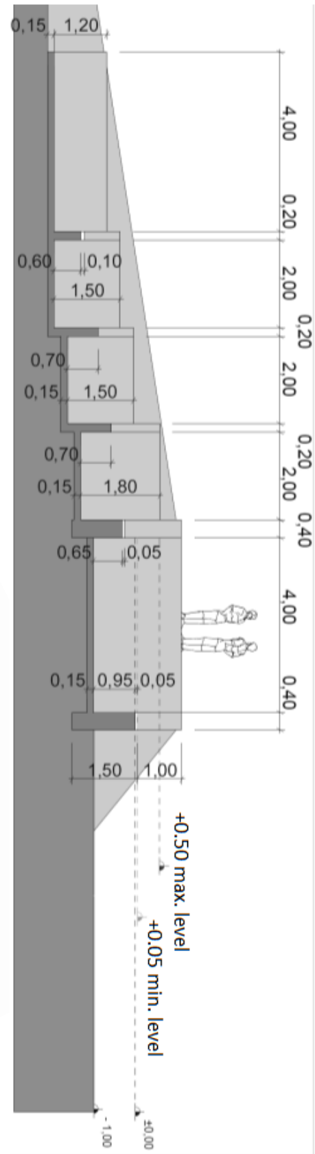
APPENDIX FIGURE 12: OUTLET CONSTRUCTION DIMENSIONS
