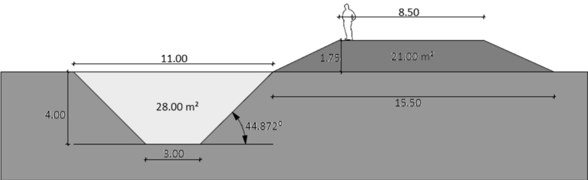
APPENDIX FIGURE 8: SPILLWAY CHANNEL DIMENSIONS
