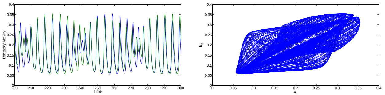
Figure 3.8: Left: Time series of the activity of excitatory populations of the quasi-periodic solution for B = 3 and \alpha = 0.115 . Right: Projection to the (E_1, E_2) plane. When the torus is close to the symmetric oscillation, the projection is close to the diagonal E_1 = E_2 .
