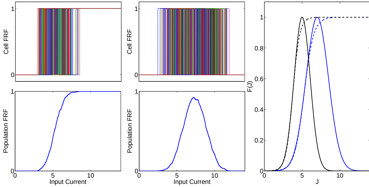
Figure 3.1: Left: Heterogeneity in firing onset for individual cells leads to a sigmoidal population FRF. Middle: Including the effect of heterogeneous thresholds for depolarization block leads to a population FRF with a maximum. Right: The FRFs used in this paper. Solid: Gaussian; Dashed: Sigmoid; Blue: Excitatory; Black: Inhibitory
