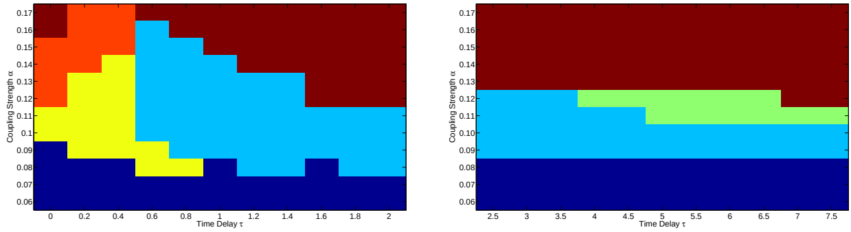
Figure 4.3: Classification of patterns after starting from random low activity history for various \tau and \alpha . Left: Small time delay; Right: Large delay. The figure on the left shows that quasi-periodic and bump activity disappears for a medium delay. The right figure shows that the in-phase solution becomes stable for a large delay. Dark blue: Low stable equilibrium; Yellow: Quasi-periodic; Light blue: Anti-phase; Green: In-phase; Red: Local bump in activity; Dark Red: High activity for all populations.
