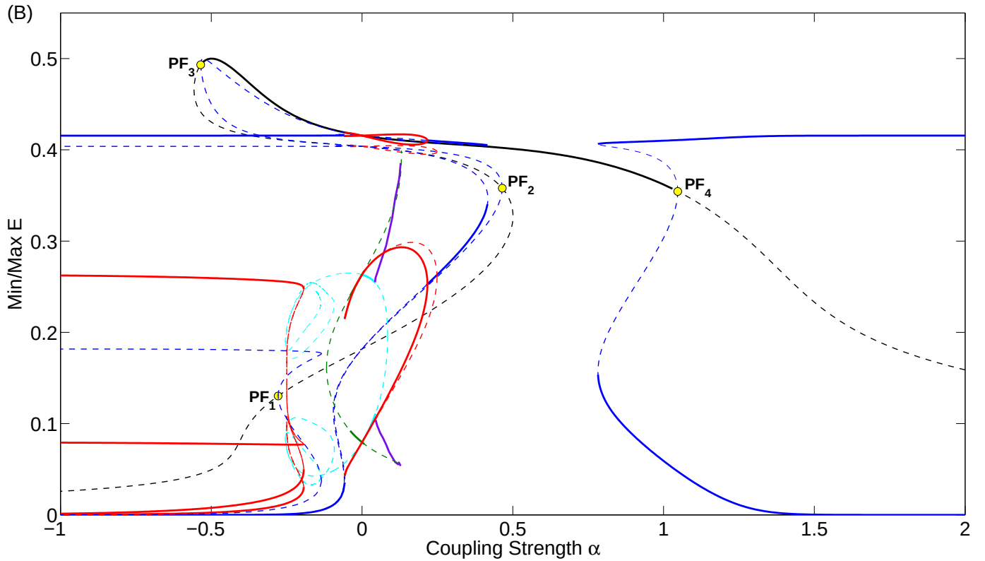
Figure 3.6: One parameter diagrams for B = 2.45 (top) and B = 3 (bottom). Black: Symmetric equilibria; Blue: Asymmetric equilibria; Green: Symmetric Oscillations; Red: Asymmetric Oscillations; Light blue: Antiphase Oscillations; Purple: Quasi-periodic oscillations. For the oscillations only the extrema are indicated. Thick solid and thin dashed lines indicate stable and unstable solutions respectively. At each pitchfork bifurcation (PF) two branches appear of which one corresponds to E_1 and the other to E_2 or vice versa.
