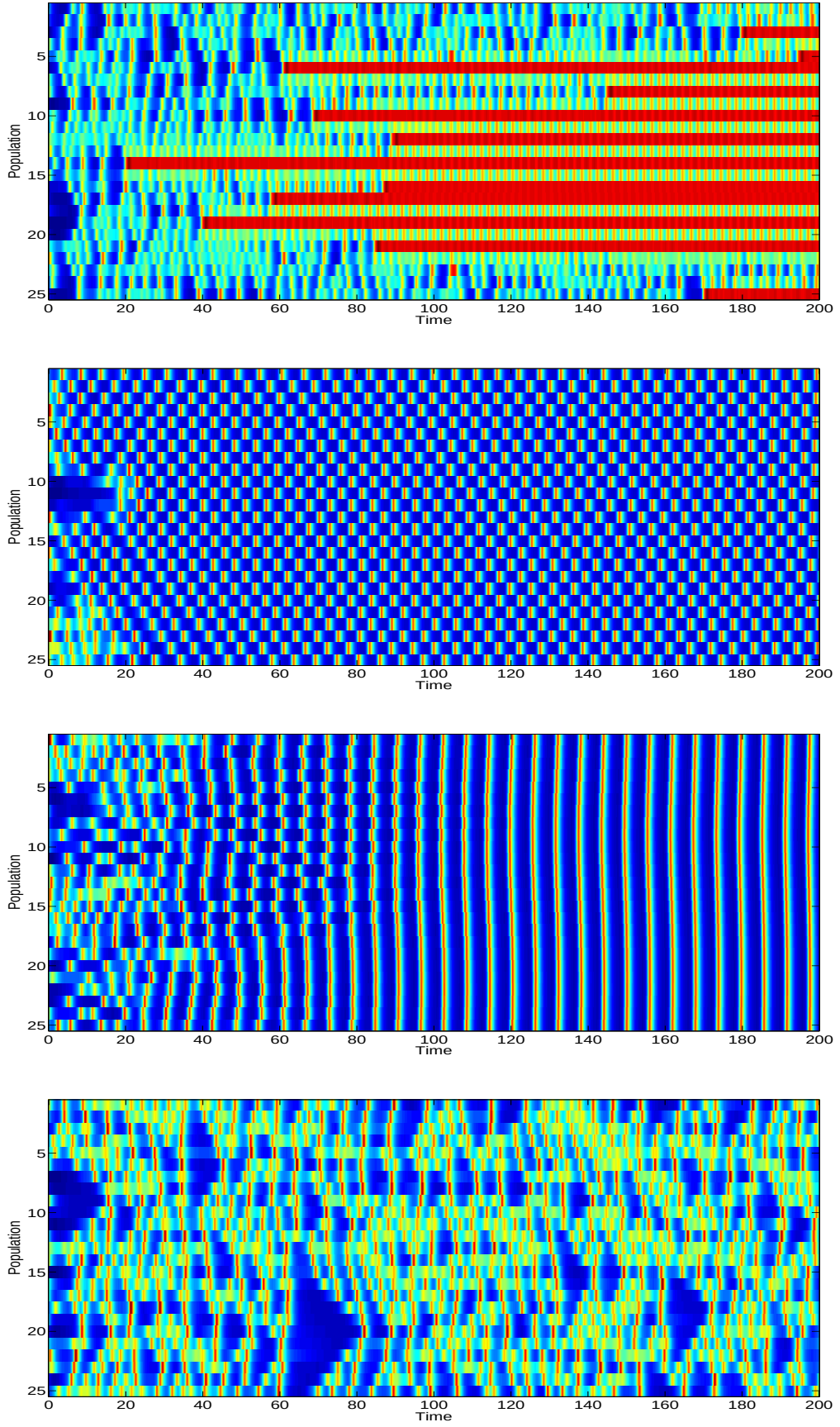
Figure 4.4: Different patterns in a neural network for (a) \{\alpha = 0.15, \tau = 0.2\} , (b) \{\alpha = 0.12, \tau = 2\} , (c) \{\alpha = 0.12, \tau = 5\} and (d) \{\alpha = 0.12, \tau = 0.2\}
