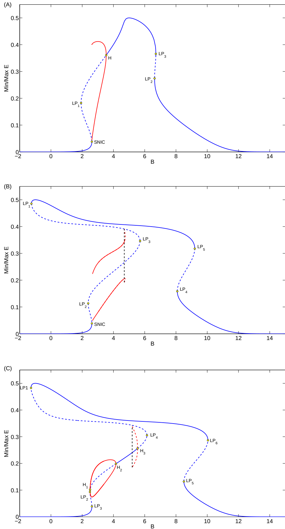
Figure 3.3: Bifurcation diagrams for w_{EI} = 13 (top), w_{EI} = 18 (middle) and w_{EI} = 20.5 (bottom) with a Gaussian FRF. Blue: Stable equilibrium; Red: Extrema of limit cycles; Solid: Stable; Dashed: Unstable. The dashed black line indicates a homoclinic bifurcation. By Increasing w_{EI} a fold bifurcation is crossed and two high activity equilibria appear. The dynamics if w_{EI} = 13 can also be found when a sigmoid FRF is used.
