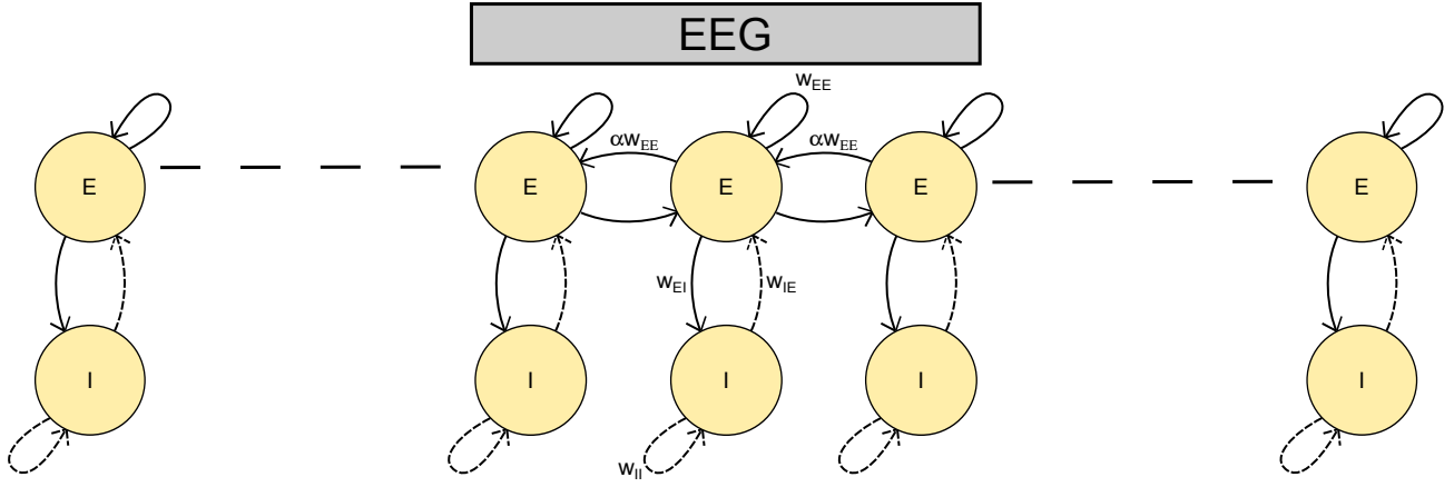
Figure 2.1: A schematic overview of the model. Each E-I pair is coupled, with or without propagation delay \tau , to its neighbors through its excitatory subpopulation. We model EEG output as the average current over three populations. Solid: Excitatory connections; Dashed: Inhibitory connections.
