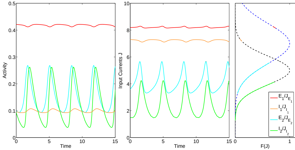
Figure 3.7: Left: Time series of the activity of the subpopulations for B = 2.3 and \alpha = 0.1 ; Middle: Input currents into each subpopulation; Right: The dynamical range of input currents J along the excitatory (blue) and inhibitory (black) FRF. Red: E_1 ; Orange: I_1 ; Light blue: E_2 ; Green: I_2 . The high and low activity populations reside on the right and left halves of the Gaussian FRF respectively.
