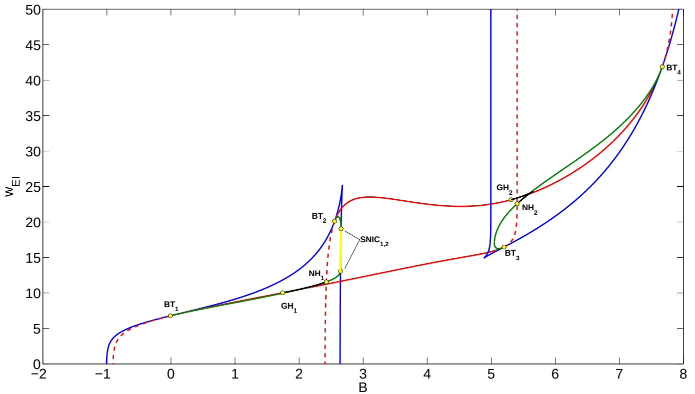
Figure 3.4: Bifurcation diagrams for Gaussian (top) and sigmoid (bottom) firing rate function, the active parameters are background input B and coupling parameter w_{EI} , other parameters as in table 2.1. Bifurcation curves are indicated with color: saddle-node (blue), Hopf (red), Limit point of cycles (black), Homoclinic to saddle (green), Saddle node on invariant curve (yellow). The red dashed line indicates a neutral saddle curve, which is not a bifurcation curve. Note the extra saddle-node curve for high values of w_{EI} and low values of B and the different horizontal scale.
