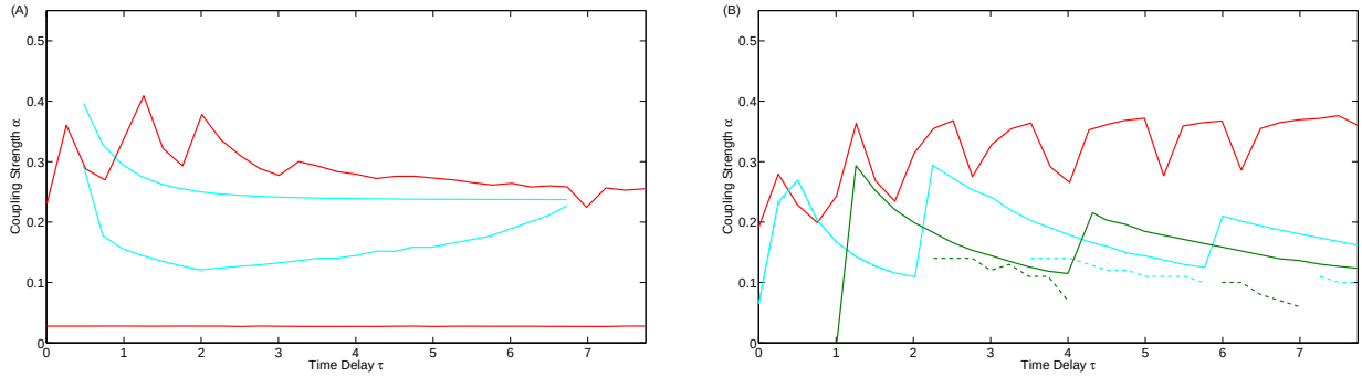
Figure 4.1: The lines indicate the upper and lower bounds in between which the periodic solutions are stable with B = 2.45 (left) and B = 3 (right). Stability was calculated at \tau = 0.25k with k = 0 \dots 32 and lines were drawn between the points. The dashed lines in the right figure are the upper bound in which simulations showed in-phase or anti-phase solutions. If B = 3 the lower bounds are smaller than zero and not shown. Note that the solid and dashed lines only overlap for \tau < 2 . Red: High-low activity; Green: In-phase low activity; Light blue: Anti-phase low activity.
