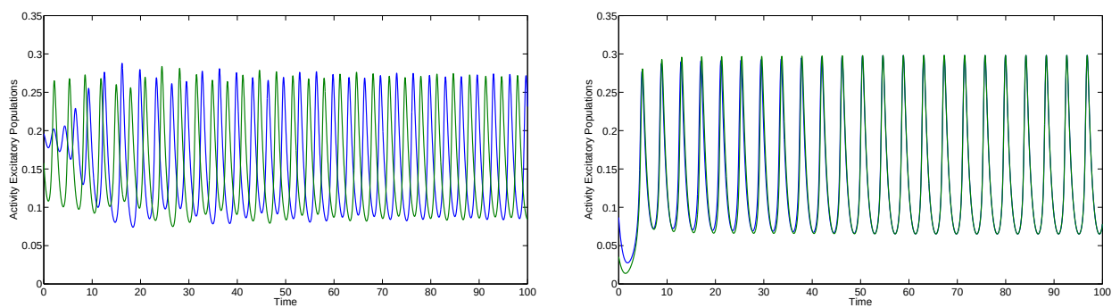
Figure 4.2: Time series for the anti-phase (left) and in-phase (right) solutions for \alpha = 0.05 , \tau = 4 starting from random low activity history.
