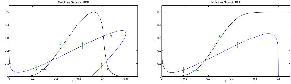
Figure 3.2: Nullclines and direction field for a Gaussian (left) and sigmoid (right) firing rate function. Parameters as in table 2.1 with B = 3 and w_{EI} = 18 . Two additional high excitatory activity states exist in the Gaussian case
