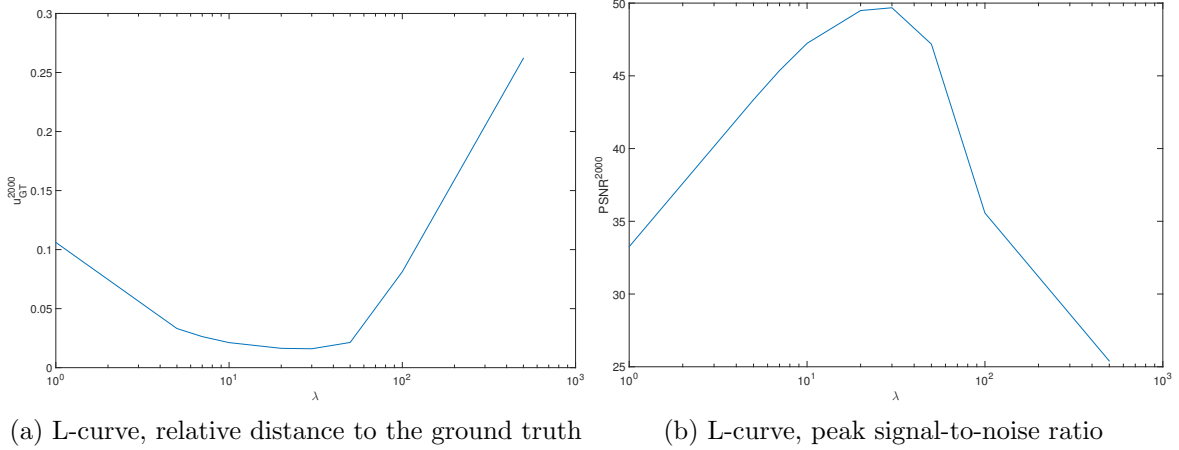
Figure 11: L-curve parameter estimation for the TV model applied to Figure 7a with s = 0.05 (see (75)) and n = 2000 . In this case \lambda = 30 would be the best choice. For the TGV_\beta^2 model the L-curve method would give a two dimensional version of these figures (since there are two parameters to estimate)
