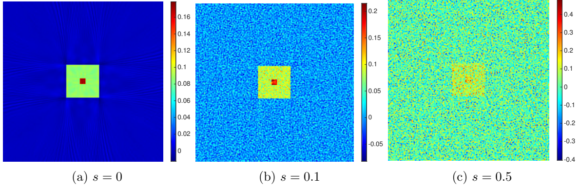
Figure 12: Reconstruction results for FBP applied to noisy data
