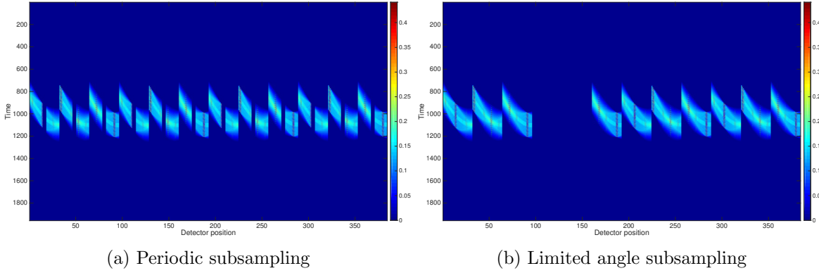
Figure 10: Subsampling strategies
