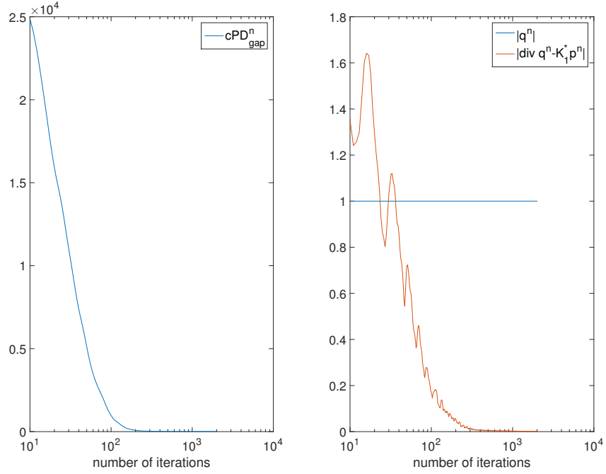
(b) Conditonal primal-dual gap & constraints cPD_{gap}^{2000} = 1.66 , |q^{2000}| = 1 , |\text{div } q^{2000} - K_1^* p^{2000}| = 5.71 \cdot 10^{-4} .
