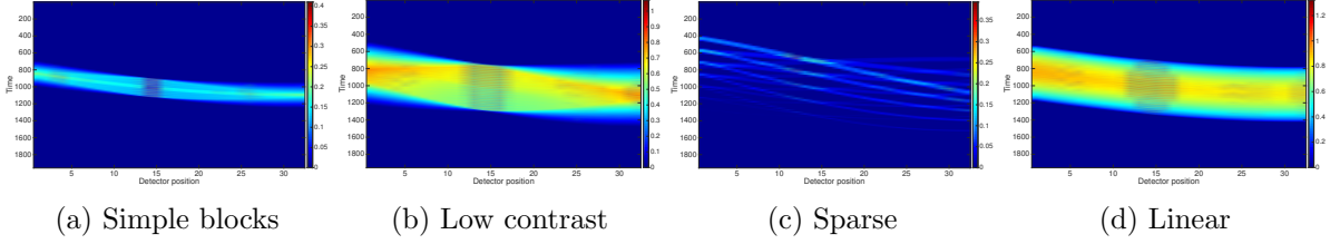
Figure 8: Partitions of the sinograms
