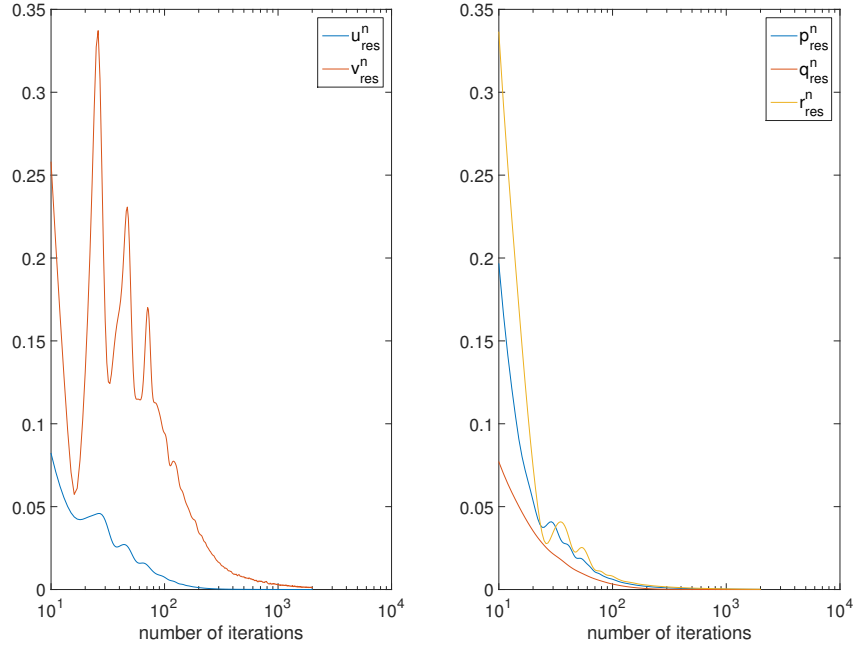
(a) Residuals
