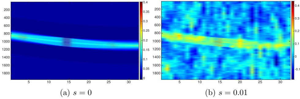
Figure 22: First partition of the solution to the outer problem
