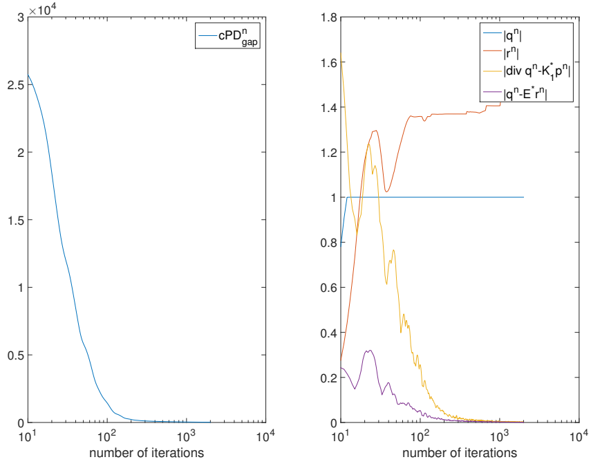
(b) Conditonal primal-dual gap & constraints
