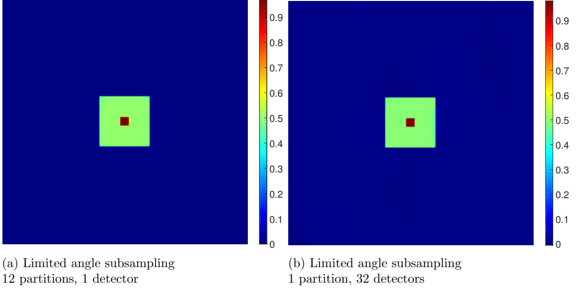
Figure 15: FBP subsampling
