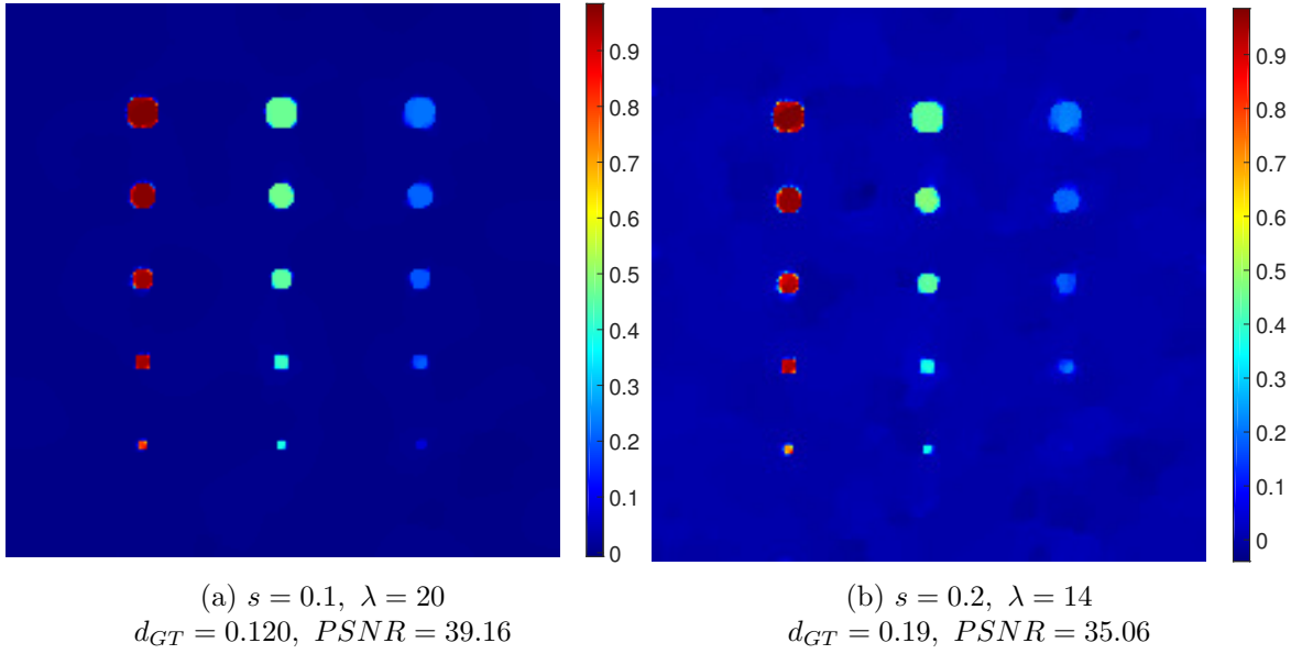
Figure 19: Reconstruction results for TV applied to sparse data
