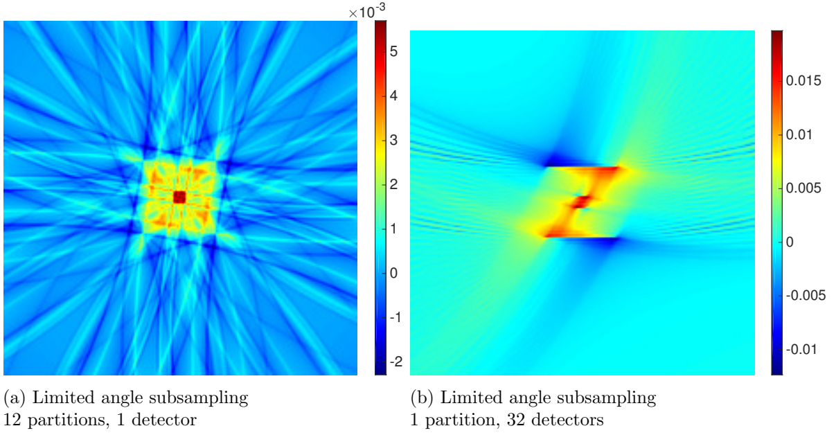
Figure 15: FBP subsampling
