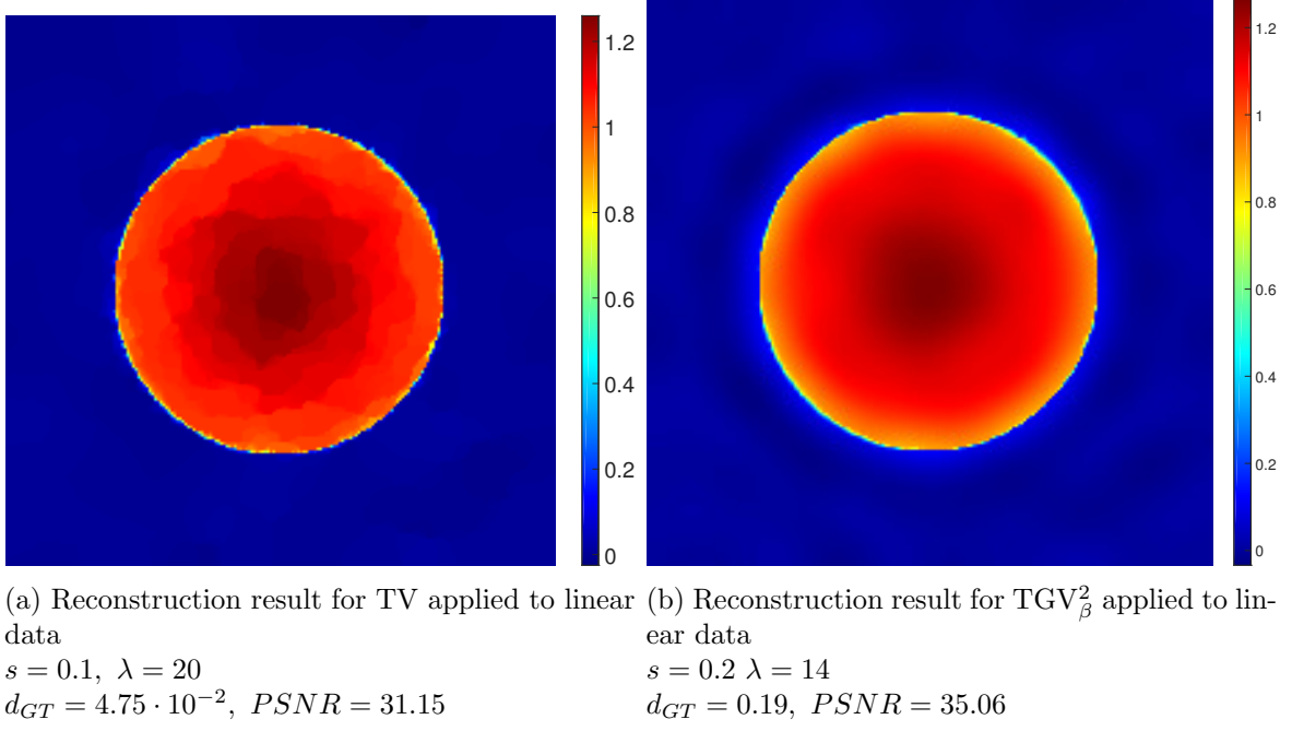
Figure 20: Linear data
