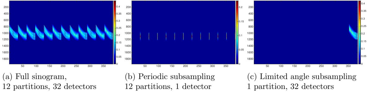
Figure 14: Sinograms with subsampling strategies
