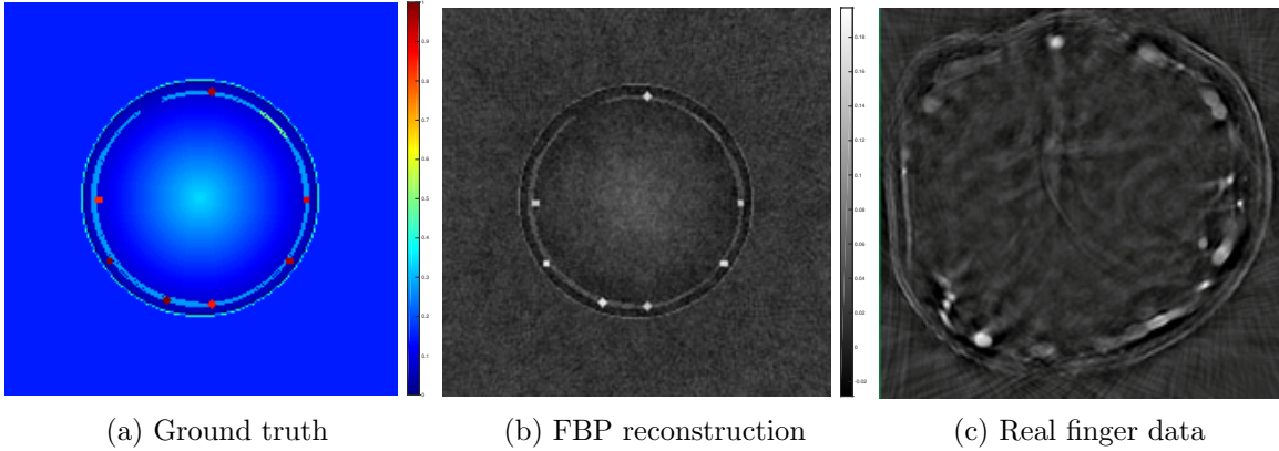
Figure 23: Creation of the realistic data set
