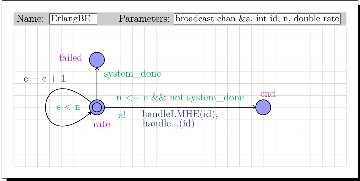
Figure 3.2: Basic Element (Trigger: Erlang( n , 1/\text{rate} ))
