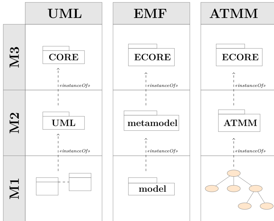
Figure 4.2: M1,M2,M3 metamodeling example
