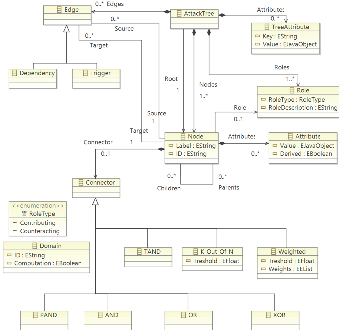
Figure 4.3: The proposed meta-model v1.0
