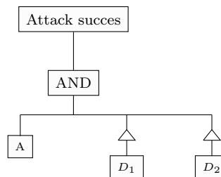
Figure 2.5: Example of an Attack Countermeasure Tree
