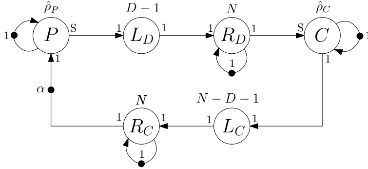
Figure 6.2: SDF model Nebula ring interconnect
