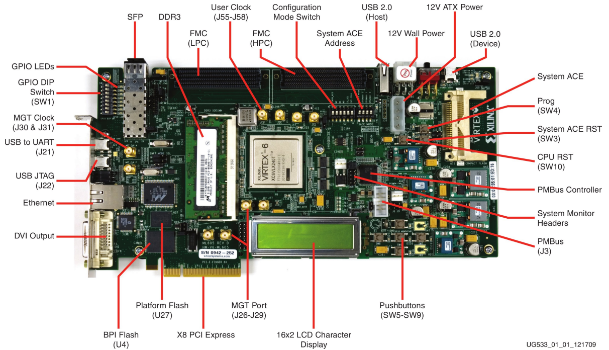
Figure 3.1: ML605 development board
