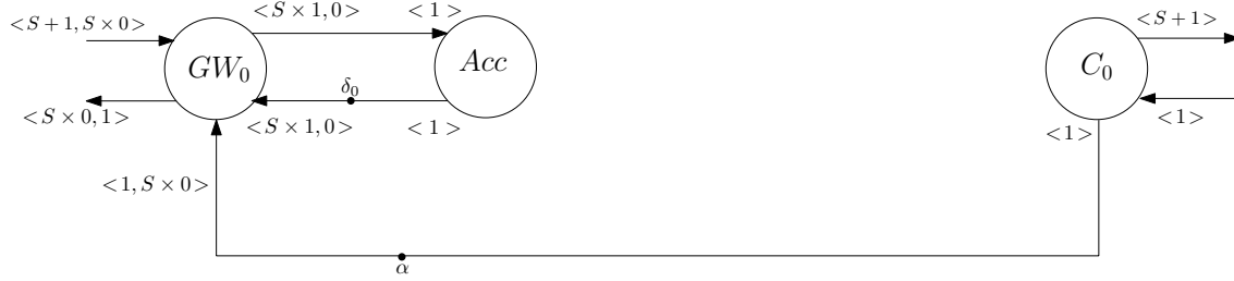
Figure 6.8: CSDF model: Hardware Accelerator added
