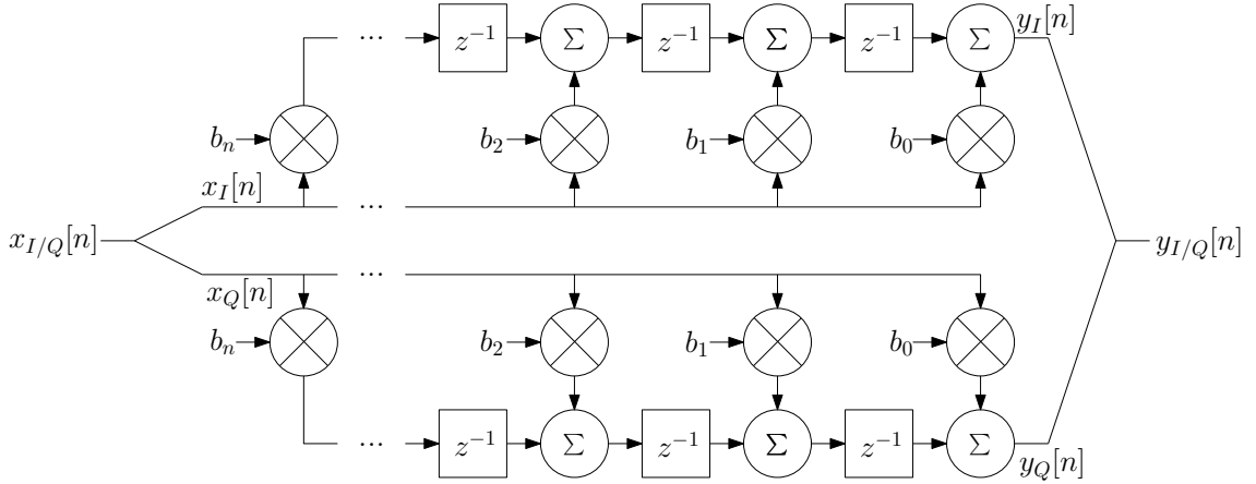
Figure 7.7: FIR filter structure with two identical pipelines for the I and Q signals
