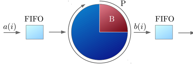
Figure 2.4: Task scheduled under TDM with a fixed budget B (in red) during a period P (in blue)
