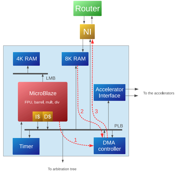
Figure 5.4: Gateway overview, including DMA Controller
