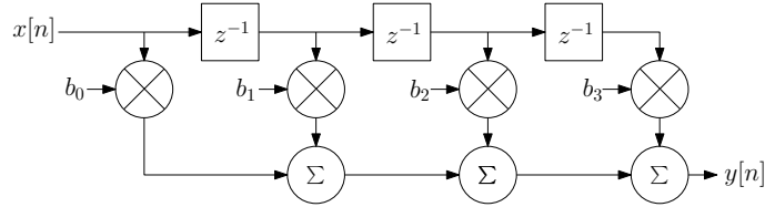
Figure 7.5: FIR filter structure (Direct Form I, N = 3 )
