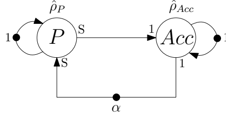
Figure 6.3: Potentially dead-locked accelerator communication model
