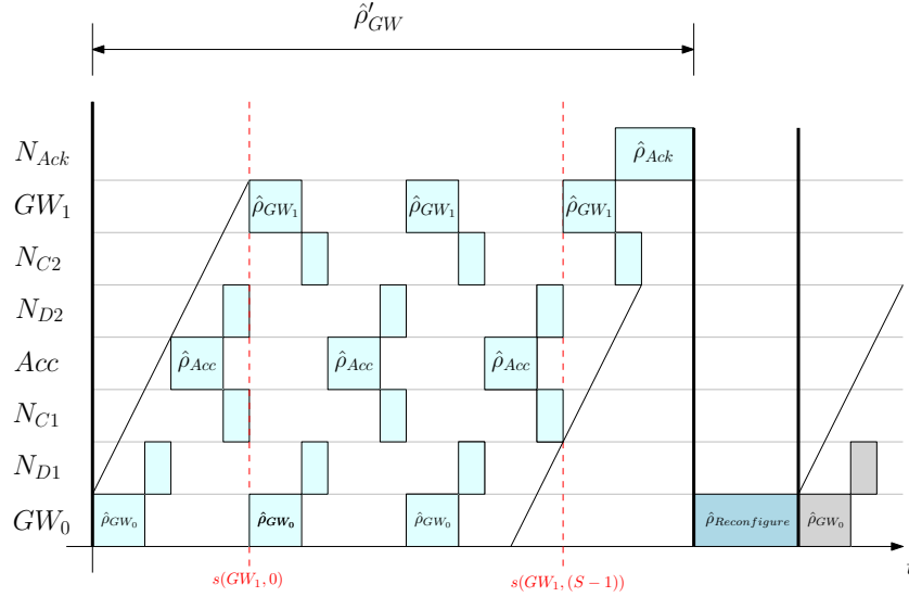
Figure 6.15: Execution schedule ( \delta_0 = 1, \delta_1 = 1, S = 3 ). For simplicity each pair of network-actors ( R_* and L_* ) is replaced by a single actor N_* .
