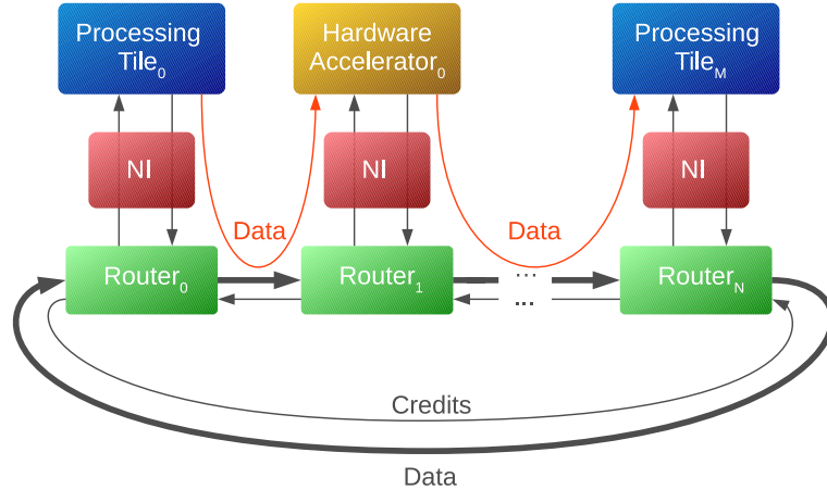
Figure 1.3: Schematic overview with one hardware accelerator, connected to the Nebula ring interconnect
