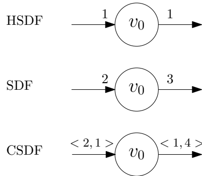
Figure 6.1: Visualization of a number of dataflow models
