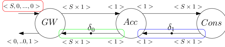
Figure 4.5: CSDF graph of an accelerator pipeline
