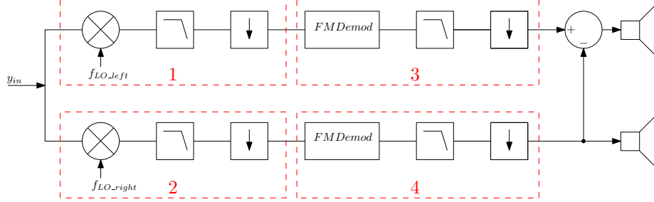
Figure 7.9: Partitioned FM decoding pipeline
