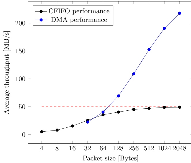
Figure 5.7: DMA performance measurements. The dashed line in red illustrates the theoretical maximum CFIFO performance
