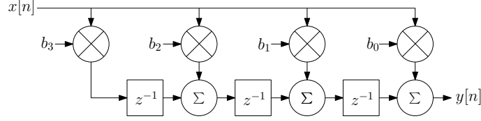
Figure 7.6: FIR filter structure (Direct Form II (Transposed form), N = 3 )
