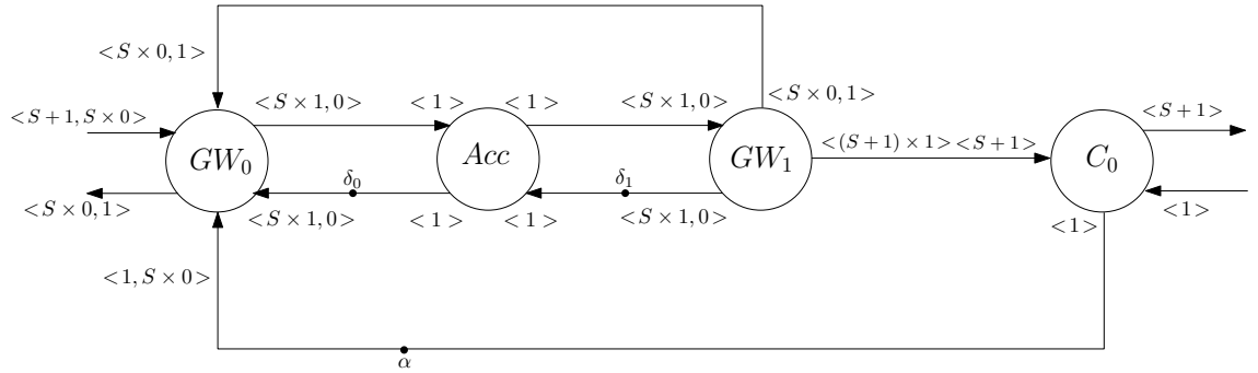
Figure 6.10: CSDF model: Back-edge added
