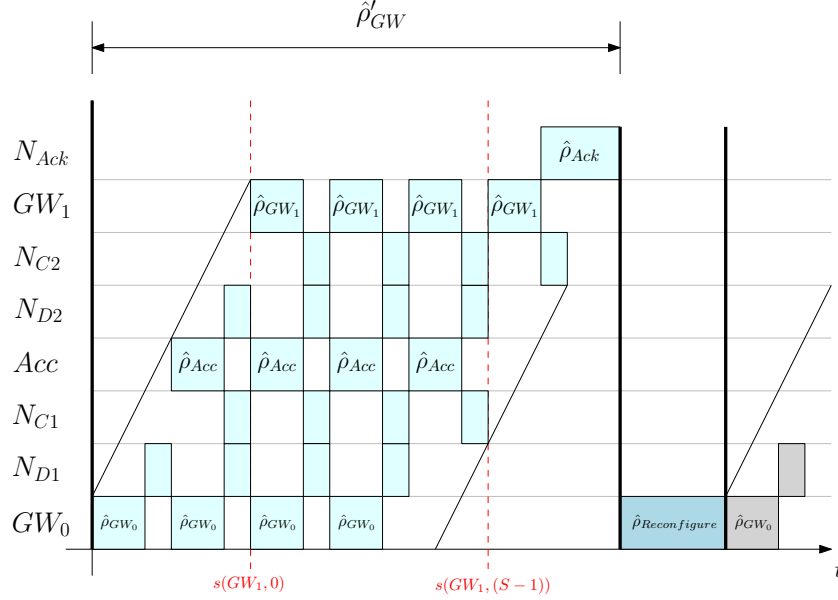
Figure 6.17: ROSPS execution schedule ( \delta_0 = 2, \delta_2 = 1, S = 4 ). For simplicity each pair of network-actors ( R_* and L_* ) is replaced by a single actor N_* .
