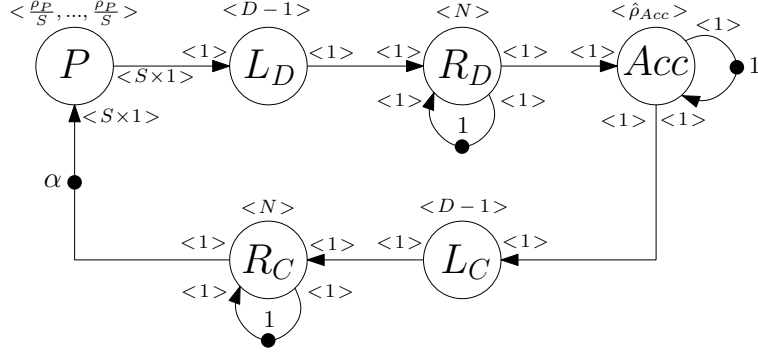
Figure 6.5: CSDF accelerator communication model
