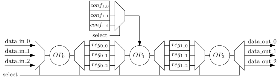
Figure 4.2: Hardware Accelerator pipeline with duplicated registers
