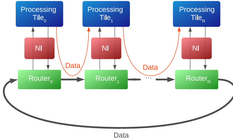
Figure 1.2: Schematic overview of the Nebula ring
