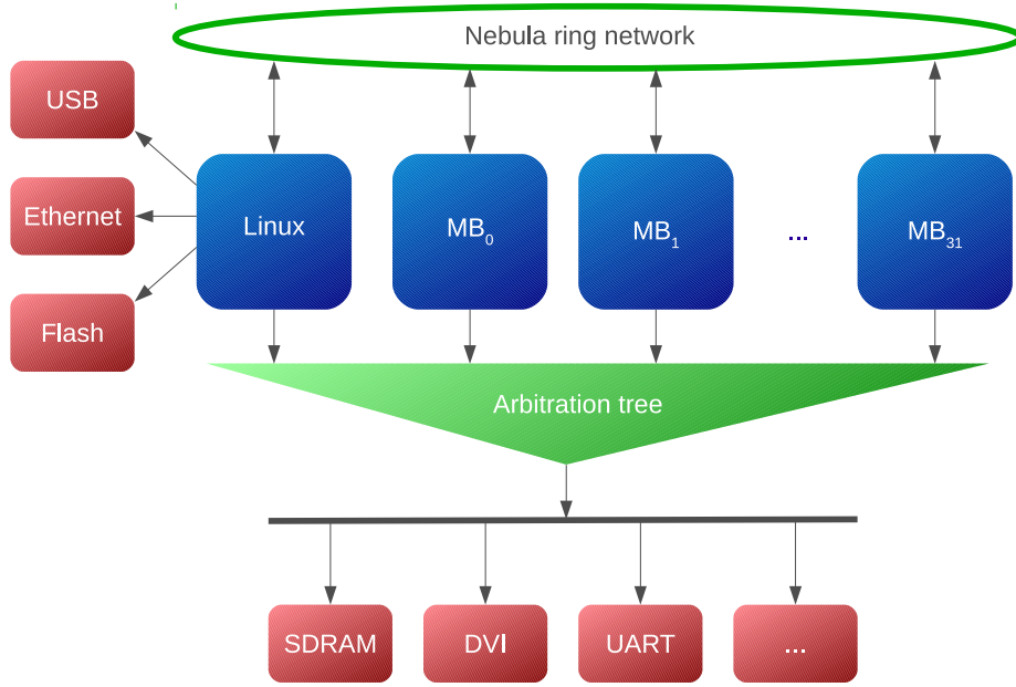
Figure 1.1: High level overview of the Starburst platform (the arrows indicate master/slave relations)
