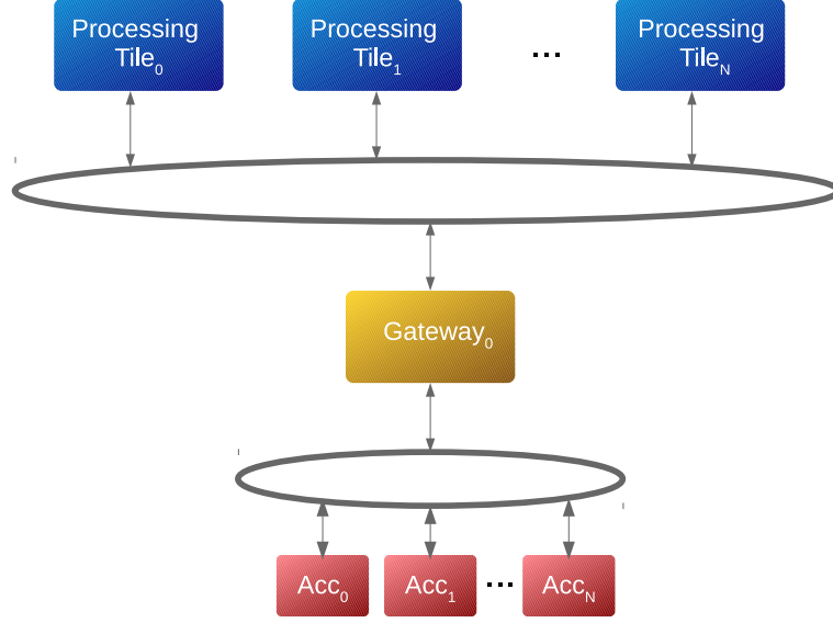
Figure 8.1: Separate Accelerator Network
