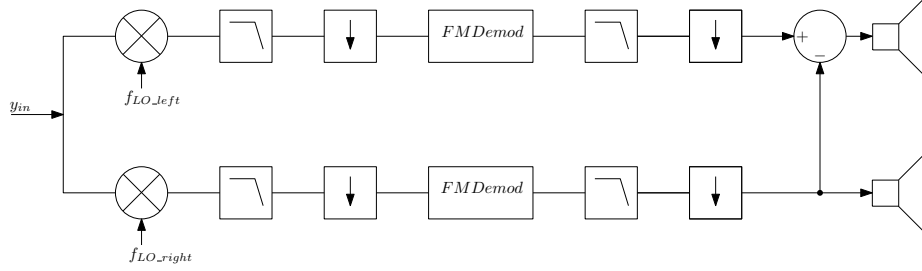
Figure 7.2: FM decoding pipeline
