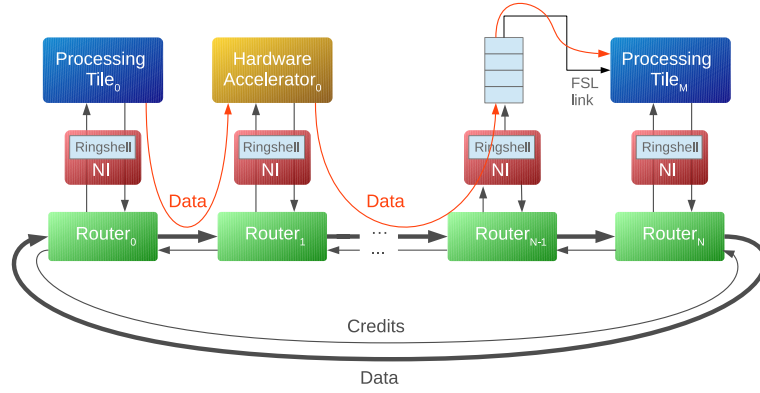
Figure 3.7: Schematic overview of two processing tiles and one hardware accelerator, connected to the Nebula ring interconnect.
