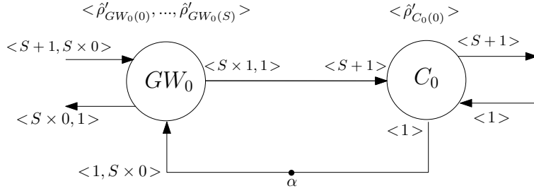
Figure 6.7: CSDF model: CFIFO communication protocol
