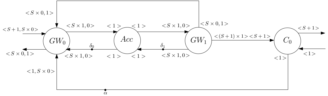
Figure 6.12: CSDF model
