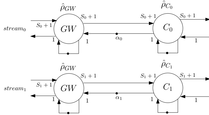
Figure 6.19: SDF model multiple data streams
