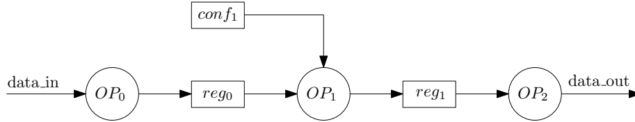
Figure 4.1: Hardware Accelerator pipeline
