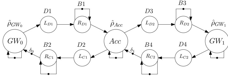
Figure 6.13: HSDF model of two gateways and one hardware accelerator
