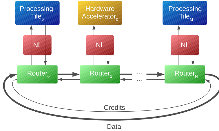
Figure 3.6: Schematic overview of two processing tiles and one hardware accelerator, connected to the Nebula ring interconnect
