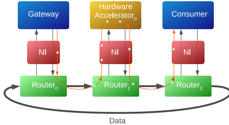
Figure 4.4: Non-preemption example: a gateway and a consumer are communicating data via a Hardware Accelerator
