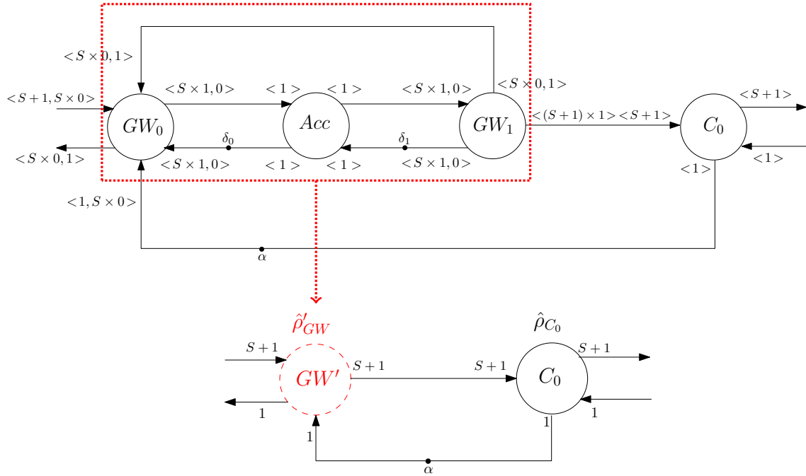
Figure 6.11: CSDF model: Abstraction
