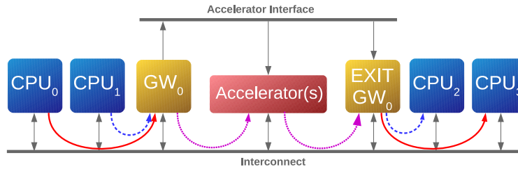
Figure 5.9: Hardware Accelerator sharing overview, including exit gateway
