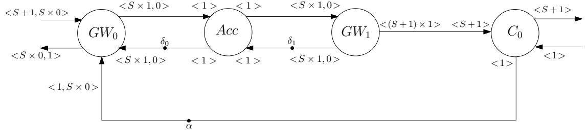
Figure 6.9: CSDF model: Exit Gateway added
