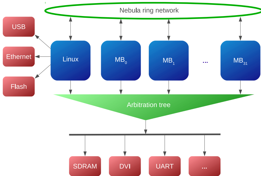
Figure 3.2: High level overview of the Starburst platform. Arrows indicate master-slave relations.
