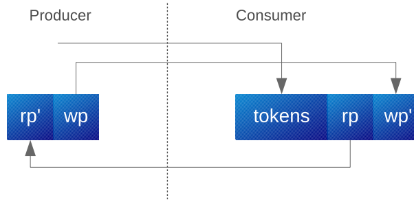
Figure 3.8: CFIFO administration overview
