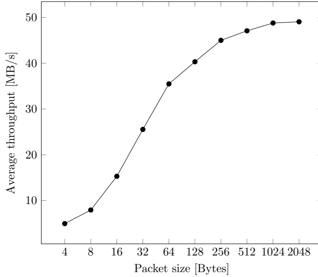
Figure 5.3: CFIFO performance measurements
