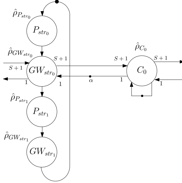
Figure 6.18: SDF model multiple data streams
