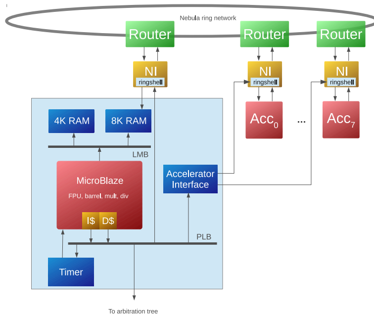
Figure 5.2: Gateway overview, including Accelerator Interface
