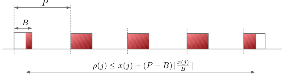
Figure 2.6: Execution of a task during its time slices
