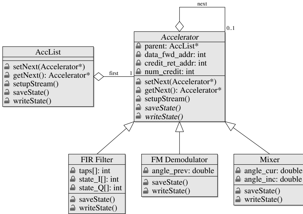
Figure 5.11: UML diagram accelerator administration
