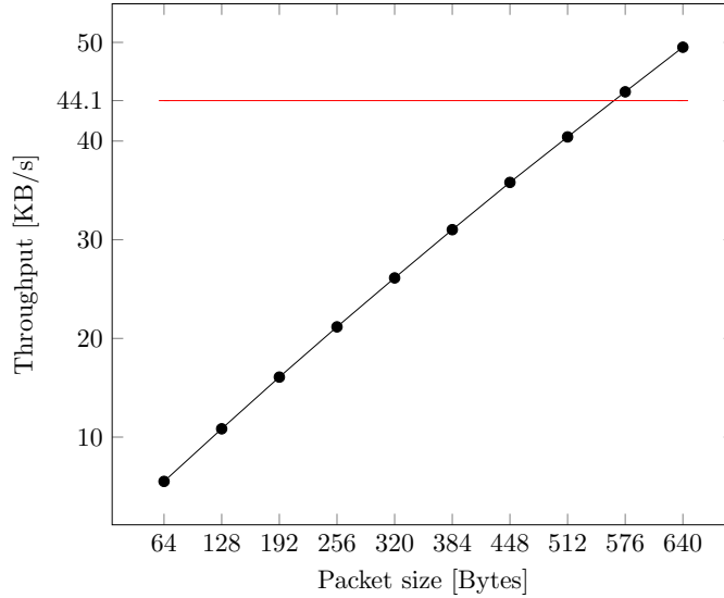
Figure 7.10: PAL audio decoder performance measurements. The red line at 44.1KB/s depicts the minimal throughput which results in a continuous (real-time) audio stream.
