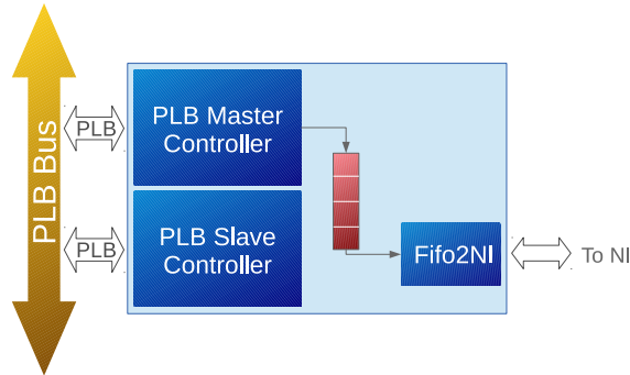
Figure 5.5: Schematic overview of the RingDMA controller
