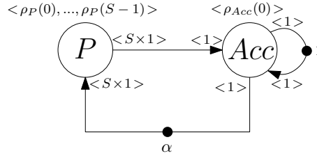
Figure 6.4: CSDF accelerator communication model
