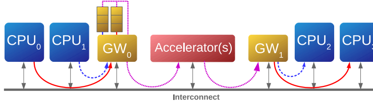
Figure 4.3: Hardware Accelerator sharing via gateways
