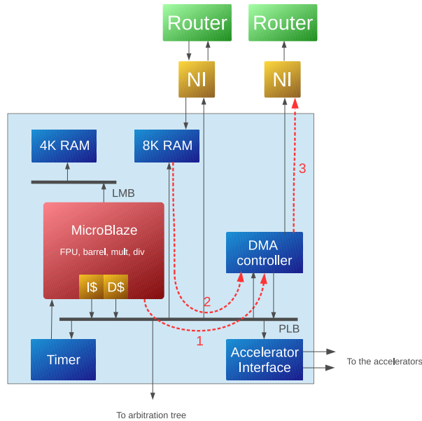
Figure 5.6: Gateway overview, including custom DMA Controller
