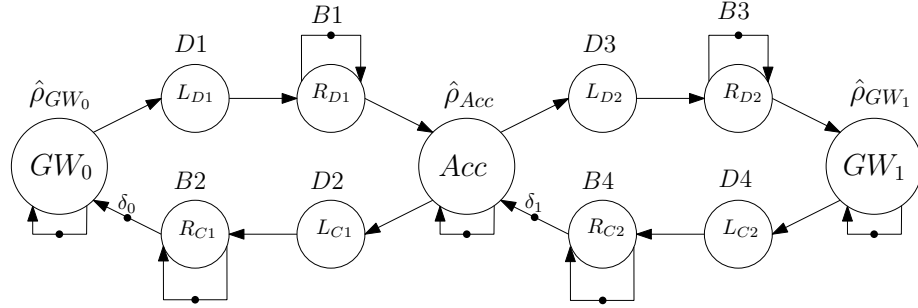
Figure 6.14: HSDF model of two gateways and one hardware accelerator
