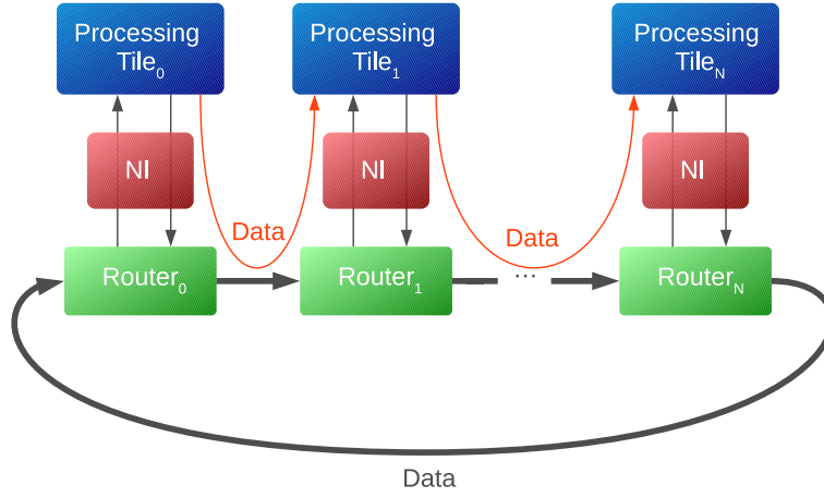
Figure 3.5: Schematic overview of the Nebula ring
