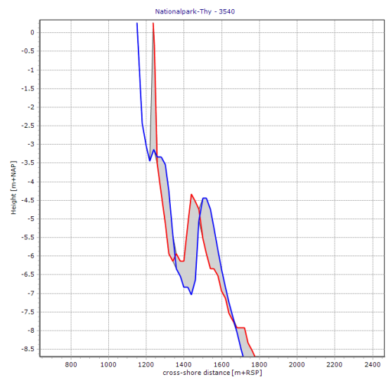
Figure 80: Transect km 30.7 in year 1938 (red) and 1955 (blue)
