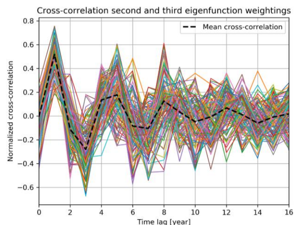
Figure 93: Cross-correlation of the second and third eigenfunction of the Holland coast, pre-nourishment data. Profiles between km. 56 and 90.
