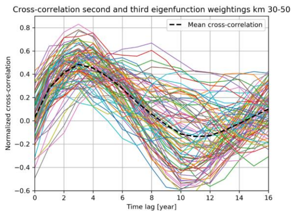
Figure 91: Normalized cross-correlation for section km. 30-50 of the Holland coast, pre-nourishment data
