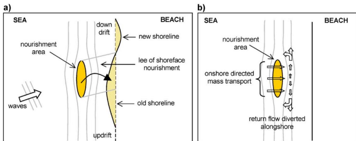
Figure 4: (a) Lee and (b) feeder effect of a shoreface nourishment (Van Duin et al., 2004)
