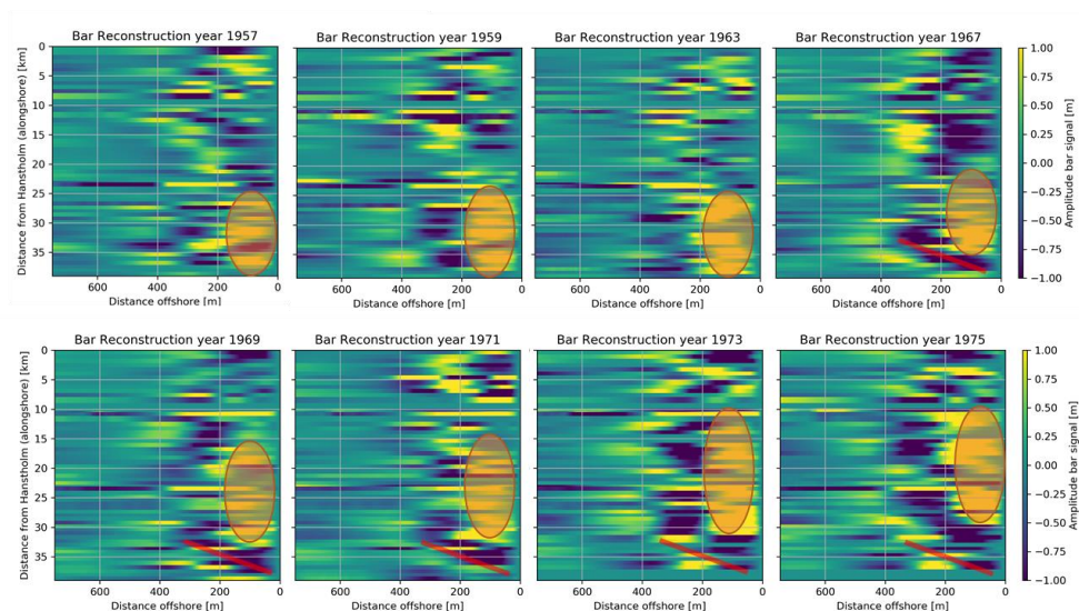
Figure 100: Bar reconstruction Nationalpark Thy 1957-1975
