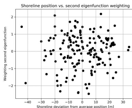
Figure 43: Relation between the position of the shoreline and the second eigenfunction weighting between km. 12 and 21
