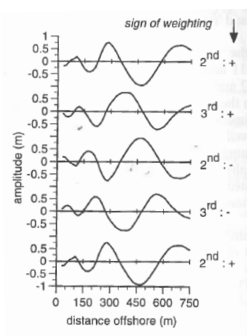
Figure 17: Visualisation of offshore moving bar based on successive dominant eigenfunctions (Wijnberg, 1995)
