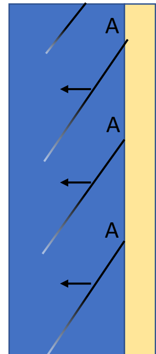
Figure 45: Schematisation of bar migration along the Midtjylland coast. Arrows indicate the migration of the nearshore sandbars (black lines). White ends indicate the fading out of the bar offshore. The 'A's represent development of a new bar close to the shore.
