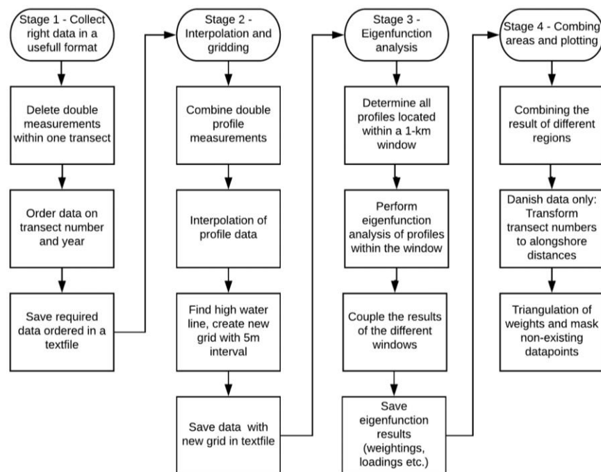
Figure 20: Overview of data-processing
