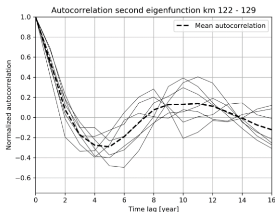
Figure 95: Autocorrelation second eigenfunction km. 122 - 129
