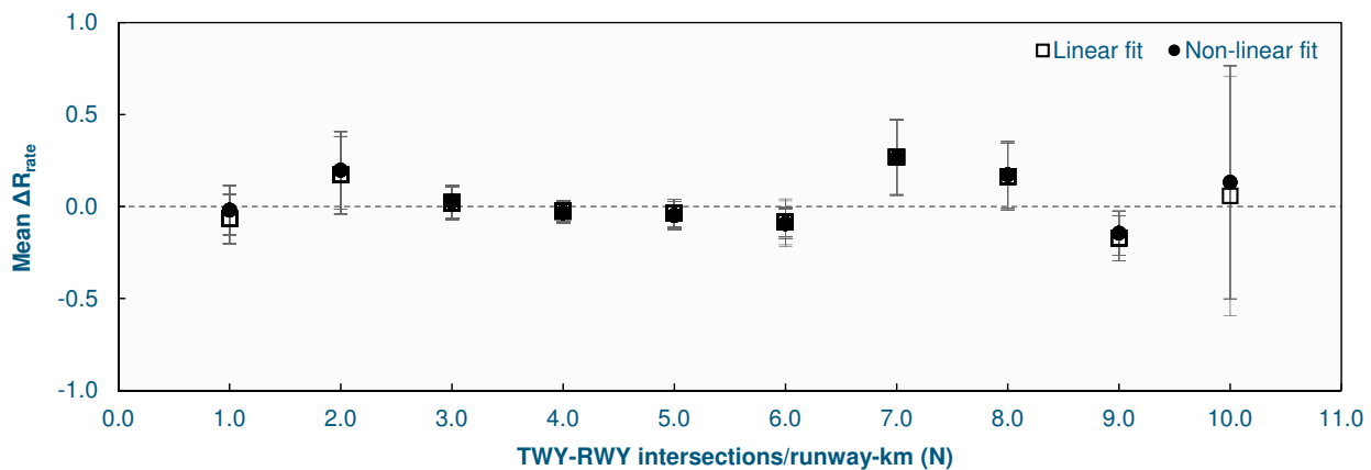
Figure 7-3: Plot of mean residuals for number of TWY-RWY intersections per runway-km variable
