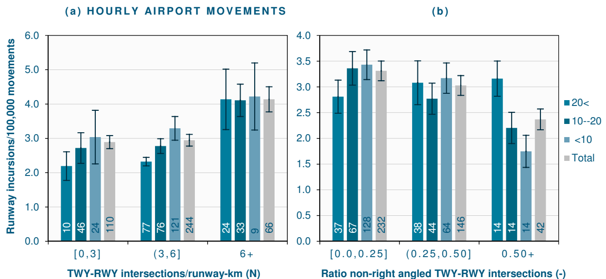
Figure 6-11: Incursion rate for number of TWY-RWY intersections per runway-km (a) and ratio non-right angled TWY-RWY intersections per hourly airport movements category (b), including 1 \sigma errors
