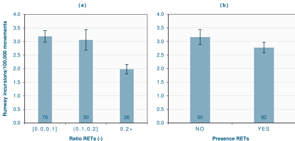
Figure 6-12: Incursion rate for ratio RETs (a) and for presence of RETs (b), including 1σ errors
