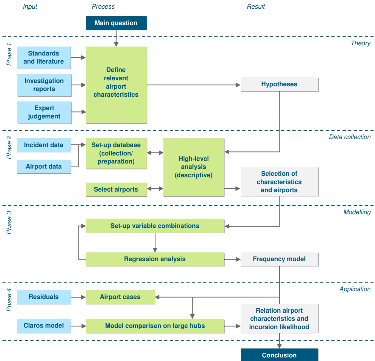
Figure 3-1: Research framework
