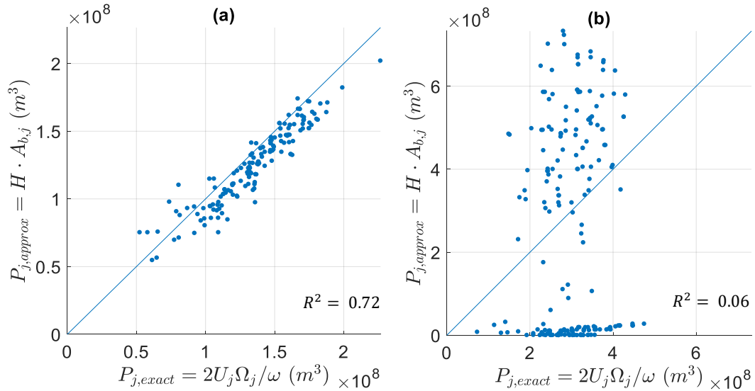
Fig. 4.8: Scatter plot of P_{j,approx} vs. P_{j,exact} for the Wadden Sea parameter set (see Table 2.1) with (a) a basin length of 2 km instead of 10 km and (b) a basin width of 50 km instead of 100 km, where R^2 is the coefficient of determination and the line represents the ideal situation in which the approximated and the actual tidal prisms are equal.
