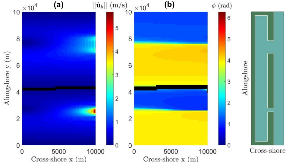
Fig. 3.2: Surface plots of (a) ||\hat{\mathbf{u}}_b|| and (b) \phi , showing the tidal divide (in black) according to (a) method 1 and (b) method 2, with two open inlets of inlet width 3 km and 10 km (so differently-sized) at y = 25 km and y = 75 km.
