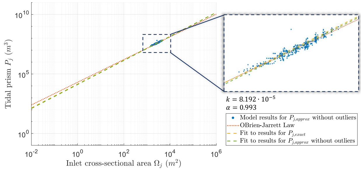
Fig. 4.6: Scatter plot of tidal prisms P_{j,approx} vs. inlet areas \Omega_j in equilibrium, with the O'Brien-Jarrett Law and the function that is fitted to the data without outliers (Georgia Bight).
