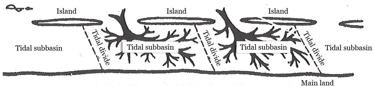
Fig. 1.4: Simplistic overview of tidal divides forming boundaries between tidal subbasins in a multi-inlet tidal system (Stive and Wang, 2003).
