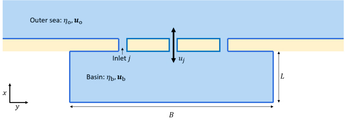
Fig. 2.1: Model geometry of a multi-inlet tidal system consisting of the outer sea that is connected to a basin by J ( J = 3 in this example) tidal inlets, where the arrow u_j denotes the flow velocity of the inflow and outflow of water through the inlets.
