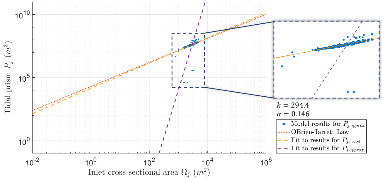
Fig. 4.5: Scatter plot of tidal prisms P_{j,approx} vs. inlet areas \Omega_j in equilibrium, with the O'Brien-Jarrett Law and the function that is fitted to the data (Georgia Bight).
