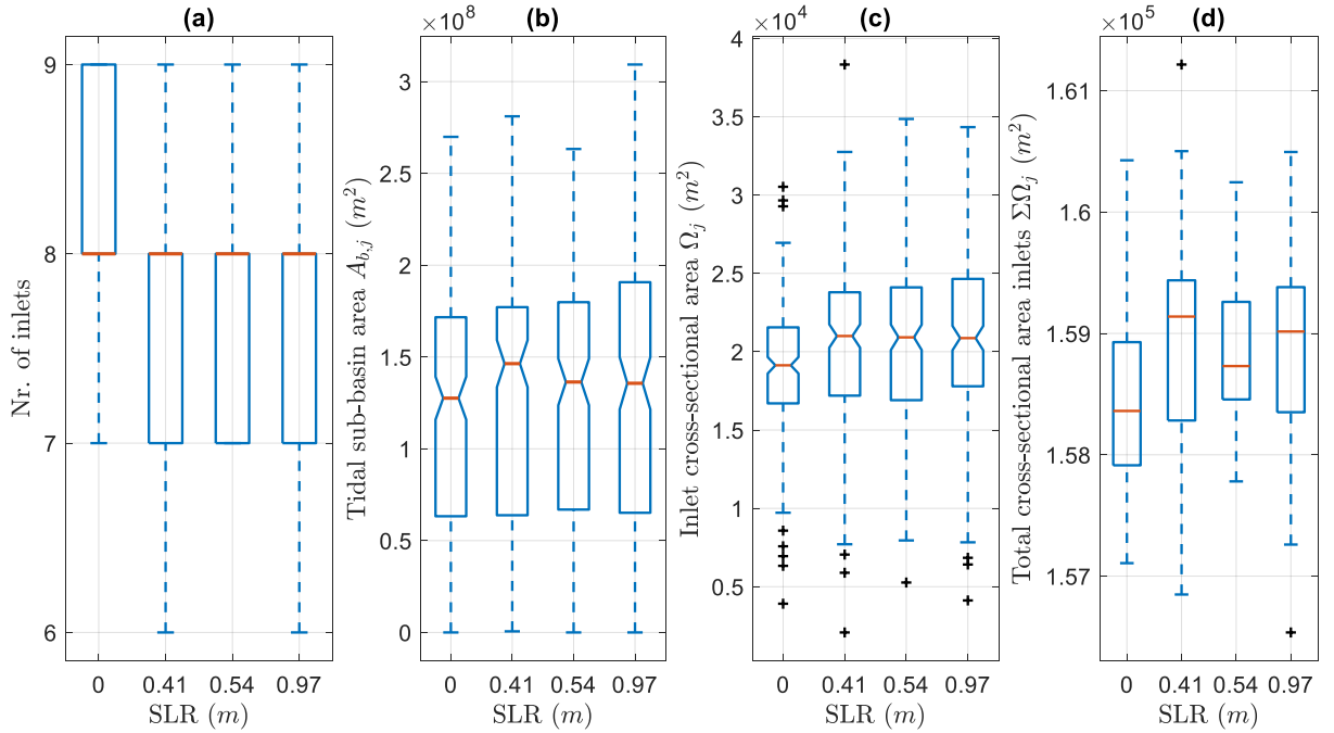
Fig. 5.1: The response of the (a) number of inlets, (b) tidal subbasin area, (c) inlet cross-sectional area per inlet and (d) total cross-sectional inlet area to the expected sea level rise until 2100.
