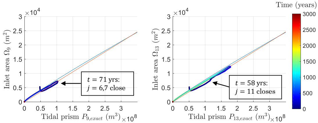
Fig. 4.12: The development of P_j and \Omega_j over time t , for inlets j = 9 and 13 (two of the 32 inlets that are closed in equilibrium).
