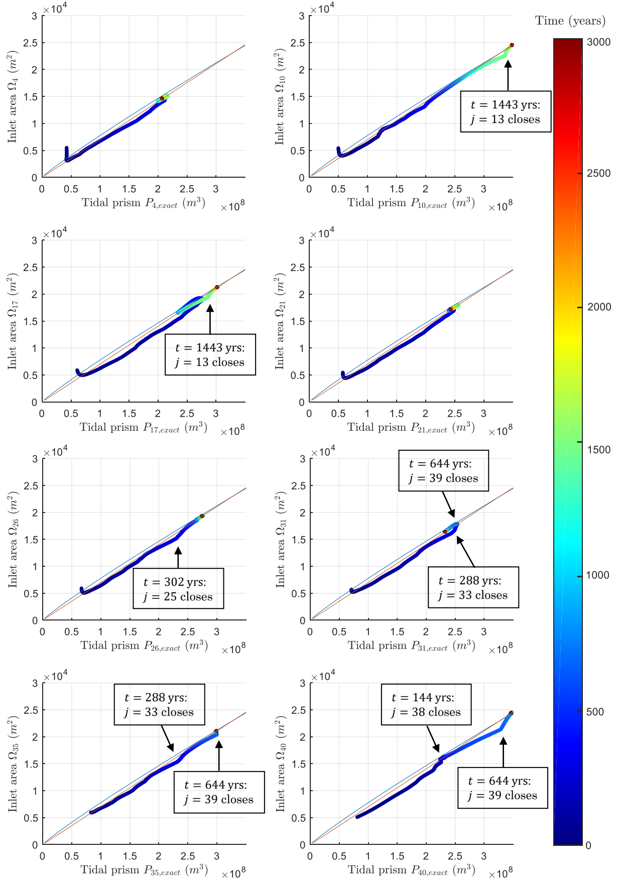
Fig. 4.10: The development of P_{j,exact} and \Omega_j over time t , for inlets j = 4, 10, 17, 21, 26, 31, 35, 40 (the inlets that remain open in equilibrium).
