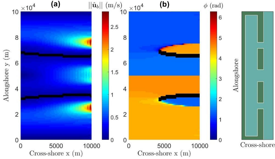
Fig. 3.5: Surface plots of (a) ||\hat{\mathbf{u}}_b|| and (b) \phi , showing the tidal divide (in black) according to (a) method 1 and (b) method 2, with three open inlets of inlet width 5 km, 10 km and 5 km (so differently-sized) at y = 25 km, y = 50 km and y = 75 km.
