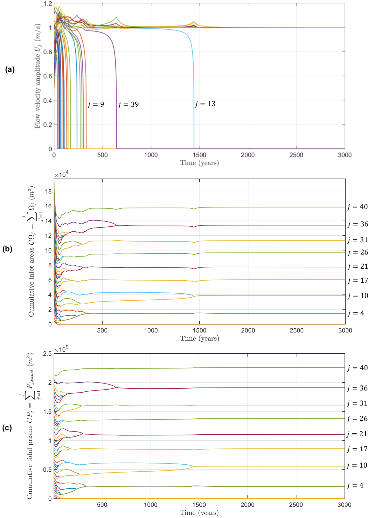
Fig. 4.11: The temporal development of (a) flow velocity amplitude U_j per inlet j , (b) cumulative inlet areas C\Omega_j (see Eq. (4.12)) and (c) cumulative tidal prisms CP_j (see Eq. (4.12)).
