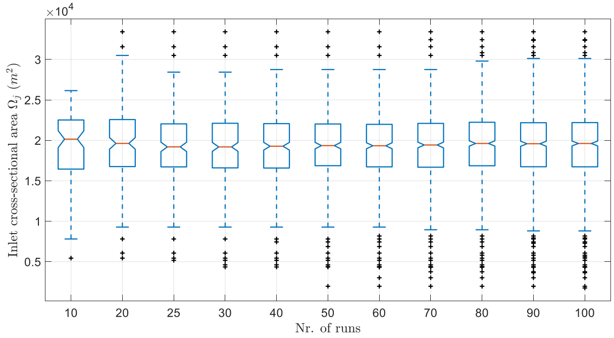
Fig. B3: Boxplots of the cross-sectional areas per inlet resulting from 10, 20, 25, 30, 40, 50, 60, 70, 80, 90 and 100 model runs.
