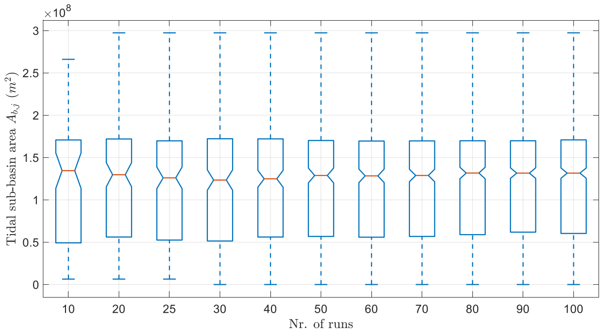
Fig. B2: Boxplots of the tidal subbasin areas resulting from 10, 20, 25, 30, 40, 50, 60, 70, 80, 90 and 100 model runs.
