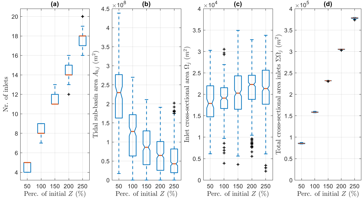
Fig. 5.4: The response of the (a) number of inlets, (b) tidal subbasin area, (c) inlet area per inlet and (d) total inlet area to changes in the tidal amplitude Z .
