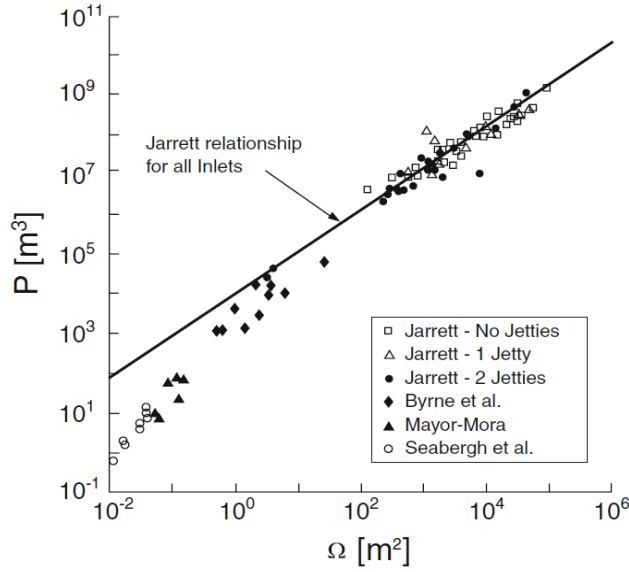
Fig. 4.1: Tidal prism P vs. equilibrium cross-sectional area \Omega , for field and laboratory data (D'Alpaos et al., 2009).
