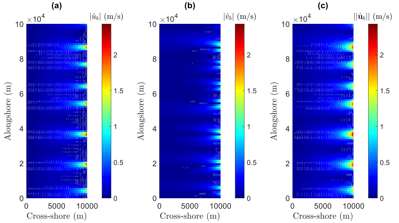
Fig. A2: Surface plot of the flow velocity amplitudes in the basin: (a) the magnitude of the complex flow velocity amplitude in the cross-shore x -direction, |u_b| (see Eq. (2.21)) (b) the magnitude of the complex flow velocity amplitude in the alongshore y -direction, |v_b| (see Eq. (2.21)) (c) The complex norm of the complex flow velocity amplitude vector, ||u_b|| (see Eq. (3.1)).
