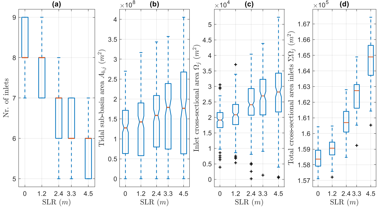
Fig. 5.2: The response of the (a) number of inlets, (b) tidal subbasin area, (c) inlet area per inlet and (d) total inlet area to sea level rise on a millennial scale.
