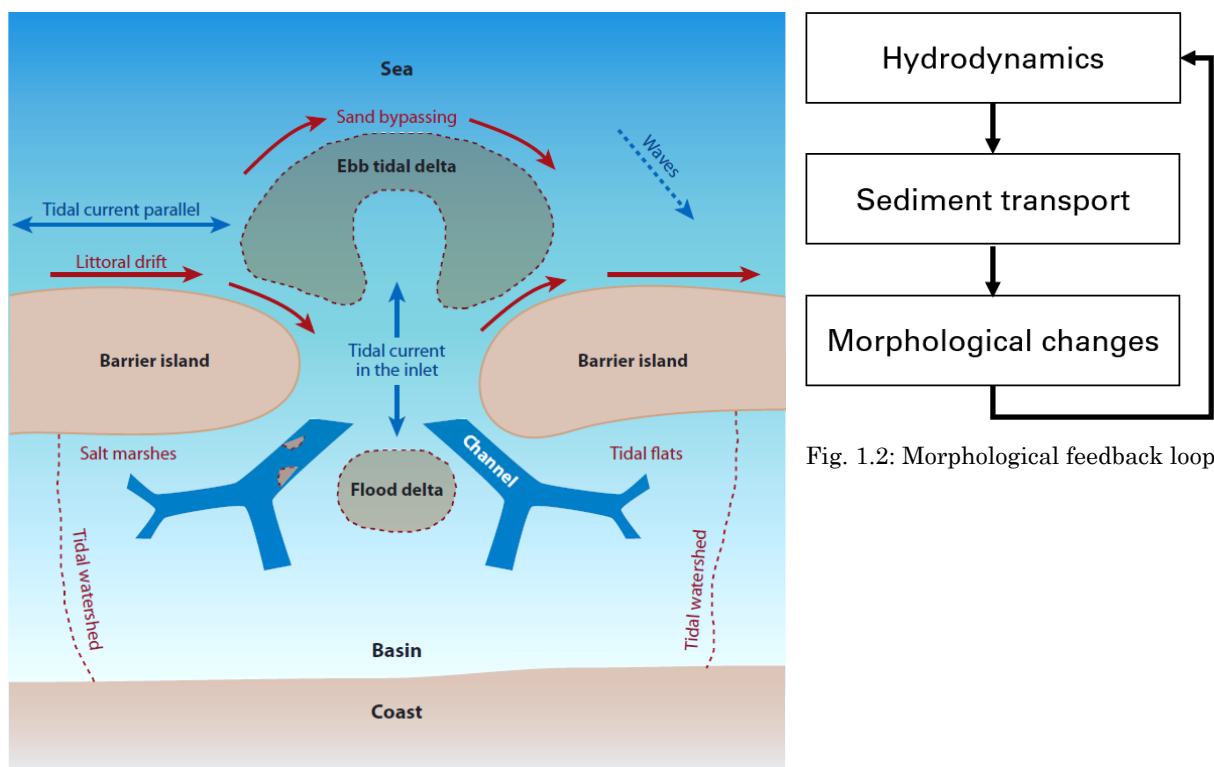
Fig. 1.1: Schematized overview of a tidal inlet system, including the different geomorphic elements and physical processes (De Swart and Zimmerman, 2009).
