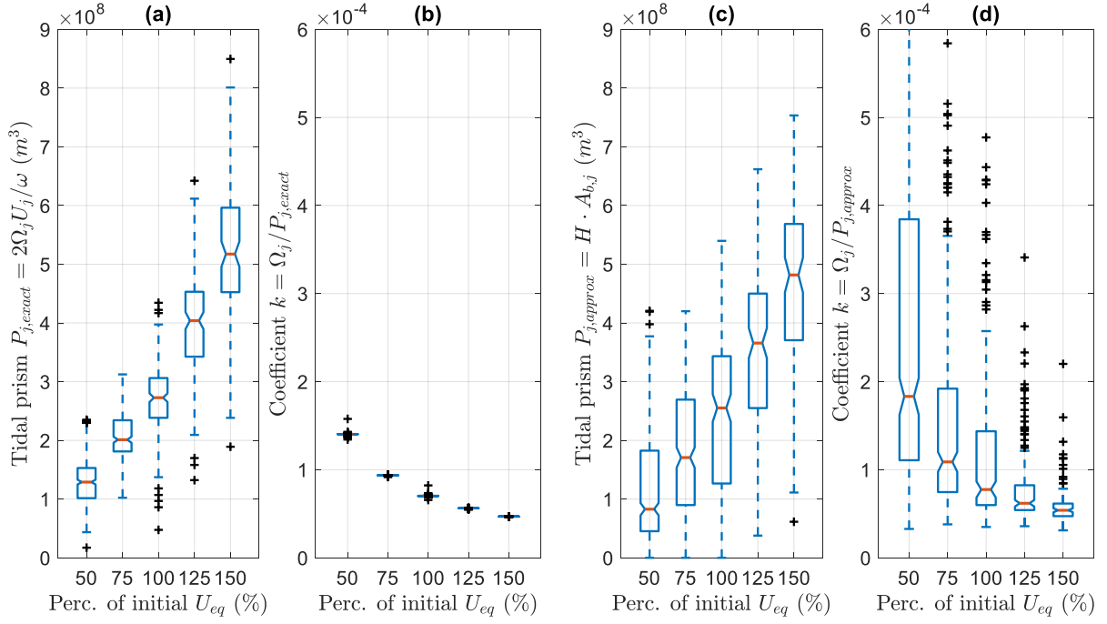
Fig. 5.7: The response of (a) tidal prism P_{j,exact} , (b) coefficient k = \Omega_j / P_{j,exact} , (c) tidal prism P_{j,approx} and (d) coefficient k = \Omega_j / P_{j,approx} to changes in the equilibrium velocity U_{eq} (and corresponding sediment import M ).
