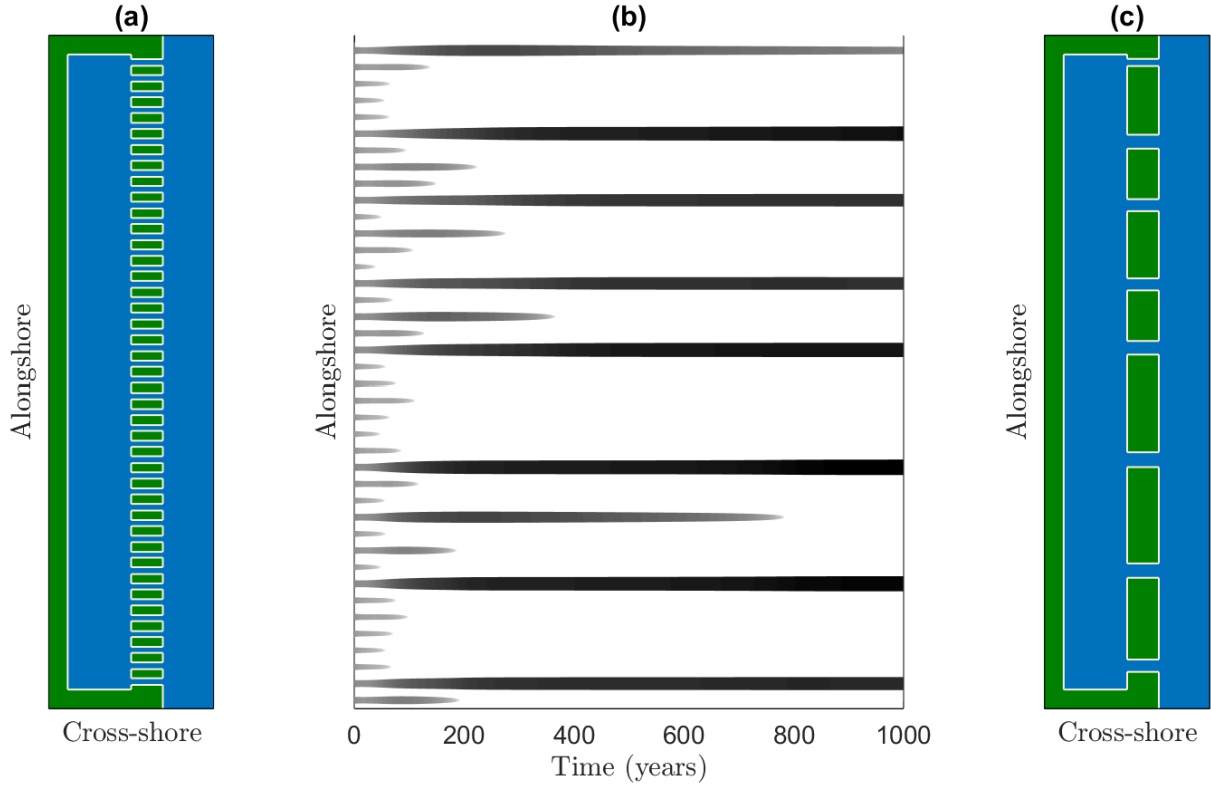
Fig. A1: Model geometry and example of a simulation, using parameter values for the Wadden Sea: (a) the initial state, shown as a plan view of the geometry with a prescribed number of 40 inlets, (b) the inlet evolution over time, showing that 32 inlets close and 8 remain open, (c) the state after 1,000 timesteps, shown as a plan view of the geometry with 8 open inlets.
