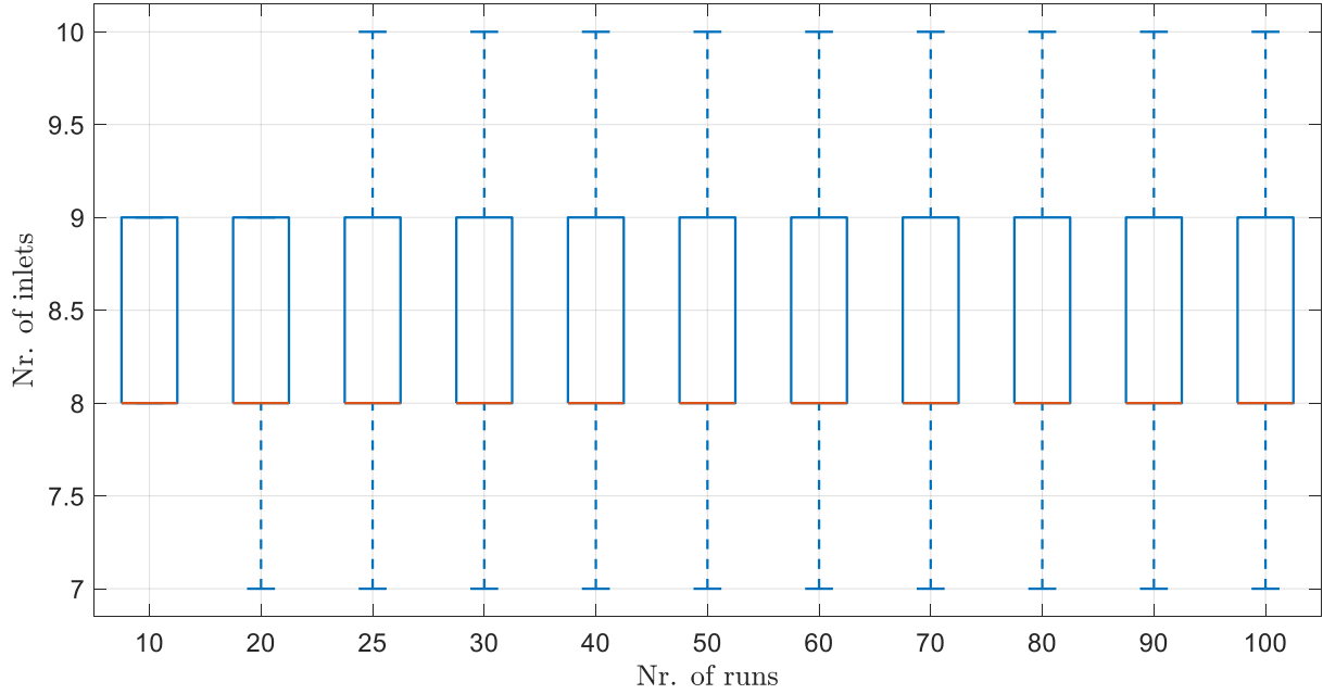
Fig. B1: Boxplots of the number of inlets resulting from 10, 20, 25, 30, 40, 50, 60, 70, 80, 90 and 100 model runs.
