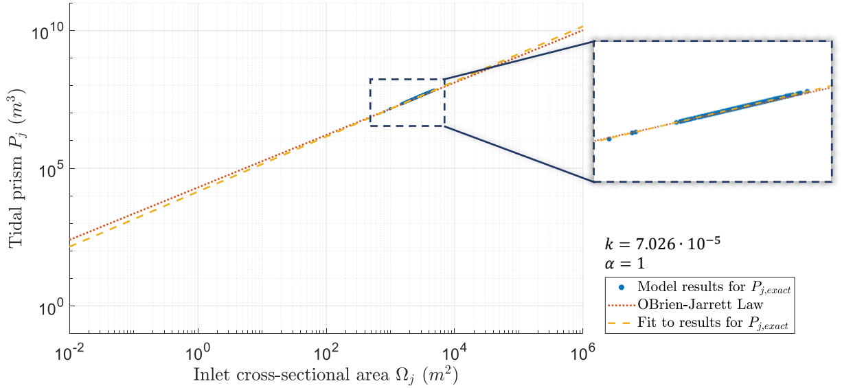
Fig. 4.4: Scatter plot of tidal prisms P_{j,exact} vs. inlet areas \Omega_j in equilibrium, with the O'Brien-Jarrett Law and the function that is fitted to the data (Georgia Bight).
