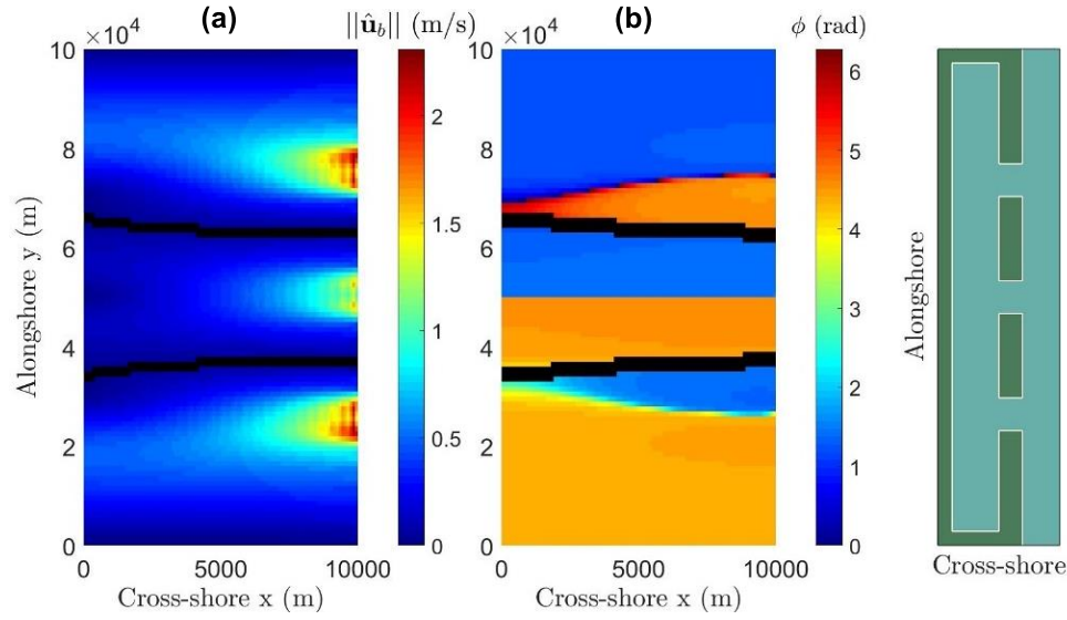
Fig. 3.3: Surface plots of (a) ||\hat{\mathbf{u}}_b|| and (b) \phi , showing the tidal divide (in black) according to (a) method 1 and (b) method 2, with three open inlets of inlet width 7 km (so equally-sized) at y = 25 km, y = 50 km and y = 75 km.
