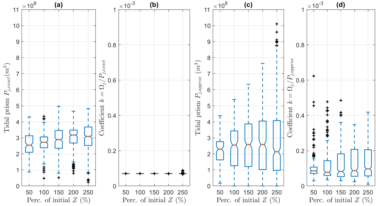
Fig. 5.5: The response of (a) tidal prism P_{j,exact} , (b) coefficient k = \Omega_j/P_{j,exact} , (c) tidal prism P_{j,approx} and (d) coefficient k = \Omega_j/P_{j,approx} to changes in tidal amplitude Z .
