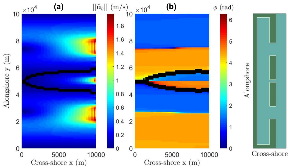
Fig. 3.4: Surface plots of (a) ||\hat{\mathbf{u}}_b|| and (b) \phi , showing the tidal divide (in black) according to (a) method 1 and (b) method 2, with three open inlets of inlet width 10 km, 2 km and 10 km (so differently-sized) at y = 25 km, y = 50 km and y = 75 km.
