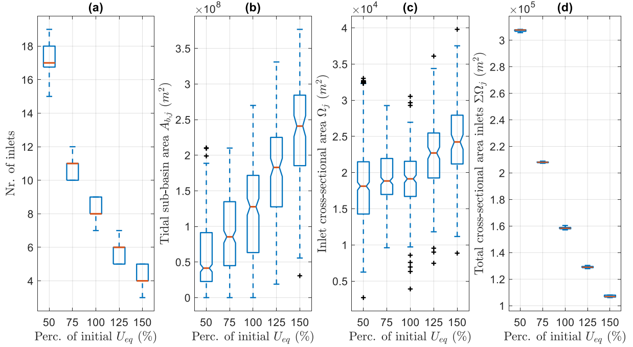
Fig. 5.6: The response of the (a) number of inlets, (b) tidal subbasin area, (c) inlet area per inlet and (d) total inlet area to changes in the equilibrium velocity U_{eq} (and corresponding sediment import M ).
