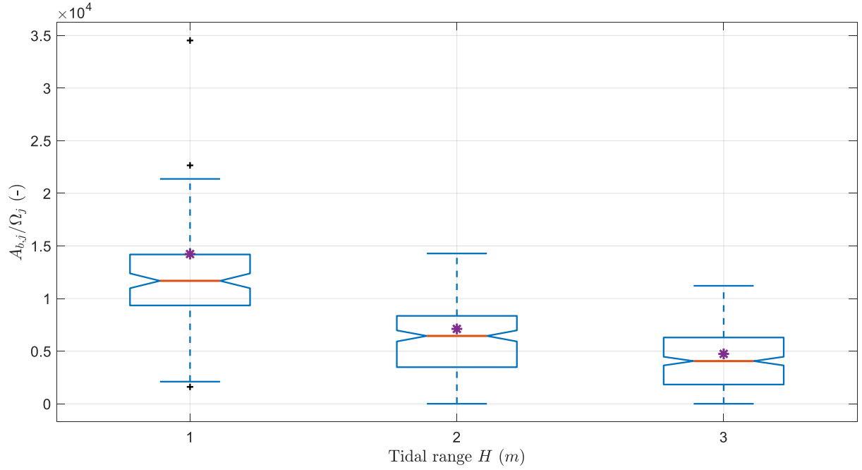
Fig. C1: The basin area A_{b,j} divided by the inlet area \Omega_j for varying tidal range H (where H = 2Z for tidal amplitude Z ), where the purple asterisk represents the expected value of 2U_{eq}/\omega H .
