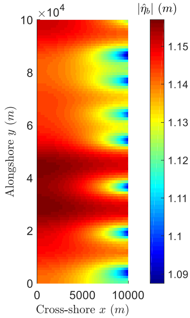
Fig. A3: Surface plot of the magnitude of the complex elevation amplitude in the basin, |\hat{h}_b| .
