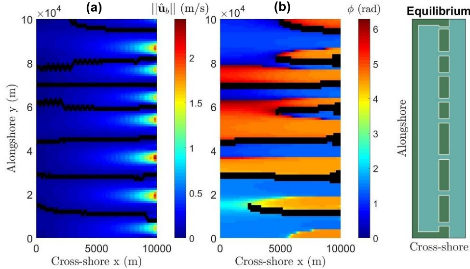
Fig. 3.7: Surface plots of (a) ||\hat{\mathbf{u}}_b|| and (b) \phi , showing the tidal divide (in black) for (a) method 1 and (b) method 2, for an equilibrium situation for the Wadden Sea parameter values, as shown in the most right figure (see Table 2.1).
