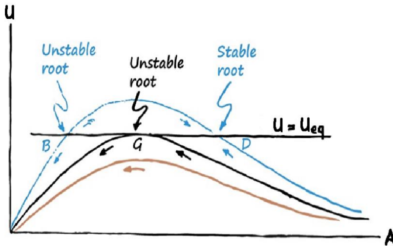
Fig. 1.3: Escoffier diagram (Escoffier, 1940), showing three possible closure curves, the equilibrium velocity U_{eq} and the stable and unstable roots resulting from intersections of the U -curves with the line U = U_{eq} .
