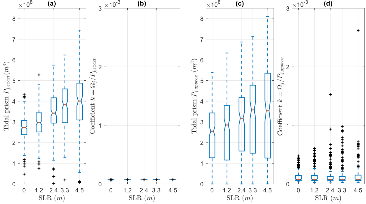
Fig. 5.3: The response of (a) tidal prism P_{j,exact} , (b) coefficient k = \Omega_j / P_{j,exact} , (c) tidal prism P_{j,approx} and (d) coefficient k = \Omega_j / P_{j,approx} to sea level rise (implemented as increased initial water depth in basin and ocean).
