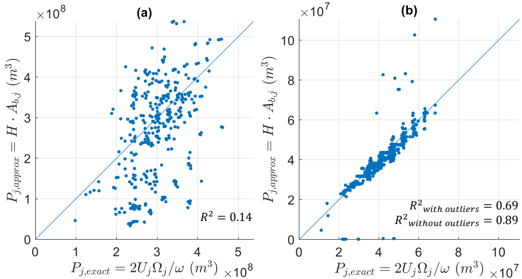
Fig. 4.7: Scatter plot of P_{j,approx} vs. P_{j,exact} for (a) the Wadden Sea parameter set and (b) the Georgia Bight parameter set (see Table 2.1), where R^2 is the coefficient of determination and the line represents the ideal situation in which the approximated and the actual tidal prisms are equal.
