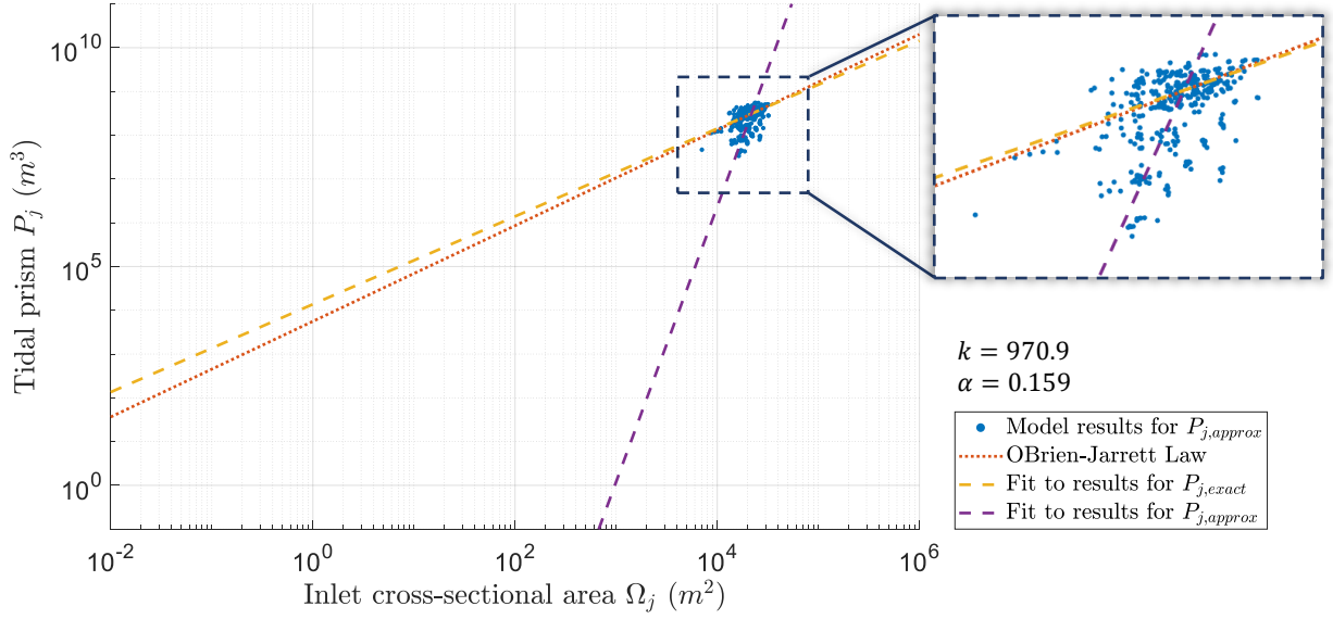
Fig. 4.3: Scatter plot of tidal prisms P_{j,approx} vs. inlet areas \Omega_j in equilibrium, with the O'Brien-Jarrett Law and the function that is fitted to the data (Wadden Sea).
