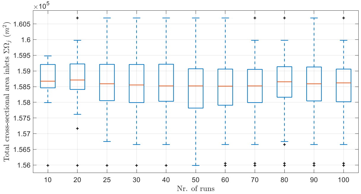
Fig. B4: Boxplots of the total cross-sectional areas per run resulting from 10, 20, 25, 30, 40, 50, 60, 70, 80, 90 and 100 model runs.
