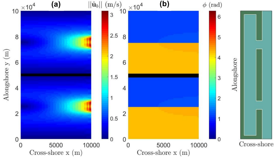
Fig. 3.1: Surface plots of (a) ||\hat{\mathbf{u}}_b|| and (b) \phi , showing the tidal divide (in black) according to (a) method 1 and (b) method 2, with two open inlets of inlet width 7 km (so equally-sized) at y = 25 km and y = 75 km.
