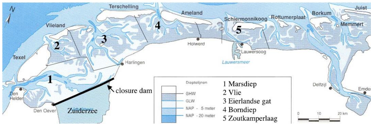
Fig. 1.5: The (approximate) tidal divides and tidal subbasins in the Wadden Sea (Kragtwijk et al., 2004).
