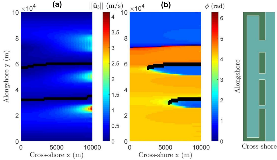
Fig. 3.6: Surface plots of (a) ||\hat{\mathbf{u}}_b|| and (b) \phi , showing the tidal divide (in black) according to (a) method 1 and (b) method 2, with three open inlets of inlet width 3 km, 5 km and 10 km (so differently-sized) at y = 25 km, y = 50 km and y = 75 km.
