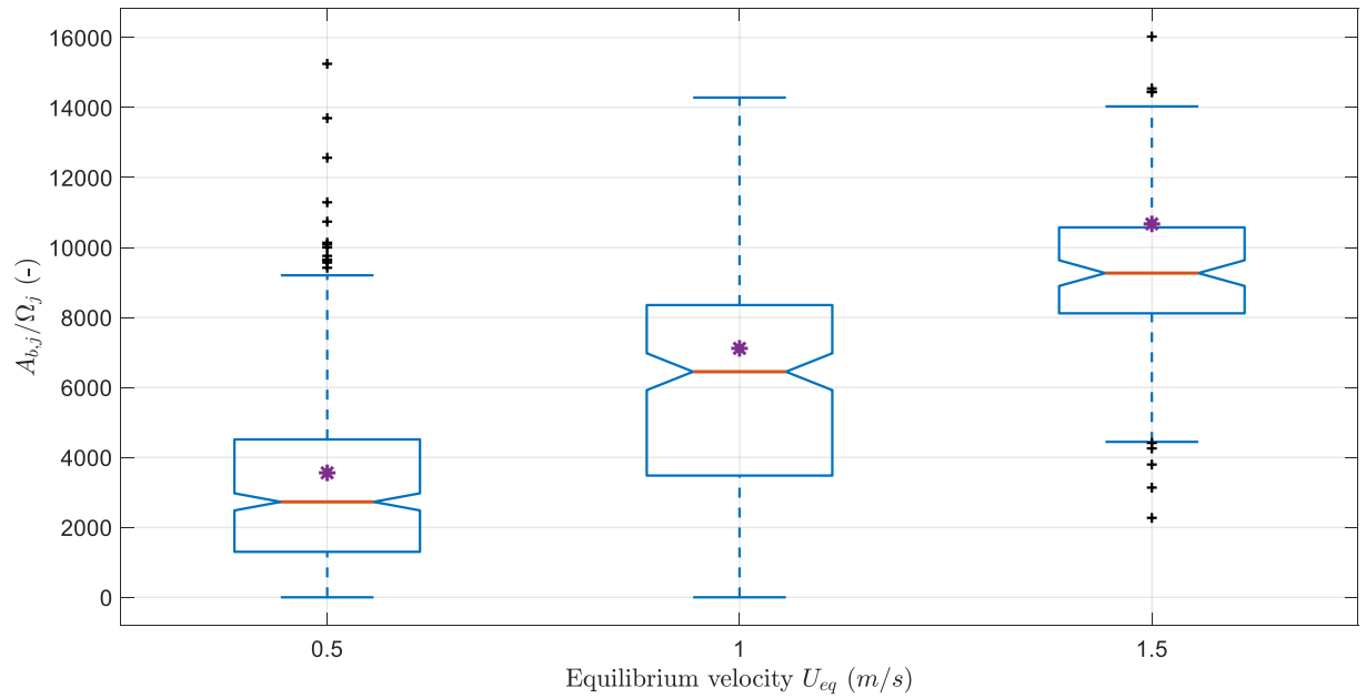
Fig. C2: The basin area A_{b,j} divided by the inlet area \Omega_j for varying equilibrium velocity U_{eq} (and corresponding sediment import M ), where the purple asterisk represents the expected value of 2U_{eq}/\omega H .
