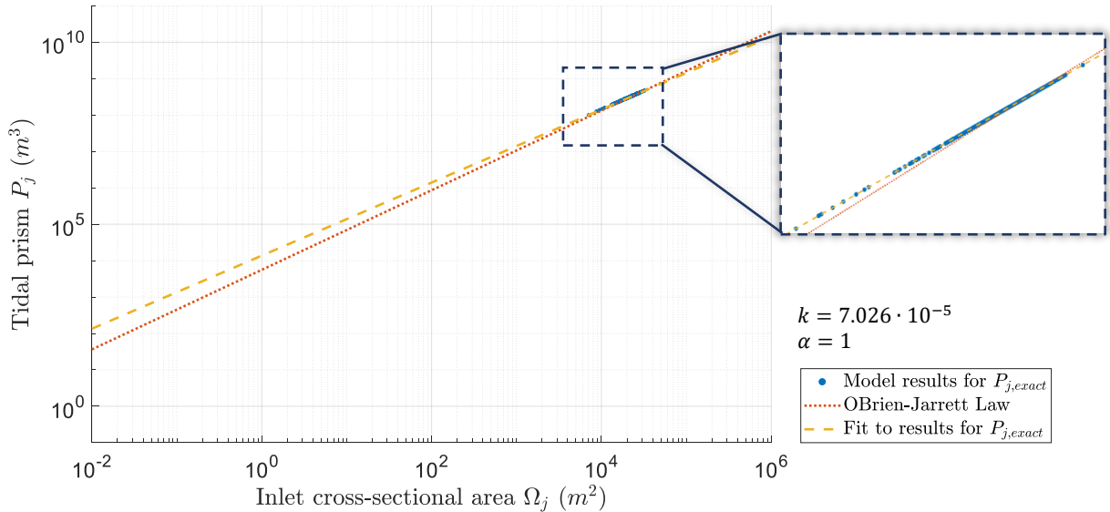
Fig. 4.2: Scatter plot of tidal prisms P_{j,exact} vs. inlet areas \Omega_j in equilibrium, with the O'Brien-Jarrett Law and the function that is fitted to the data (Wadden Sea).
