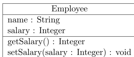
Figure 2.2: A class in a class diagram
