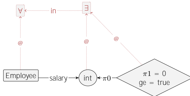
Figure 6.4: The positiveSalary invariant in GROOVE.
