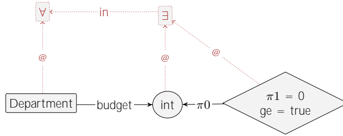
Figure 2.7: The rule graph that corresponds to: context Department inv: self.budget >= 0.
