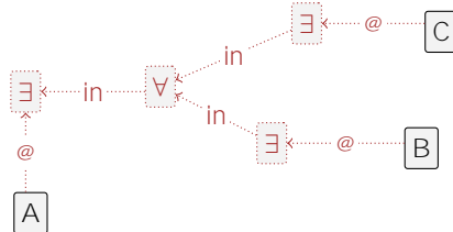
Figure 2.6: The way to encode \exists(\boxed{A}), \exists(\boxed{B}) \vee \exists(\boxed{C}) in GROOVE.
