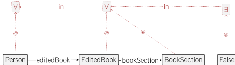
Figure 8.1: A way to encode a false nested graph constraint.
