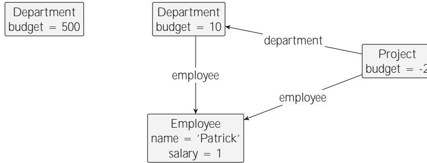
Figure 2.8: An instance model where every department has a positive budget.
