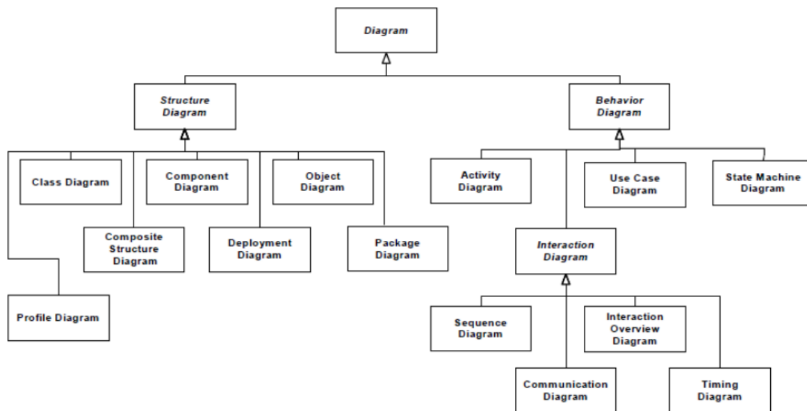
Figure 2.1: An overview of all UML 2.5 diagrams [2].
