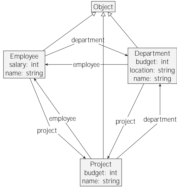
Figure 5.1: GROOVE type graph corresponding to the UML class diagram in Figure 2.3.
