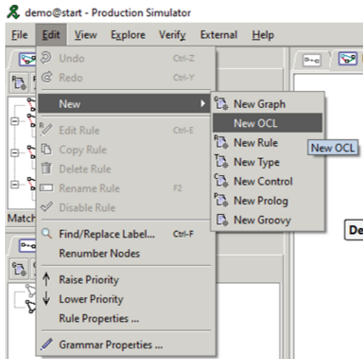
Figure 6.2: The location to create a new OCL constraint in GROOVE.
