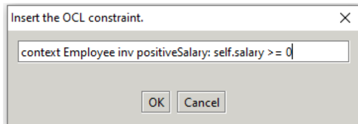
Figure 1.3: The way to create a new OCL constraint in GROOVE.
