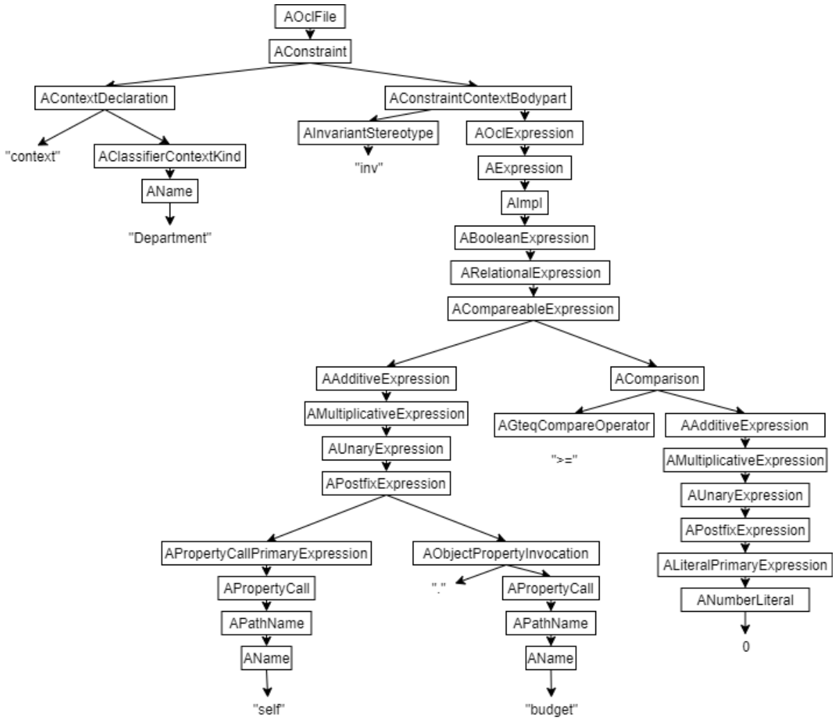
Figure 6.1: The CST of the OCL constraint: context Department inv: self.budget >= 0.
