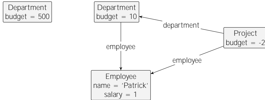
Figure 2.4: An instance of the class diagram in Figure 2.3.
