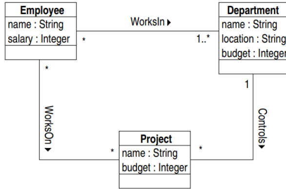
Figure 1.1: An example of a UML class diagram [4].
