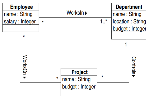
Figure 7.1: The USE case study class diagram [4].
