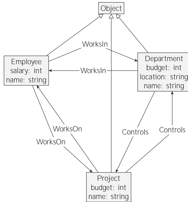
Figure 1.2: GROOVE type graph corresponding to the UML class diagram in Figure 2.3.
