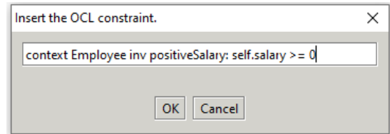
Figure 6.3: The way to create a new OCL constraint in GROOVE.
