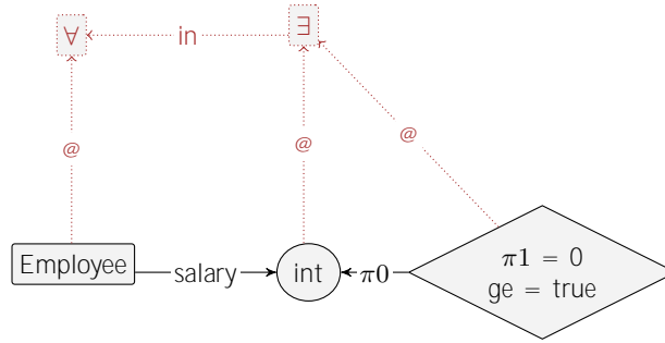
Figure 1.4: The positiveSalary invariant in GROOVE.
