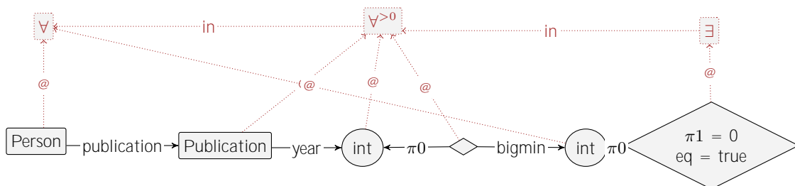
Figure 5.4: The way to encode the min operation with a bigmin in GROOVE.
