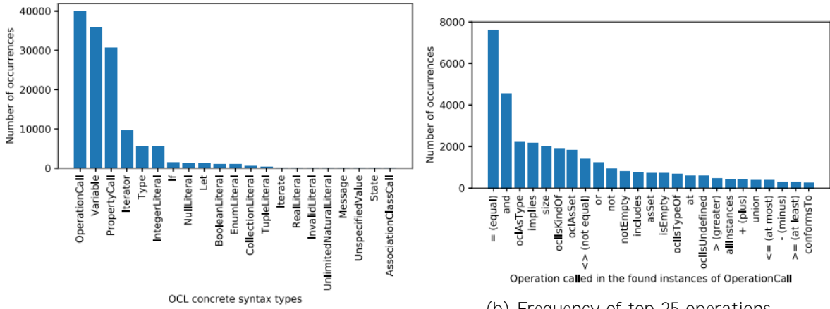
(a) Frequency of OCL constructs.
