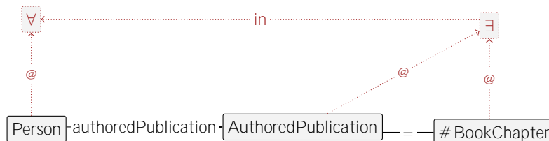
Figure 5.3: An example of a sharp type check in GROOVE.
