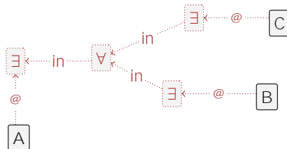
Figure 5.2: The way to encode \exists(A) \vee (\exists(B) \wedge \exists(C)) in GROOVE.
