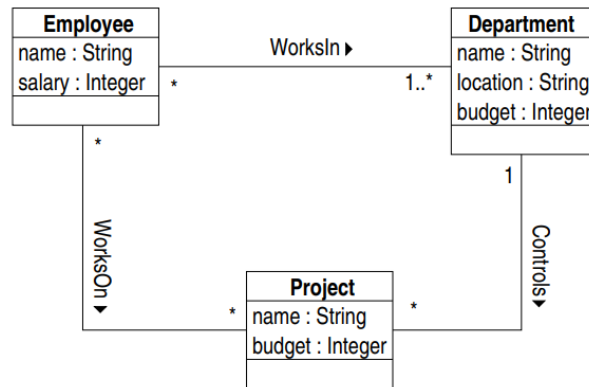
Figure 2.3: An example of a UML class diagram [4].
