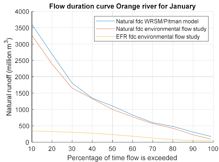
Figure 41: Flow duration curves (fdc) for January
