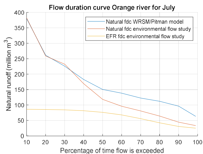
Figure 38: Flow duration curves (fdc) for July
