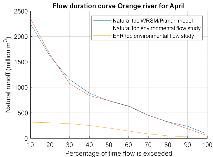
Figure 44: Flow duration curves (fdc) for April
