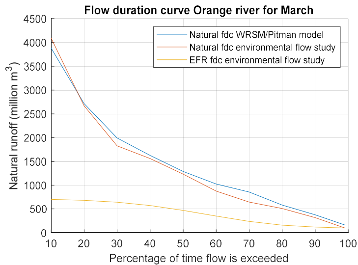
Figure 43: Flow duration curves (fdc) for March
