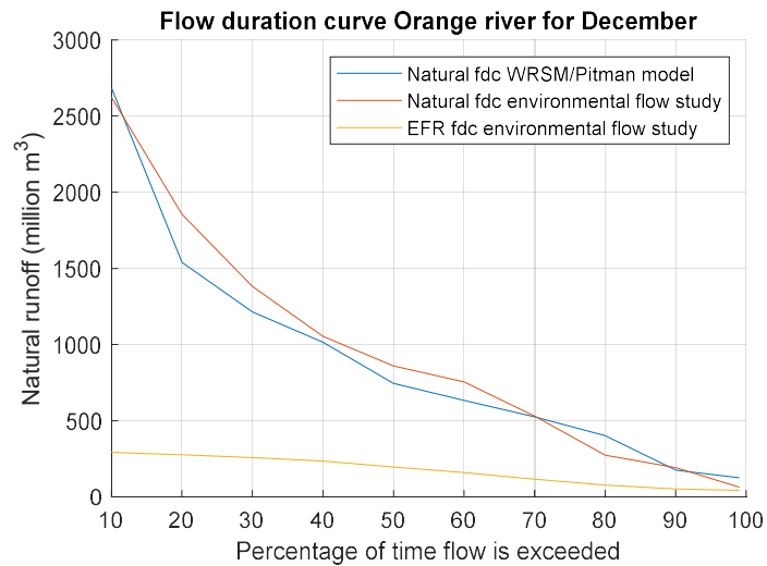
Figure 40: Flow duration curves (fdc) for December
