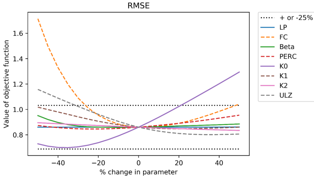
Figure 6: The parameter sensitivity of the HBV model of the Ommerkanaal reflected by the RMSE
