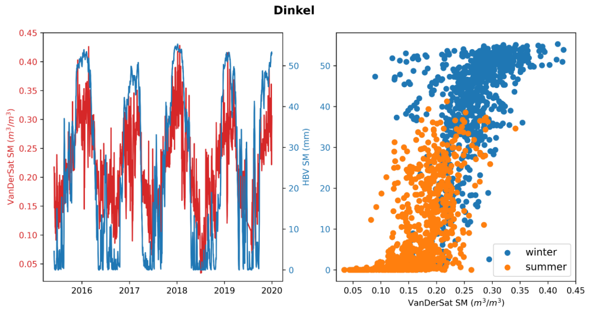
Figure E.2: The soil moisture simulated by the HBV model and the remotely sensed soil moisture for the catchment of the Dinkel and the scatter plot of the same data
