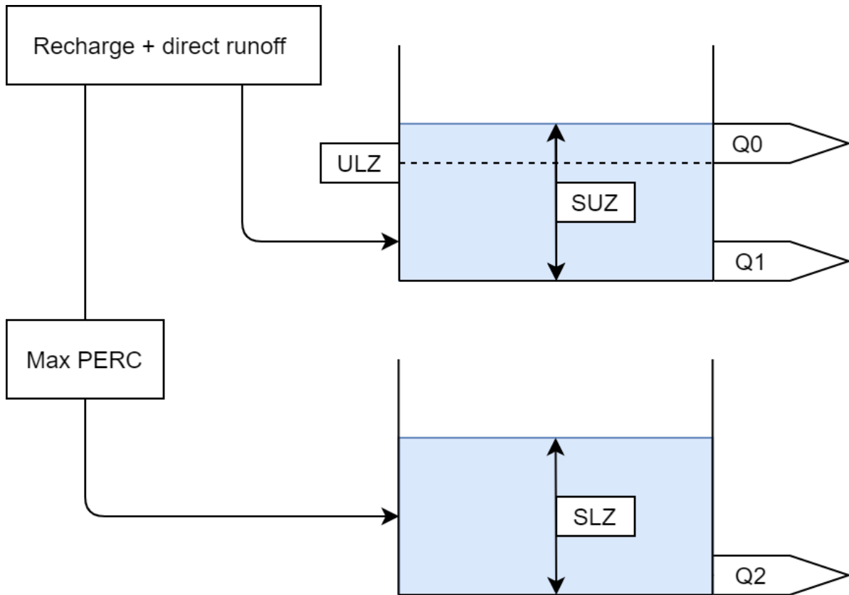
Figure 3: The schematization of the runoff routine
