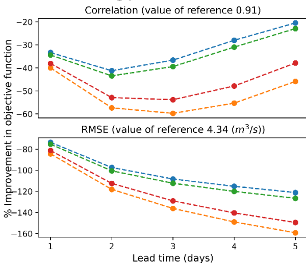
Figure D.11: The result of the assimilation on 5 periods, expressed in the objective functions used.
