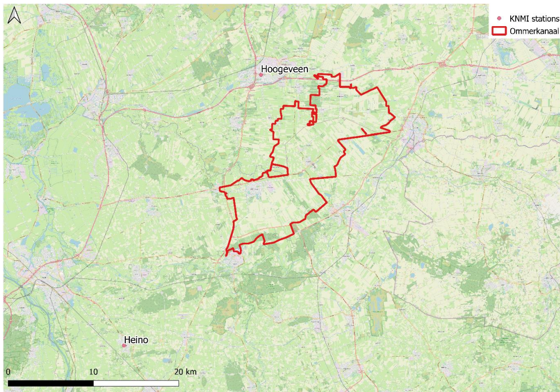
Figure A.6: Location of the Ommerkanaal to the 2 KNMI measuring stations
