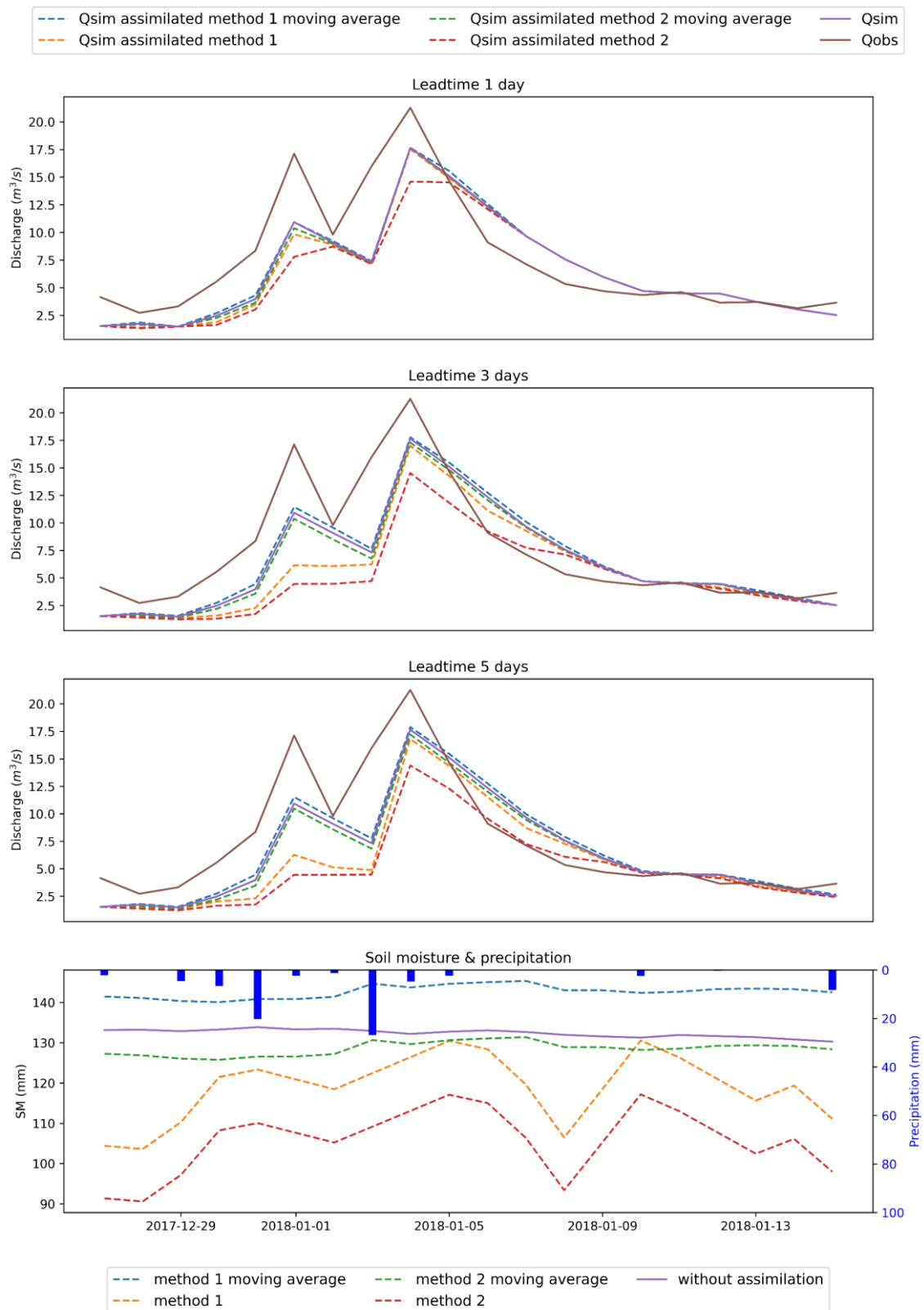
Figure C.4: The effect of the assimilation of soil moisture on the discharge of one peak flow event for the Ommerkanaal for the period of 27-12-2017 to 15-1-2018
