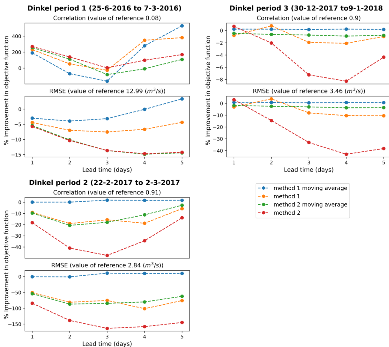
Figure E.5: The result of the assimilation on the 3 periods for the Dinkel, expressed by the objective functions used.
