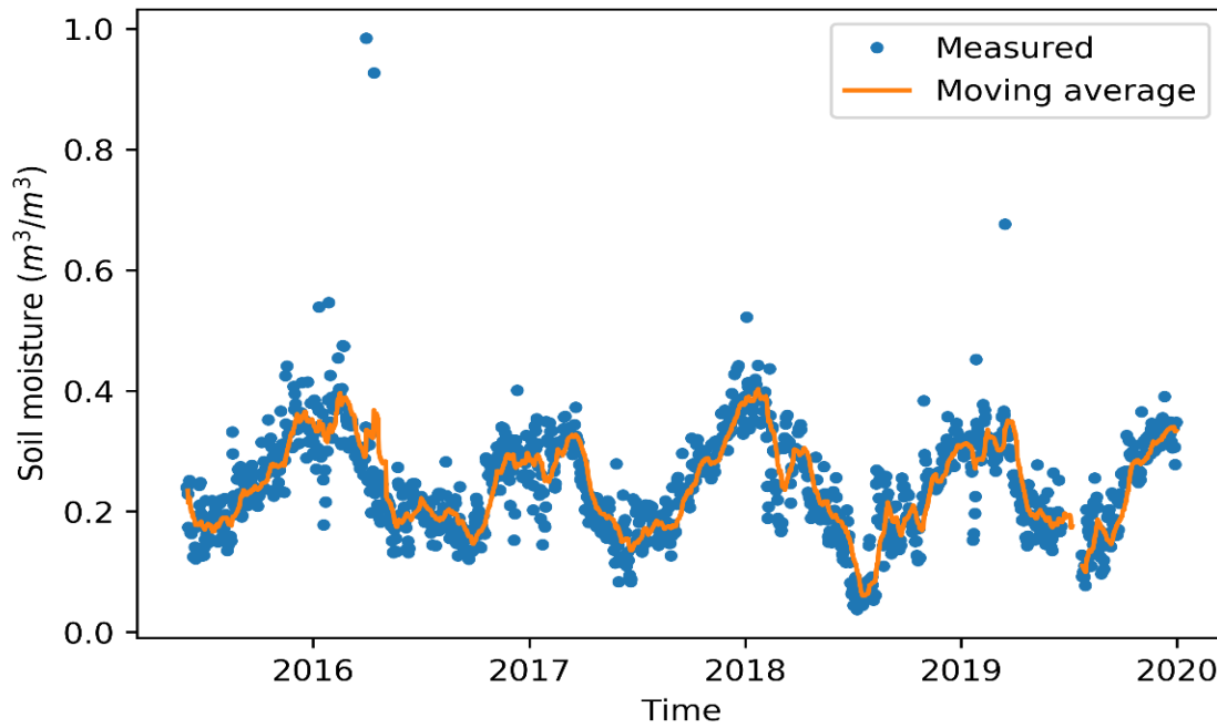
Figure A.2: Remoted sensed soil moisture measured by VanderSat for the area of the Ommerkanaal for the period of 06-2015 up to and including 12-2019.
