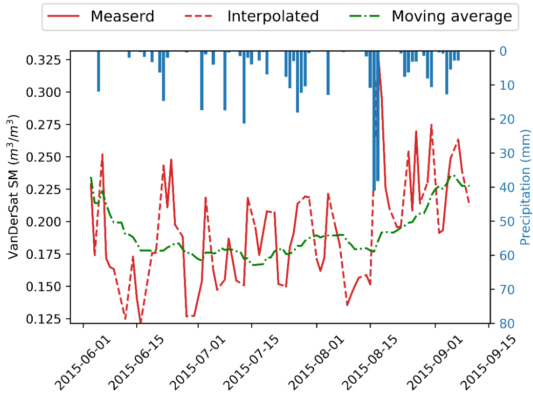
Figure A.4: Soil moisture measured by VanderSat, averaged for the area Ommerkanaal and the measured precipitation from the radar measurements for the Ommerkanaal
