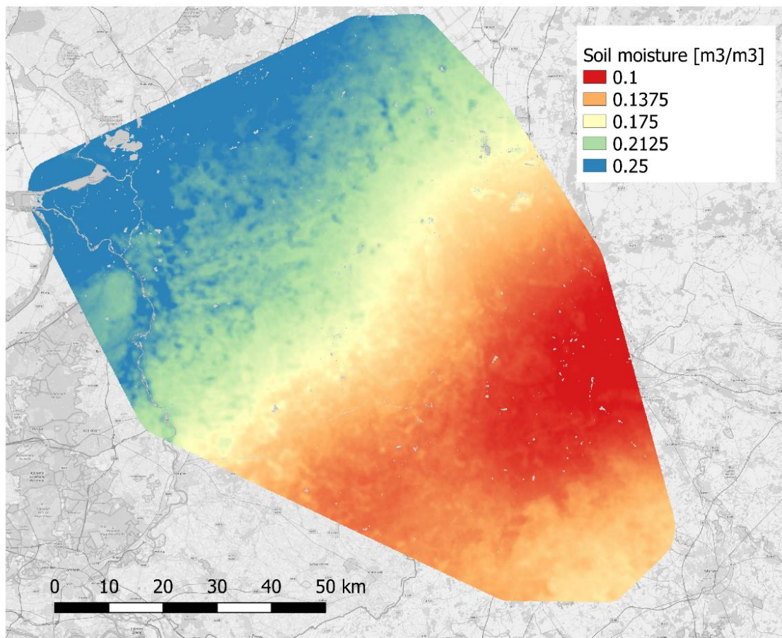
Figure A.1: Satellite image for 24-01-2017 as delivered by VanderSat
