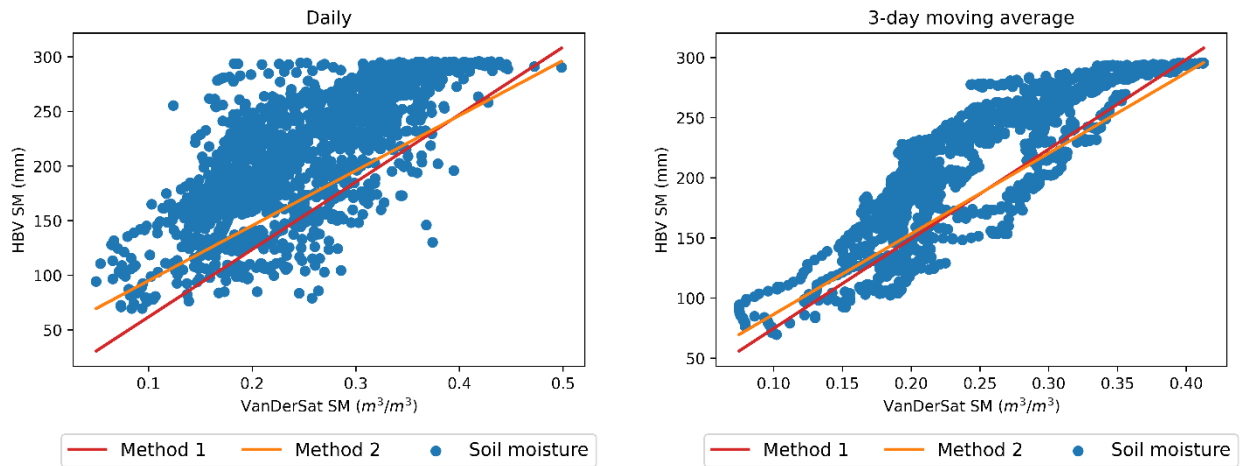
Figure D.5: The remotely sensed soil moisture in comparison to the transformed soil moisture.
