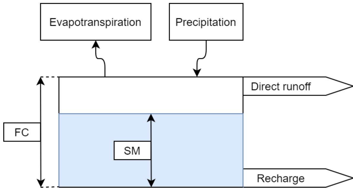
Figure 2: The schematization of the soil routine
