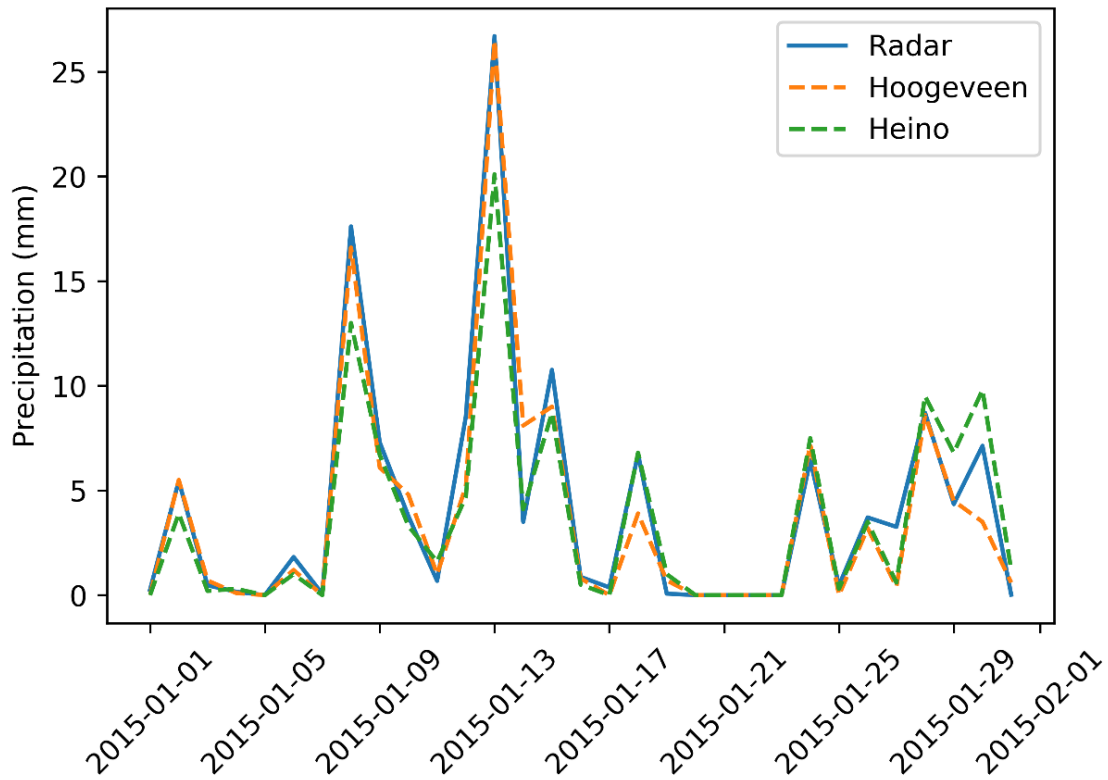
Figure A.5: Precipitation derived for the Ommerkanaal compared to 2 KNMI measuring stations close by the Ommerkanaal.
