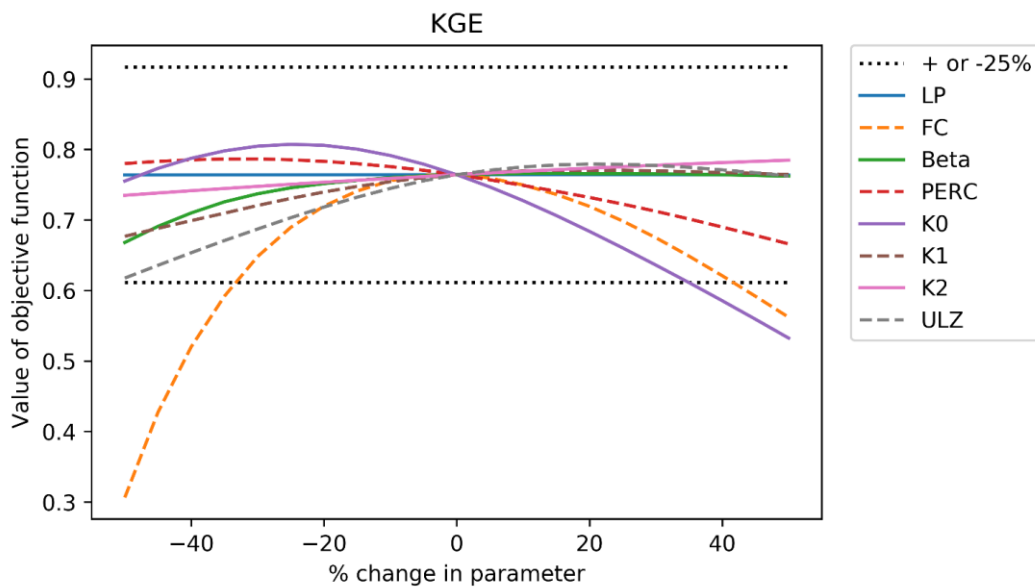
Figure 7: The parameter sensitivity of the HBV model of the Ommerkanaal reflected by the KGE
