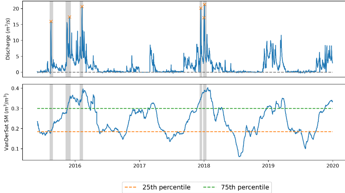
Figure 5: The selection of periods with peak discharges for the Ommerkanaal
