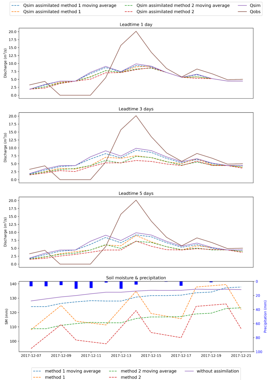
Figure C.3: The effect of the assimilation of soil moisture on the discharge of one peak flow event for the Ommerkanaal for the period of 7-12-2017 to 21-12-2017
