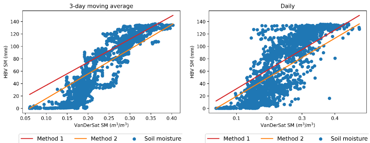
Figure 15: The remotely sensed soil moisture in comparison to the transformed soil moisture.
