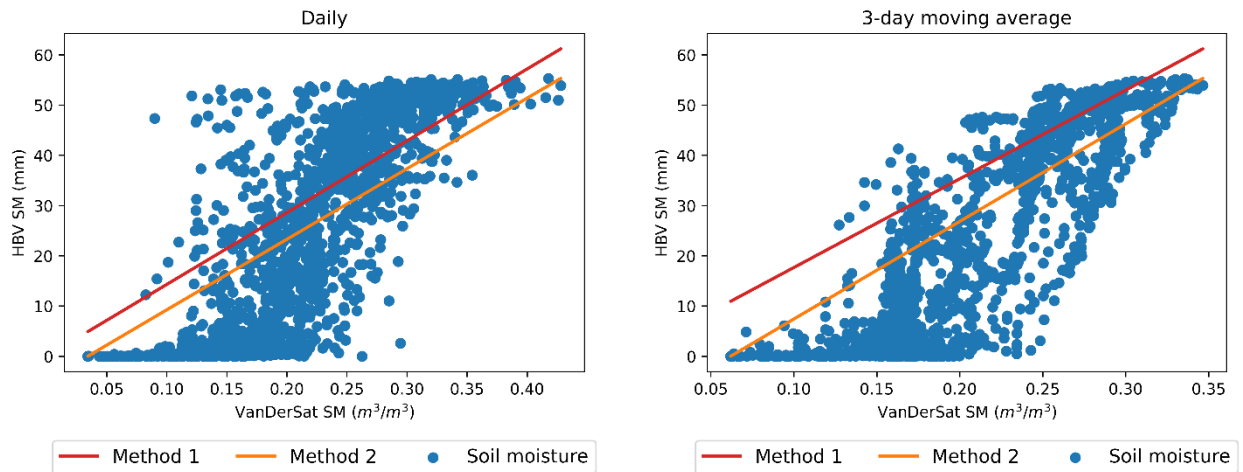
Figure E.4: The remotely sensed soil moisture in comparison to the transformed soil moisture.
