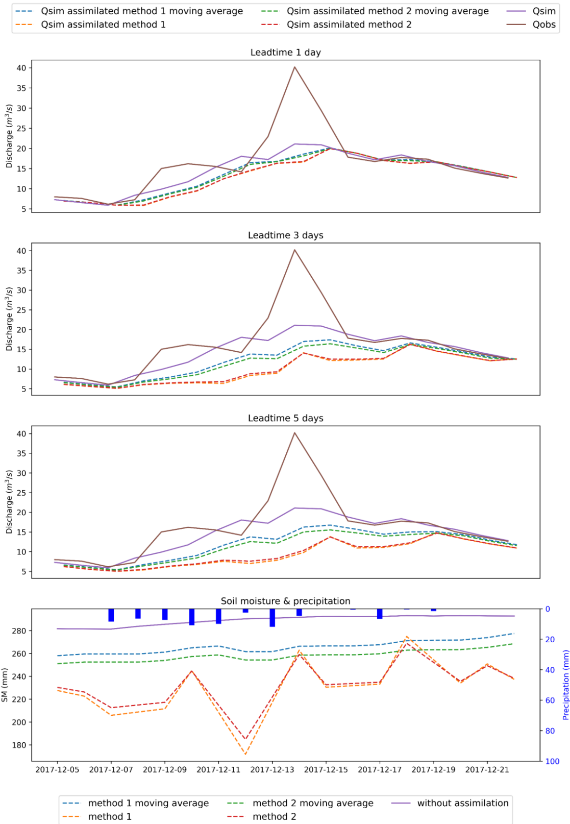
Figure D.9: The effect of the assimilation of soil moisture on the discharge of one peak flow event for the Sallandse Wetering for the period of 5-12-2017 to 22-12-2017
