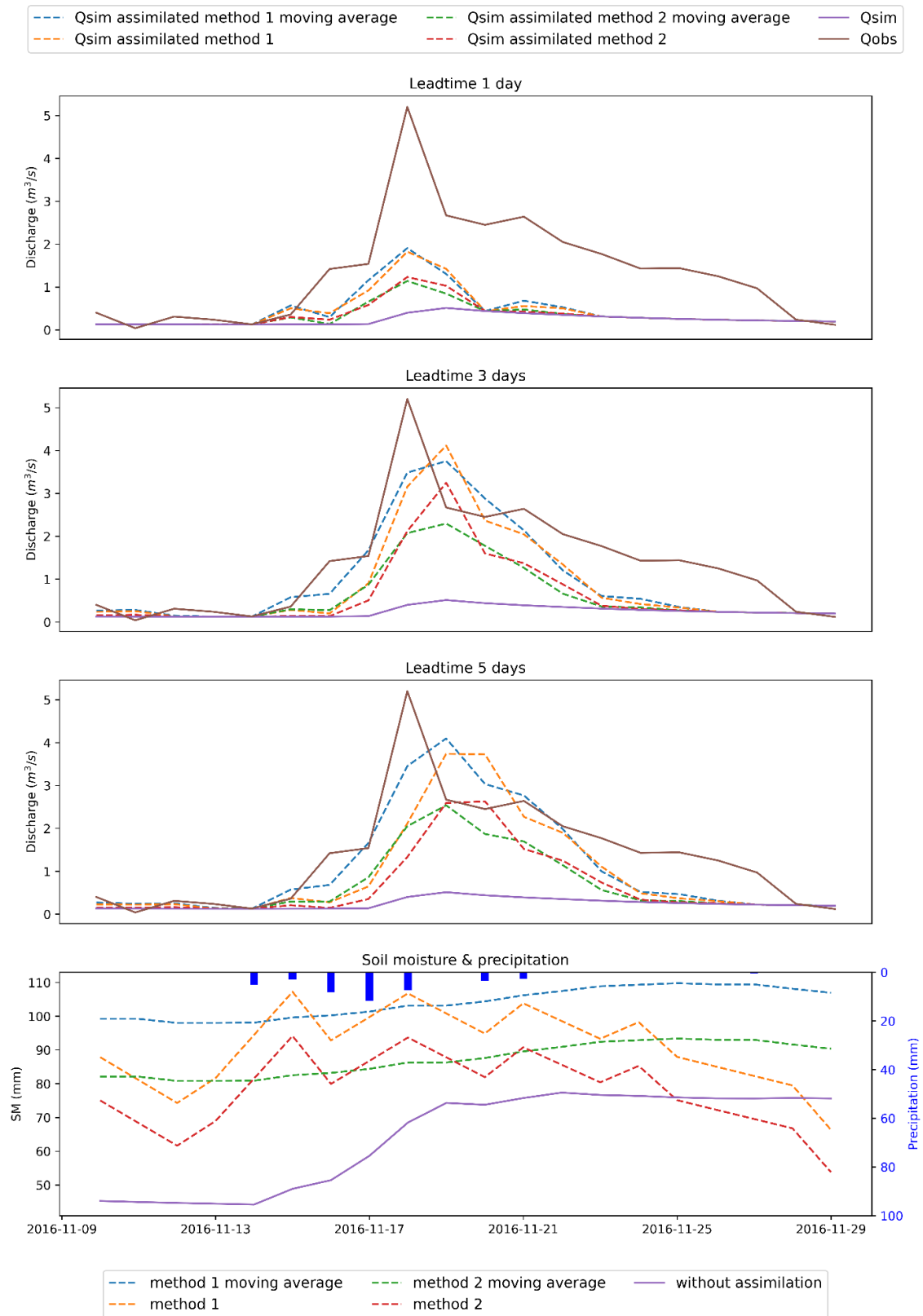
Figure C.5: Extra period used during the assimilation, in which the HBV model does an under estimation of the discharge during a dry period.
