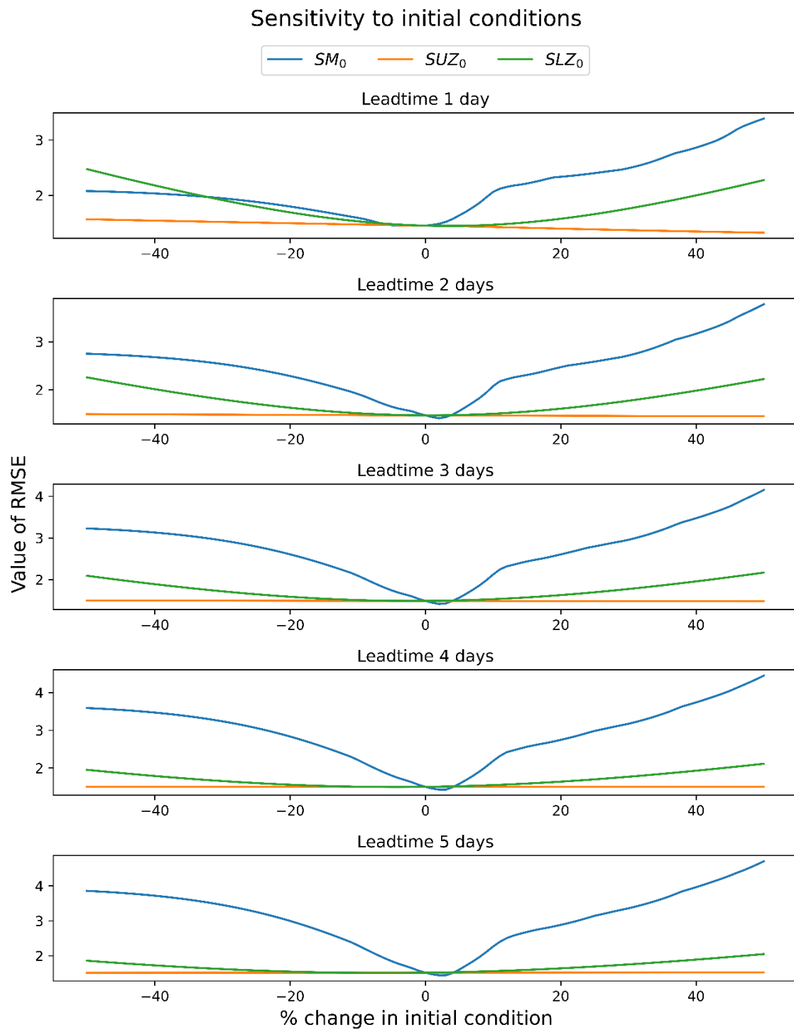
Figure D.2: Outcome of the sensitivity analysis of the HBV model for the Sallandse Wetering for its initial conditions reflected by the RMSE for different lead times of 1 to 5 days
