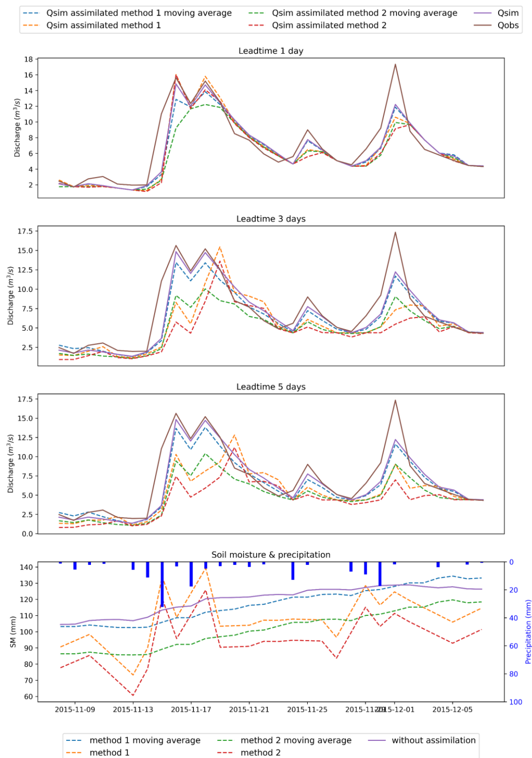
Figure C.1: The effect of the assimilation of soil moisture on the discharge of one peak flow event for the Ommerkanaal for the period of 8-11-2015 to 7-12-2015
