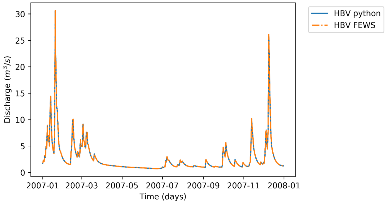
Figure 4: The comparison of FEWS HBV vs the HBV model in Python for the Ommerkanaal for the year 2007, before calibration.
