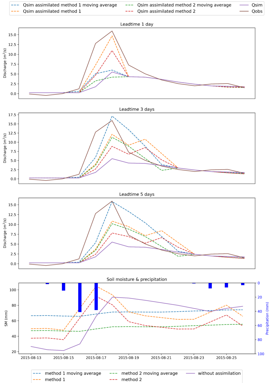
Figure 17: The effect of the assimilation of soil moisture on the discharge of one peak flow event
