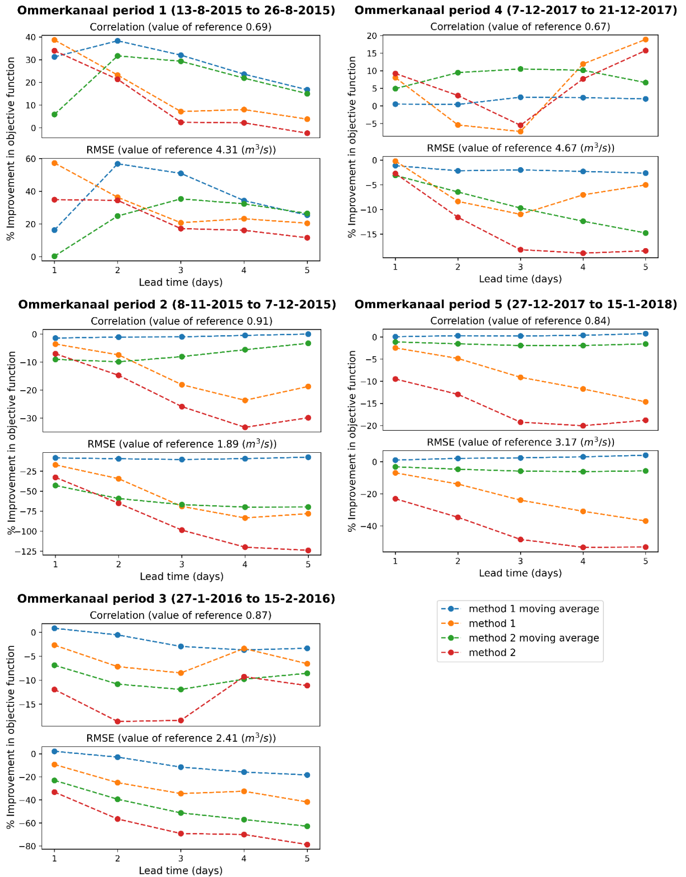
Figure 16: The result of the assimilation for 5 periods for the Ommerkanaal, expressed in the objective functions used.
