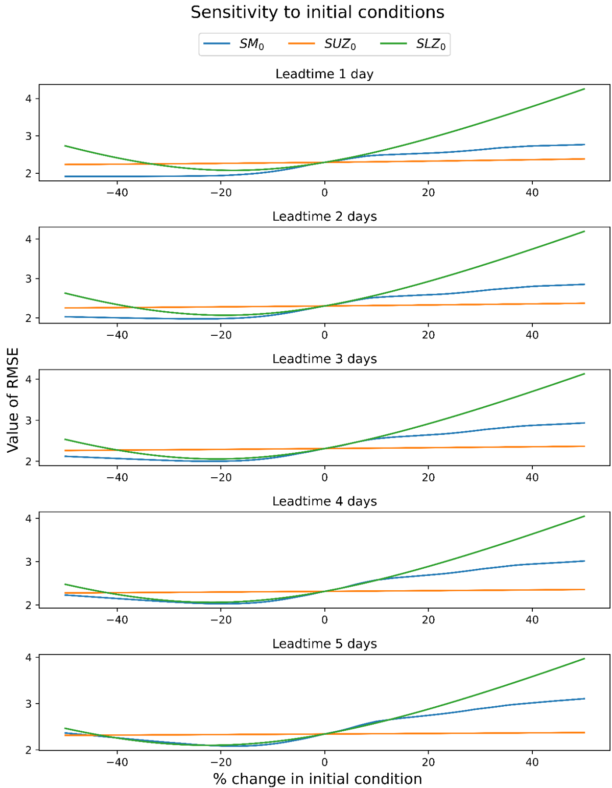
Figure 11: Outcome of the sensitivity analysis of the HBV model for the Dinkel for its initial conditions reflected by the RMSE for different lead times of 1 to 5 days
