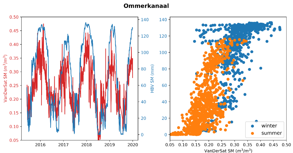
Figure 12: The soil moisture simulated by the HBV model and the daily remotely sensed soil moisture for the catchment of the Ommerkanaal and the scatter plot of the same data
