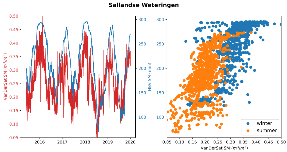
Figure D.3: The soil moisture simulated by the HBV model and the remotely sensed soil moisture for the catchment of the Sallandse Wetering and the scatter plot of the same data
