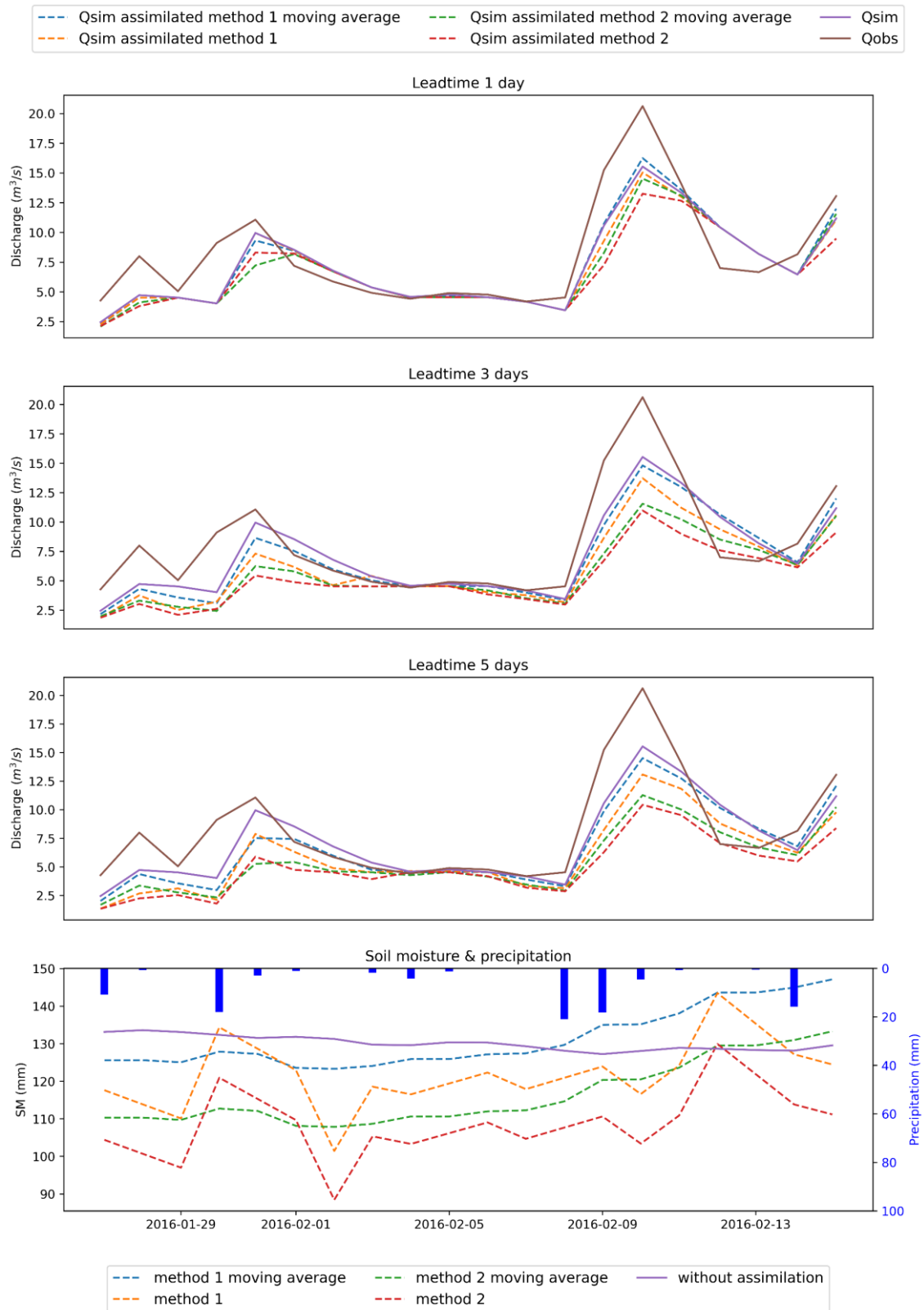
Figure C.2: The effect of the assimilation of soil moisture on the discharge of one peak flow event for the Ommerkanaal for the period of 27-1-2016 to 15-2-2016
