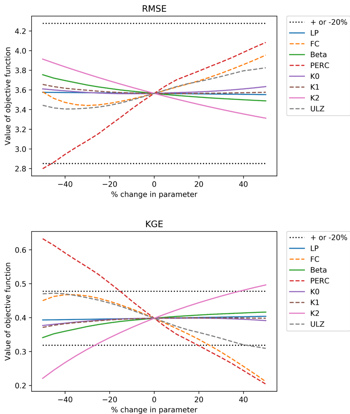
Figure E.1: The parameter sensitivity of the HBV model of the Dinkel reflected by the RMSE and the KGE
