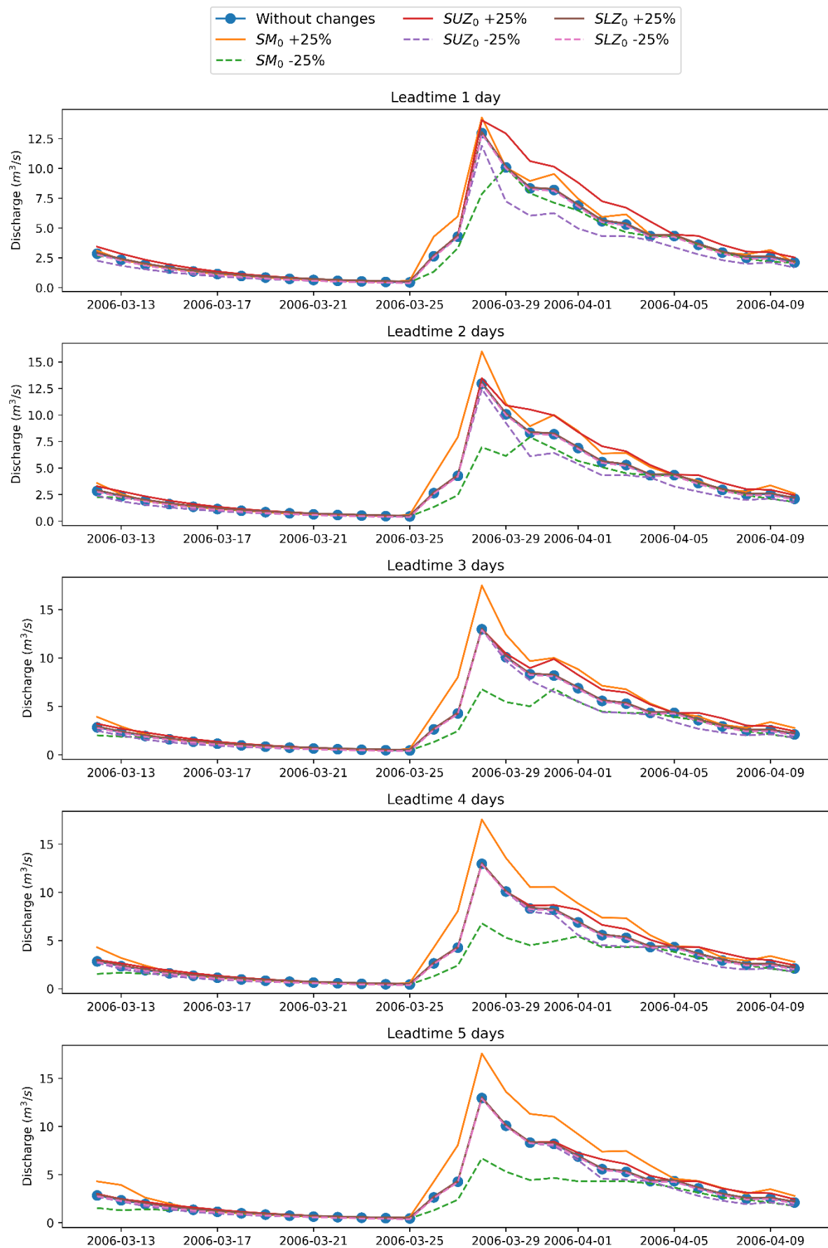
Figure 10: Sensitivity of the initial conditions for one peak flow event at the Ommerkanaal
