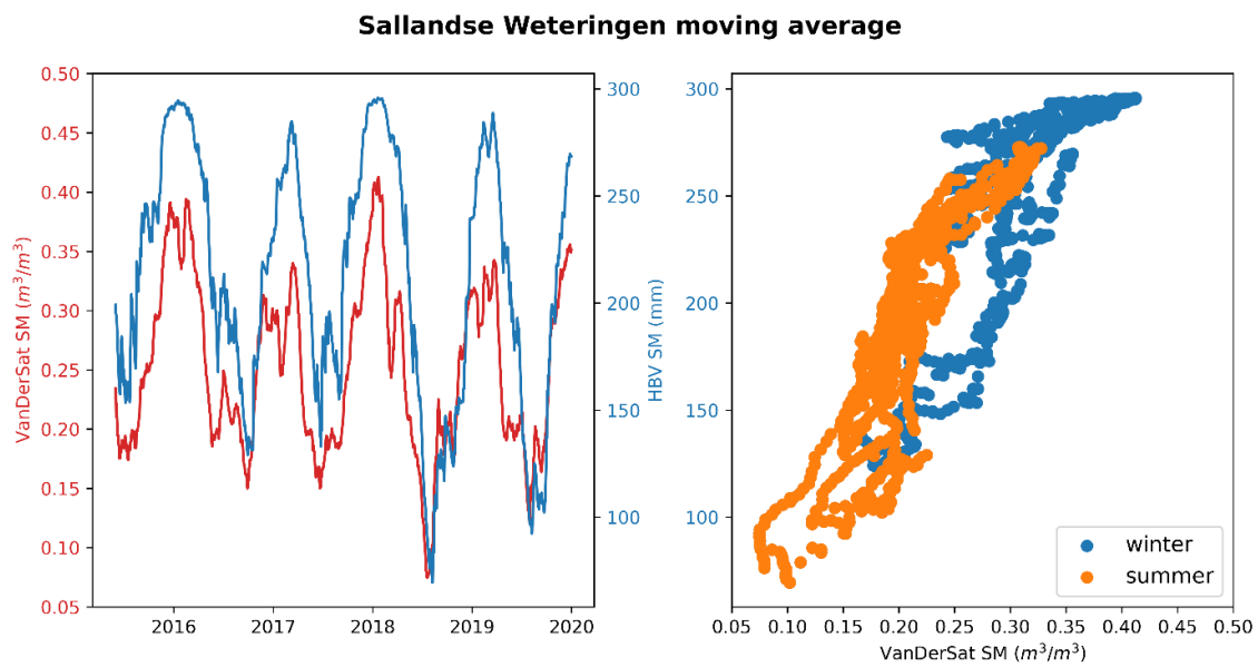
Figure D.4: The soil moisture simulated by the HBV model compared with the moving average of the remotely sensed soil moisture for the Sallandse Wetering and the scatter plot for the same data
