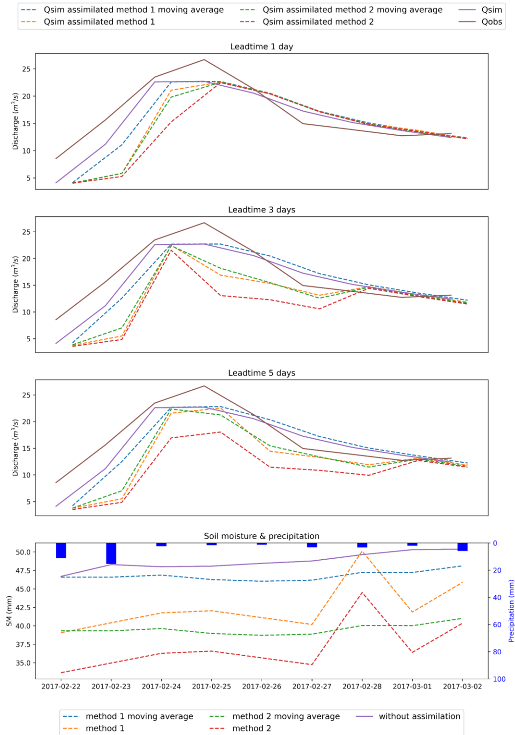
Figure E.7: The effect of the assimilation of soil moisture on the discharge of one peak flow event for the Dinkel for the period of 22-2-2017 to 2-3-2017
