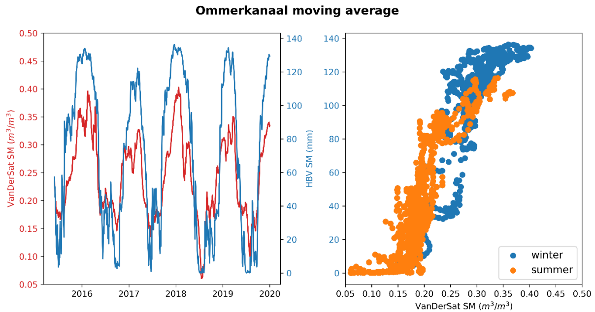
Figure 13: The soil moisture simulated by the HBV model compared with the moving average of the remotely sensed soil moisture for the Ommerkanaal and the scatter plot for the same data
