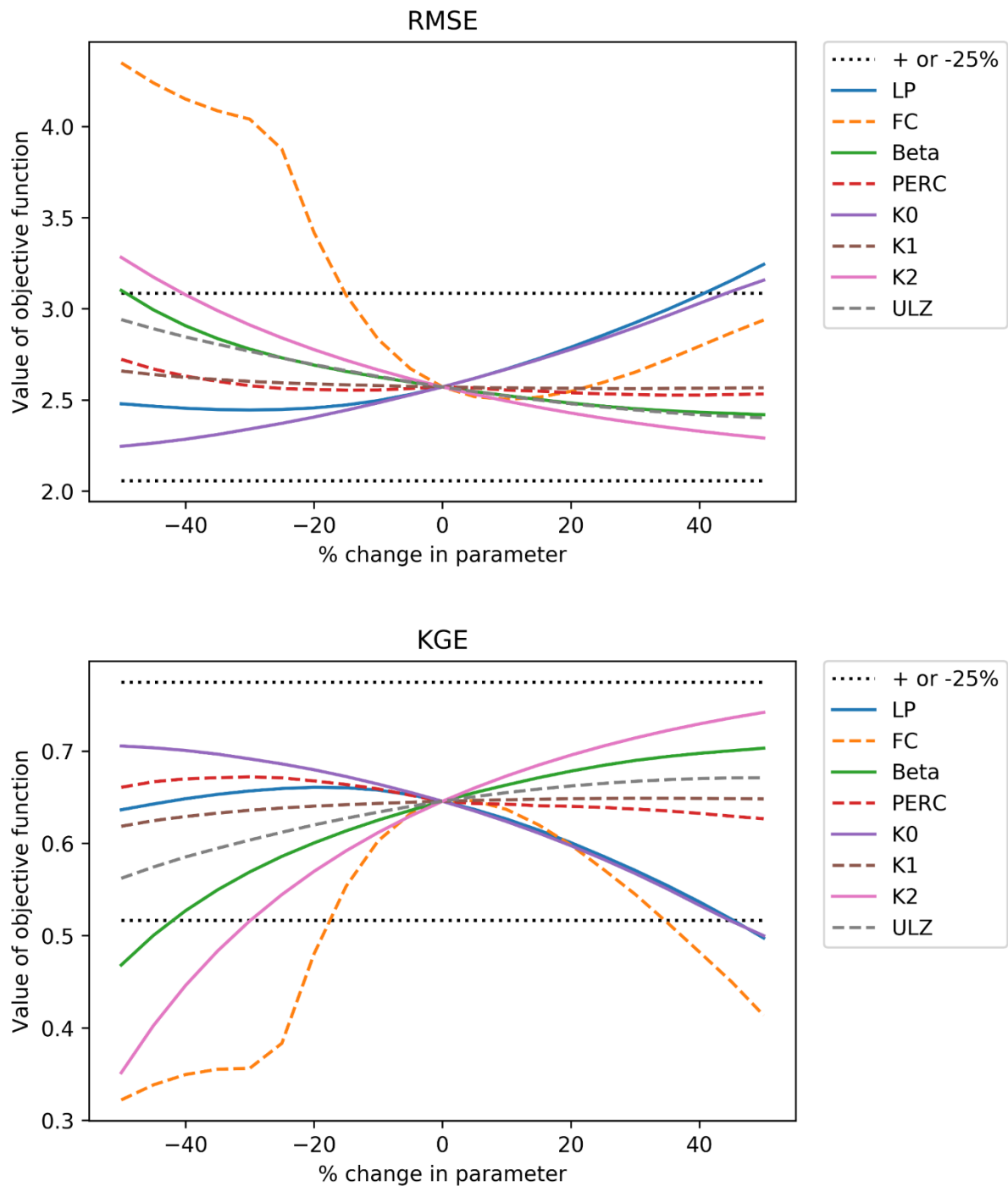
Figure D.1: The parameter sensitivity of the HBV model of the Sallandse Wetering reflected by the RMSE and the KGE
