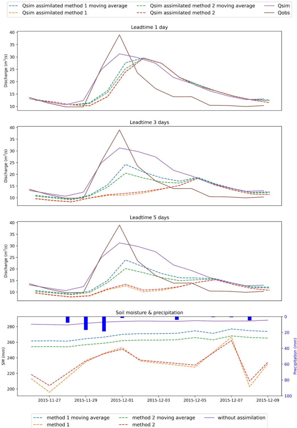
Figure D.6: The effect of the assimilation of soil moisture on the discharge of one peak flow event for the Sallandse Wetering for the period of 26-11-2015 to 9-12-2015
