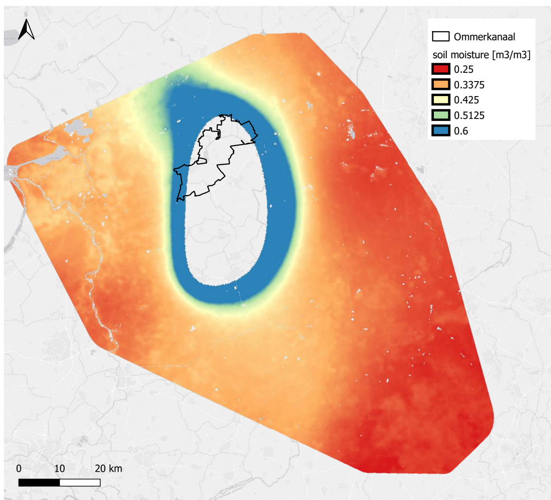
Figure A.3: Satellite image of 31-06-2016 with a large rain event, with the Ommerkanaal outlined.
