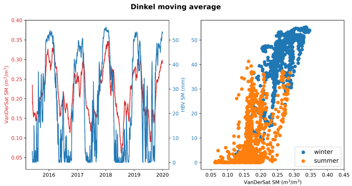
Figure E.3: The soil moisture simulated by the HBV model compared with the moving average of the remotely sensed soil moisture for the Dinkel and the scatter plot for the same data
