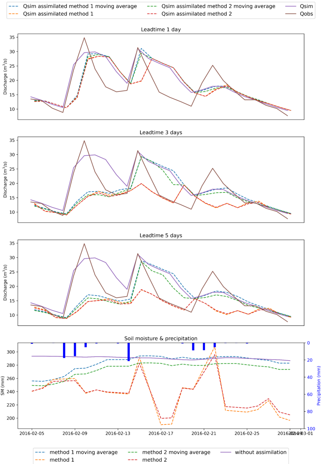
Figure D.7: The effect of the assimilation of soil moisture on the discharge of one peak flow event for the Ommerkanaal for the period of 5-2-2016 to 29-2-2016
