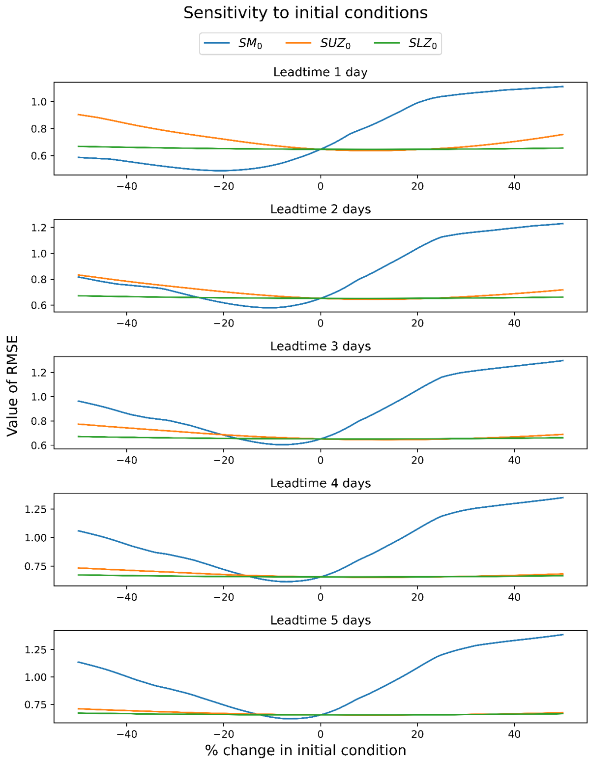
Figure 9: Outcome of the sensitivity analysis of the HBV model for the Ommerkanaal for its initial conditions reflected by the RMSE for different lead times of 1 to 5 days
