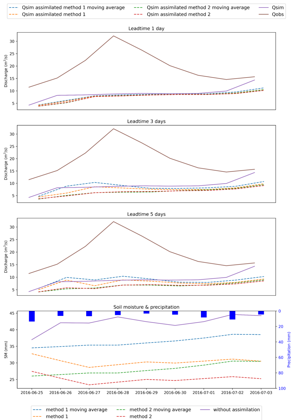
Figure E.6: The effect of the assimilation of soil moisture on the discharge of one peak flow event for the Dinkel for the period of 25-6-2016 to 3-7-2016
