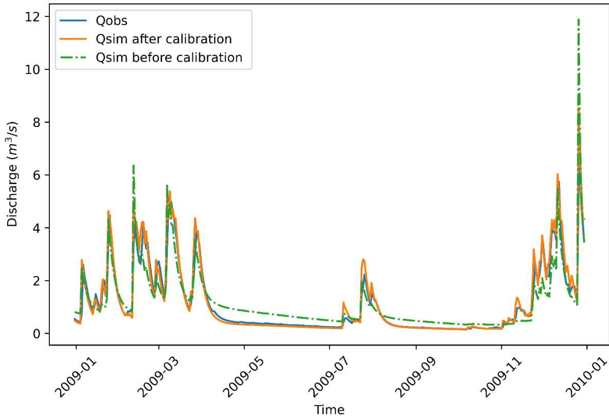
Figure 8: Hydrograph for the Ommerkanaal for 2009 only, to illustrate the effect of the calibration on the simulated discharge, with the observed and simulated discharge before and after calibration.
