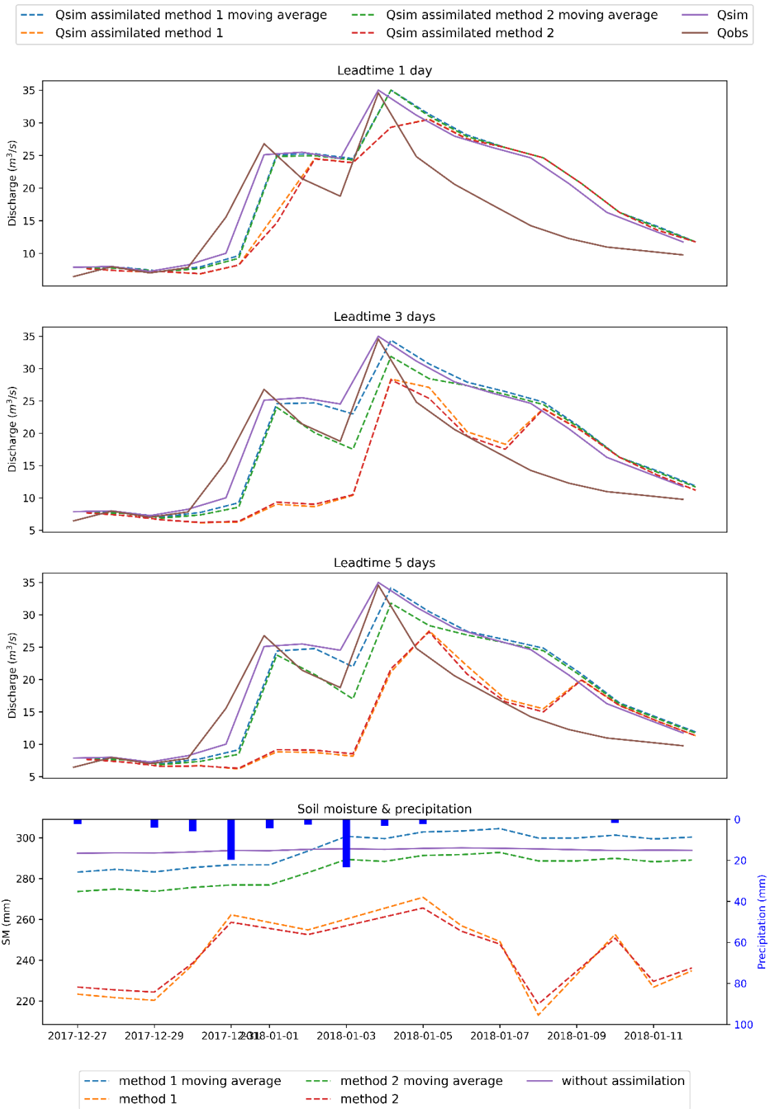
Figure D.10: The effect of the assimilation of soil moisture on the discharge of one peak flow event
