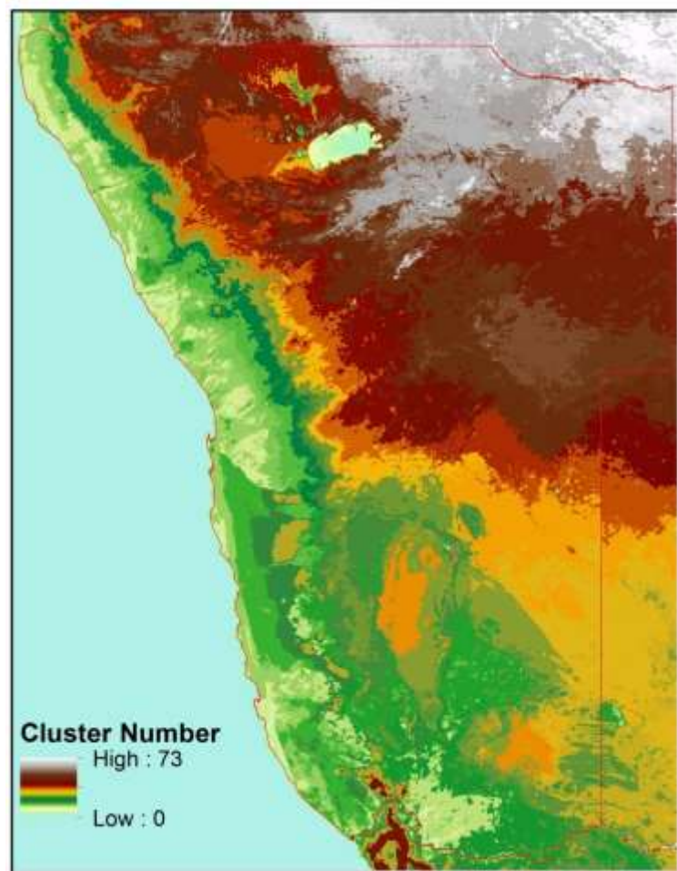
Figure 7 ISODATA classification from SPOT-VGT NDVI time series with 73 clusters
