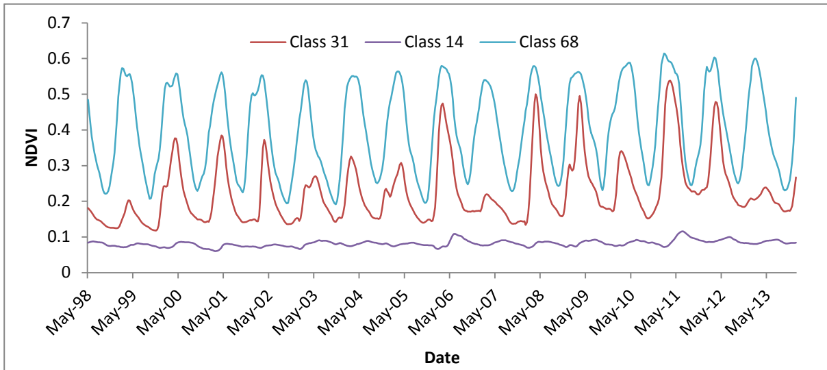
Figure 6 NDVI temporal profiles from clusters 14, 31 and 68 from ISODATA classification from SPOT-VGT NDVI time series with 73 clusters
