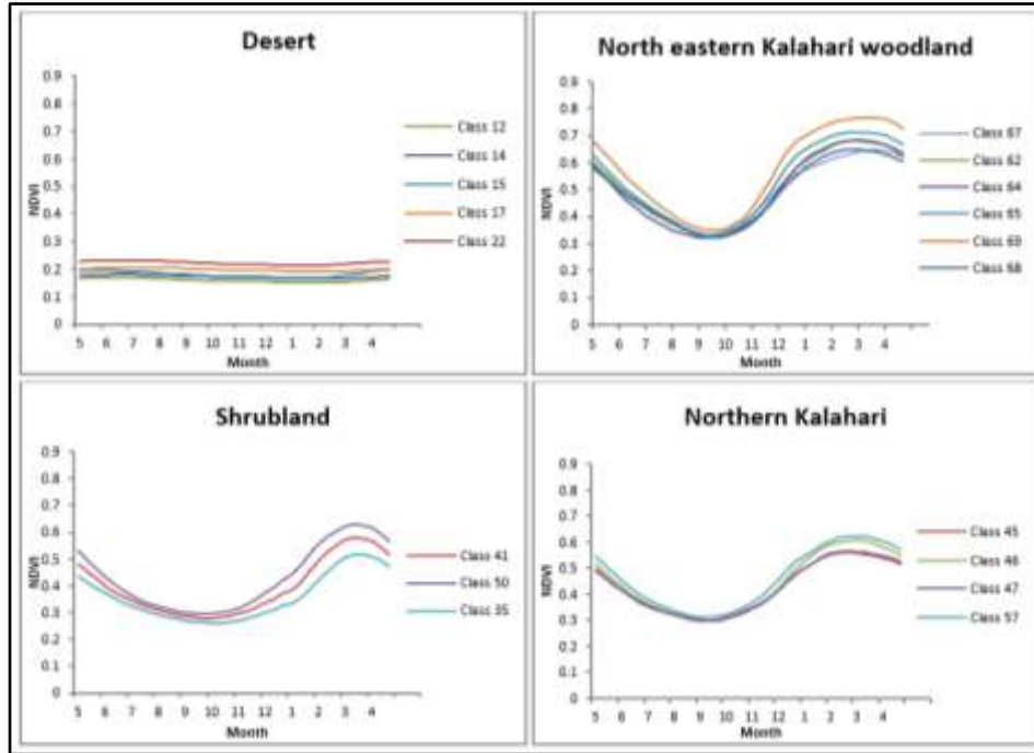
Figure 10 Multiannual NDVI profiles for 4 different vegetation types
