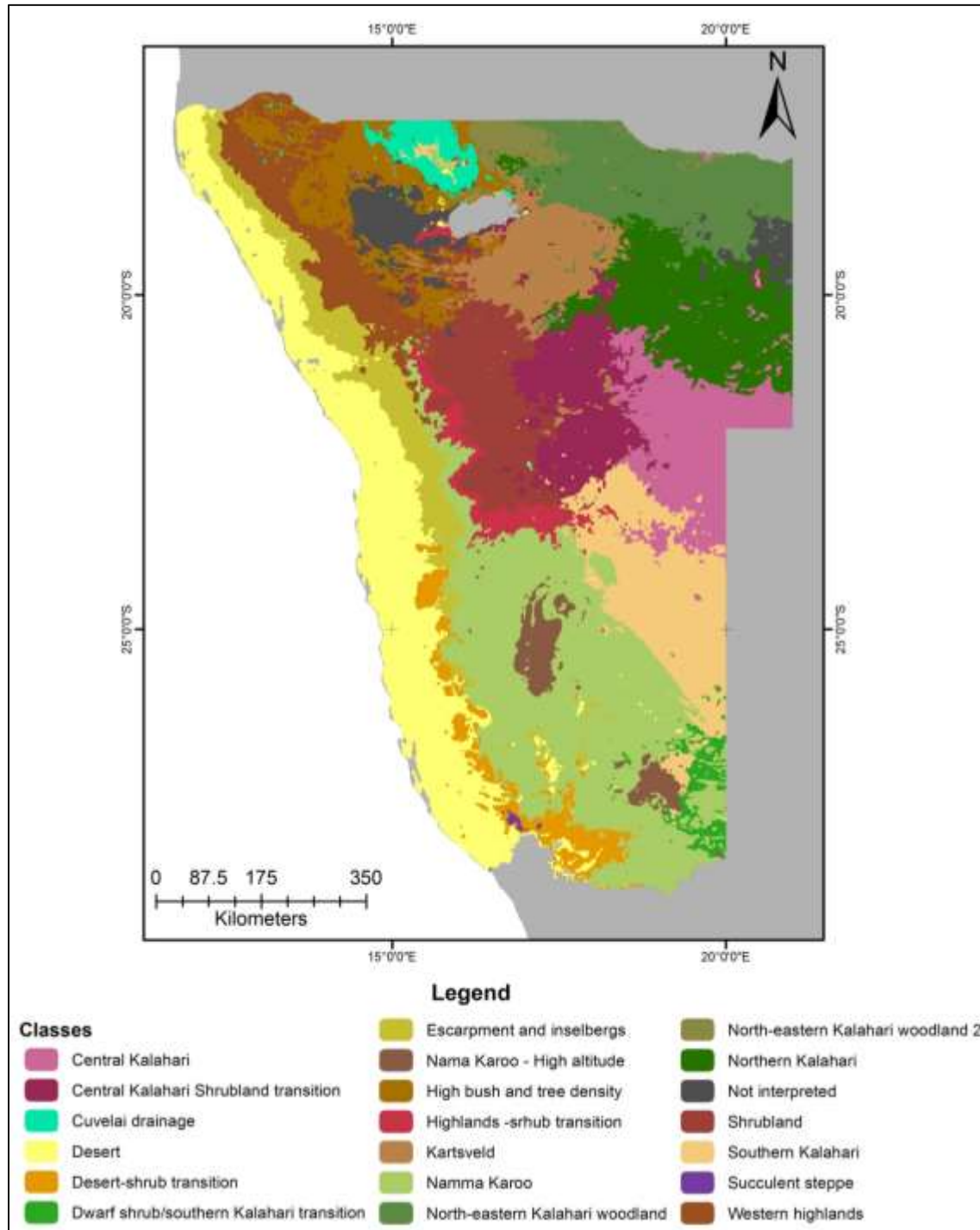
Figure 4 Grouping of the 73 SPOT-VGT NDVI clusters into Vegetation types
