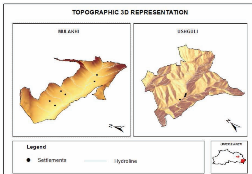
Figure 3.2: 3D representation of the study areas.
