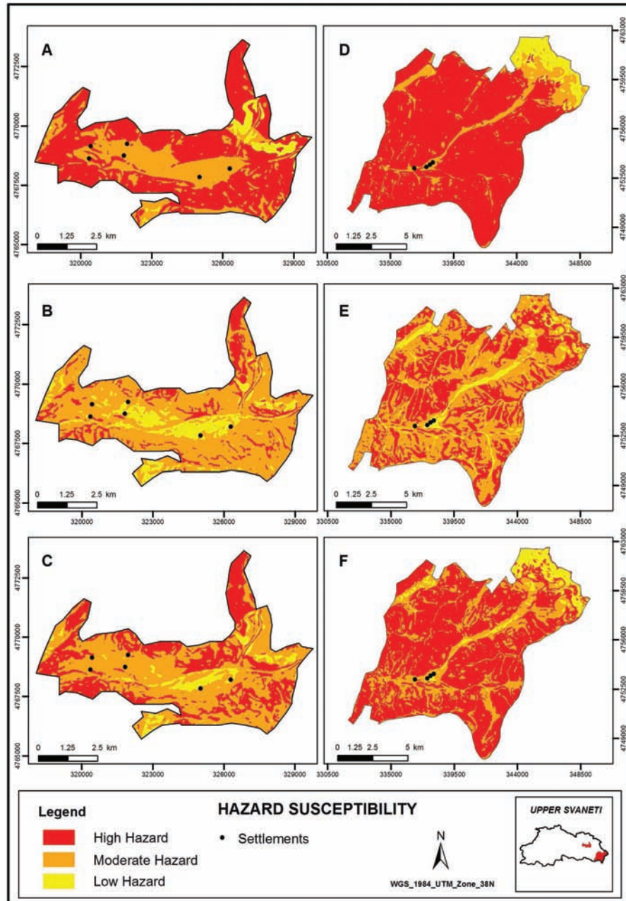
Figure 6.2: Hazard susceptibility in the study area. Mulakhi: Landslide, avalanche and multi-hazard (A, B and C respectively). Ushguli: Landslide, avalanche and multi-hazard (D, E and F respectively).
