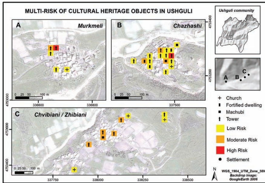
Figure 6.10: Multi-risk (landslide and avalanche) of cultural heritage objects in Ushguli.
