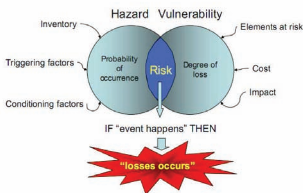
Figure 2.1: Graphical representation of risk and its consequences (Alexander, 2002, cited in Castellanos Abella, 2008a).
