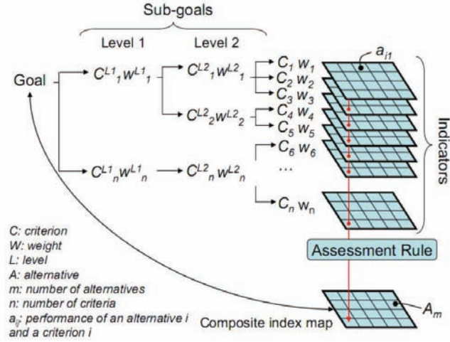
Figure 2.2: Schematic procedure for spatial multi-criteria evaluation based on the analytical hierarchical process (Castellanos Abella, 2008a, van Westen, 2009).
