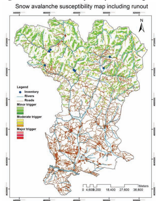
Figure5. 6. Snow avalanche susceptibility map including runoff
