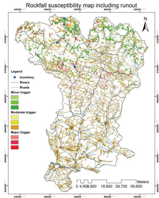
Figure5. 5. Rockfall susceptibility when using DEM generated from contour lines
