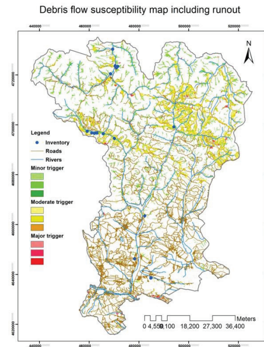
Figure5. 4. Debris flow susceptibility map including runout
