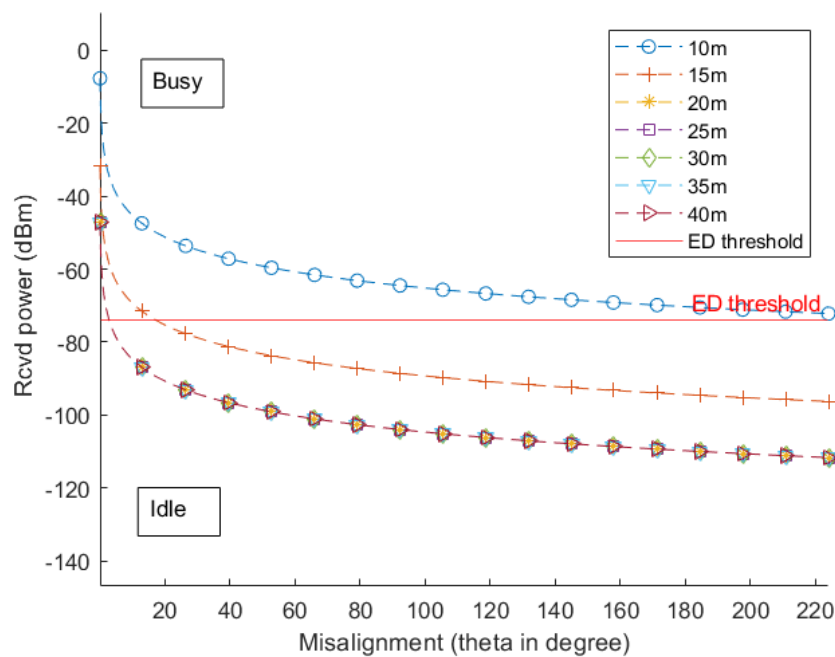
Figure 5.4: Received power vs increasing Misalignment, for gNBs' beamwidth of 30^\circ under increasing distances between WiFi-AP and gNB
