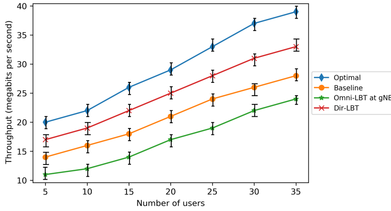
Figure 5.7: Impact of number of users on throughput. As number of users increases, the throughput increases. The optimal approach results in the maximum throughput.
