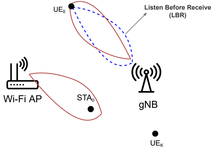
Figure 3.3: The receiver beam does not have any interference with the transmission of WiFi-AP along STA 0 on performing LBR.
