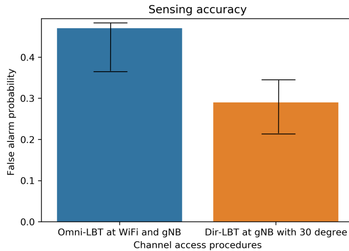
Figure 5.9: False alarm probability when equipped with Omni-LBT and Dir-LBT. It can be seen the Omni-LBT has a higher false alarm probability leading to overprotective nature and lesser throughput.
