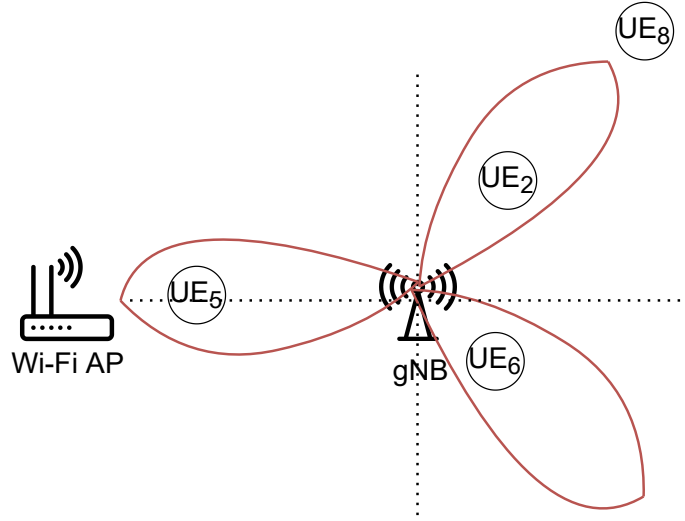
Figure 4.3: gNB uses a 15 degree beamwidth to sense along 3 particular directions to understand the location of Wi-Fi-AP with respect to the UEs in that particular direction.
