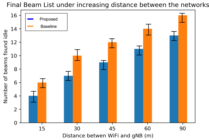
Figure 5.17: Number of beams found idle when distance between the two networks is increased, The number of beams found idle increases with distance between the two networks.
