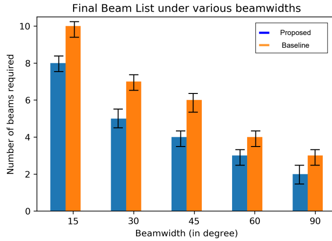
Figure 5.11: Number of beams required under increasing beamwidth
