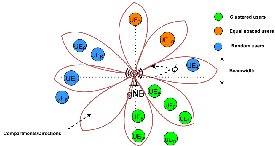
Figure 5.18: Various user distributions are depicted such as clustered users, random user distribution and equally spaced users. Clustered user distribution are depicted as group of users lying under the certain beams. Under random user distribution, the users are randomly distributed and users are spread out equally in all directions for fixed user distribution. The goal is to understand the impact of user distribution on spectrum sensing
