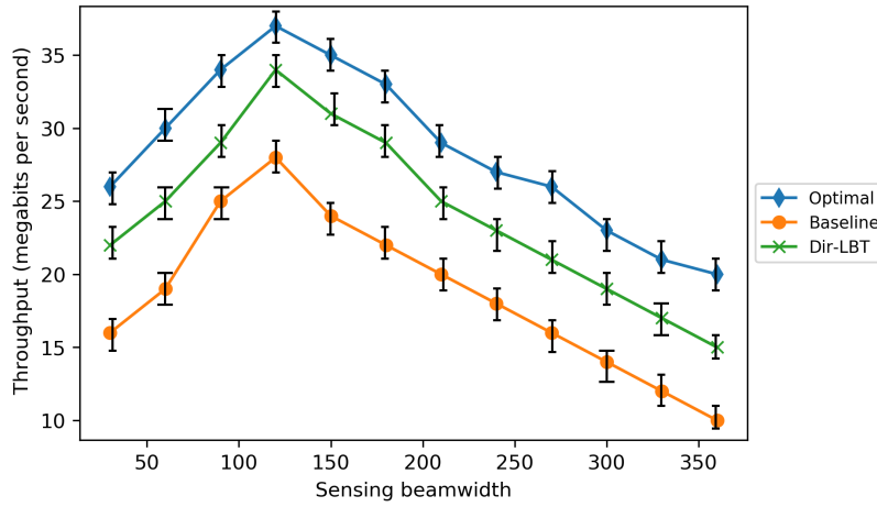
Figure 5.13: Impact of sensing beamwidth on throughput. As sensing beamwidth increases, the throughput increases for a while and decreases further during omnidirectional sensing. Most of the time the spectrum is sensed to be busy.
