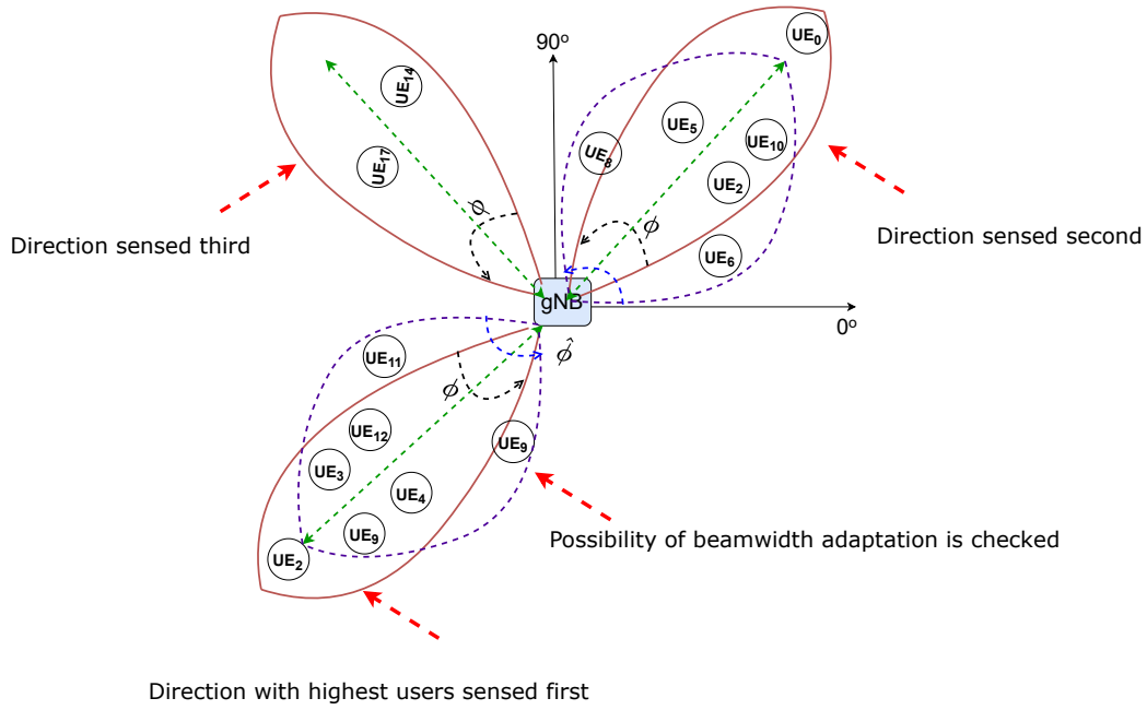
Figure 4.7: The representation of the directional spectrum sensing performed on gNB based on our heuristic algorithm. The direction with the highest number of users is sensed first followed by the possibility of beamwidth adaptation. Next, the direction with the second highest number of users is sensed according to the sorted order.
