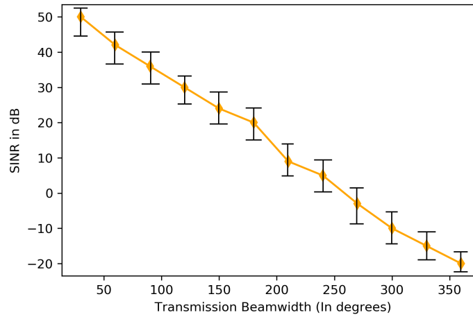
Figure 5.14: Impact of transmission beamwidth on SINR. As transmission beamwidth increases, the SINR decreases as wider beamwidths are more prone to interference.
