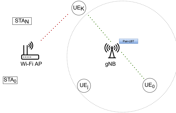
Figure 2.3: Pair-LBT does not detect all the hidden nodes present
