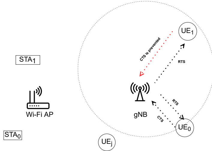
Figure 2.5: CTS is prevented due to the fact that it previously heard a CTS transmitted by a user who was out of range with their targeted transmitter during the time period of the desired data-packet reception
