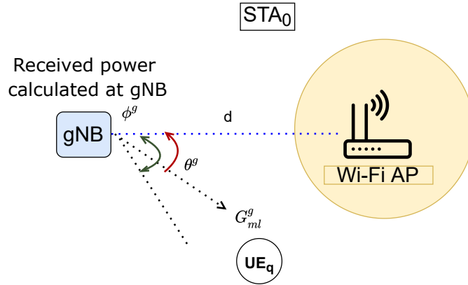
Figure 5.3: A representation of the scenarios considered to evaluate the impact of received power of gNB with increasing distance between them. WiFi-AP uses Omni-LBT, while gNB uses Dir-LBT towards its users.
