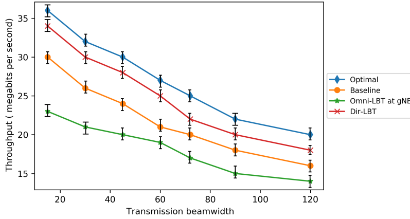
Figure 5.12: Impact of transmission beamwidth on throughput. As transmission beamwidth increases, the throughput decreases as the level of interference of increases when wider beamwidth is employed. Therefore in order to maximize throughput, narrow beamwidth should be preferred.
