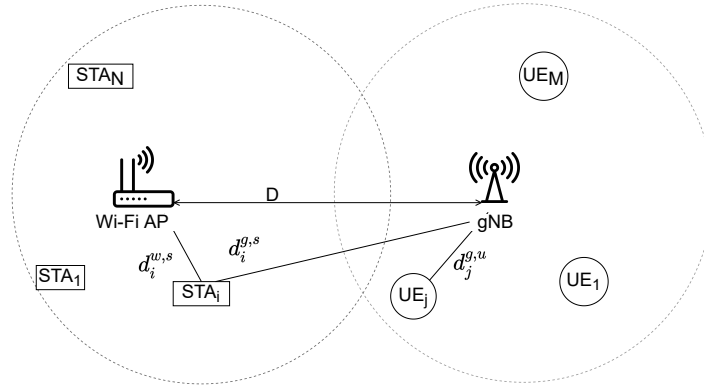
Figure 3.1: System model depicting coexistence of WiFi-AP and gNB with N WiFi stations and M cellular users. The transmitters are separated with a distance of D within the interference range of each other.
