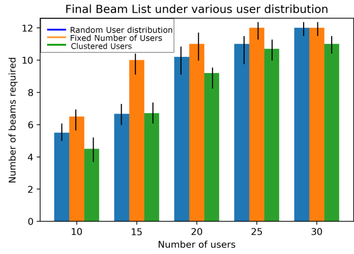
Figure 5.20: The number of beams required for spectrum sensing with increasing number of users for a beamwidth of 30°
