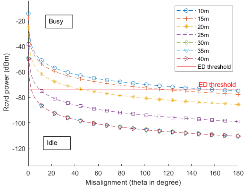
Figure 5.5: Received power vs increasing misalignment, for gNBs' beamwidth of 90^\circ under increasing distances between WiFi-AP and gNB
