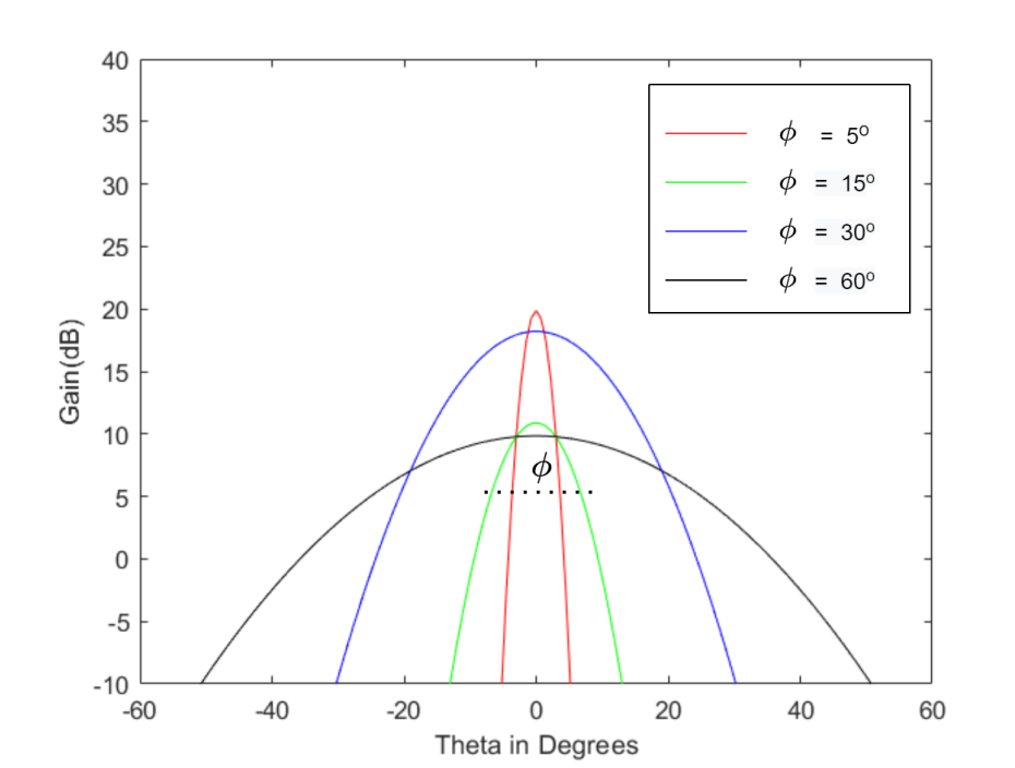
Figure 5.1: The impact of gNBs gain versus increasing values of misalignment, The goal is the examine the impact of narrow beams and wider beams on misalignment.
