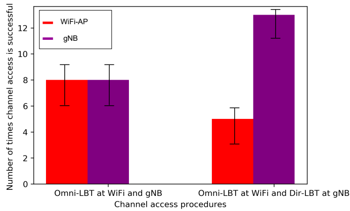
Figure 5.8: The number of successful attempts to access the channel when Omni-LBT and Dir-LBT is equipped at gNB. The overprotective nature of Omni-LBT is seen as the number of successful attempts to access the channel is lower.
