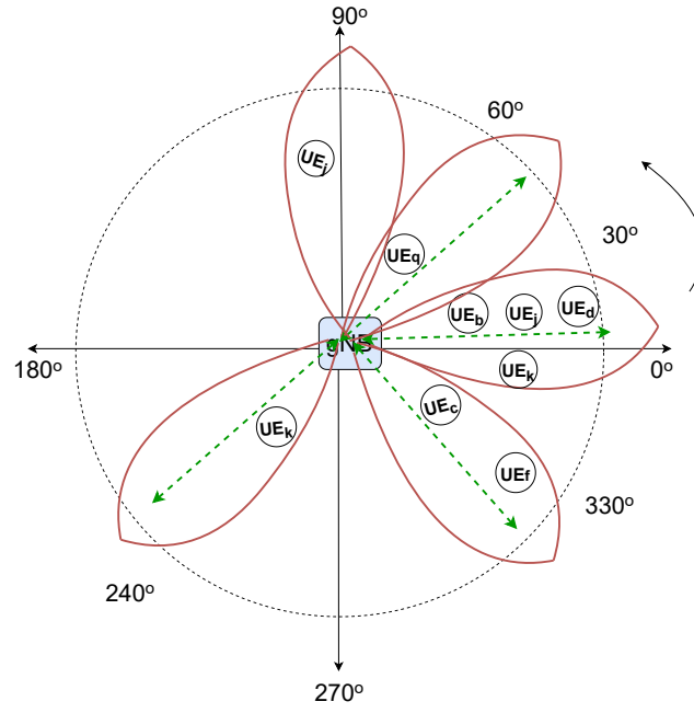
Figure 5.6: The representation of the directional spectrum sensing performed on gNB for a beamwidth of 30^\circ (12 sectors) based on our baseline algorithm. The possibility of beamwidth adaptation is checked followed by sensing towards the particular direction. Certain directions are skipped if no UEs are present.
