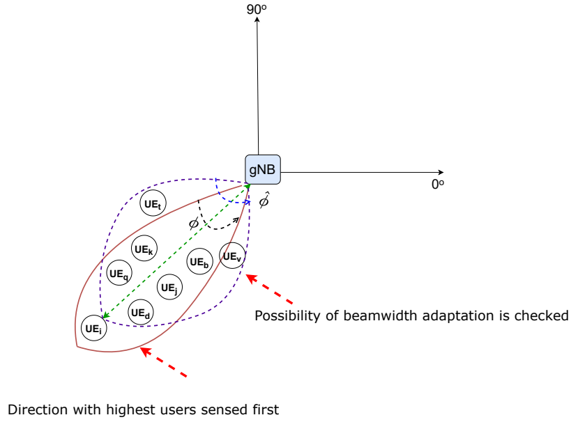
Figure 4.1: The representation of the directional spectrum sensing performed on gNB based on our heuristic algorithm. The direction with the highest number of users is sensed first followed by the possibility of beamwidth adaptation.
