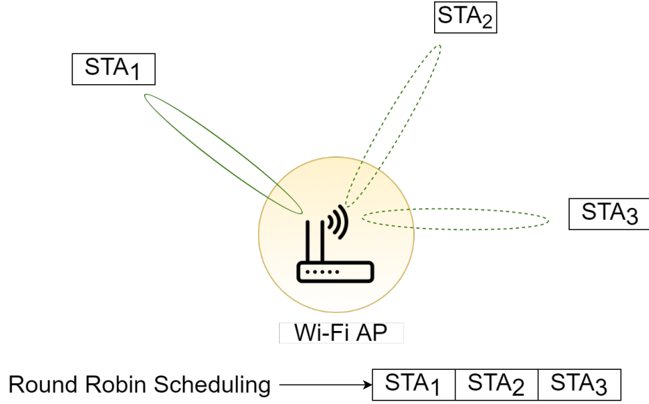
Figure 3.5: The representation of round robin scheduling used in WiFi-AP to transmit data towards its users.
