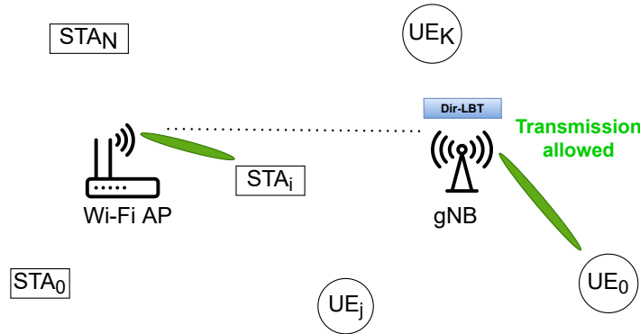
Figure 2.2: Dir-LBT senses along the transmission beam
