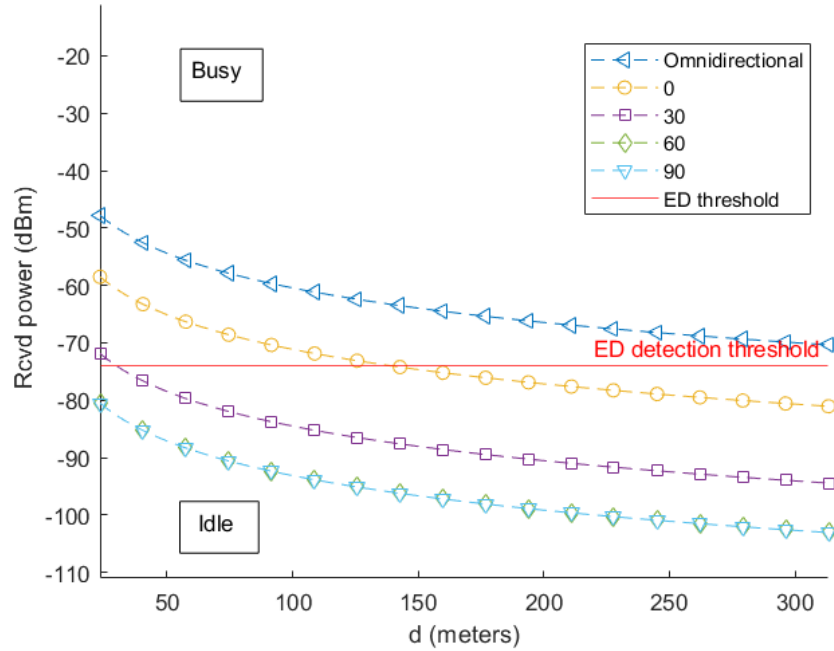
Figure 5.2: Received Power vs distance under 2 scenarios including Dir-LBT at gNB with beamwidth of (60°), while WiFi-AP with a beamwidth of (360°) and Omni-LBT at gNB and WiFi-AP
