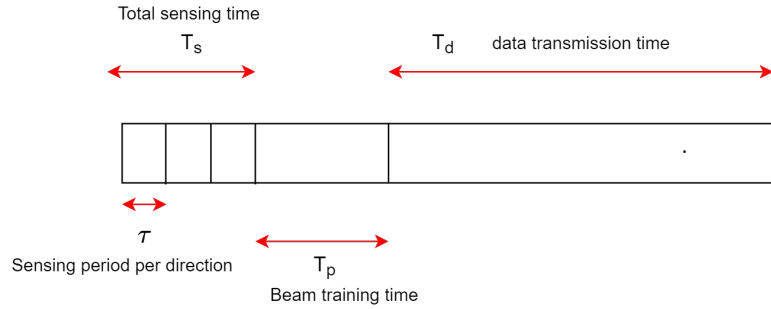
Figure 3.2: Time slotted system of gNB where T represents the total time slot duration in milliseconds. T_s is the total time taken for sensing along multiple directions with each having a constant sensing period of \tau , T_p is the time taken to beam training along the directions which were found idle and T_d is the time taken to perform data transmission.
