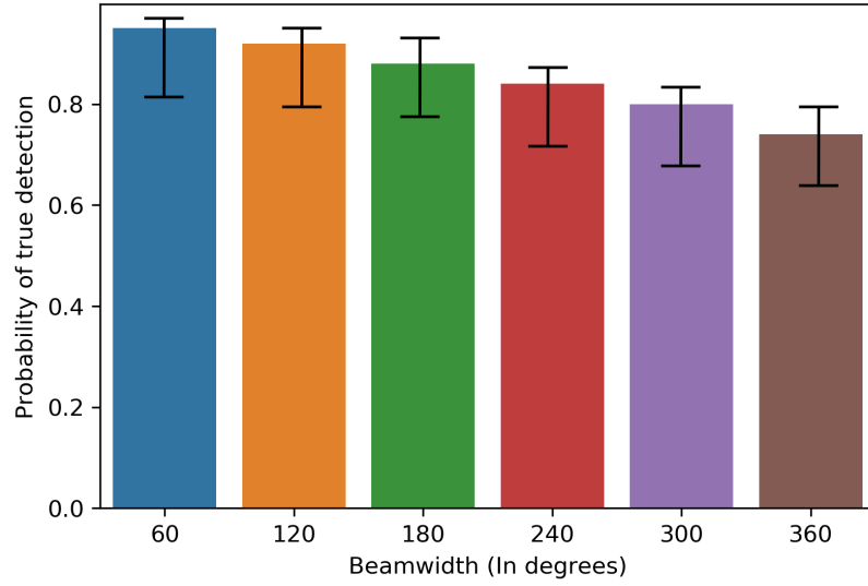
Figure 4.4: Impact of sensing accuracy over sensing beamwidth.
