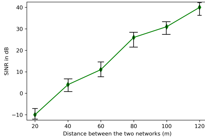
Figure 5.15: Impact of the distance between the two networks on SINR. As distance between the two networks increase, the SINR increases as the interference decreases.
