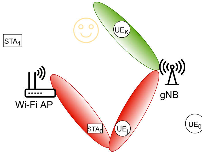
Figure 1.1: Coexistence of WiFi-AP and gNB. Interference occurs at the receivers, when both WiFi-AP and gNB transmit data along the same direction towards their respective users.
