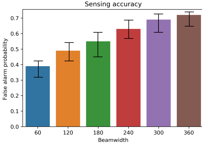
Figure 4.5: False alarm probability under increasing beamwidth. In terms of sensing, a smaller beamwidth of gNB results in lesser false alarms resulting in higher throughput. As beamwidth increases, the false alarm probability increases leading to few opportunities to transmit towards the users.
