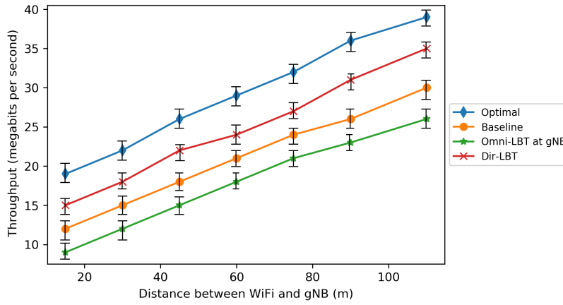
Figure 5.16: Impact of the distance between the two networks on throughput. As distance increases, the level of interference on the neighbouring network decreases resulting in a higher throughput.
