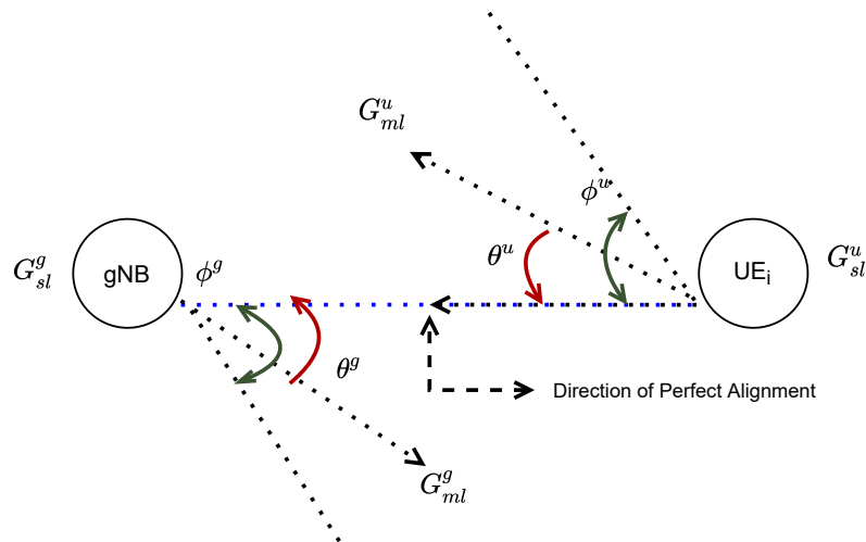
Figure 3.4: Antenna Model adapted from [18]. The figure depicts the alignment of gNB towards one of its users UE i . The misalignment of gNB towards its user is given by \theta and the gain of the main lobe is given by G_{ml}^g .
