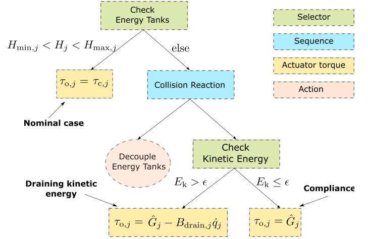
Fig. 5: Behaviour tree for regulating the actuator torques.
