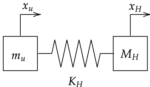
Figure 2.3: Human-robot collision simplified in a mass-spring-mass model
