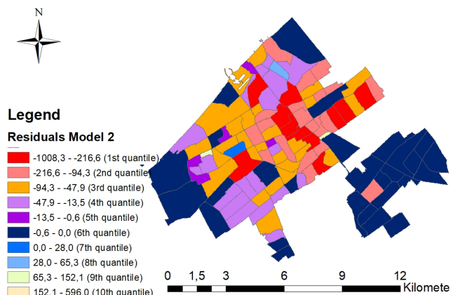
FIGURE J.8: Residuals of negative binomial regression model in The Hague
