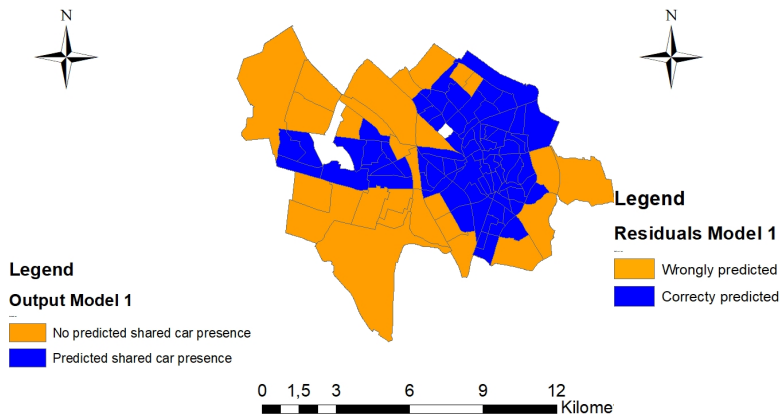
FIGURE J.5: Results of binary logistic regression model in Utrecht
