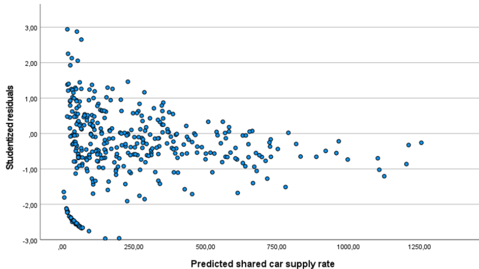
FIGURE 6.5: Plot of the studentized residuals against the predictions of the negative binomial regression
