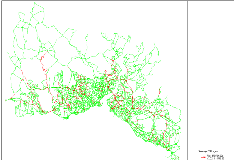
Figure 6-49: Volume-to-capacity ratio, existing situation (option 1a)
