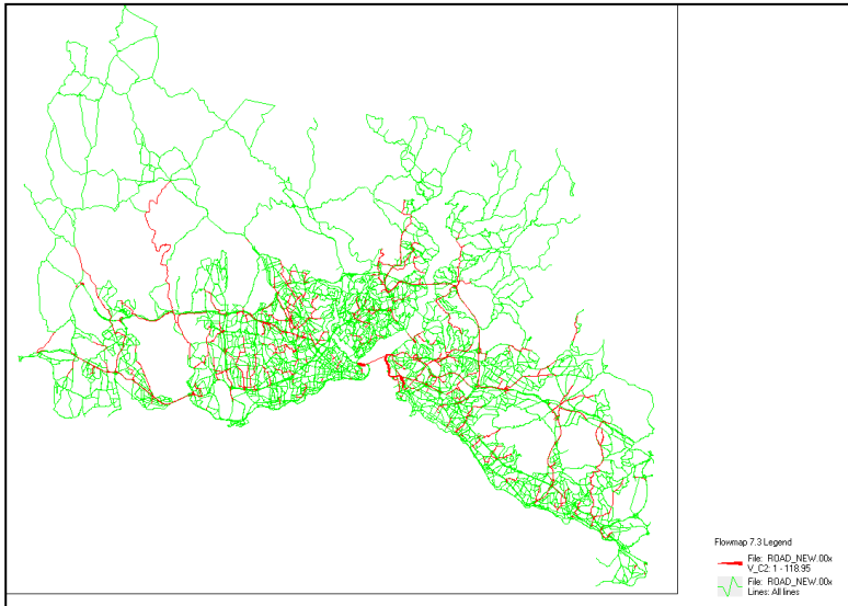
Figure 6-51: Volume-to-capacity ratio, option 2a
