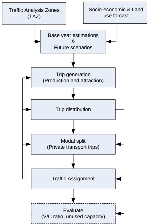
Figure 6-43: 4-Step transport model
