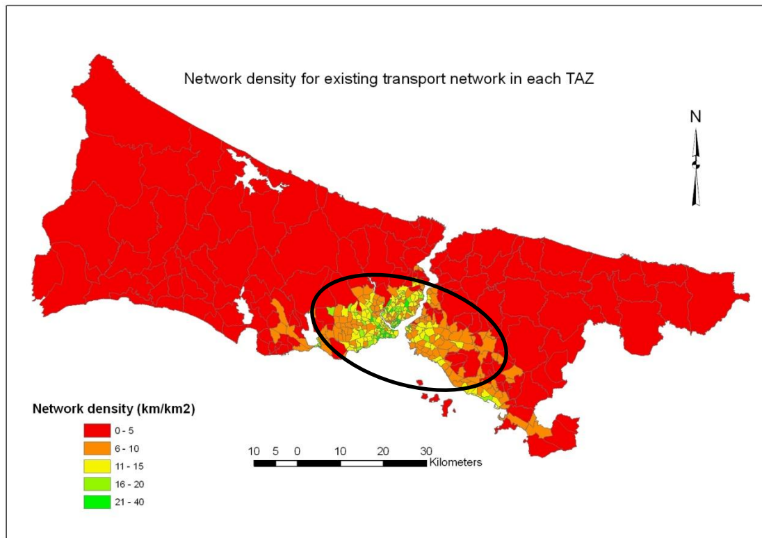
Figure 5-5: Network density for existing transport network in each TAZ, 2006
