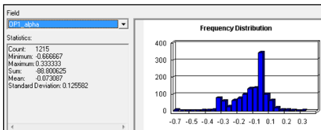
Figure 6-9: Histogram - Alpha index of urban Istanbul, existing network
