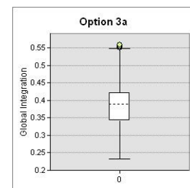
Figure 6-40: Box plot global integration – Option 3a
