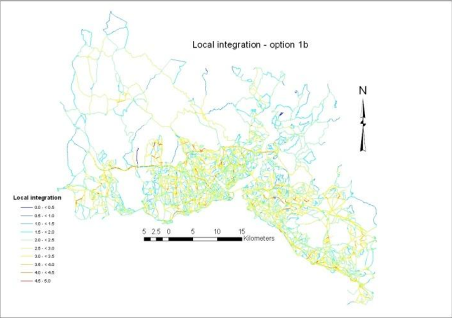
Figure 6-27: Local integration – Option 1b
