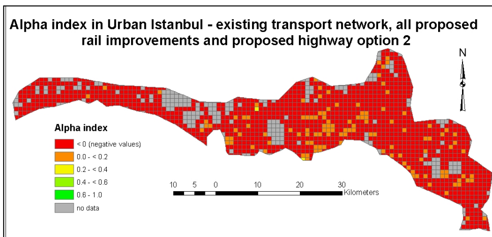
Figure 6-10: Alpha index of urban Istanbul – existing transport network, all proposed rail improvements and proposed highway option 2
