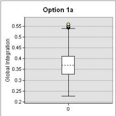
Figure 6-34: Box plot global integration – Option 1a (existing network)
