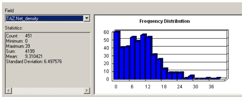
Figure 5-7: Network density histogram for existing transport network
