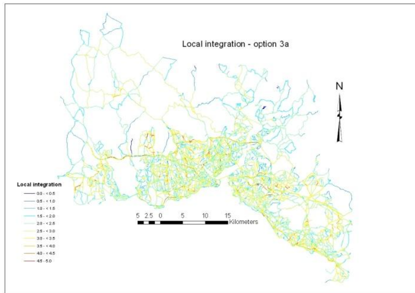
Figure 6-31: Local integration – Option 3a
