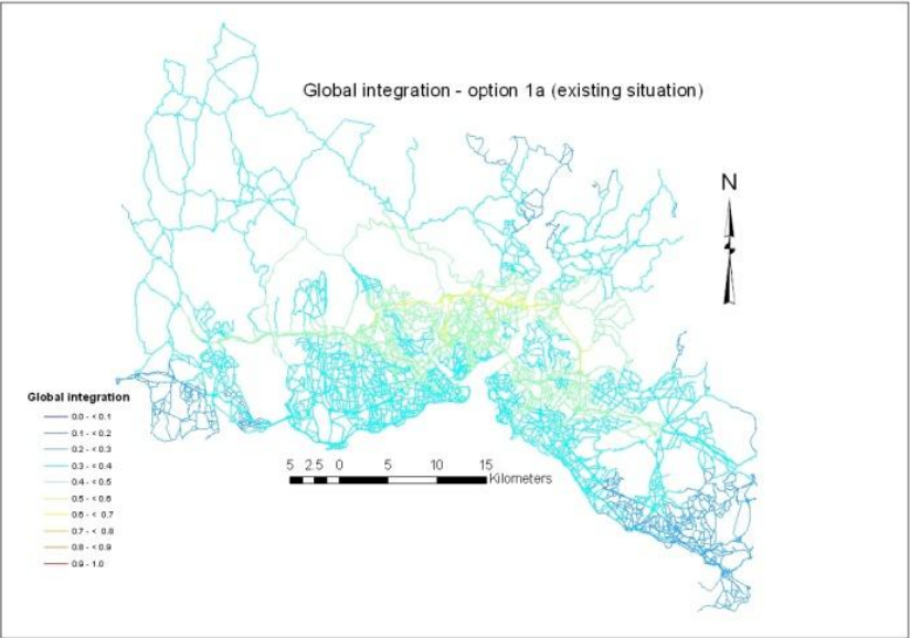
Figure 6-33: Global integration - Option 1a (existing network)
