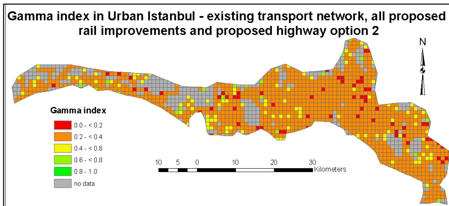
Figure 6-15: Gamma index of urban Istanbul – existing transport network, all proposed rail improvements and proposed highway option 2
