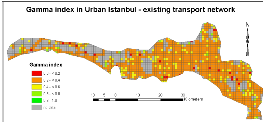
Figure 6-13: Gamma index of urban Istanbul – existing network
