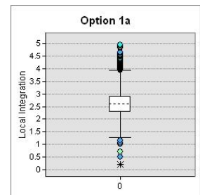
Figure 6-26: Box plot local integration – Option 1a (existing network)
