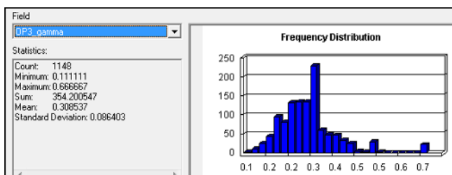
Figure 6-16: Histogram - Gamma index of urban Istanbul: existing transport network, all proposed rail improvements and proposed highway option 2
