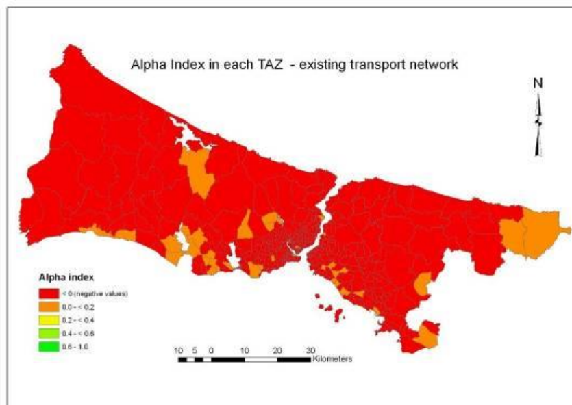
Figure 6-1: Alpha index in each TAZ – existing transport network
