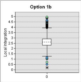
Figure 6-28: Box plot local integration – Option 1b
