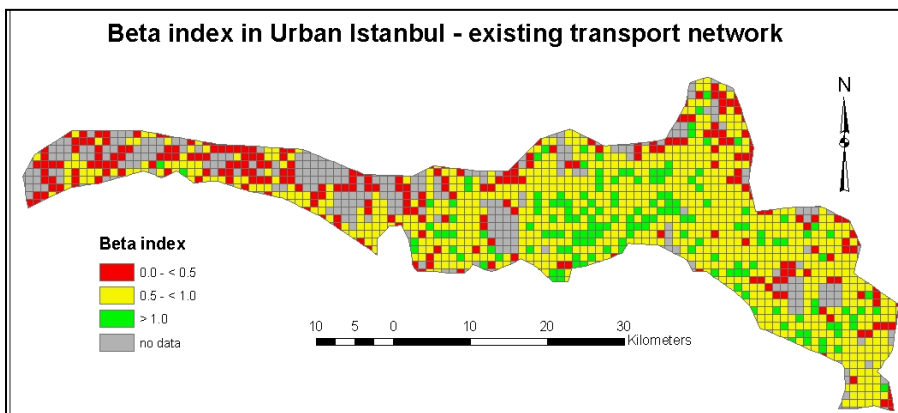
Figure 6-18: Beta index of urban Istanbul – existing network
