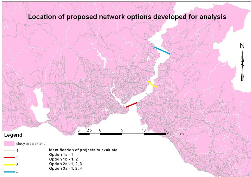
Figure 5-4: Location of proposed network options developed for analysis
