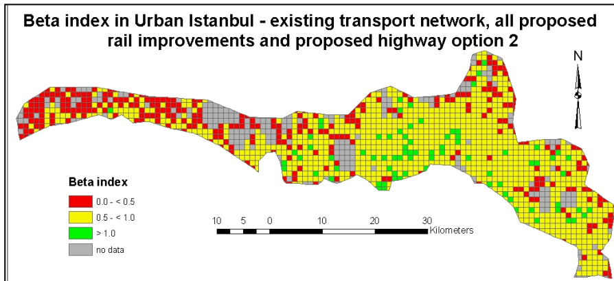
Figure 6-20: Beta index of urban Istanbul – existing transport network, all proposed rail improvements and proposed highway option 2
