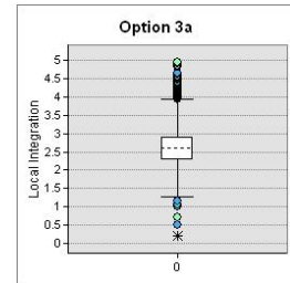
Figure 6-32: Box plot local integration – Option 3
