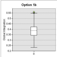
Figure 6-36: Box plot global integration – Option 1b
