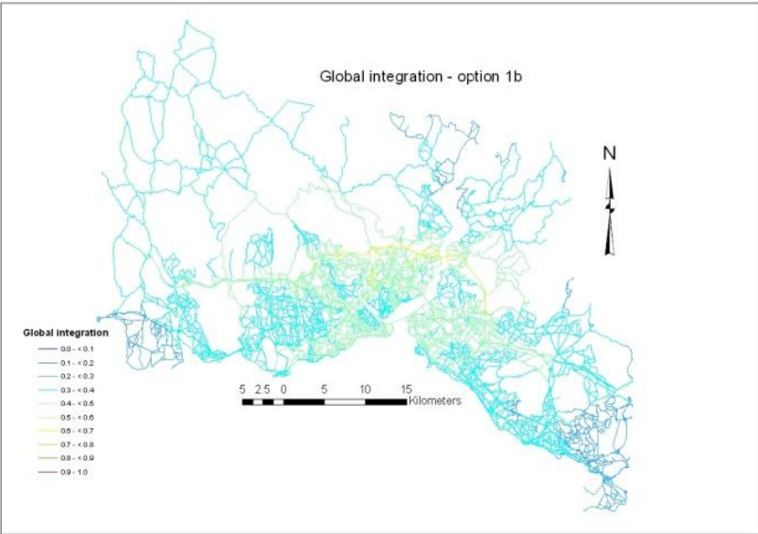
Figure 6-35: Global integration – Option 1b
