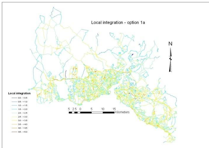
Figure 6-25: Local integration - Option 1a (existing network)
