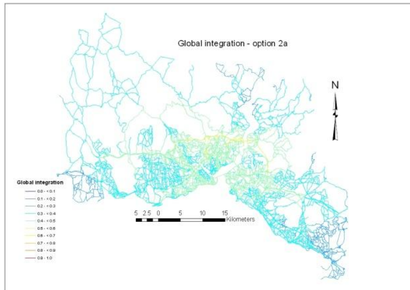
Figure 6-37: Global integration – Option 2a
