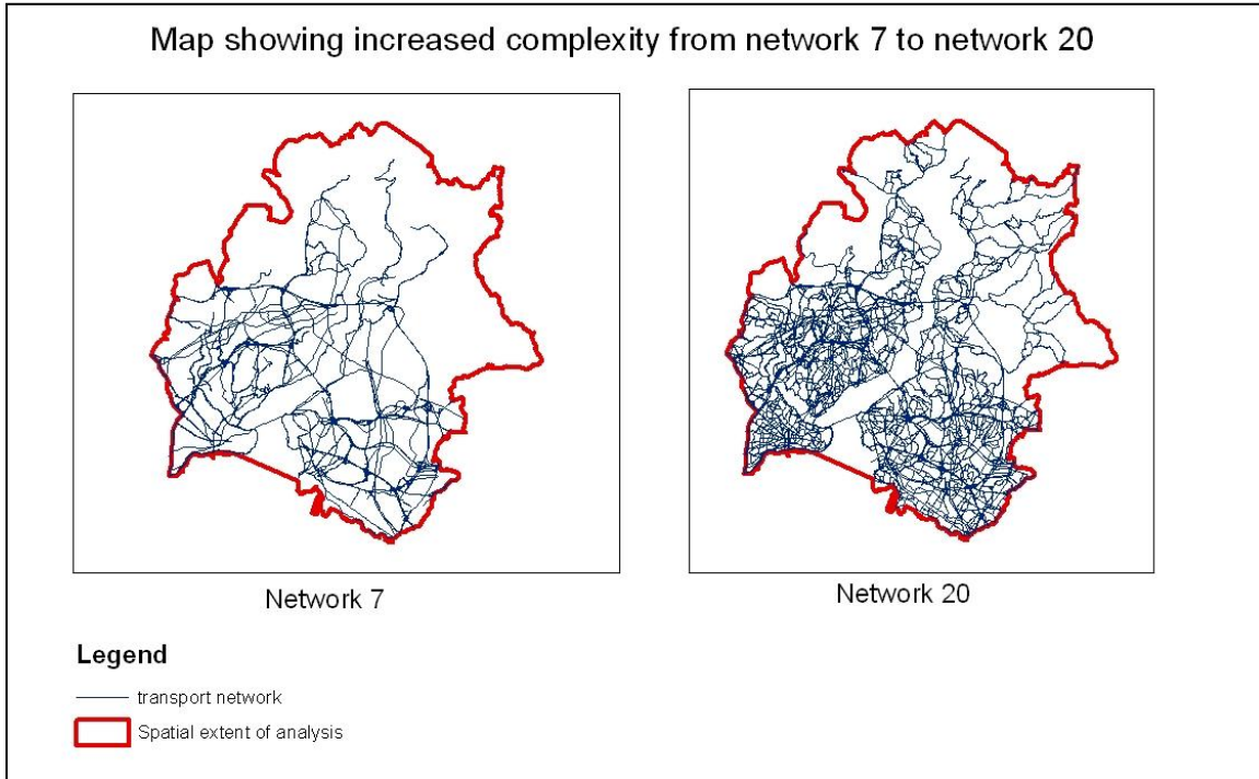
Figure 6-24: Level of complexity from network 7 to 20
