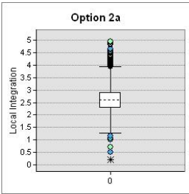
Figure 6-30: Box plot local integration – Option 2a
