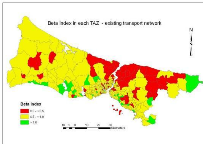
Figure 6-5: Beta index in each TAZ – existing transport network
