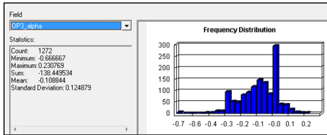
Figure 6-11: Histogram - Alpha index of urban Istanbul: existing transport network, all proposed rail improvements and proposed highway option 2
