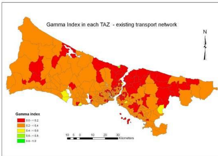
Figure 6-3: Gamma index in each TAZ – existing transport network
