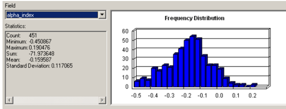
Figure 6-2: Frequency distribution – alpha index existing network
