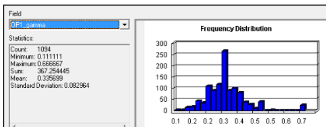
Figure 6-14: Histogram - Gamma index of urban Istanbul, existing network
