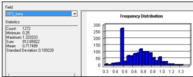
Figure 6-19: Histogram - Beta index of urban Istanbul, existing network
