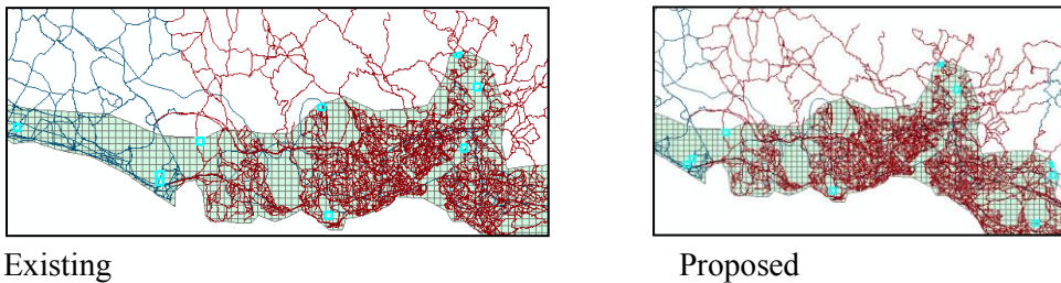
Figure 6-17: Top 10 gamma indicator in grid for existing and proposed situation (highlighted in blue)
