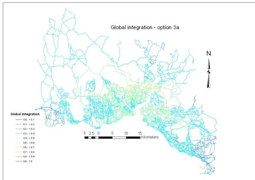
Figure 6-39: Global integration – Option 3a
