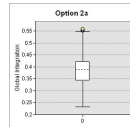
Figure 6-38: Box plot global integration – Option 2a
