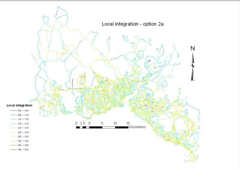
Figure 6-29: Local integration – Option 2a
