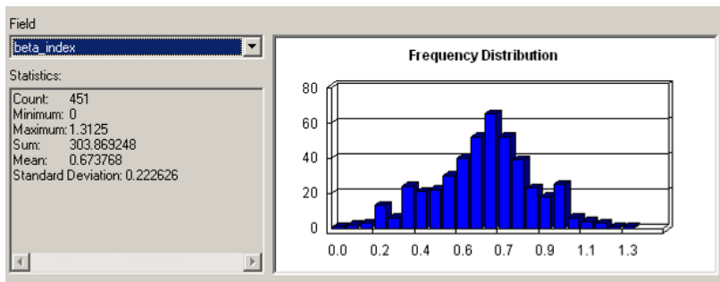
Figure 6-6: Frequency distribution – beta index existing network
