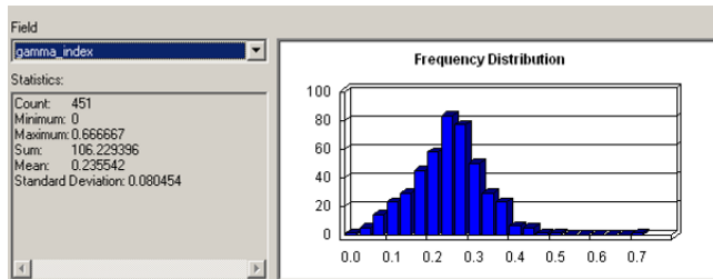
Figure 6-4: Frequency distribution – gamma index existing network
