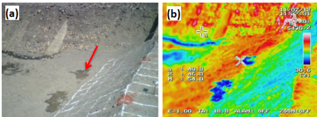
Figure 1.1: Base seepage downstream with (a) being a situation RGB image and (b) being a thermal image ( Chen et al., 2018 )
