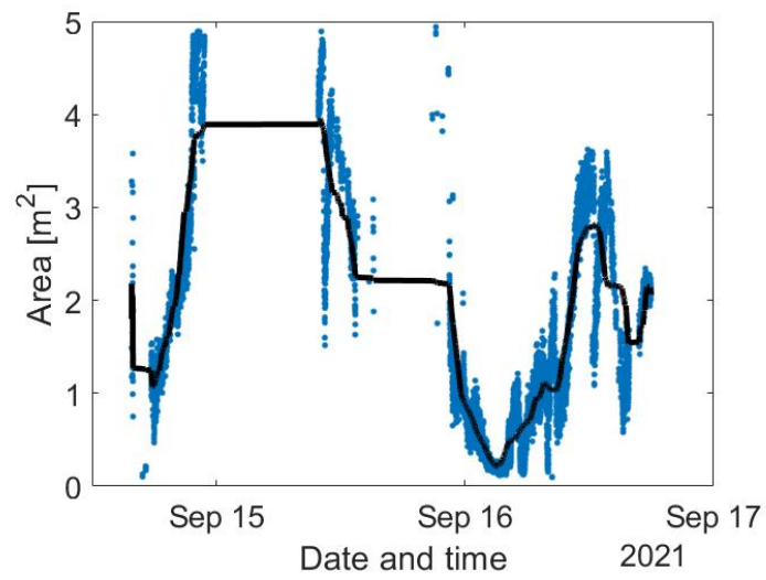
Figure E.4: Smoothed areas curve with a range of 0.6 °C plotted with the original data points.
