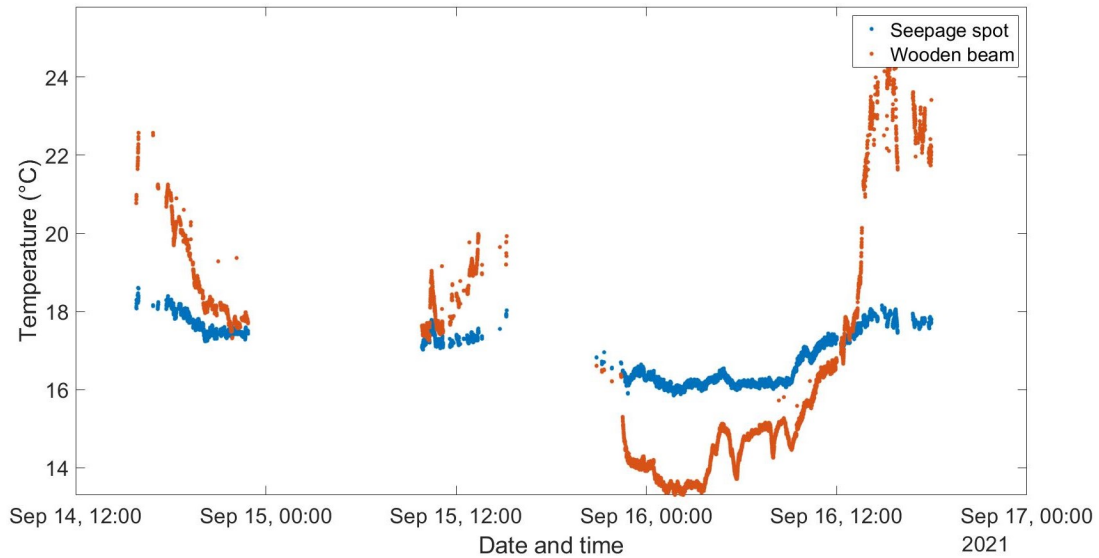
Figure 5.9: A plot of the core temperature of the main seepage spot and the ambient wooden beam temperature over time.
