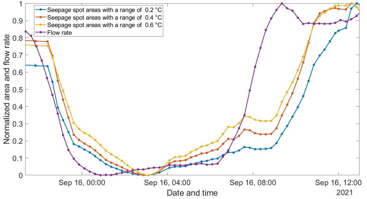
Figure 5.15: Normalized flow rate and areas for the time period of 15 September 21:20h up to 16 September 13:00h.
