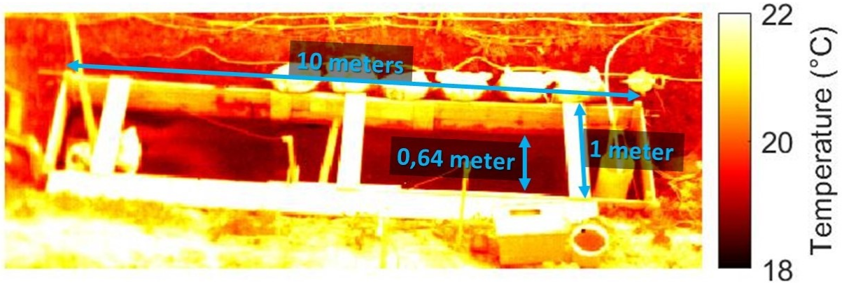
Figure 5.11: Known dimensions in the image which are used for the determination of the pixel size.
