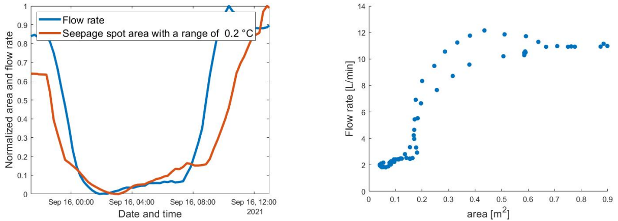
Figure 5.16: Scenario where the area with a range of 0.2 °C is correlated with the shifted flow rate. Left: a normalized plot of the flow rate and area in time. Right: a scatter plot of the flow rate versus the areas.
