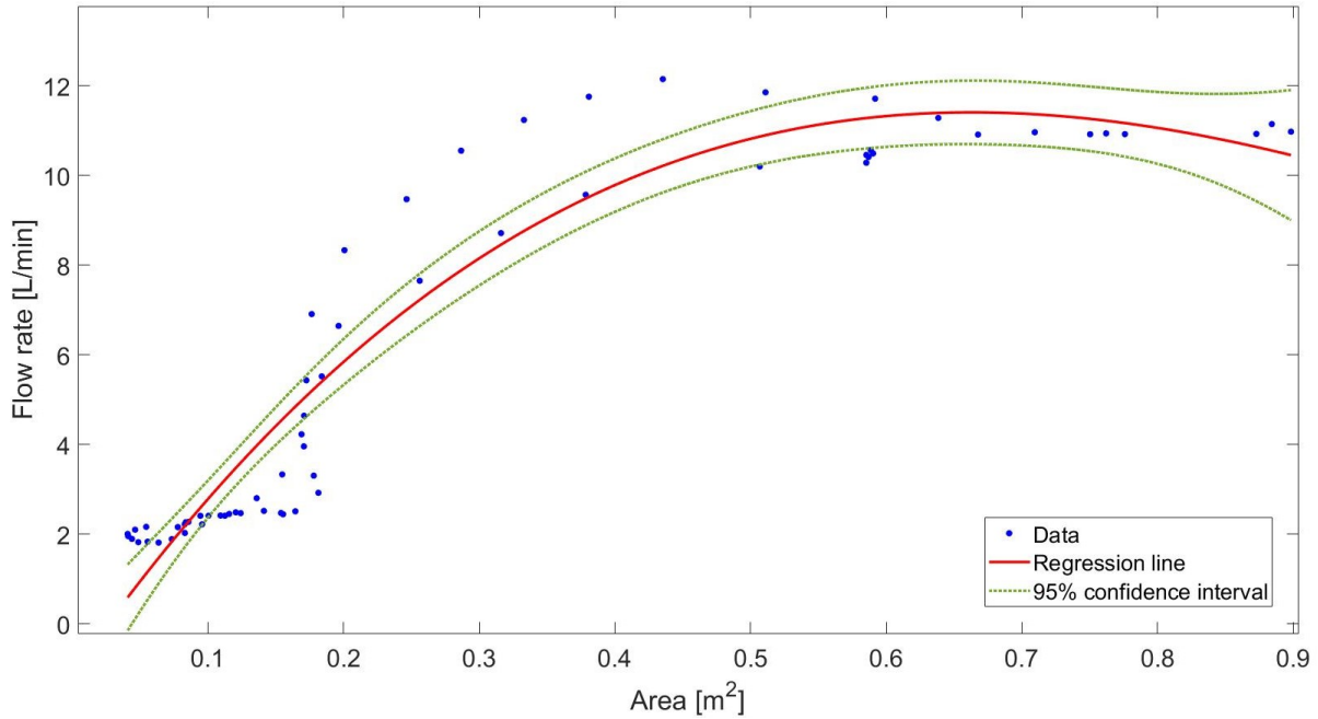
Figure 5.17: A third degree polynomial Regression line that represents the best correlating data set. The 95% confidence interval of the regression line is given as well.
