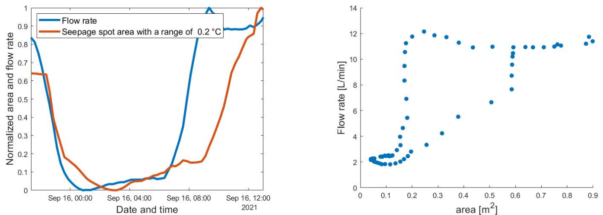
Figure F1: Scenario where the area with a range of 0.2 °C is correlated with the original flow rate. Left: a normalized plot of the flow rate and area in time. Right: a scatter plot of the flow rate versus the areas.
