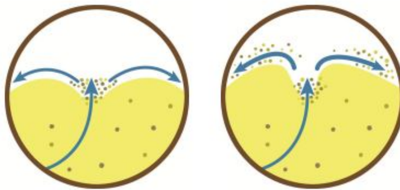
Figure 2.2: Left: a sand boil without sand deposition, the fluid flow is in equilibrium with the weight of the sand mass. Right: a sand boil with sand deposition, the flow velocity is high enough to deposit sand ( van Beek, 2015 ).
