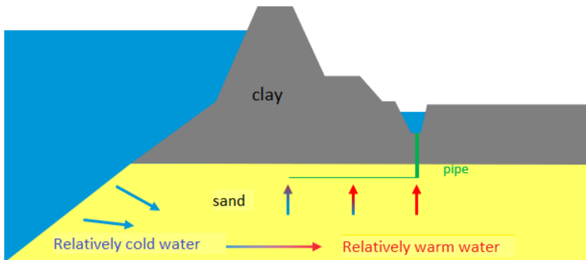
Figure 2.4: Temperature change of seepage water (van de Voort et al., 2021), an example of relatively cold infiltrating water which is changing to a higher temperature by the seepage process.
