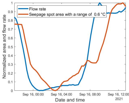
Figure F3: Scenario where the area with a range of 0.6 °C is correlated with the original flow rate. Left: a normalized plot of the flow rate and area in time. Right: a scatter plot of the flow rate versus the areas.
