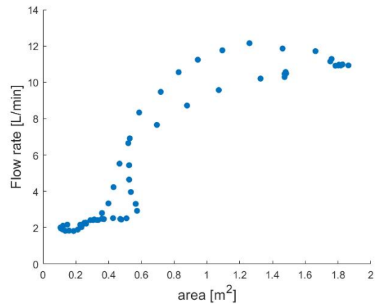
Figure F5: Scenario where the area with a range of 0.4 °C is correlated with the shifted flow rate. Left: a normalized plot of the flow rate and area in time. Right: a scatter plot of the flow rate versus the areas.
