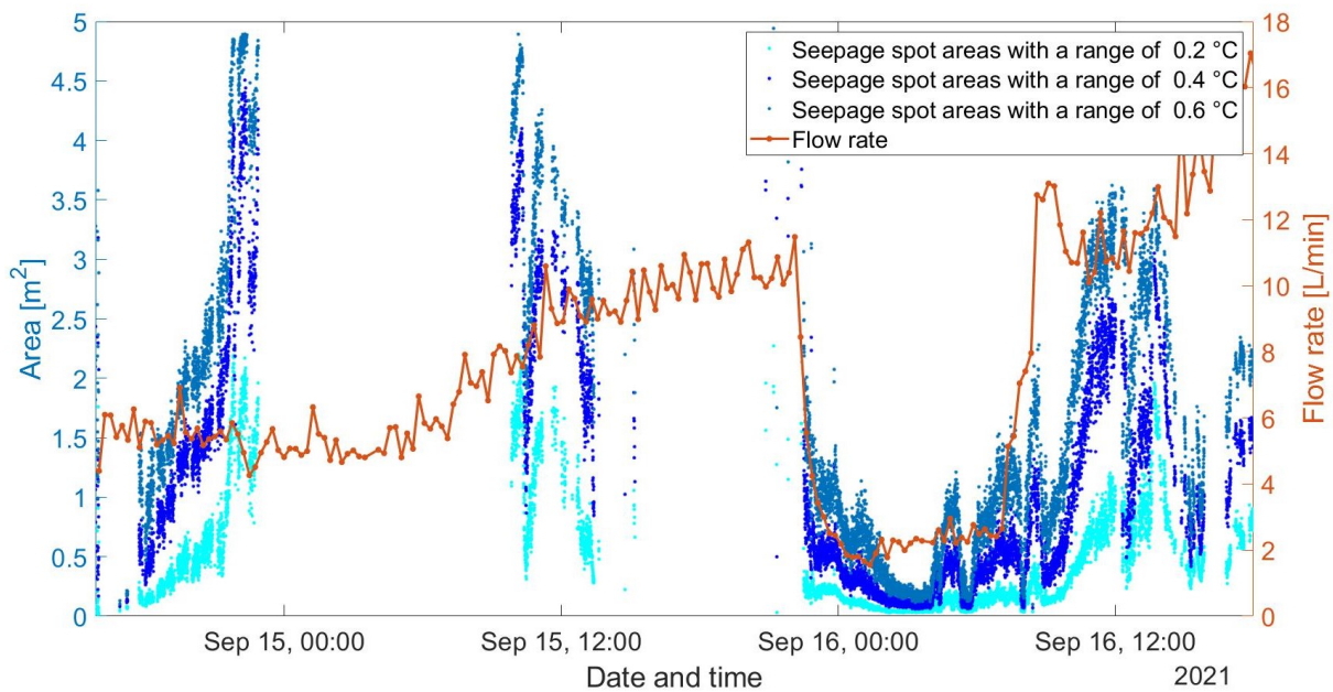
Figure 5.13: Flow rate compared with the areas of the seepage spots for different temperature ranges.
