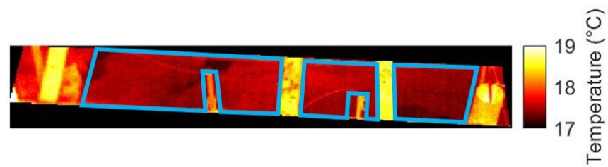
(e) Thermal image 15 September 18:06h
