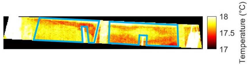
(b) Thermal image 15 September 00:01h
