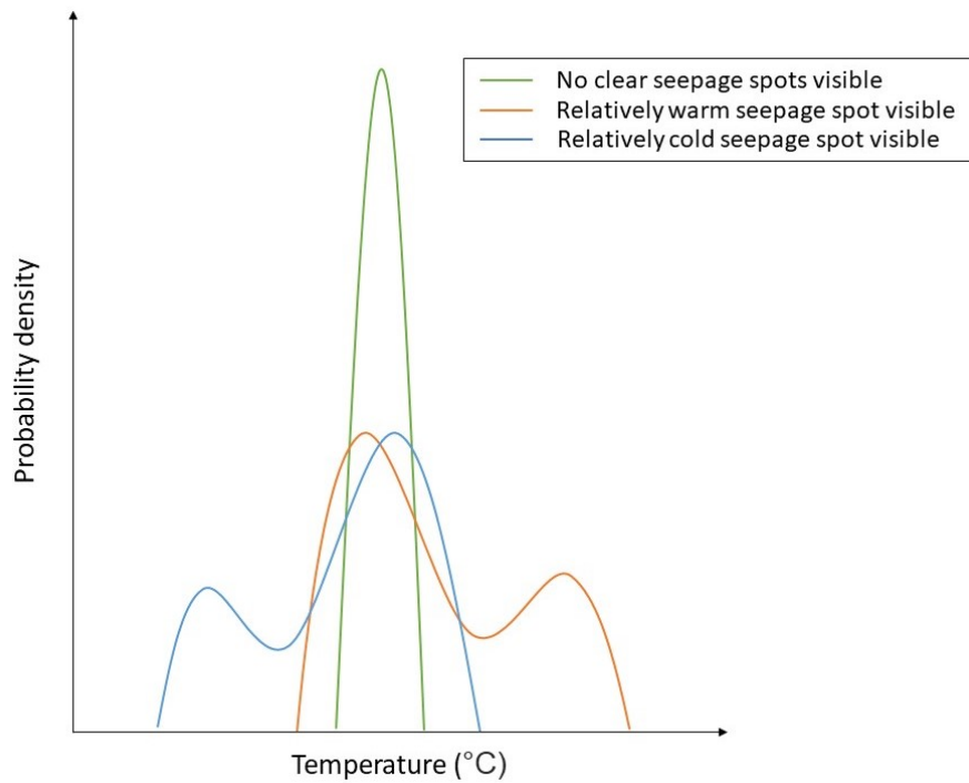
Figure 4.3: Expected temperature distributions in thermal images with and without seepage spots, based on the methods of Jiang et al. (2016) and Tsanakas and Botsaris (2012)
