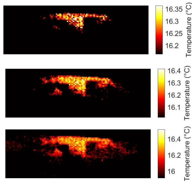
Figure 5.8: The quantified area for three different temperature ranges: 0.2 °C (top), 0.4 °C (middle) and 0.6 °C (bottom) where the yellow/orange/red colors indicate the pixels that are counted as the area. The image is a cropped part of the ditch.
