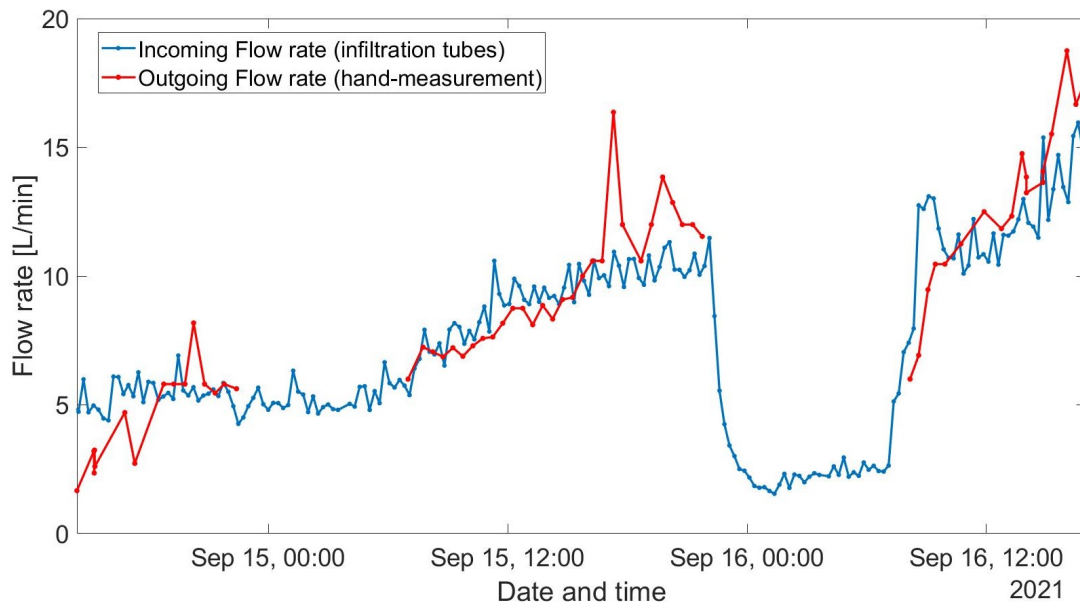
Figure 3.4: Comparison of the flow rate at the infiltration tubes and the hand-measured flow rate out of the ditch.
