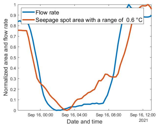
Figure F6: Scenario where the area with a range of 0.6 °C is correlated with the shifted flow rate. Left: a normalized plot of the flow rate and area in time. Right: a scatter plot of the flow rate versus the areas.
