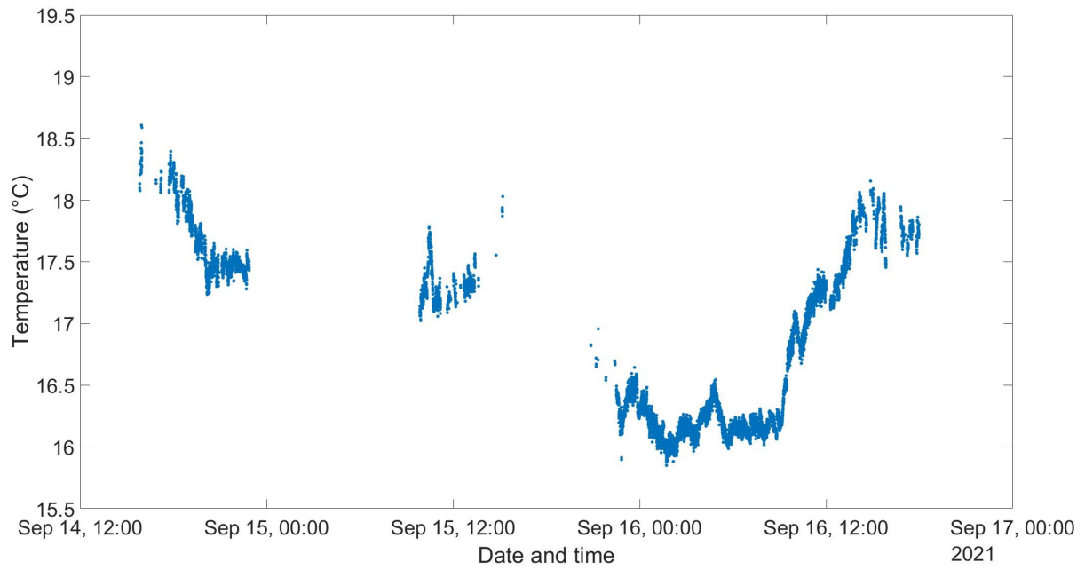
Figure 5.7: A plot of the core temperature of the main seepage spot over time.
