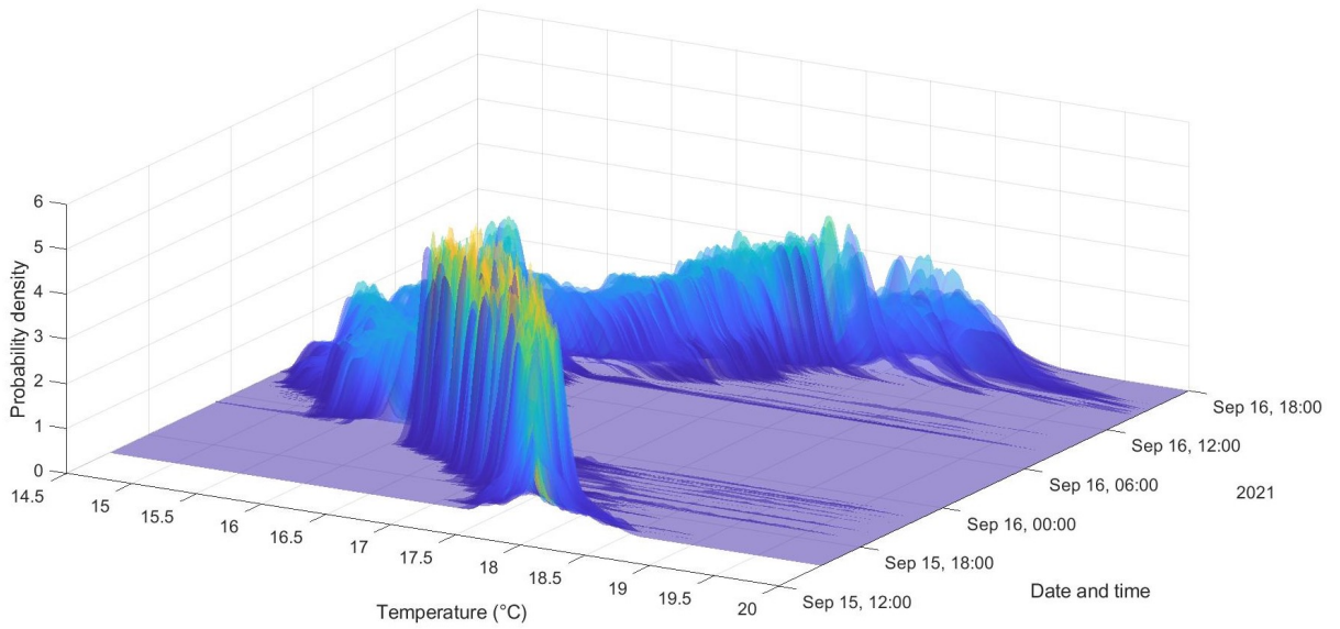
Figure 5.5: Plot of all fitted curves in time for Setting 3 with the purpose to show temperature differences in thermal images
