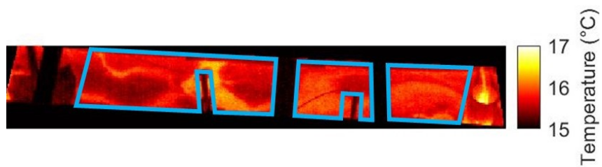
(f) Thermal image 16 September 6:00h
