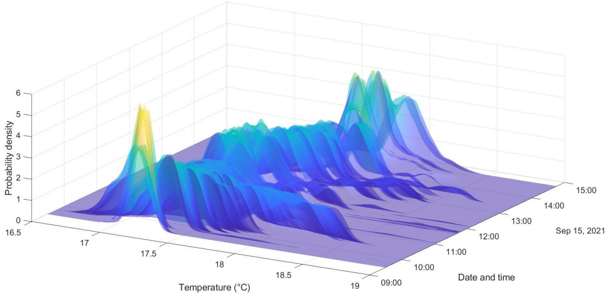
Figure 5.4: Plot of all fitted curves in time for Setting 2 with the purpose to show temperature differences in thermal images
