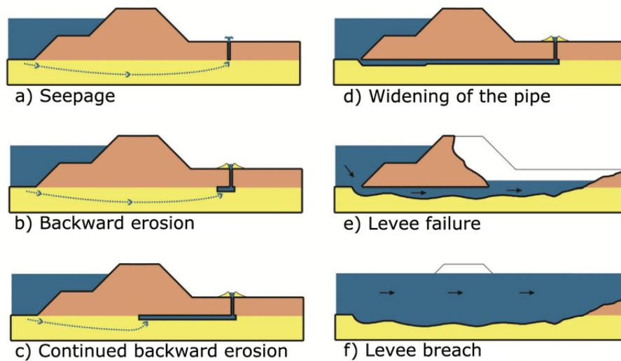
Figure 2.1: The phases of the piping process (Semmens and Zhou, 2019).
