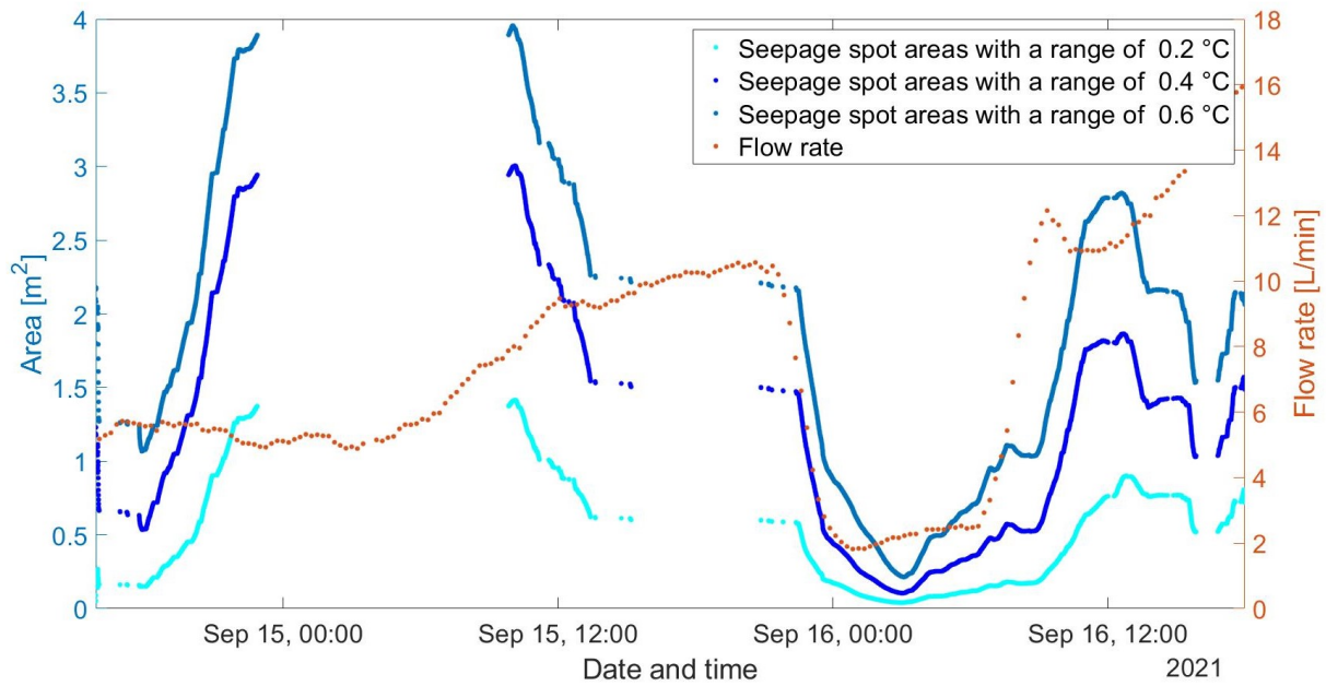
Figure 5.14: Flow rate compared with the smoothed areas of the seepage spots for different temperature ranges.
