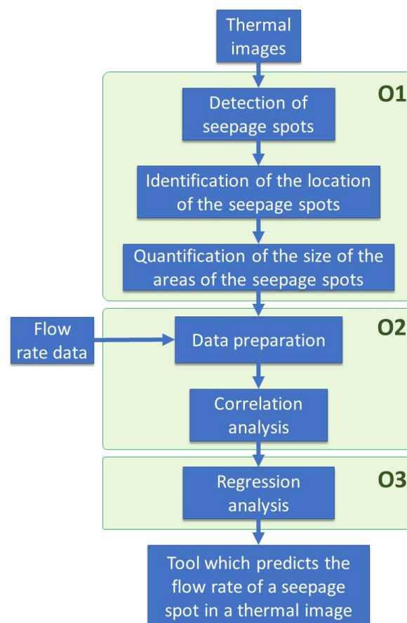
Figure 4.1: Flow chart of the methodology which summarizes the steps taken in the study, where the green squares make a division per objective (O).
