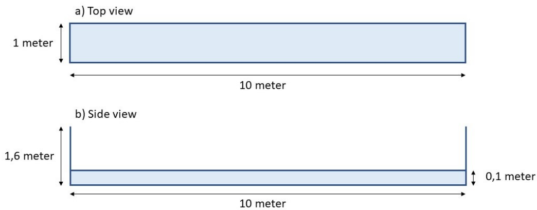
Figure 3.2: Schematic drawing of the dimensions of the ditches at the LLHPP.
