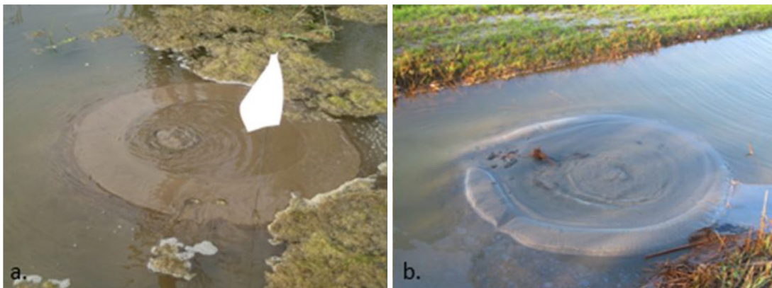
Figure 2.3: Two examples of a typical sand boil in the ditch on the outside of the river dyke. Locations: a. Mississippi River b. Waal River Netherlands. The size can range from millimeters to meters in diameter (Talukdar and Dey, 2019).
