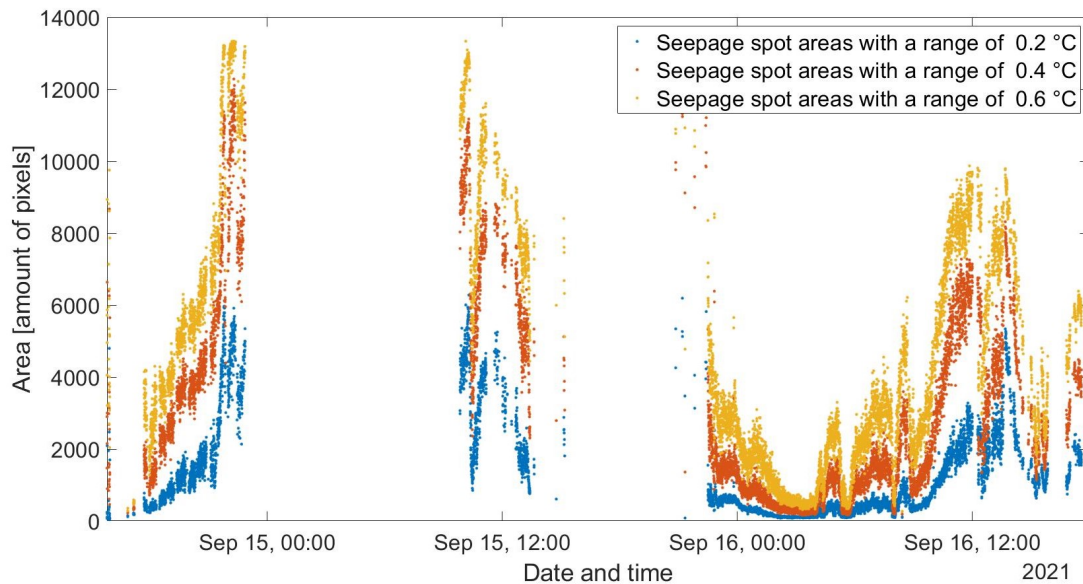
Figure 5.10: The extracted areas from the thermal images in amount of pixels over time for the three different temperature ranges.
