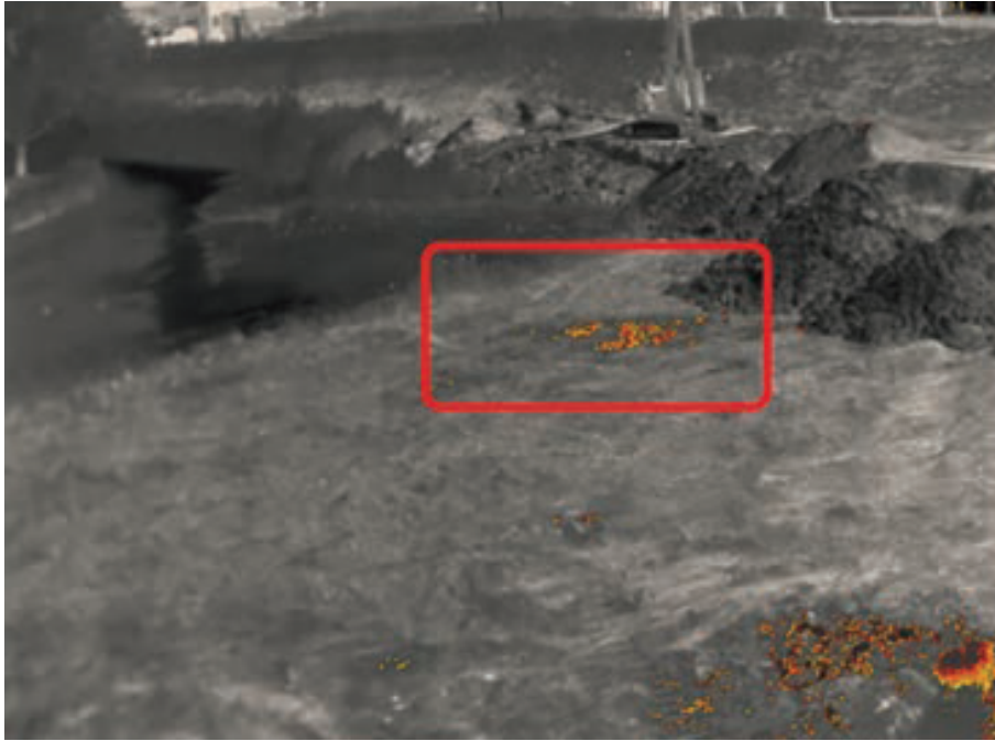
Figure 1.2: Seepage seen in a thermal image, the rectangle with rounded corners indicates one of the seepage spots where the colors indicate seepage spot by lighting up a certain temperature ( Wiggers et al., 2019 )
