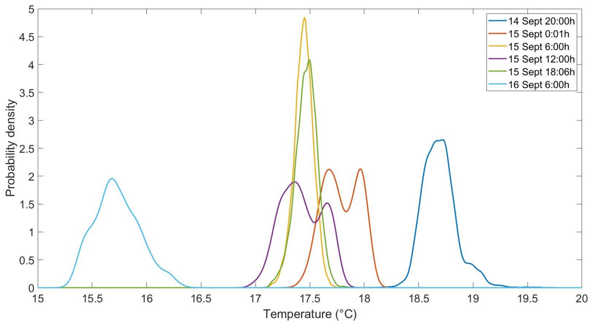
Figure C.1: Examples of fitted curves showing narrow ranges with high peaks and wide ranges with low peaks, the corresponding thermal images can be seen in Figure C.2a to Figure C.2f.
