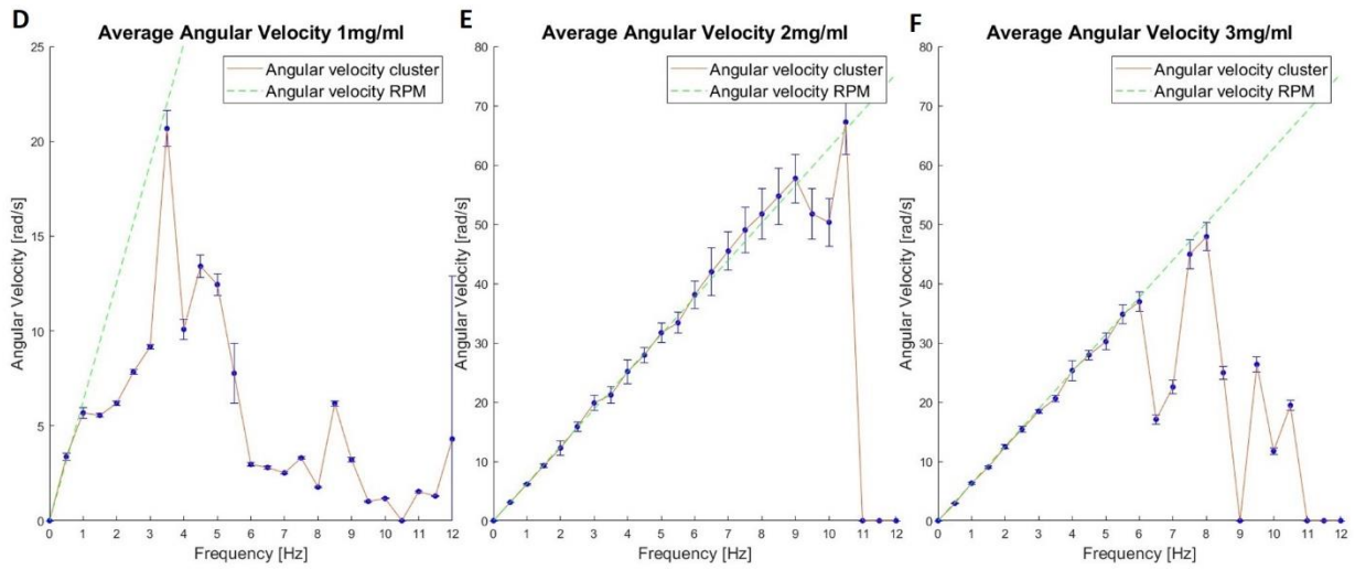
Figure 4 As clusters of IRONSperm are actuated by the RPM they perform a rolling locomotion over the surface of the PVC tube. In this case, the clusters are actuated to the right. (A-C) Samples 2-4 are actuated by the RPM at a frequency of 1.5Hz. The respective cluster diameters are 1.41mm, 1.2mm, and 2.83mm based on the prolate ellipses drawn over the clusters. (D-F) The average angular velocities of samples 2-4 as they are actuated at frequencies from 0.5-12Hz compared to the angular velocity of the RPM. The respective step-out frequencies of samples 2 and 4 are 3.5 and 6Hz. For sample 3 no step-out frequency could be determined.
