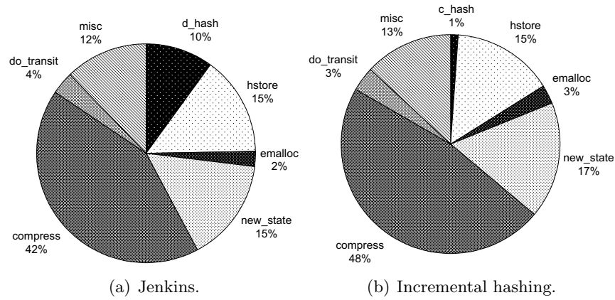
Figure 6.1: Percentual stakes of six most time-consuming functions for BEEM benchmarks compiled with -O0.
