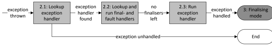
Figure 3.4: Flow diagram of exception handling mode.
