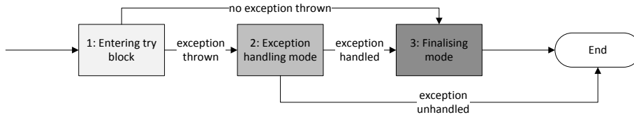
Figure 3.3: Global overview of structured exception handling.
