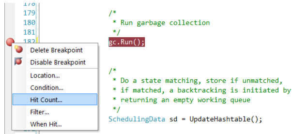
Figure A.1: Setting a hitcounter breakpoint before the garbage collector is called.
