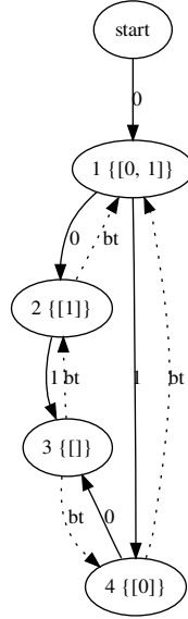
Figure A.3: An example state space visualised by GraphViz's dot.
