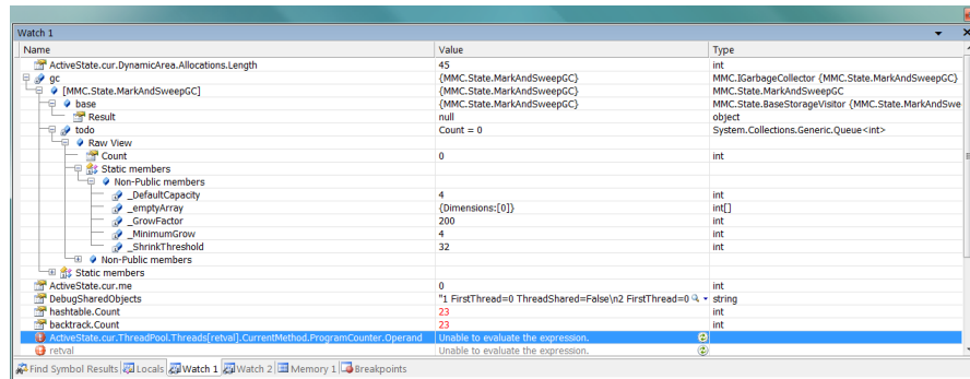
Figure A.2: Watch window upon a breakpoint.
