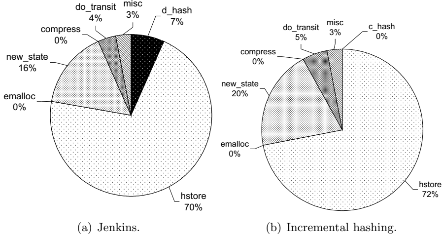
Figure 6.2: Percentual stakes of six most time-consuming functions for BEEM benchmarks compiled with -O3.
