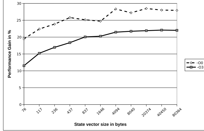
Figure 6.3: Relative performance gain of the incremental hash function with Szymanski's mutual exclusion model plotted against the state vector size.
