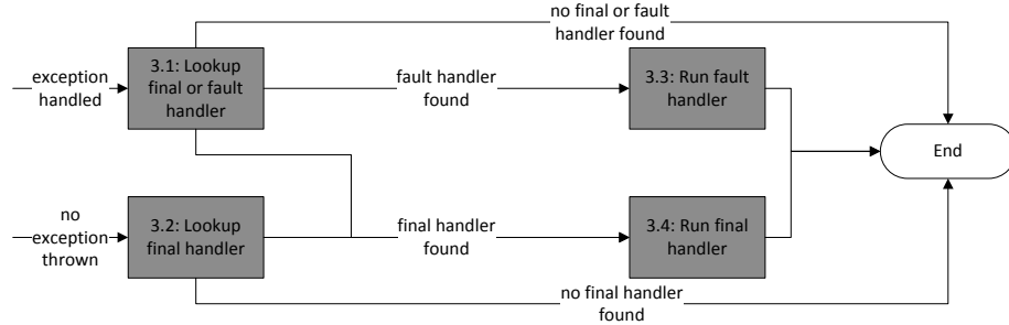
Figure 3.5: Flow diagram of finalising mode.
