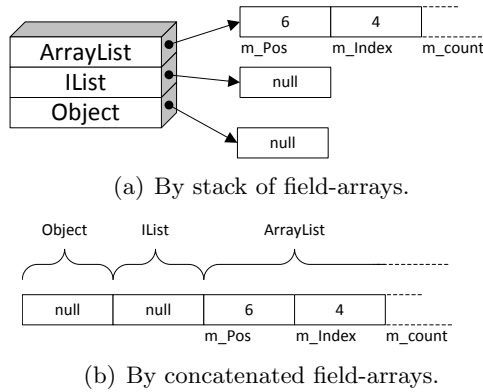
Figure 3.6: Modelling inherited fields.
