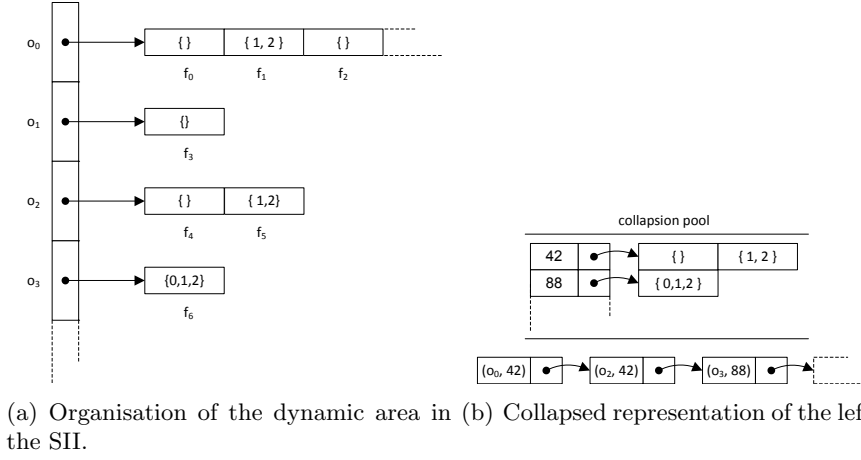
Figure 4.1: SII organisation and collapse.
