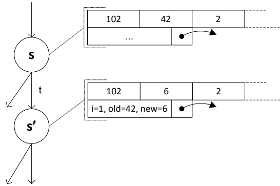
Figure 3.8: The linked list in the ChangingIntVector associated with state s' contains the changes between itself and state s .
