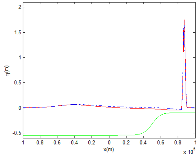
Figure 4.4: Comparison of numerical (blue dashed line) and analytical (red solid line) solution for mild slope ( w = 10km )
