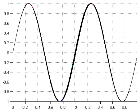
Figure A.16: Initial condition of harmonic waves
