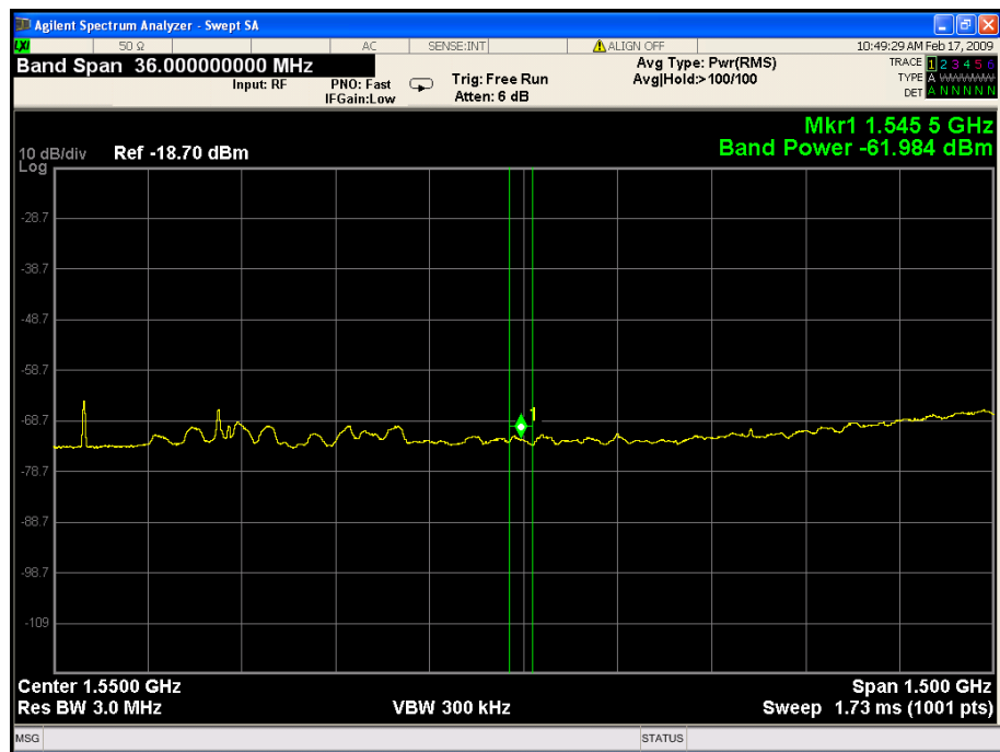
Figure 6.12: DVB Signal with OBPN Desynchronized
