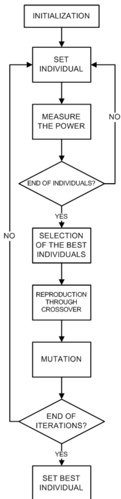
Figure 5.4: Genetic Algorithm Flow Diagram
