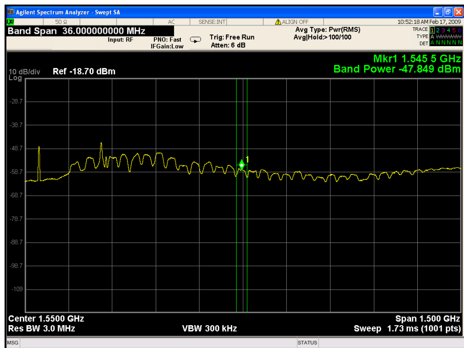
Figure 6.13: DVB Signal with OBPN Synchronized: The transponders are all clearly visible
