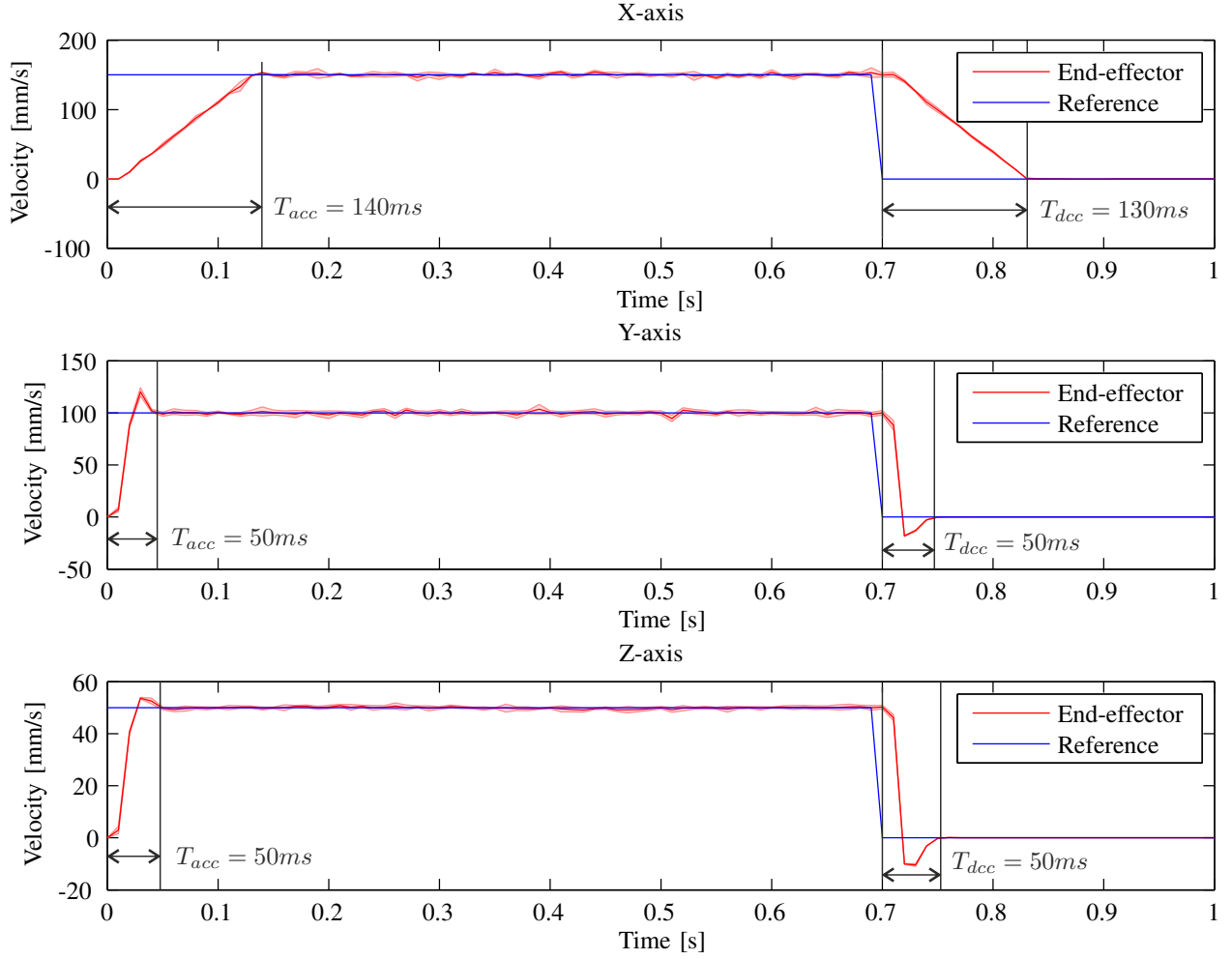
Fig. 6. The velocity responses to the applied velocity profiles (Fig. 5). T_{acc} describes the time to accelerate to reach the required velocity, while T_{dcc} describes the time to decelerate to zero velocity.
