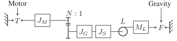
Fig. 4. The Ideal Physical Model (IPM) of a linear stage, including motor, gear head, lead screw, load mass and the loads gravitational force. T represents the torque delivered by the electric motor, while F describes the gravitational force acting on the load mass ( M_L ). Further, J_M , J_G and J_S describe the inertias of the motor, gear head and lead spindle, respectively. N describes the gear head reduction ratio, while L describes the lead (pitch) of the lead screw.
