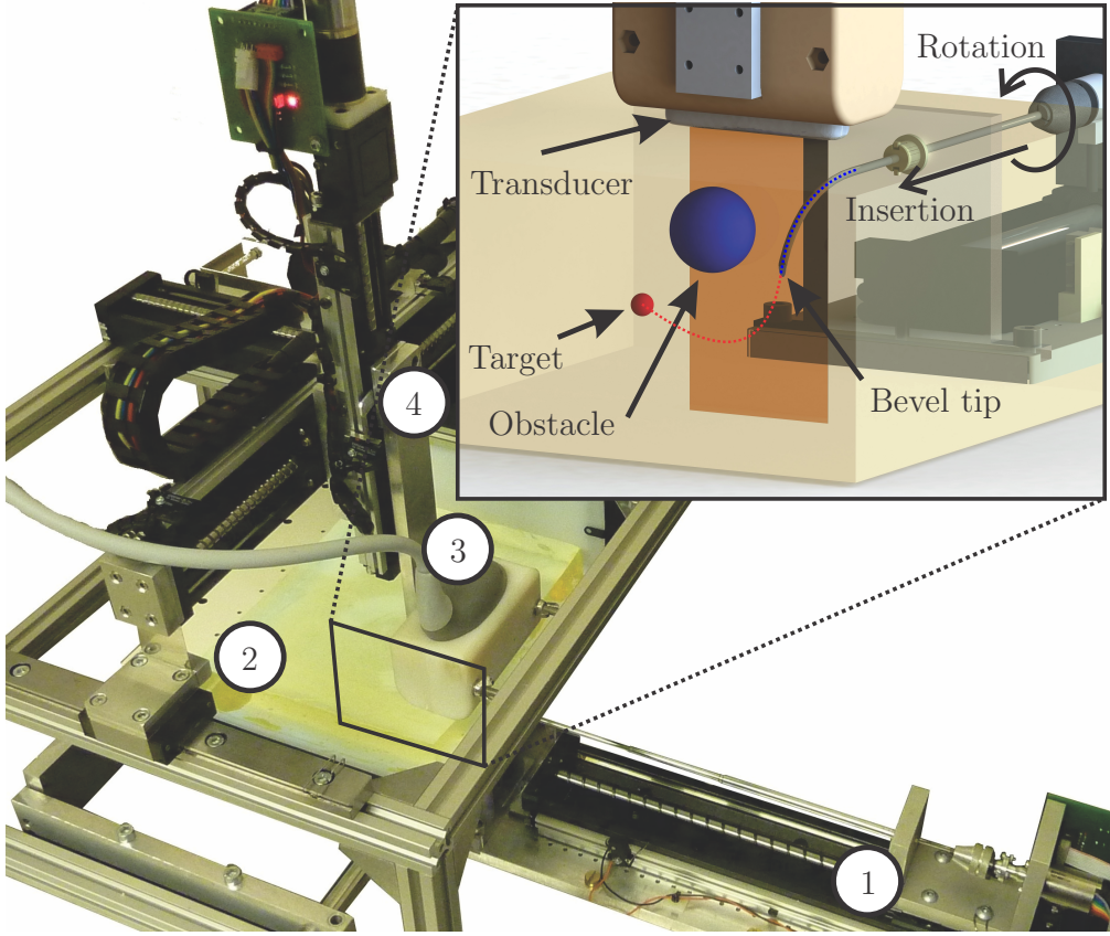
Figure 7: The experimental setup used to track and steer a flexible needle to reach a target while avoiding an obstacle. The needle, which is controlled at its base (inset) by a needle insertion device ① is inserted into the soft-tissue simulant ②. The two-dimensional ultrasound transducer ③ is positioned above the needle tip during insertion by a transducer positioning device ④, which provides feedback for steering.
