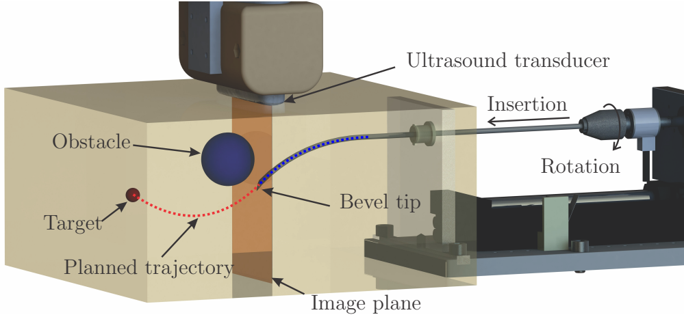
Figure 1: A flexible bevel-tipped needle is steered in the soft-tissue simulant by using a device that inserts and rotates the needle. The needle deflects along a curved trajectory in the direction of the bevel tip. A two-dimensional ultrasound transducer, which is orientated perpendicular to the needle insertion direction, is used to track the needle tip in three-dimensional space during insertion. A transducer positioning device is used to track the needle tip during insertion in order to compute the needle tip pose. The needle tip pose is used to plan and control the needle motion along a desired trajectory to reach a target while avoiding obstacles.
