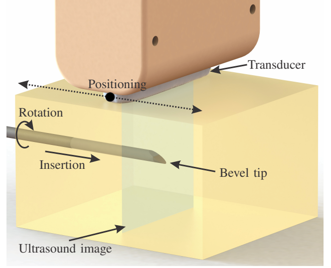
Fig. 2. A flexible bevel-tipped needle is inserted in the soft-tissue simulant. During insertion the needle deflects along a curved trajectory in the direction of the bevel-tip. An two-dimensional ultrasound transducer is placed perpendicular to the needle insertion-axis. The transducer is relocated along the insertion-axis at the needle tip during insertion to provide visual feedback.
