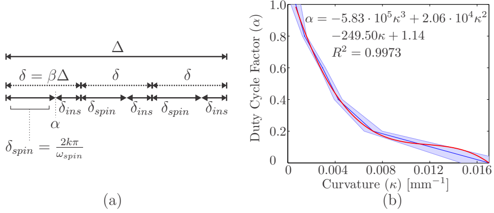
Figure 6: (a) The time duration ( \Delta ) is split into multiple (three) intervals of duration \delta each for \beta = 1/3 . Each interval is then composed of two intervals: (I) a spin interval of duration \delta_{\text{spin}} = (2k\pi/\omega_{\text{spin}}), k \in \mathbb{Z} in which the needle is both inserted and rotated, and (II) an insertion interval of duration \delta_{\text{ins}} in which the needle is only inserted without any rotation. (b) Characterization of the relationship \alpha = h(\kappa) for needle insertion in the soft-tissue simulant.
