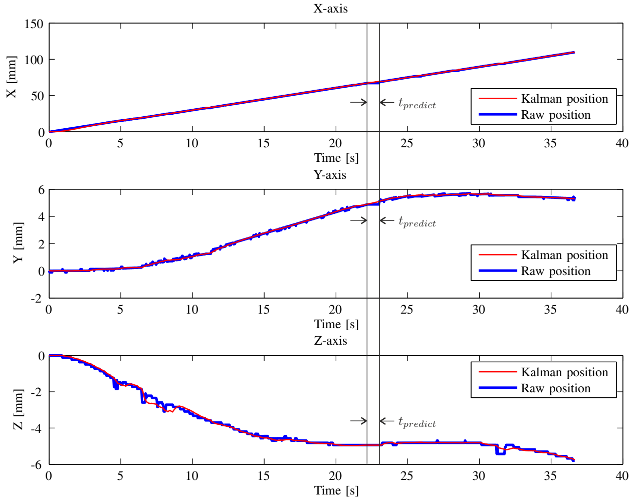
Fig. 2. The position measurements of the needle during insertion. t_{predict} describes a single time interval when no measurement was available and the Kalman observer predicts the subsequent states. The three plots show the needle tip position of the Kalman observer (red) and the raw needle tip position directly determined from image processing (blue).
