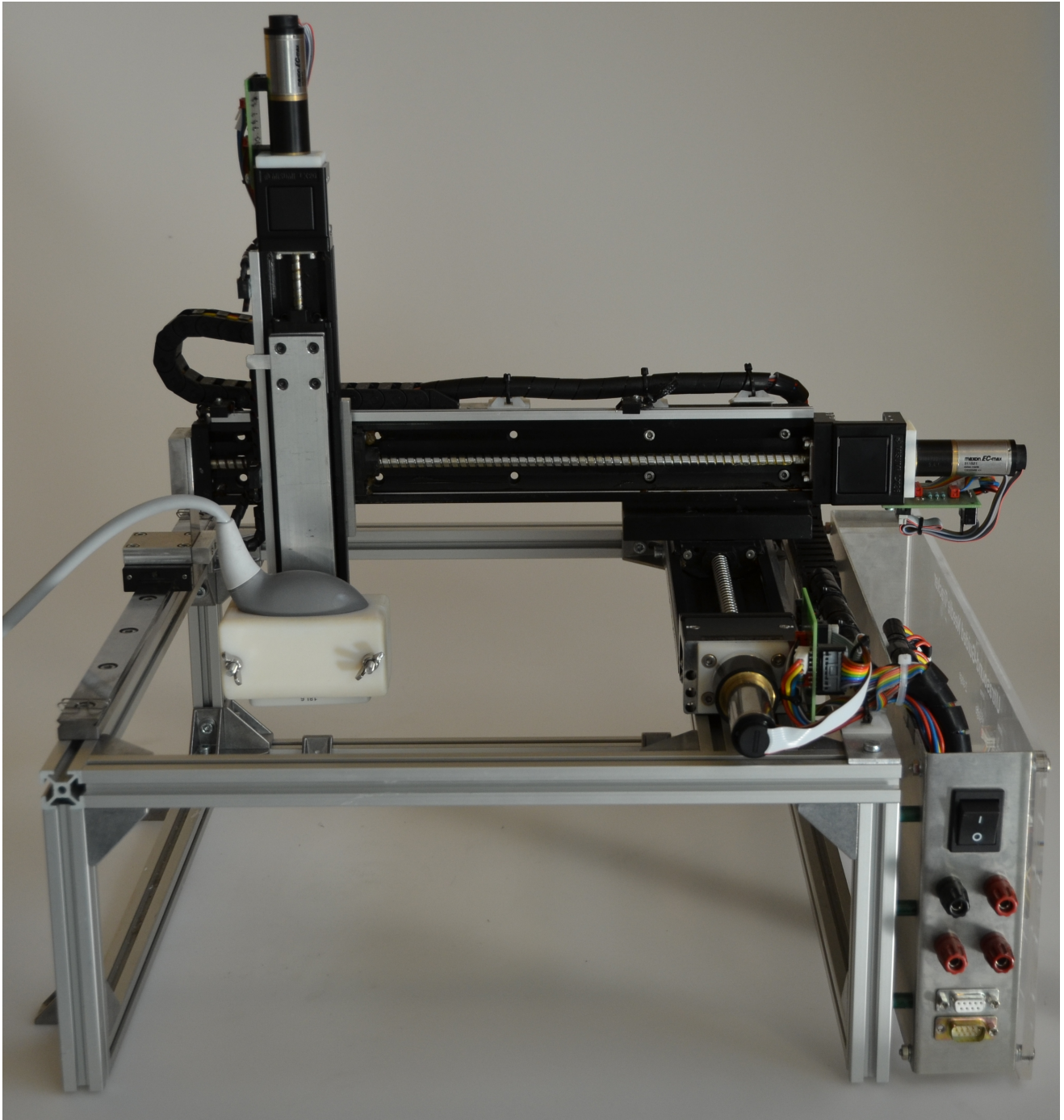
Fig. 4. Picture of the ultrasound positioning device holding the ultrasound transducer.
