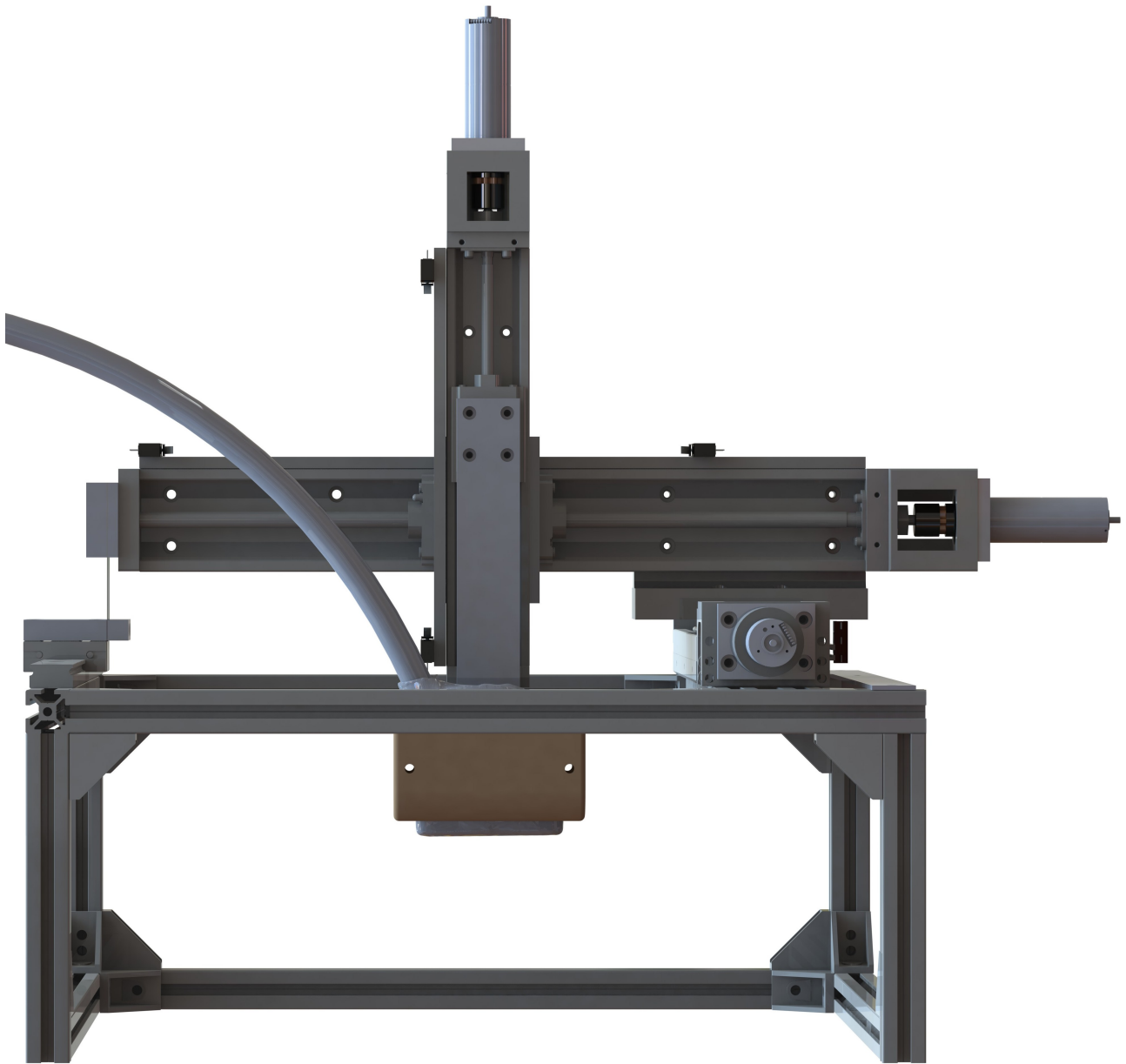
Fig. 1. Solid Works Drawing of the ultrasound positioning device (Front view).
