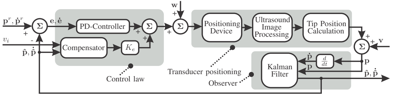
Fig. 4. The controller architecture used to track the needle tip in real-time, as it is inserted through the soft-tissue simulant. Transducer positioning along the x -axis ( \Psi_0 ) is performed by a compensator and gain scheduler ( K_e ) according to (3) and (7), respectively. The proportional-derivative-(PD)-controller (proportional gain ( K_p = 0.4 ) and derivative gain ( K_d = 0.1 )) is used to compensate the needle tip motion along the y -axis (frame ( \Psi_0 )), while motion in z -axis (frame ( \Psi_0 )) is not compensated for. A cartesian robotic system is used to position the ultrasound transducer at the needle tip to measure its position, which is denoted by \mathbf{p} . The time derivative of \mathbf{p} results in \dot{\mathbf{p}} . The reference positions and velocities are denoted by \mathbf{p}^r and \dot{\mathbf{p}}^r , respectively. The Kalman observer is used to minimize the effects of process ( \mathbf{w} ) and measurement ( \mathbf{v} ) noise on the states ( \mathbf{p} and \dot{\mathbf{p}} ), and to predict the subsequent state.
