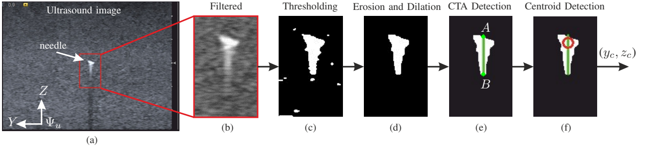
Fig. 2. Image processing methodology to determine the needle centroid location (y_c, z_c) in the ultrasound images. (a) The ultrasound input image is a radial cross-sectional view of the needle with the comet tail artifact (CTA). (b) In order to minimize speckle in the ultrasound image, a median filter is applied to the needle with the CTA. (c) A binary image is obtained by thresholding. (d) The remaining speckle in the image is removed by erosion and dilation. (e) A line detection algorithm using Hough transform is applied to detect the needle with the CTA. This line is denoted \overline{AB} . (f) In \overline{AB} , A represents the needle surface. The needle centroid (y_c, z_c) is evaluated as the center of the red circle (since the diameter of the needle is known).
