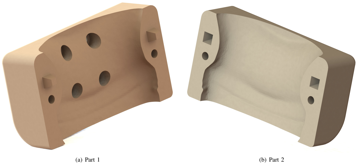
Fig. 6. Two-dimensional (2D) ultrasound transducer clamp. The 2D ultrasound transducer is mounted to the positioning device in a fixed pose using a clamp. (a) Part 1 of the clamp is mounted to the end-effector of the positioning device, while (b) Part 2 of the clamp is used to fix the transducer in Part 1. The designed clamp is 3D printed using a Eden 250 3D printer (Objet Ltd., Rehovot, Israel).
