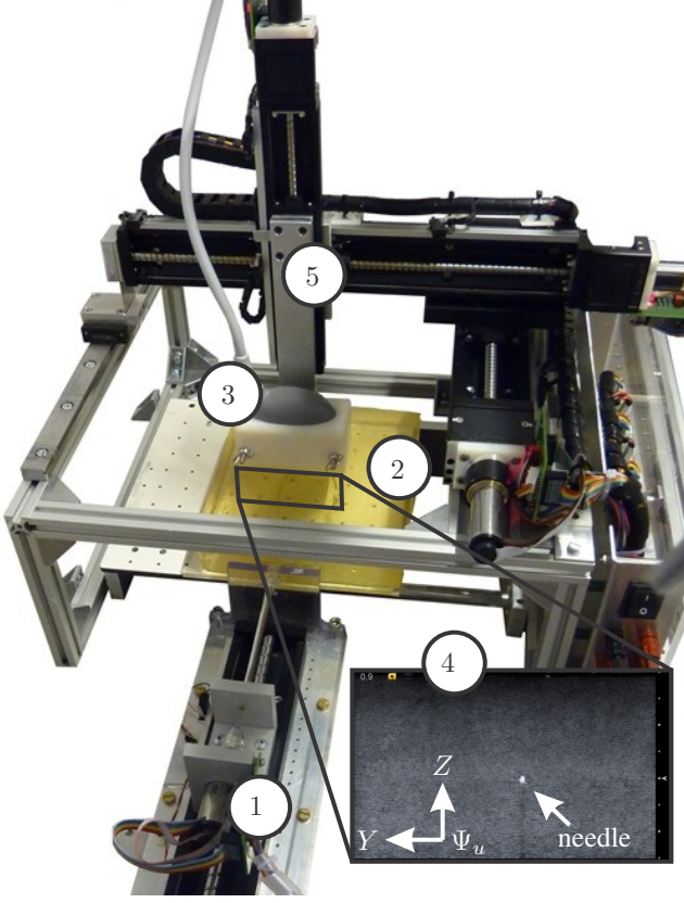
Fig. 5. The experimental setup used for three-dimensional needle tip tracking. ① Needle insertion device. ② Soft-tissue simulant based on gelatin mixture. ③ Ultrasound transducer. ④ Ultrasound image with a radial cross-sectional view of the needle. ⑤ Robotic ultrasound transducer positioning device.
