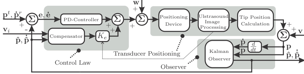
Figure 4: An overview of the controller architecture to control the transducer motion in order to enable real-time three-dimensional needle tip tracking. The transducer motion along the x -axis (frame (\Psi_0) ) is computed by the compensator using the needle insertion velocity \mathbf{v}_i according to (3). In order to provide closed loop control, gain scheduling ( K_e ) according to (8) is applied. In-plane motion ( y -axis of frame (\Psi_0) ) of the needle tip is compensated by a proportional-derivative-(PD)-controller (proportional gain ( K_p = 0.4 ) and derivative gain ( K_d = 0.1 )). The needle tip motion in the z -axis (frame (\Psi_0) ) is not compensated for, instead it is used to keep contact between the transducer and the soft-tissue simulant. The transducer motion is enabled by a Cartesian positioning device and used to provide the needle tip position ( \mathbf{p} ). The needle tip velocity ( \dot{\mathbf{p}} ) is obtained by taking the time derivative of \mathbf{p} . The tracker reference signals are denoted \mathbf{p}^r and \dot{\mathbf{p}}^r , while the tracker errors are denoted \mathbf{e} and \dot{\mathbf{e}} , respectively. The process ( \mathbf{w} ) and measurement ( \mathbf{v} ) noises on the states ( \mathbf{p} and \dot{\mathbf{p}} ) are minimized by a Kalman observer, which also predicts the subsequent state. The estimated needle tip position and velocity are denoted \hat{\mathbf{p}} and \dot{\hat{\mathbf{p}}} , respectively.
