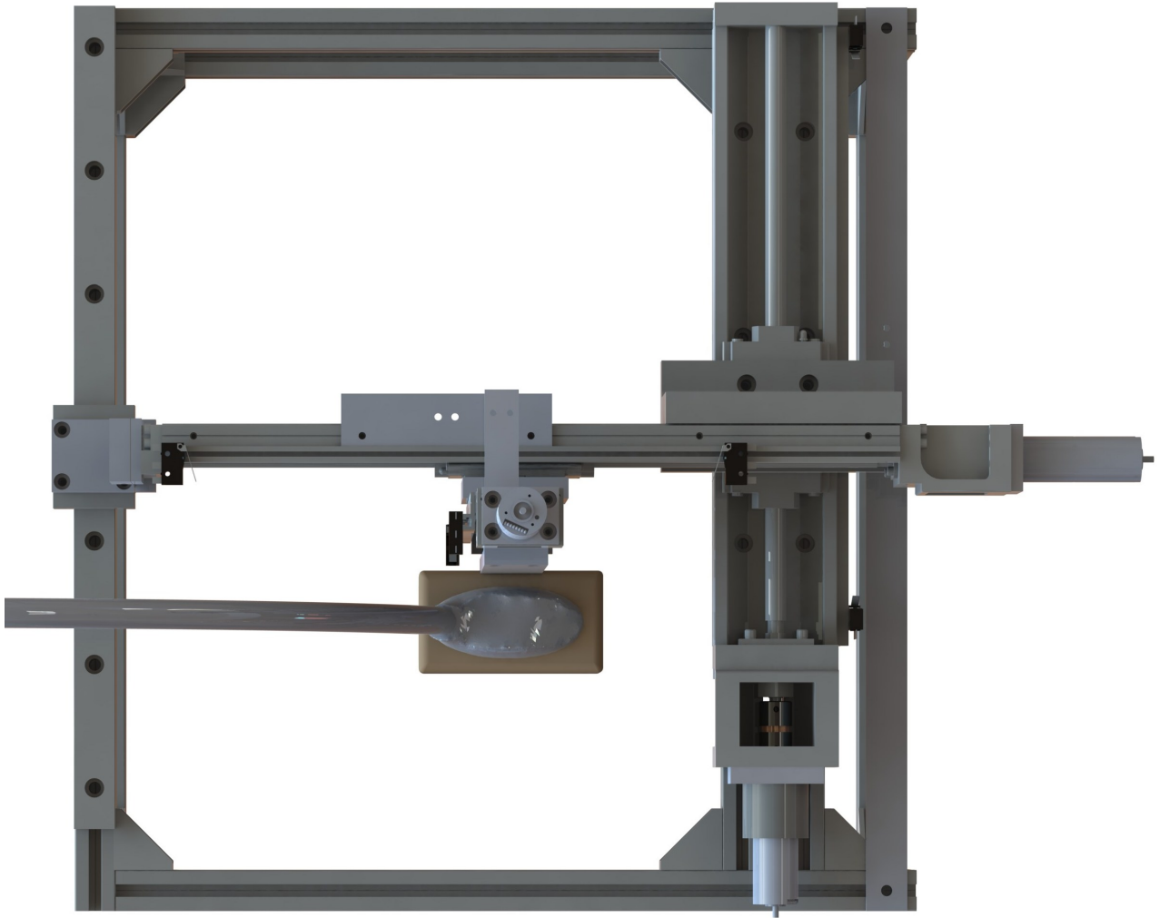
Fig. 3. Solid Works Drawing of the ultrasound positioning device (Top view).
