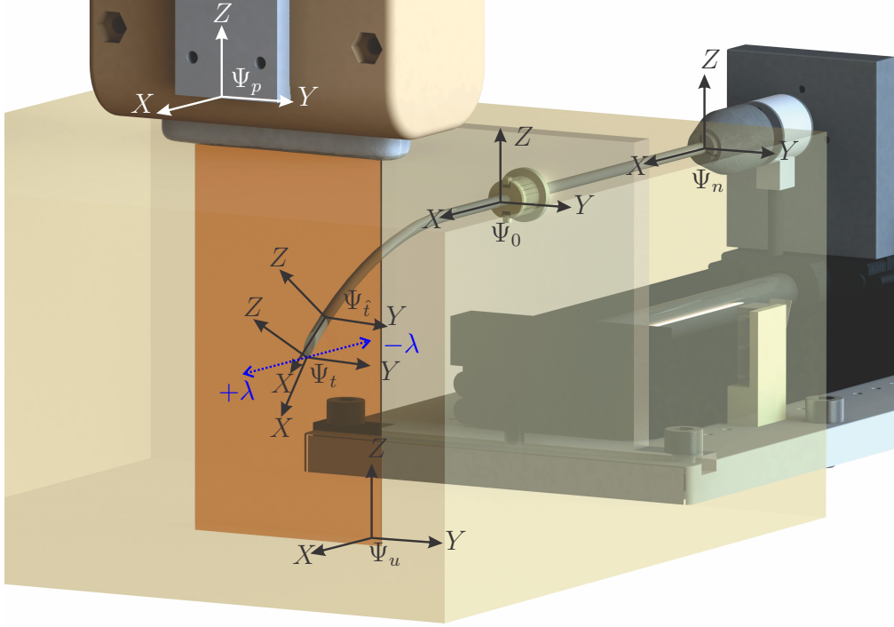
Figure 3: The various coordinate frames used to compute the needle tip pose: Frame ( \Psi_0 ) is used as fixed reference frame located at the needle entry point. Frame ( \Psi_n ) is attached to the needle insertion device end-effector, while frame ( \Psi_p ) is located at the end-effector of the transducer positioning device. Frame ( \Psi_u ) is fixed to the ultrasound image plane. Frame ( \Psi_t ) is located at the needle tip, while frame ( \Psi_i ) is fixed at the computed needle tip location. The ultrasound transducer aberration along the needle insertion axis ( x -axis of frame \Psi_0 ) is denoted by \pm\lambda .
