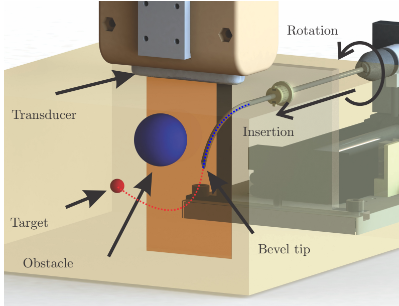
Figure 2: Illustration of needle steering. The needle is steered under ultrasound image-guidance using a needle insertion device. The needle is steered to reach a target while avoiding an obstacle.
