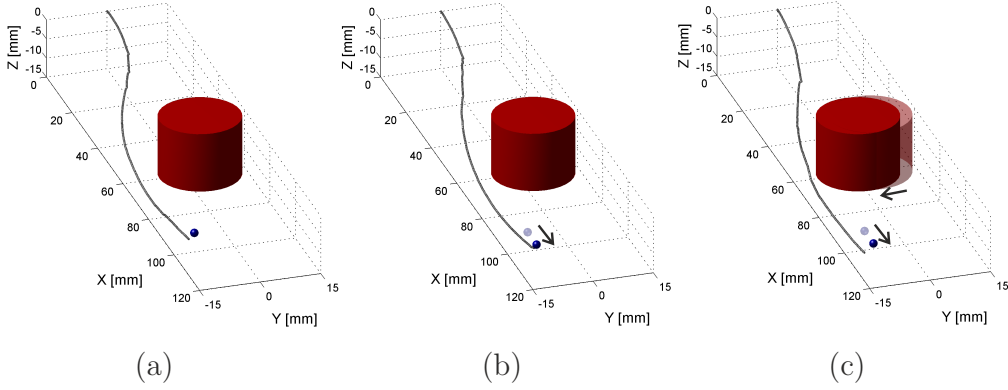
Figure 9: Representative experimental needle steering results and Root Mean Square (RMS) targeting errors: (a) Case I (no obstacle or target motion) - RMS error: 2.78 mm. (b) Case II (only target motion) - RMS error: 1.66 mm. (c) Case III (both obstacle and target motion) - RMS error: 3.45 mm. The initial position of the cylindrical obstacle (blood vessel) is shaded red, while its end position is solid red. The shaded blue sphere represents the initial target location, while the final target locations is represented by a solid blue sphere.
