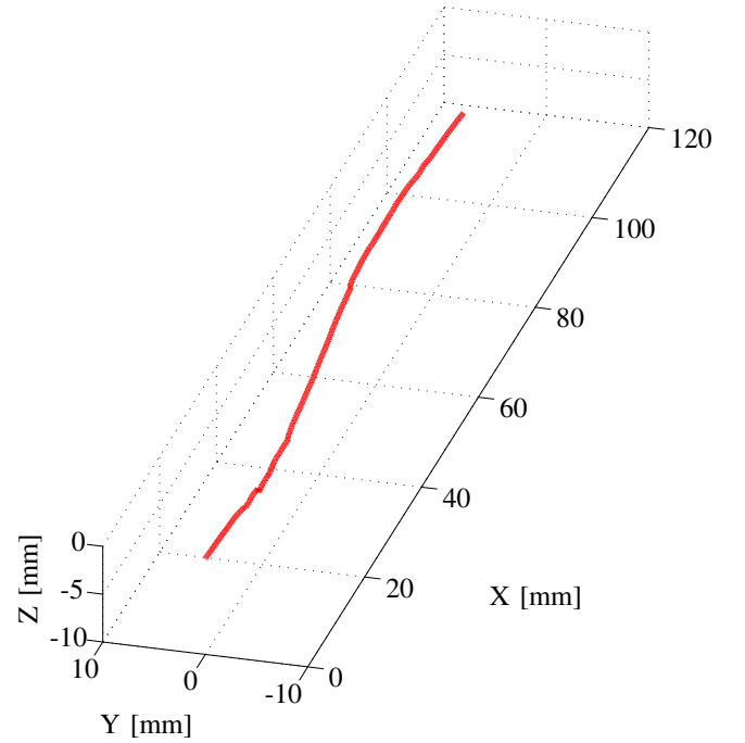
Fig. 1. Three-dimensional needle shape. A bevel-tipped flexible needle is inserted 110 mm and rotated at the same time. During the insertion a full rotation is performed in order to obtain a helical needle shape.
