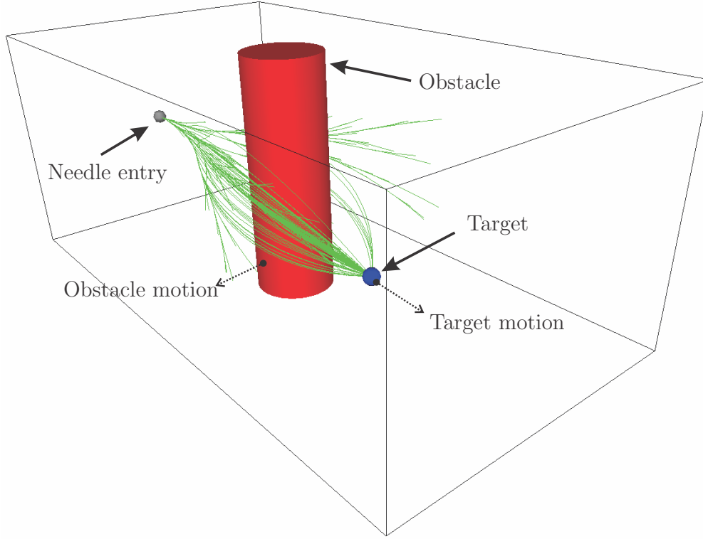
Figure 8: Experimental needle steering scenario: The needle tip pose is tracked using an ultrasound transducer (Fig 7). A cylindrical-shaped obstacle (blood vessel) is placed in the direct path of the needle to reach a spherical target. Needle paths are computed (green lines) using a customized sampling-based rapidly exploring random trees motion planner. The feasible needle paths are selected, and an optimal path is chosen which maximizes the clearance from the obstacle. The needle is steered along the chosen path. During the various experimental cases, the needle path is replanned online in order to compensate for the virtual obstacle and target motion.
