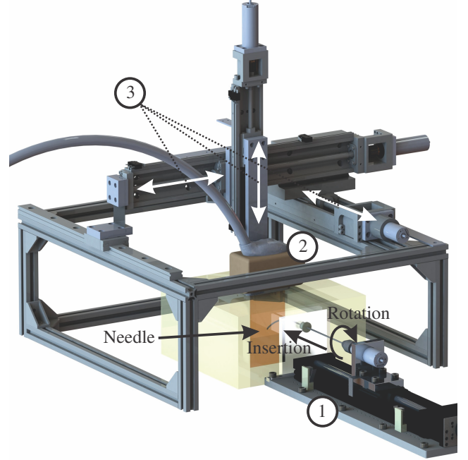
Fig. 1. A flexible needle with a bevel tip is inserted in the soft-tissue simulant by a needle insertion device (NID) ①. Depending on the orientation of the bevel tip, the needle can deflect in the three-dimensional space. An ultrasound transducer ② is used to track the needle tip, which is placed perpendicular to the needle insertion direction. The ultrasound transducer is repositioned by a positioning device along ③ at the needle tip during needle insertion.
