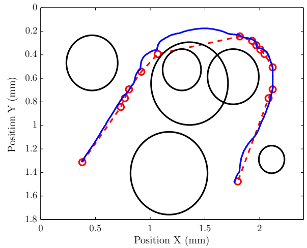
Fig. 16. The top middle obstacle has moved after planning the path (red dashed line). Due to the repulsive forces of the obstacles, the particle is forced out of its path around the obstacle (blue line). The particle starts at the bottom left and moves towards the bottom right in the figure.
