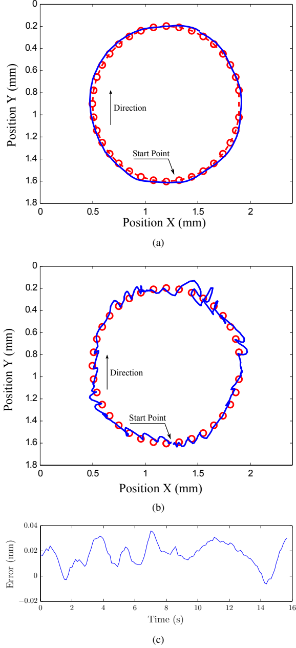
Fig. 11. Particle trajectory tracking a circular path. The red dashed line represents the path defined by the waypoints. The blue line represents the actual path taken by the particle. (a) Is the result for tracking a circular path using the current controller. The average speed achieved was 286 \mu\text{m s}^{-1} . For comparison, (b) shows the result from the previous work. Here the average speed achieved was 83 \mu\text{m s}^{-1} . (c) shows the deviation from the circular path for (a) assuming a perfect circle. A positive error means the particle is outside the circle, a negative error means it is inside.
