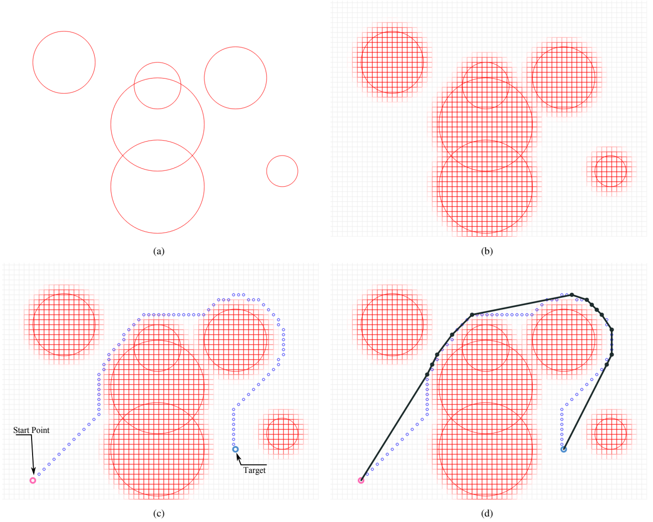
Fig. 7. (a) The obstacles around which a path needs to be planned. (b) S grid is defined and cost map is created. The cost map shows the cost to reach a certain area. The shade of red determines the cost to reach that point on the grid. The darkest red is unreachable space and the faded red is reachable but at an added cost. (c) The A* algorithm determines a low cost path through the grid. Where the thick green circle is the starting position and the thick blue circle is the target position. (d) The smoothing algorithm reduces the previously calculated set of grid points to a smooth path for the particle to follow.
