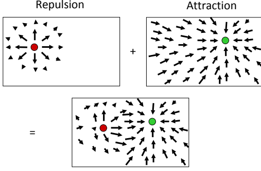
Fig. 5. The idea of potential fields with repulsive and attractive forces. The red circle represents an obstacle and the green circle is the target.
