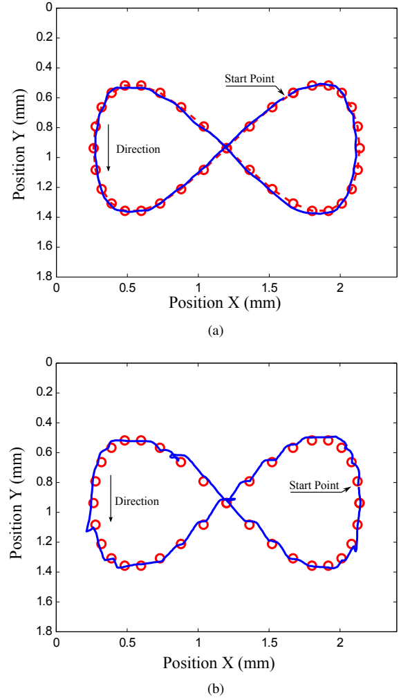
Fig. 12. Particle trajectory tracking a figure-eight path. The red dashed line represents the path defined by the waypoints. The blue line represents the actual path taken by the particle. (a) Shows the result using the current controller the average speed was measured to be 197 \mu\text{m s}^{-1} . (b) Shows the result from the previous work where an average speed of 122 \mu\text{m s}^{-1} was achieved.
