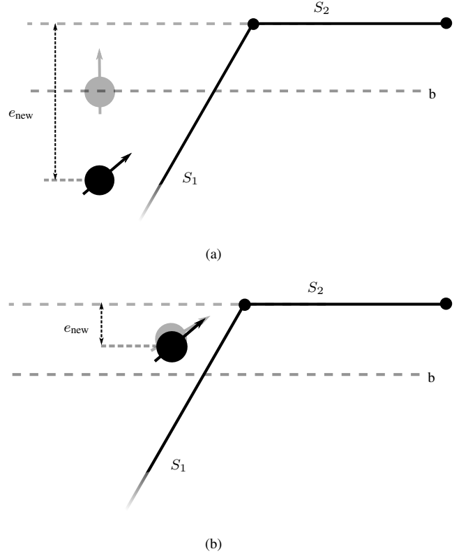
Fig. 3. Smooth waypoint switching. The black circle is the current control angle. The gray circle represents the calculated control angle for the new line segment S_2 . In (b) both control angles match up, and when a switch is made from tracking S_1 to tracking S_2 the transition will be smooth.
