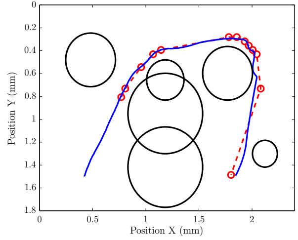
Fig. 15. Result of experiment using static obstacles and path planning. The red dashed line represents the preferred path. The blue line represents the actual path taken by the particle. The particle starts at the bottom left and moves towards the bottom right in the figure.
