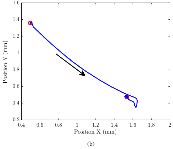
Fig. 9. Tracking performance to a single setpoint: (a) Each axis separately. (b) 2D trajectory of the combined axis. The red lines and circles represent the setpoints given to the controller. The arrow indicates the direction of movement.
