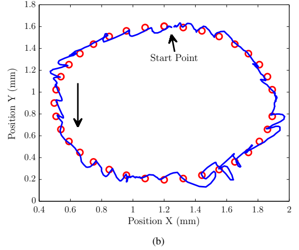
Fig. 10. Tracking performance of a circular path: (a) Each axis separately. (b) 2D trajectory of the combined axis. The red lines and circles represent the setpoints given to the controller. The arrow indicates the direction of movement. The controller gains were K_p = 3 and K_i = 1.8 .
