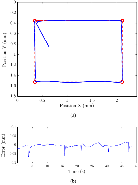
Fig. 10. Particle trajectory tracking a squared path using the improved waypoint switching algorithm. The red dashed line represents the path defined by the setpoints. The blue line represents the actual path taken by the particle. The particle moves in a clockwise direction starting at the top left corner.
