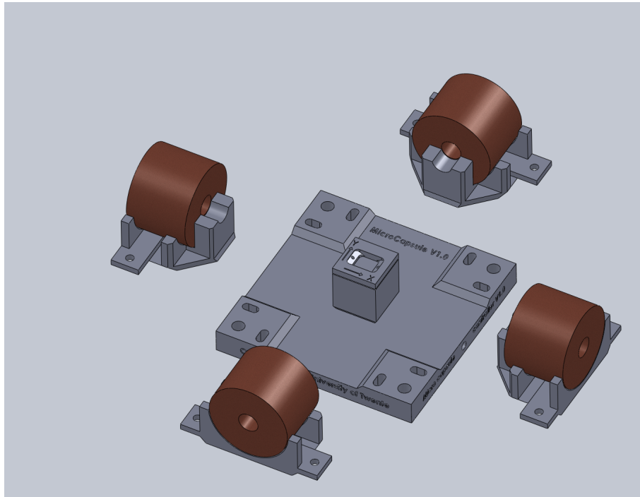
Figure 3: First iteration of the setup. The magnets are fixed in holders and can be placed on the base plate. The relevant dimensions can be found in Part I. All experiments from Part I are done using this setup.
