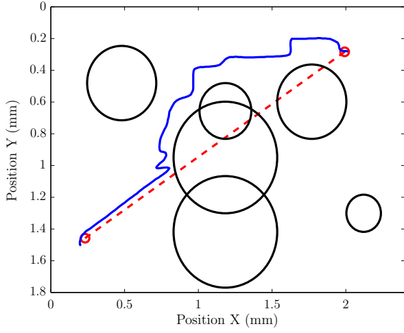
Fig. 13. Experiment using potential field method. The red dashed line represents the shortest path. The blue line represents the actual path taken by the particle. The particle starts at the bottom left and moves towards the top right in the figure.
