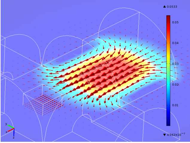
Fig. 4. FEM simulation results for a 1 Ampere current through one coil. Only the planar case for z = 0 is shown. The arrows represent \mathbf{B} and the colored plane represents \|\mathbf{B}\| .
