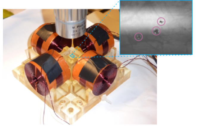
Fig. 8. Picture of the designed and assembled setup. Four coils fixed in a frame around a reservoir for liquids. The microscope objective is positioned above the reservoir. The image captured by the camera shows three particles.
