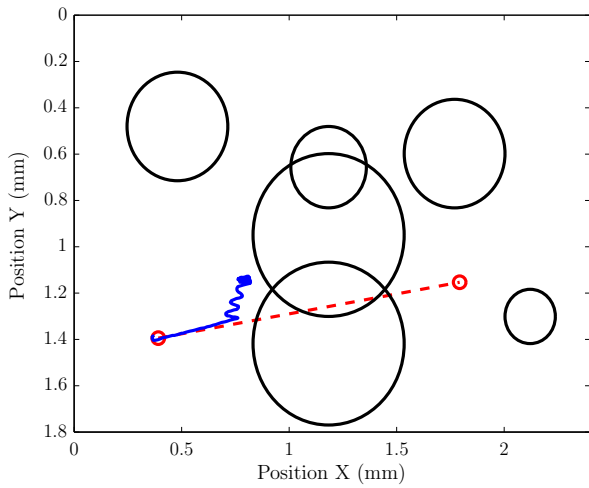
Fig. 14. Experiment demonstrating local minima in the potential field method. The red dashed line represents the preferred path. The blue line represents the actual path taken by the particle. The particle tries to move from the bottom left to the right in the figure.
