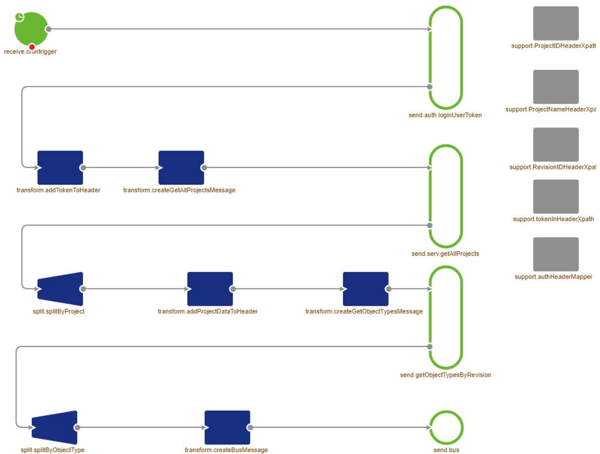
Figure 17. eMagiz entry connector flow for message 'bims-upd' from system bimserv.
