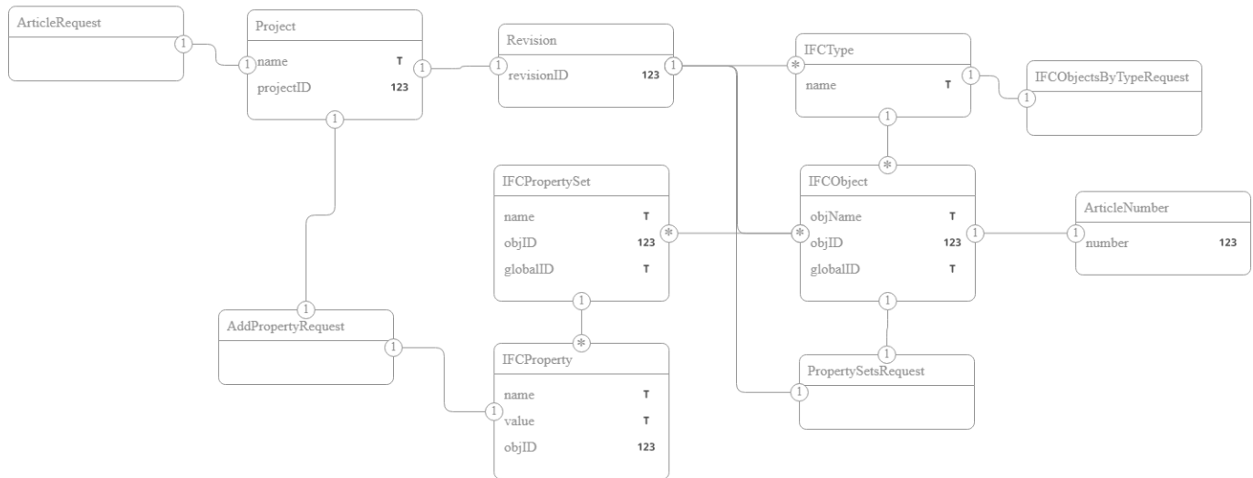
Figure 15. The Common Data Model used in the Prototype
