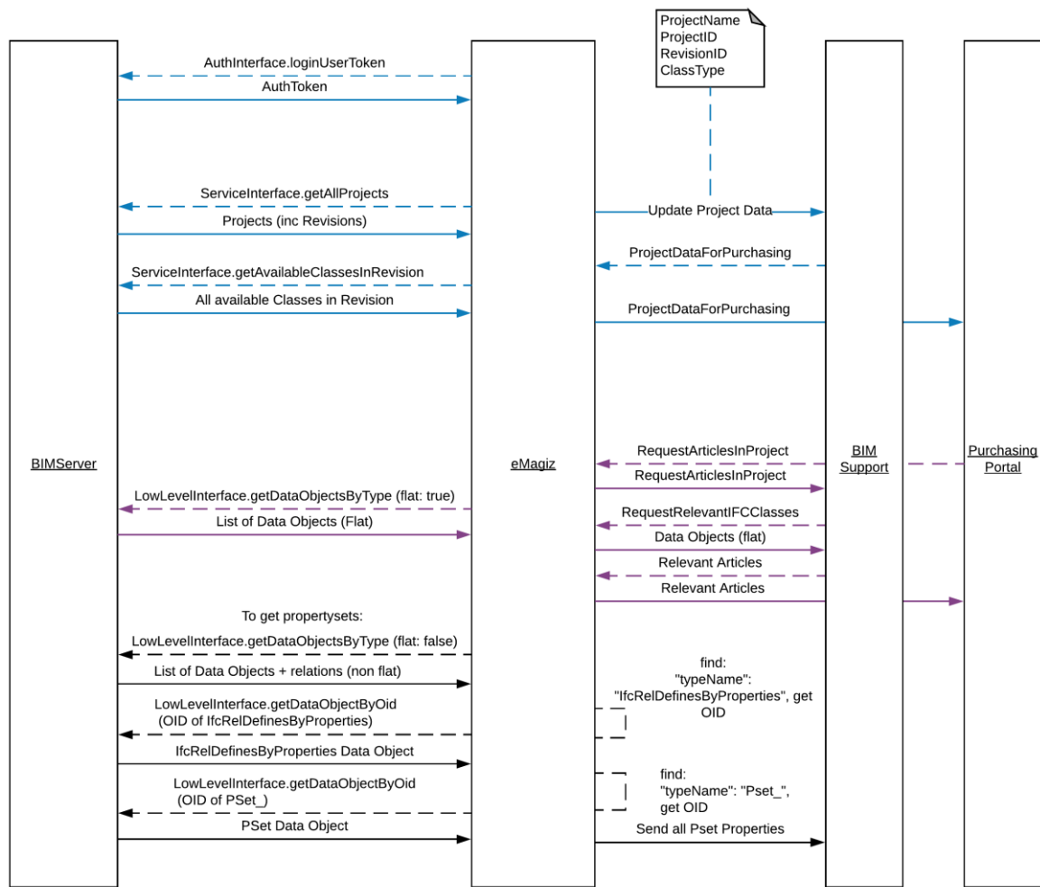
Figure 23. Message flow for retrieving BIM data
