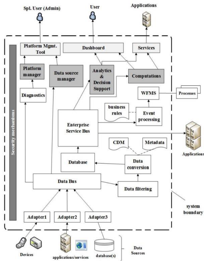
Figure 6. Reference Architecture for Integration Platforms by Singh et al. (P. M. Singh, Van Sinderen, and Wieringa 2017)
