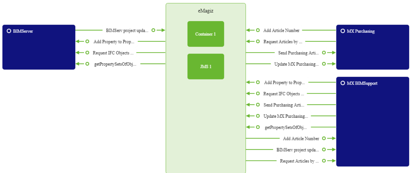
Figure 16. The message flow of the bus component
