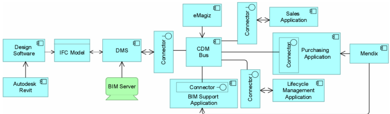
Figure 11. A Reference Architecture for BIM integration
