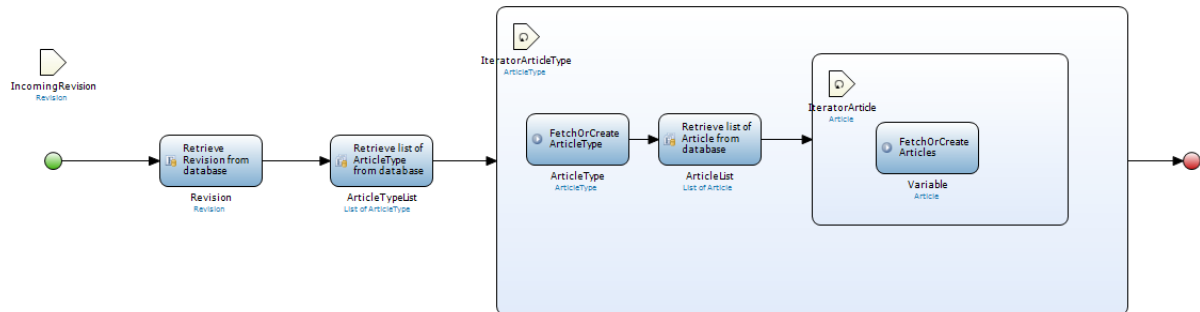
Figure 22. ReceiveArticles Microflow
