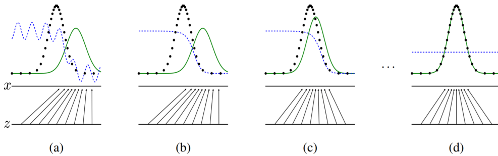
Figure 2.5: Learning process of a GAN. The lower horizontal line represents the domain from which z is sampled. This domain is mapped to the domain of x by x = G(z) and imposes the non-uniform distribution p_g (green solid line). The distribution of the real data p_x is visualised as the black dotted line. The blue dashed line represents the discriminative distribution D . (a) Shows a near convergence scenario with D the partially accurate classifier. (b) With G fixed, D is trained to discriminate generated samples from real samples. (c) Now keeping the updated D fixed, G is trained and has moved to regions that are more likely classified as real data. (d) At this point both G and D cannot be improved anymore, i.e. D_G^* = 0.5 has been reached. This point is only reached if both networks have enough capacity. (Goodfellow et al., 2014)
