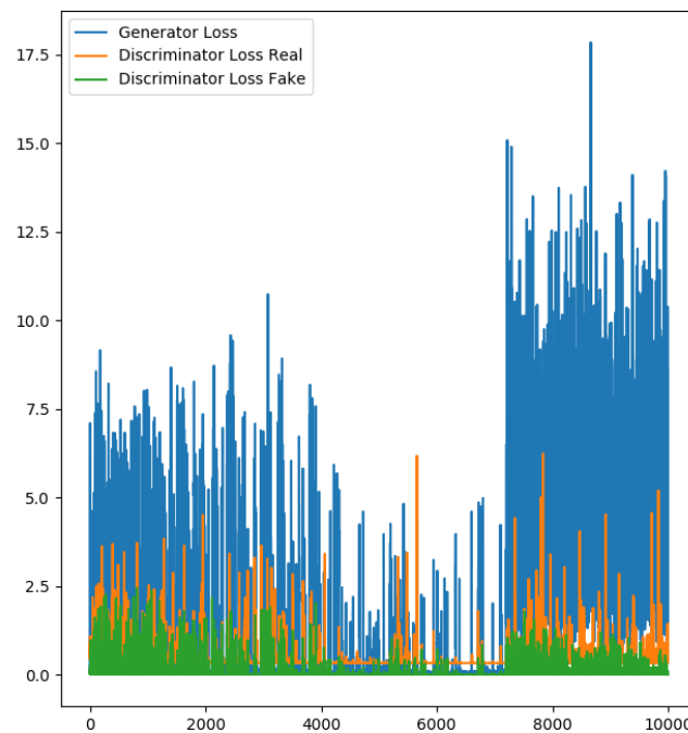
Figure 5.5: Graph of loss of both generator and discriminator. The graph shows the loss of the generator and the discriminator after every epoch. The loss of the discriminator is divided in the loss after updating with a real image batch and after updating with a generated image batch. The y-axis shows the loss and the x-axis shows number of epochs.
