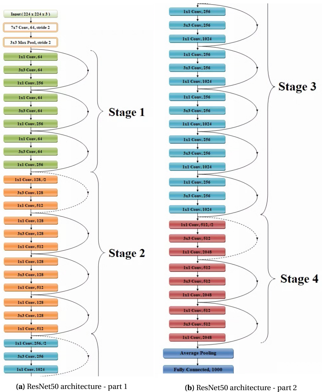
Figure E.2: ResNet50 architecture schematically represented. Picture taken from https://cv-tricks.com/keras/understand-implement-resnets/
