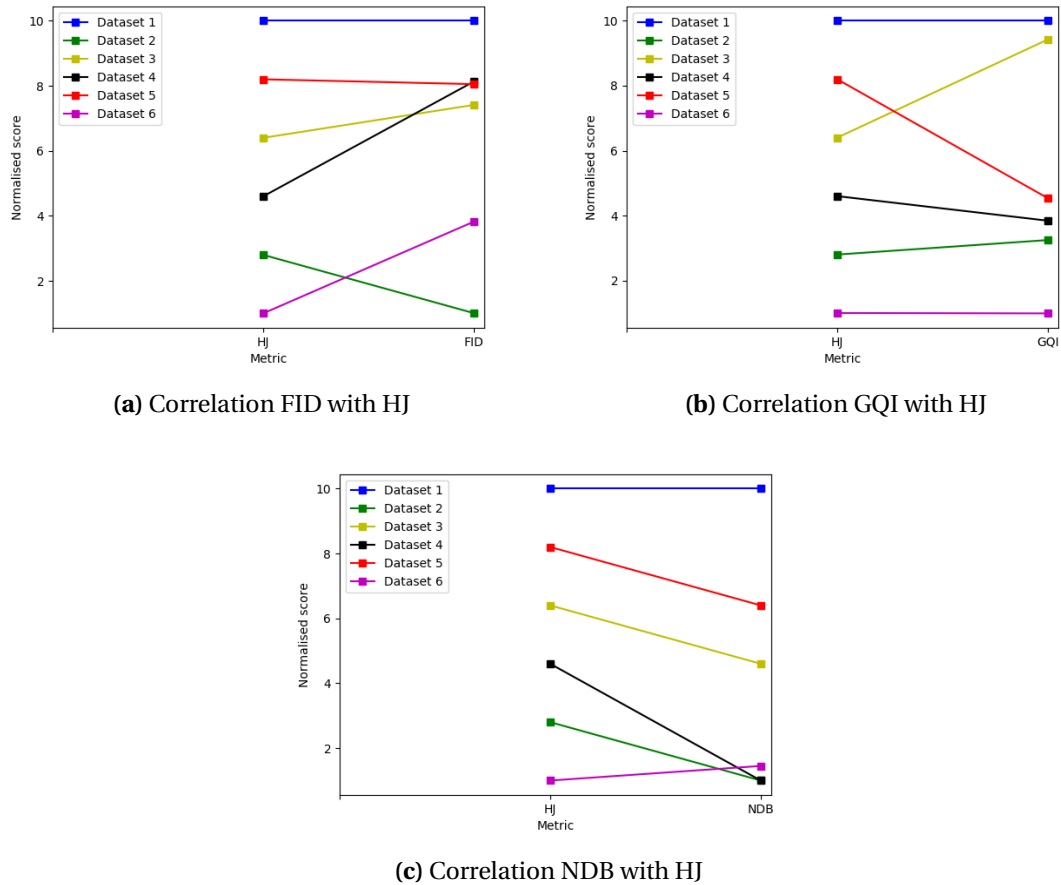
Figure 4.4: Correlation of the three different metrics with human judgement. Subfigure (a) to (c) show graphs of the correlation with metric FID, GQI and NDB respectively. In each of the graphs the y-axis shows the normalised score and the x-axis shows the metric. The different colours represent the different Image data sets.
