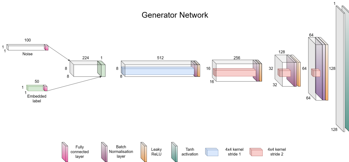
Figure 3.3: Network architecture of the used generator. It takes a noise vector of dimension 100 and an embedded label of dimension 50 as input. The network has five transposed convolutional layers, each followed by a batch normalisation layer and a leaky ReLU, except for the last transposed convolutional layer, which is followed by a hyperbolic tangent (tanh) activation layer. The network outputs an image of 128 \times 128 .
