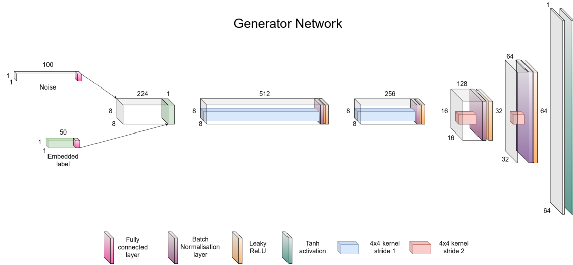
Figure 5.2: Network architecture of the used generator. It takes a noise vector of latent dimension 100 and an embedded label of dimension 50 as input. The network has five transposed convolutional layers, each followed by a batch normalisation layer and a leaky ReLU, except for the last transposed convolutional layer, which is followed by a hyperbolic tangent (tanh) activation layer. The network outputs an image of 64 \times 64 .
