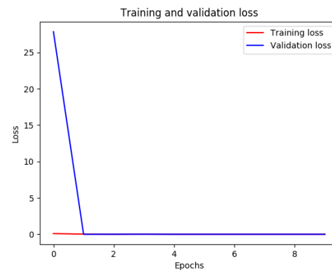
(b) Loss of classifier over 10 epochs
