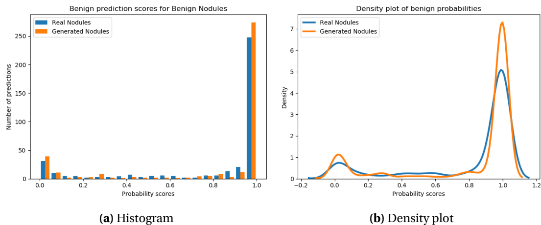
Figure 5.6: Graph showing the benign probability scores assigned to benign test images from both the real nodules test set and the generated nodules test set. Figure 5.6a shows a histogram in which the benign probability scores are plotted. The x-axis represents the probability scores and the y-axis represents the number of predictions. Figure 5.6b shows the density plot of these probability scores. The x-axis shows again the probability scores and the y-axis shows the density.
