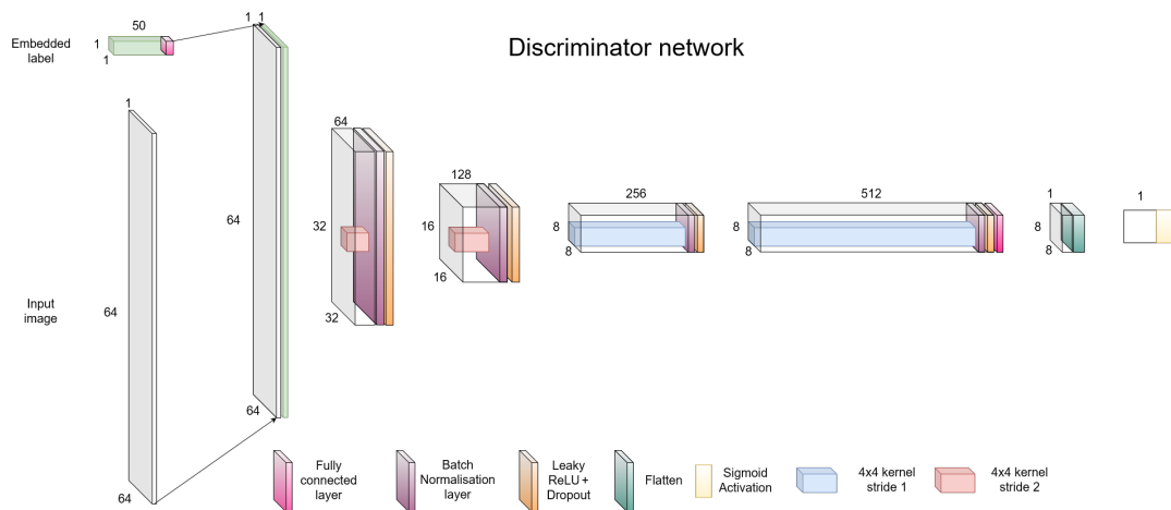
Figure 5.3: Network architecture of the used discriminator. It takes an image of 64 \times 64 , which can either be generated or real, and an embedded label of dimension 50 as input. The network has five convolutional layers, each followed by a batch normalisation layer and a leaky ReLU, except for the last convolutional layer, which is followed by a fully connected layer. Finally a 'sigmoid' activation layer is applied to give a probability as output.
