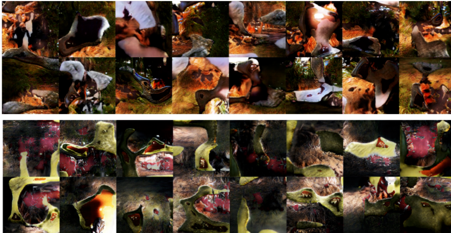
Figure 2.8: Result of what happens if Batch Normalisation is used with small size mini-batches. The upper and the lower set are both a mini-batch produced by a generator. The variation in the mean and standard deviation of feature values in a mini-batch can have an influence that is more dominant than the images individually in that mini-batch. Figure taken from Goodfellow (2016).
