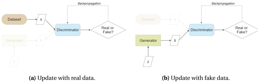
Figure 2.3: Situation when D is trained. To train D it requires one update with real data and one update with the generated data.
