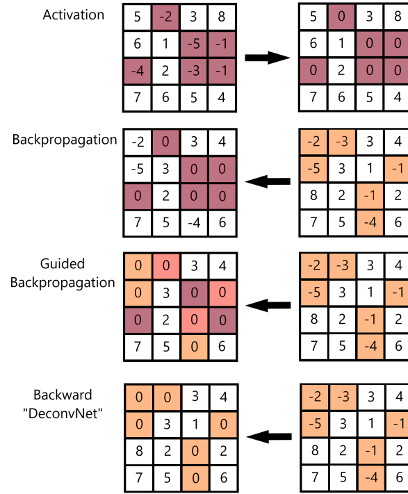
Figure A.1: Activation and different types of backpropagations. From top to bottom respectively, the figure visually shows activation, backpropagation, guided backpropagation and backpropagation using a deconvolution network.
