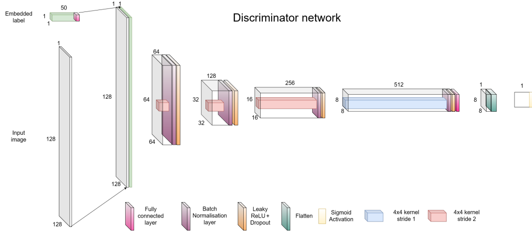
Figure 3.4: Network architecture of the used discriminator. It takes an image of 128 \times 128 , which can either be generated or real, and an embedded label of dimension 50 as input. The network has five convolutional layers, each followed by a batch normalisation layer and a leaky ReLU, except for the last convolutional layer, which is followed by a fully connected layer. Finally a 'sigmoid' activation layer is applied to give a probability as output.
