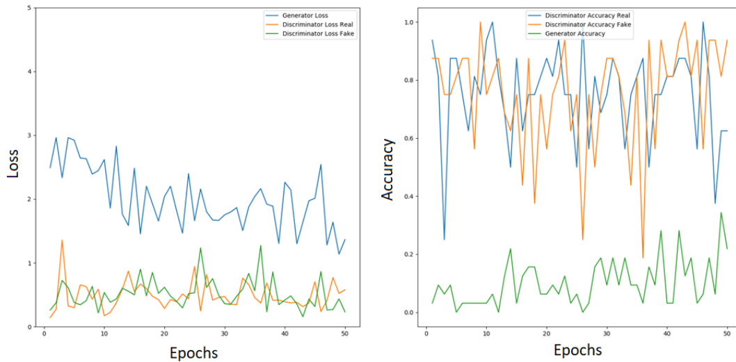
Figure 3.6: Graphs of loss and accuracy of both generator and discriminator. The left graph shows the loss of the generator and the discriminator after every epoch. The loss of the discriminator is divided in the loss after updating with a real image batch and after updating with a generated image batch. The y-axis shows the loss and the x-axis shows number of epochs. The right graph shows the accuracy of the generator and the discriminator after every epoch. In this case also, the accuracy of the discriminator is divided in the accuracy after updating with a real image batch and after updating with a generated image batch. The y-axis shows the accuracy and the x-axis shows the number of epochs.
