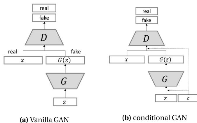
Figure 2.6: Two different GAN architectures. The vanilla GAN can is schematically represented on the left and the cGAN on the right. (Mino and Spanakis, 2018)
