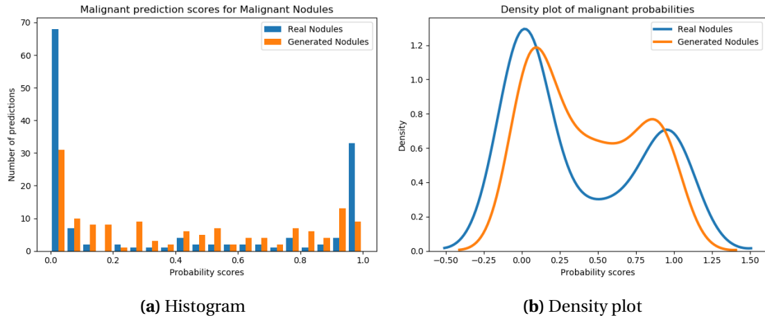
Figure 5.7: Graph showing the malignant probability scores assigned to malignant test images from both the real nodules test set and the generated nodules test set. Figure 5.7a shows a histogram in which the malignant probability scores are plotted. The x-axis represents the probability scores and the y-axis represents the number of predictions. Figure 5.7b shows the density plot of these probability scores. The x-axis shows again the probability scores and the y-axis shows the density.
