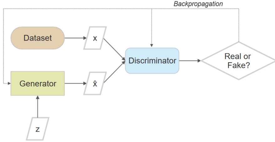
Figure 2.2: Schematic of the basic concept of GANs. The generator takes as input a noise vector ( z ) and has as an output a generated image ( \hat{x} ). The discriminator takes this generated images as input, but also has images from the real dataset as input ( x ). The discriminator has to decide if the image it receives is either a real image or a fake/generated image. Through backpropagation both the discriminator and the generator improve.
