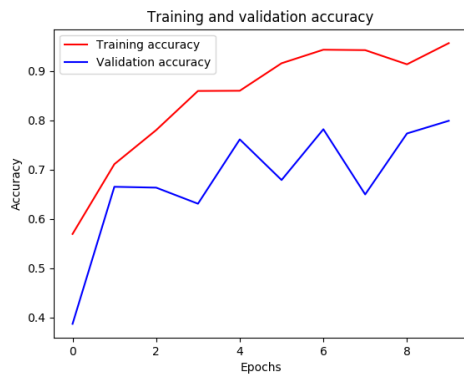
(a) Accuracy of classifier over 10 epochs
