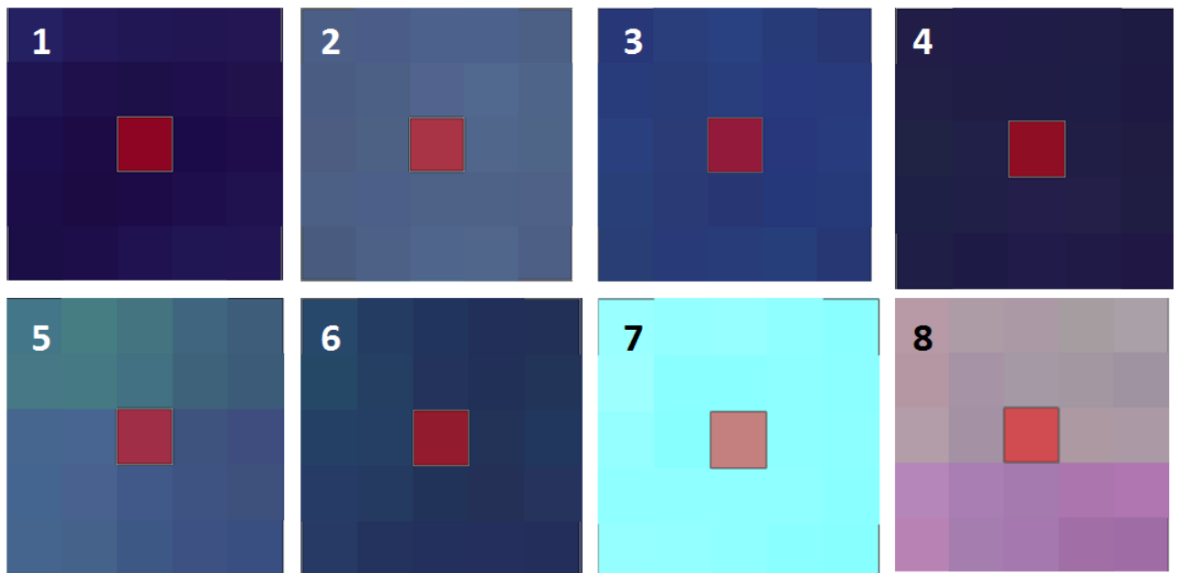
Fig. 43 Eight spectral endmember were collected from EO-1 Hyperion of Krafla area : (1) Cauliflower AA; (2) Old lava; (3) Pahoehe; (4) Rubbly AA; (5) Sandur deposit; (6) Shelly Pahoehe; (7) Upper Pleistocene formation; and (8) Vegetation.
