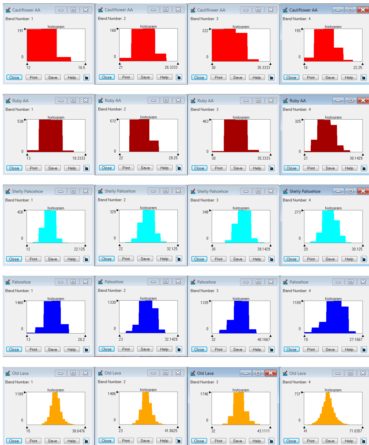
Fig. 50 Pixel histogram distribution of lava morphology in Krafla; (1) Cauliflower AA; (2) Rubbly AA; (3) Shelly pahoehoe; (4) Pahoehoe; and (5) Old lava.
