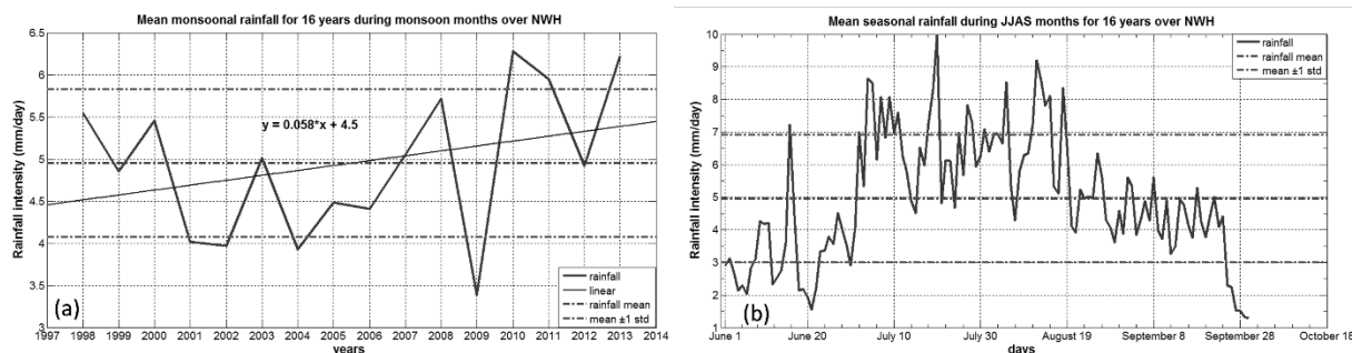
Figure j: Mean seasonal rainfall plots for monsoon season from 1998-2013 over NWH (a) Inter-annual plot (b) seasonal plot
