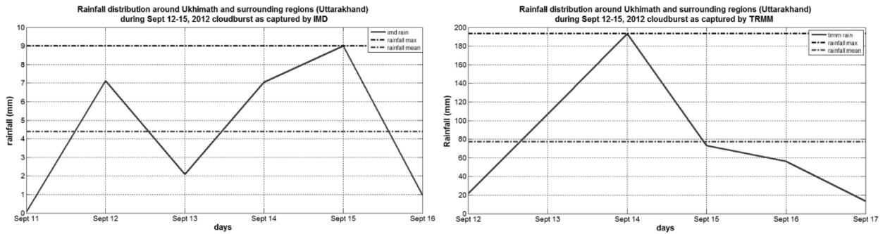
Figure e: Rainfall distribution around Ukhimath and nearby regions during cloudburst event on Sept 12-15, 2012 as captured by (a) IMD data (b) TRMM data
