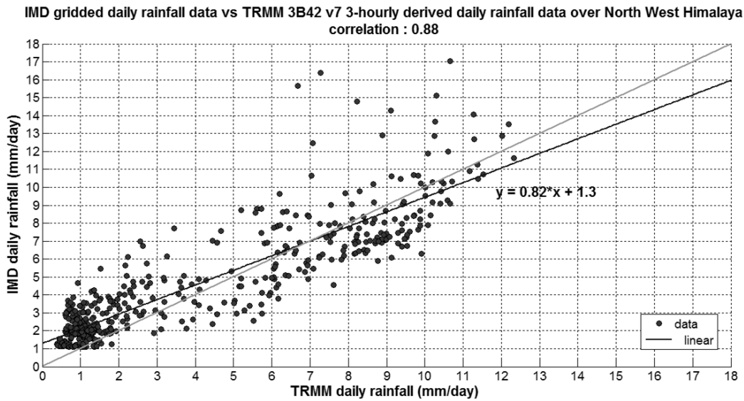
Figure 5.1: Correlation between IMD derived average daily rainfall data (represented on y-axis) and TRMM derived average daily rainfall (shown on x-axis) data for each pixel in NWH region. The light colored line is 1:1 line. The dark color line shows the linear fitting of the data.
