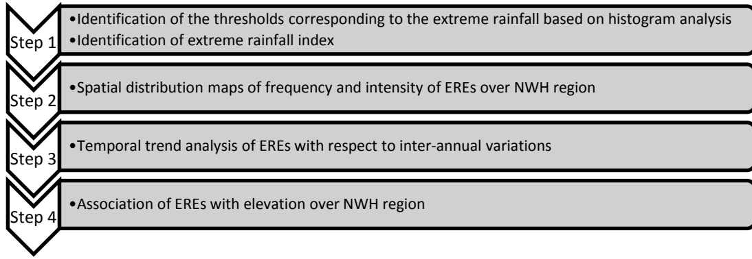
Figure 4.2: Steps for the analysis of EREs
