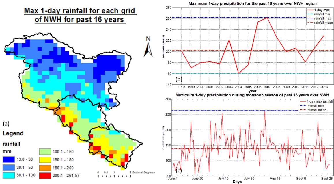
Figure 5.6: Maximum 1-day precipitation event (a) spatial distribution for each grid of NWH (b) year-wise plot for the past 16 years i.e. 1998-2013 (c) day-wise plot during monsoon season of past 16 years
