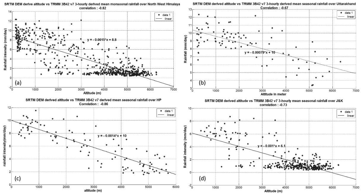
Figure k: Correlation analysis between SRTM DEM derived elevation and TRMM 3B42 v7 derived mean seasonal rainfall over (a) Northwest Himalaya region (b) Uttarakhand region (c) Himachal Pradesh region (d) Jammu & Kashmir region
