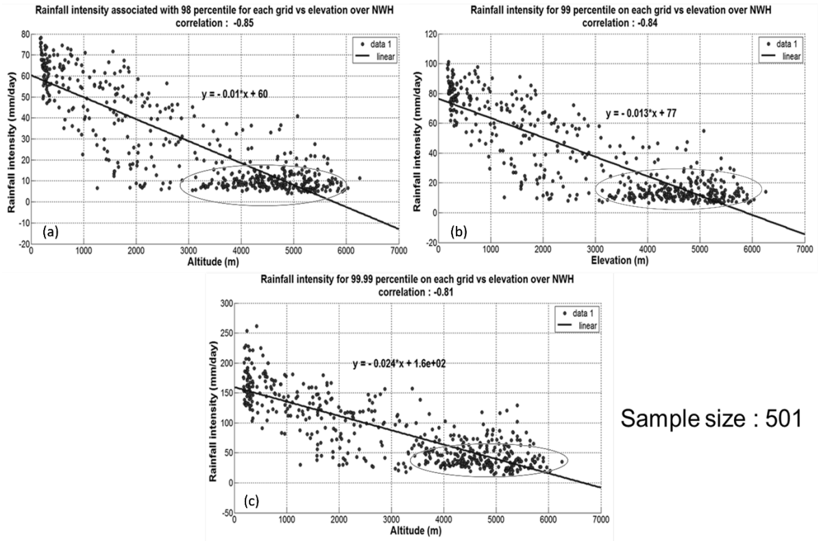
Figure 5.12: Correlation analysis between elevation and rainfall intensities associated with (a) 98 th percentile (b) 99 th percentile (c) 99.99 th percentile for each pixel of NWH region for the period 1998 – 2013
