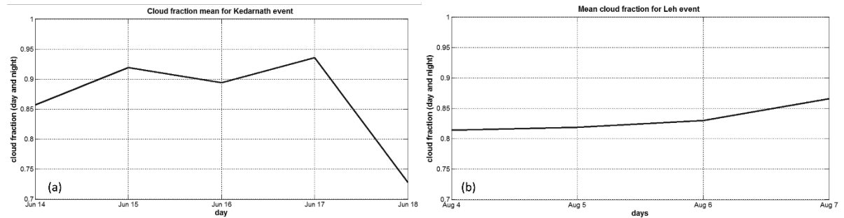
Figure 5.20: cloud fraction profile for (a) Kedarnath event (left panel) (b) Leh event (right panel)
