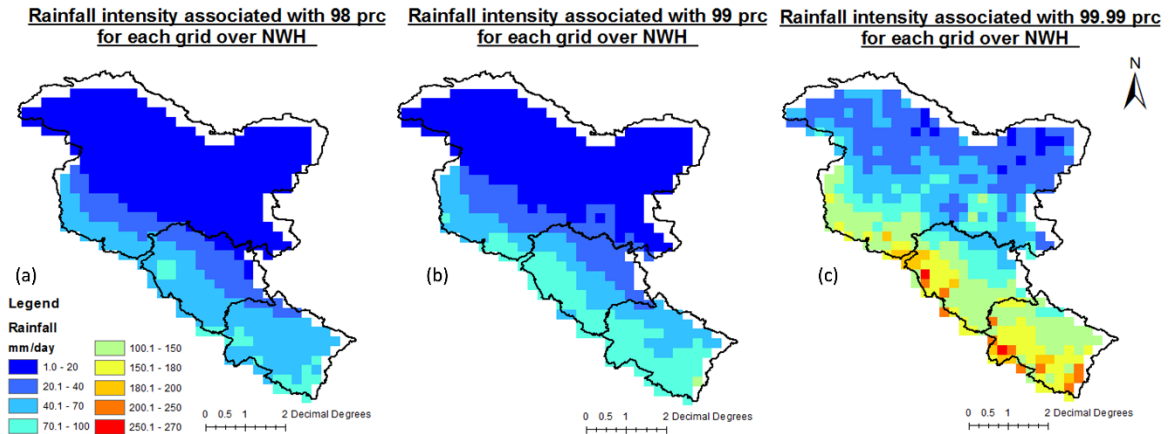
Figure 5.8: Rainfall intensities for each pixel/grid of NWH for (a) 98 th percentile (b) 99 th percentile (c) 99.99 th percentiles during monsoon season of the period 1998 – 2013
