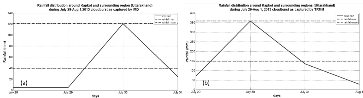
Figure 5.2: Rainfall distribution around Kapkot and nearby regions during cloudburst event on July 29-August 1, 2013 as captured by (a) IMD data (b) TRMM data
