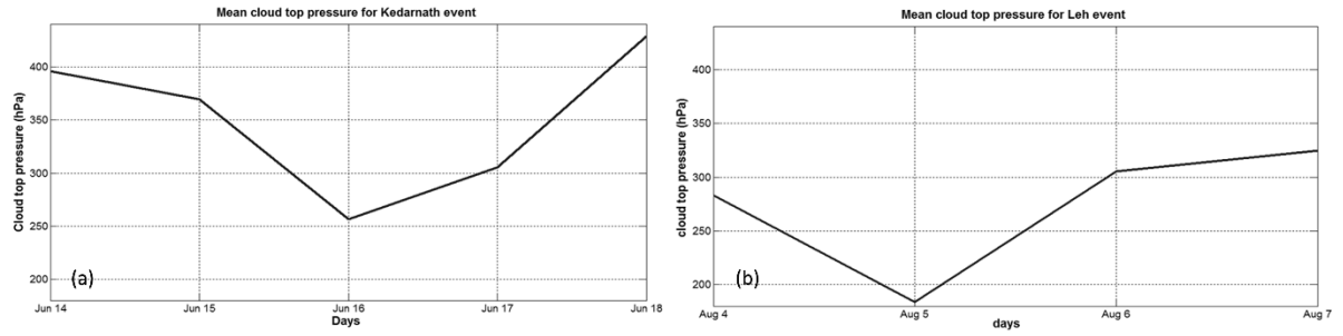
Figure 5.19: cloud top pressure profile for (a) Kedarnath event (left panel) (b) Leh event (right panel)
