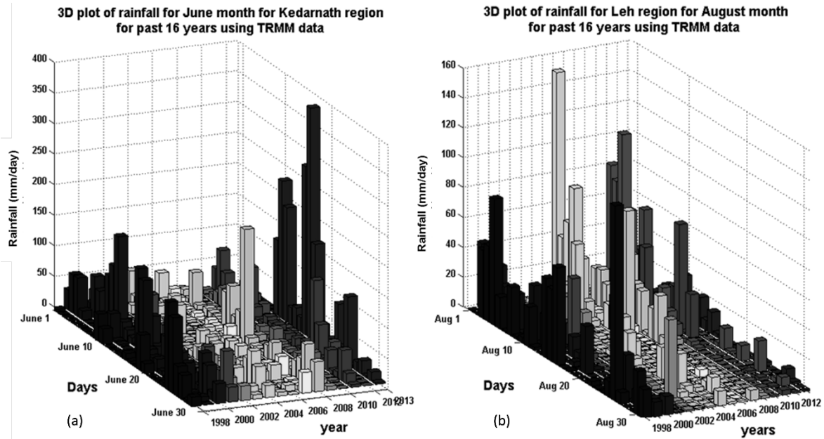
Figure 5.15: 3D rainfall plots for (a) Kedarnath region for June month of past 16 years (b) Leh region for August month of past 16 years respectively; x-axis represents the year, y-axis represents the number of days (June for Kedarnath and August for Leh) and z-axis for rainfall amount
