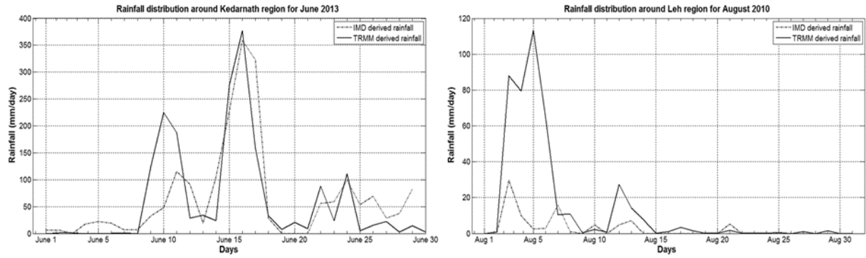
Figure 5.14: Rainfall distribution using TRMM and IMD data for (a) Kedarnath region for the month of June, 2013 (b) Leh region for the month of August 2010
