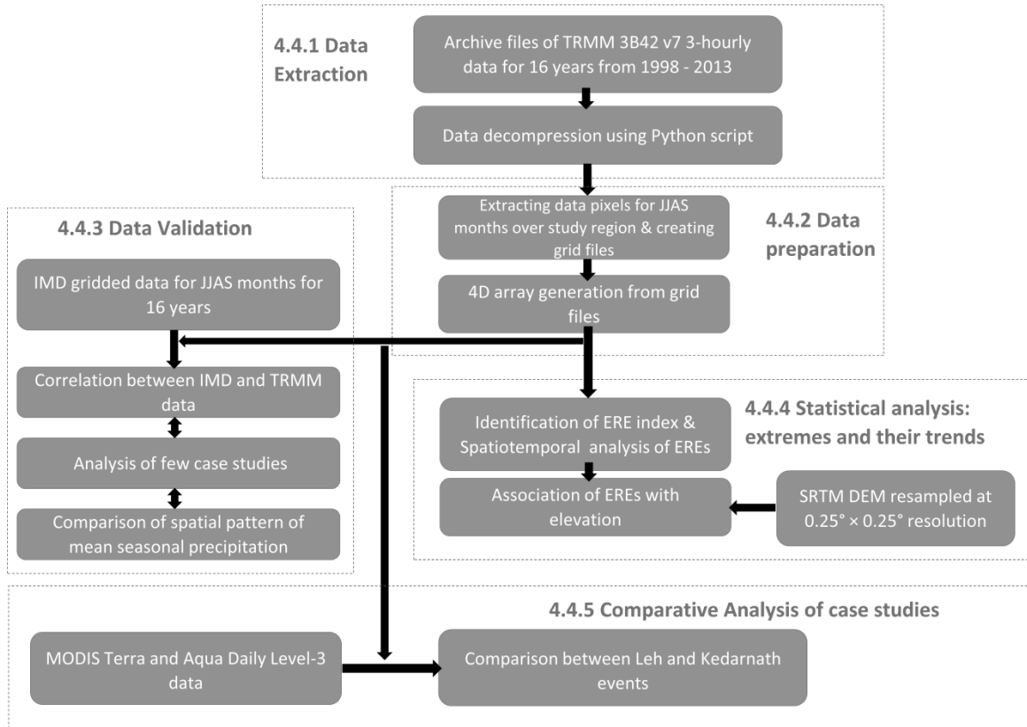
Figure 4.1: Research methodology adopted for this study. The number represents the section where the steps are described in detail.
