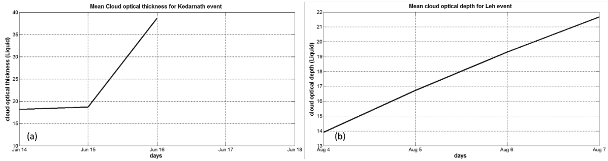
Figure 5.21: Cloud optical depth during (a) Kedarnath event (left panel) (b) Leh event (right panel)
