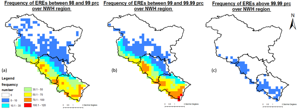
Figure 5.7: Spatial distribution of frequency of EREs over NWH for (a) frequency of EREs with intensity \geq 98^{\text{th}} & < 99^{\text{th}} percentile (b) same as (a) but for \geq 99^{\text{th}} & < 99.99^{\text{th}} percentile (c) same as (a) but for \geq 99.99^{\text{th}} percentile
