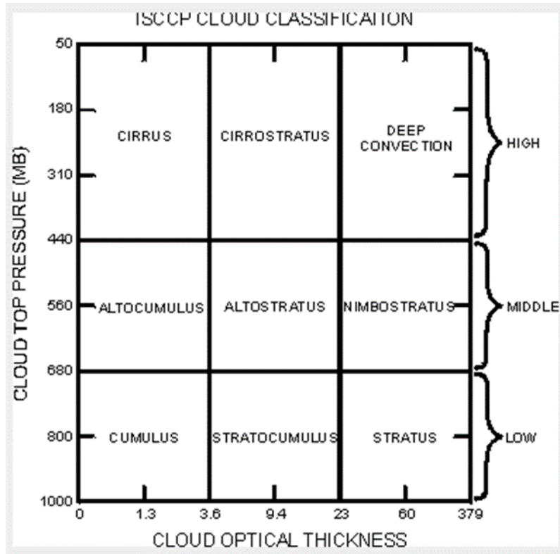
Figure m: ISCCP cloud classification scheme
