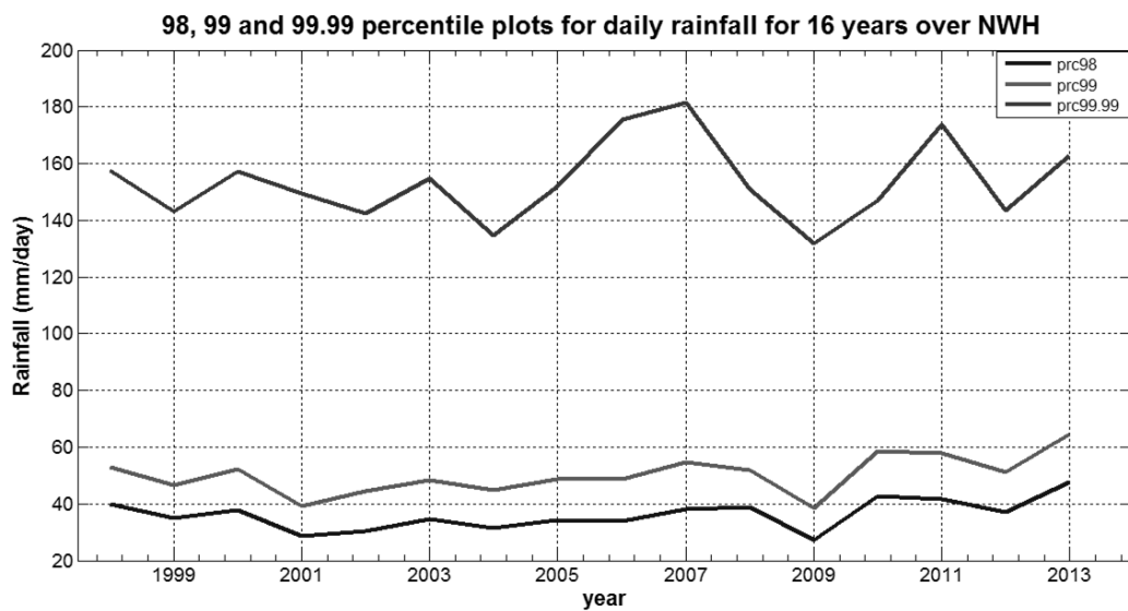
Figure i: 98 th , 99 th and 99.99 th percentile plots for monsoon season NWH using 16 years of TRMM data
