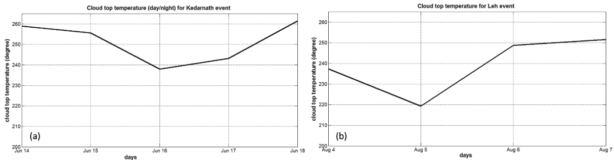
Figure 5.18: cloud top temperature profile for (a) Kedarnath event (b) Leh event
