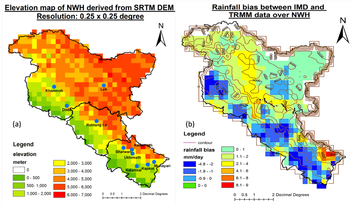
Figure 5.4: (a) Elevation map of NWH generated using resampled SRTM DEM (b) Rainfall bias map generated for NWH region with contours depicting elevation ranges in meter (0 contour line is present on the borders due to absence of raster data outside NWH region)
