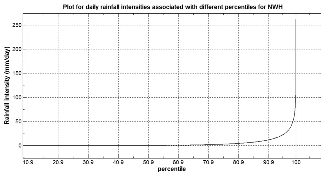
Figure h: Plot depicting rainfall intensity associated with different percentiles over NWH using 16 years of TRMM data
