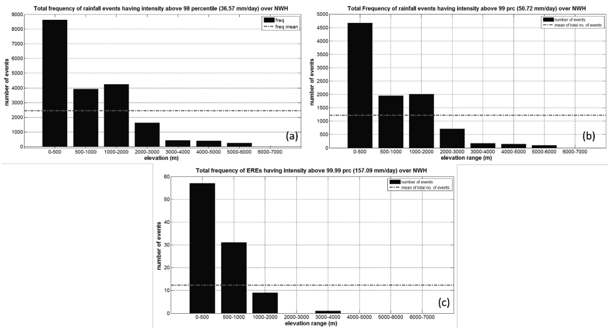
Figure 5.13: Plots depicting frequency of EREs for different elevation ranges over NWH region for (a) 98 th percentile (b) 99 th percentile (c) 99.99 th percentile for the period 1998-2013
