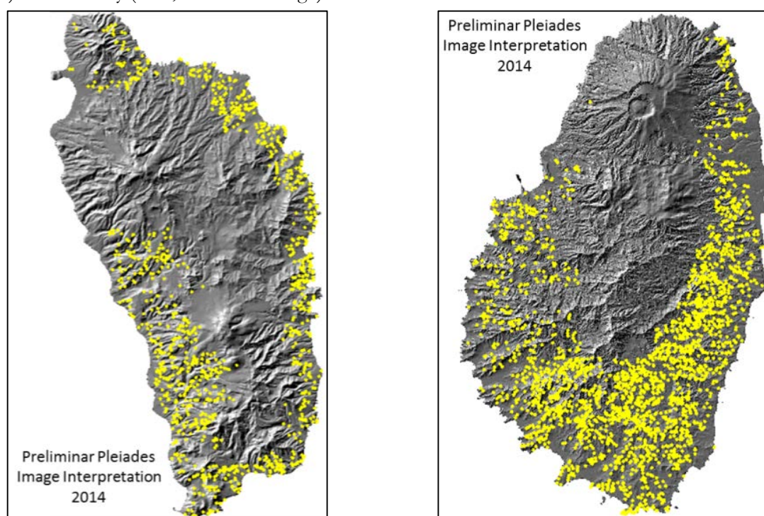
Figure 11. Preliminary landslide inventories based on image interpretation of very high resolution Pleiades images from 2014
