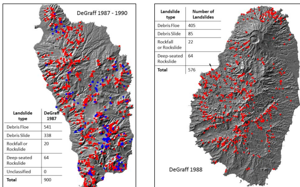
Figure 10. DeGraff landslide inventories for both islands. For Dominica the blue points represent 1990 Landslide Inventory.
