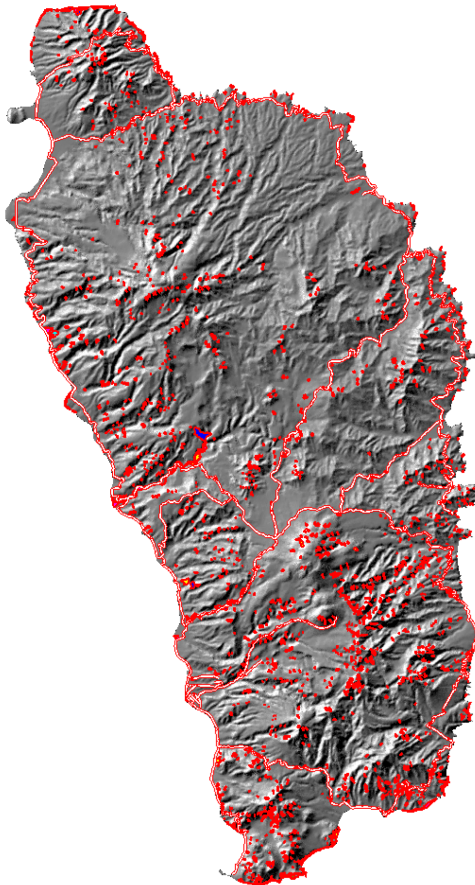
Figure 23. Final Polygon based landslide inventory for Dominica.
