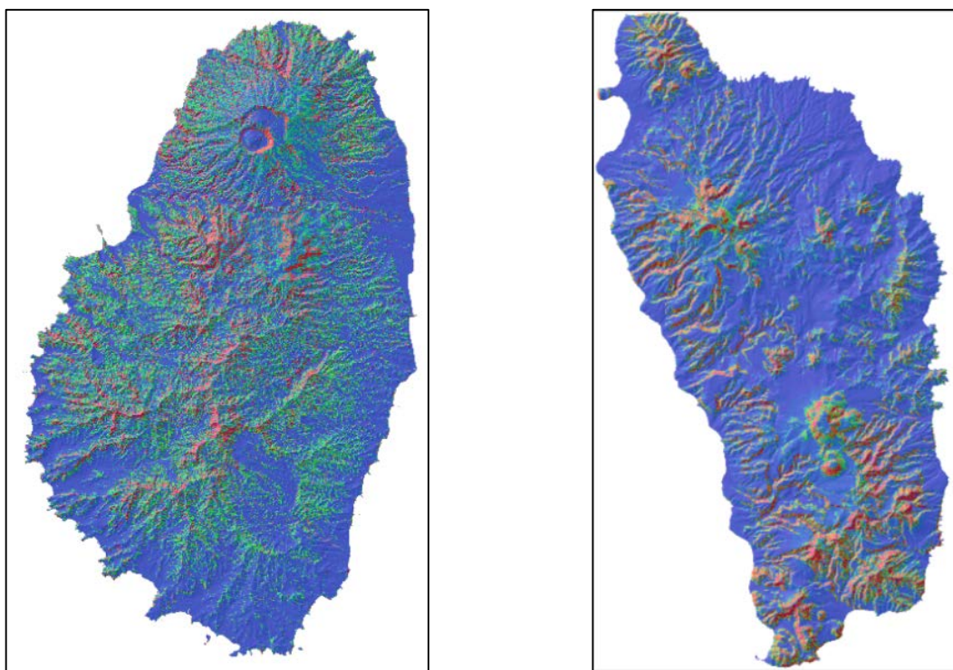
Figure 40. Maps generated with new standardization method. Saint Vincent on the left and Dominica on the Right.
