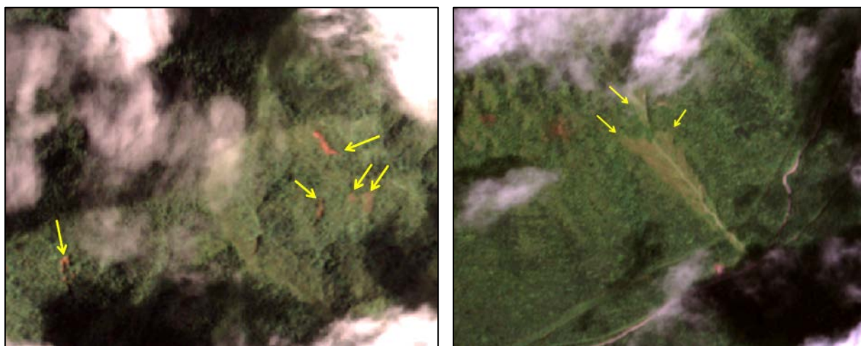
Figure 12. Examples of Landslide image interpretation. A. Active debris flows in Saint Vincent (left) and B. Recent one in Dominica (Right) near Fresh Lake.
