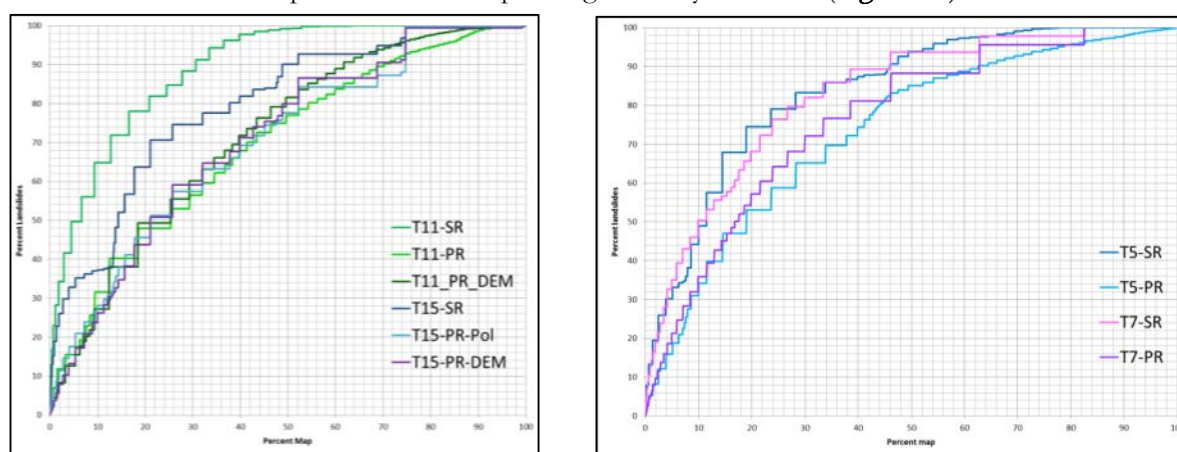
Figure 41. Success and Prediction rate for the initial and final models with standardization method Benefit-Goal, as well as for DEM derivatives for Saint Vincent (left) and Dominica (right).
