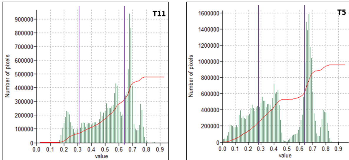
Figure 44. Histograms used to classify the final landslide susceptibility maps of Saint Vincent (left) and Dominica (right), the limits of the classes are shown as purple vertical lines.
