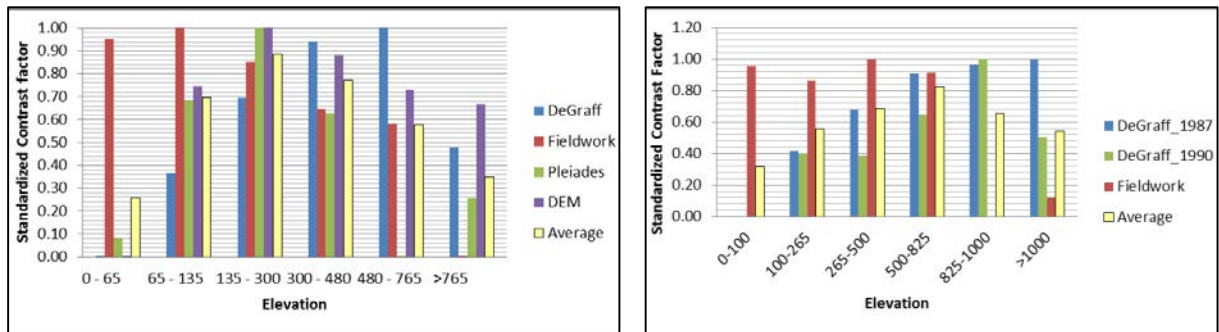
Figure 30. Bar graph showing the contrast factor of each elevation class for Saint Vincent (left) and Dominica (right)
