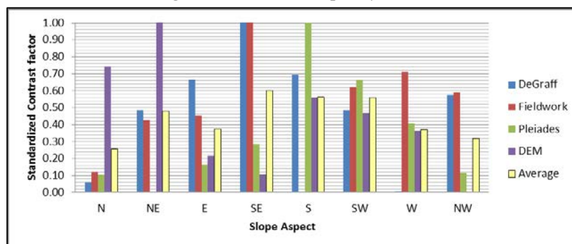
Figure 34. Bar graph showing the contrast factor of each Aspect class for Saint Vincent (left)
