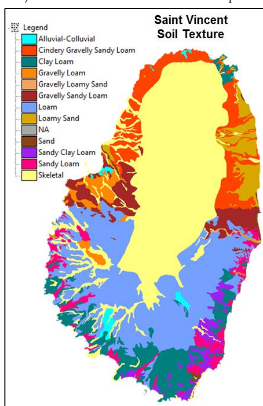
Figure 26. Soil Texture map of Saint Vincent
