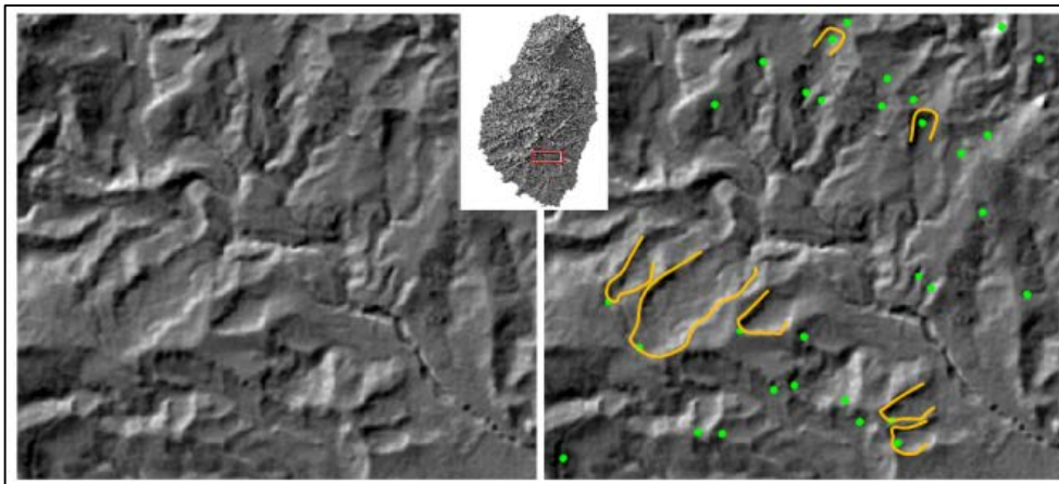
Figure 16. Example of Landslide interpretation on the DEM Left raw image, on the right it is indicated some of the landslide points in green with some of the crowns in orange.
