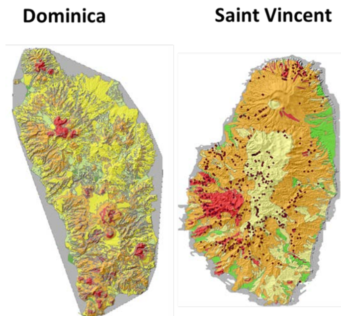
Figure 1. Dominica: study carried out by CIPA for USAID in 2006, as part of a multi-hazard mapping project. Saint Vincent: Susceptibility map generated by DeGraff in 1988.
