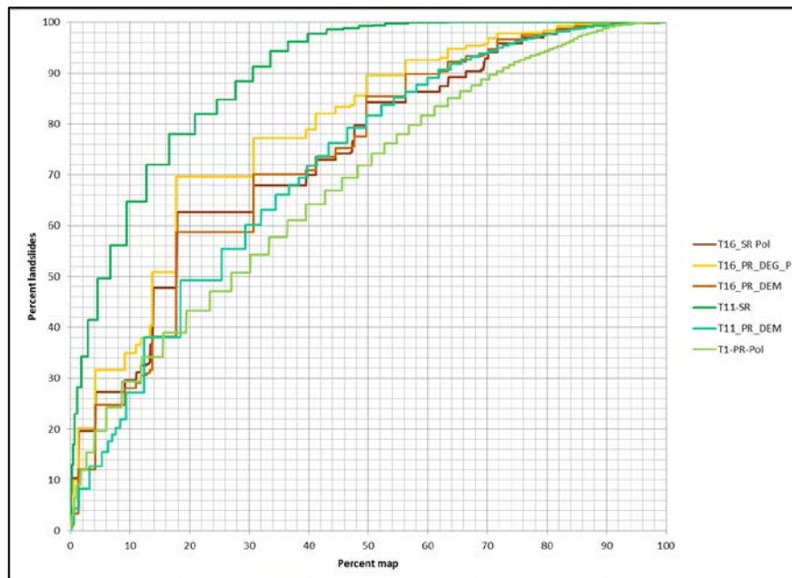
Figure 43. Prediction and success rates of different spatial representation of the landslide inventories for Saint Vincent.
