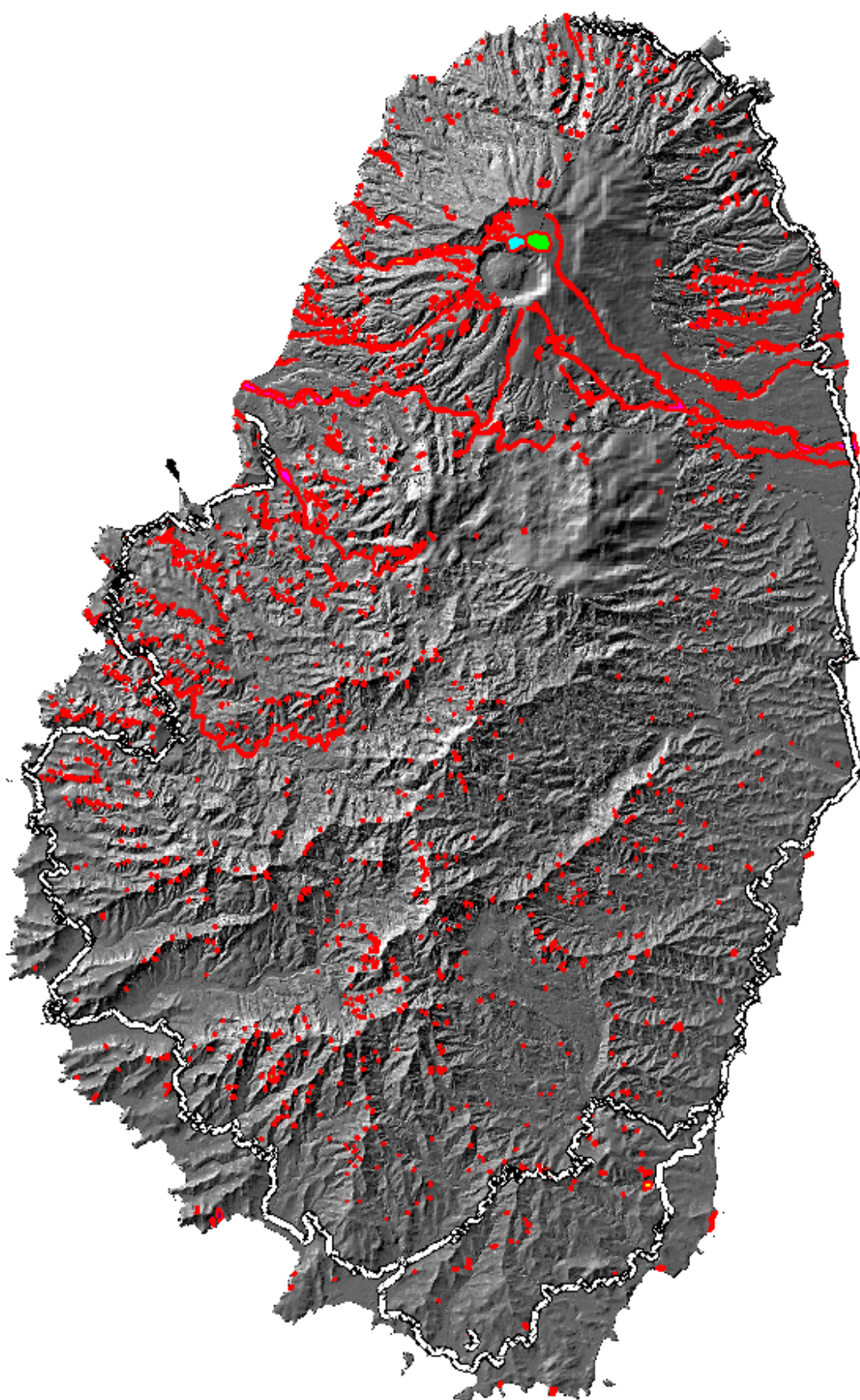
Figure 24. Final Polygon based landslide inventory for Saint Vincent.
