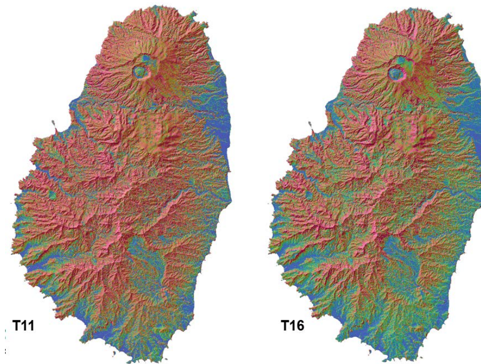
Figure 42. Comparison of maps using point based inventory to model (left) and polygon based inventory to model (right).
