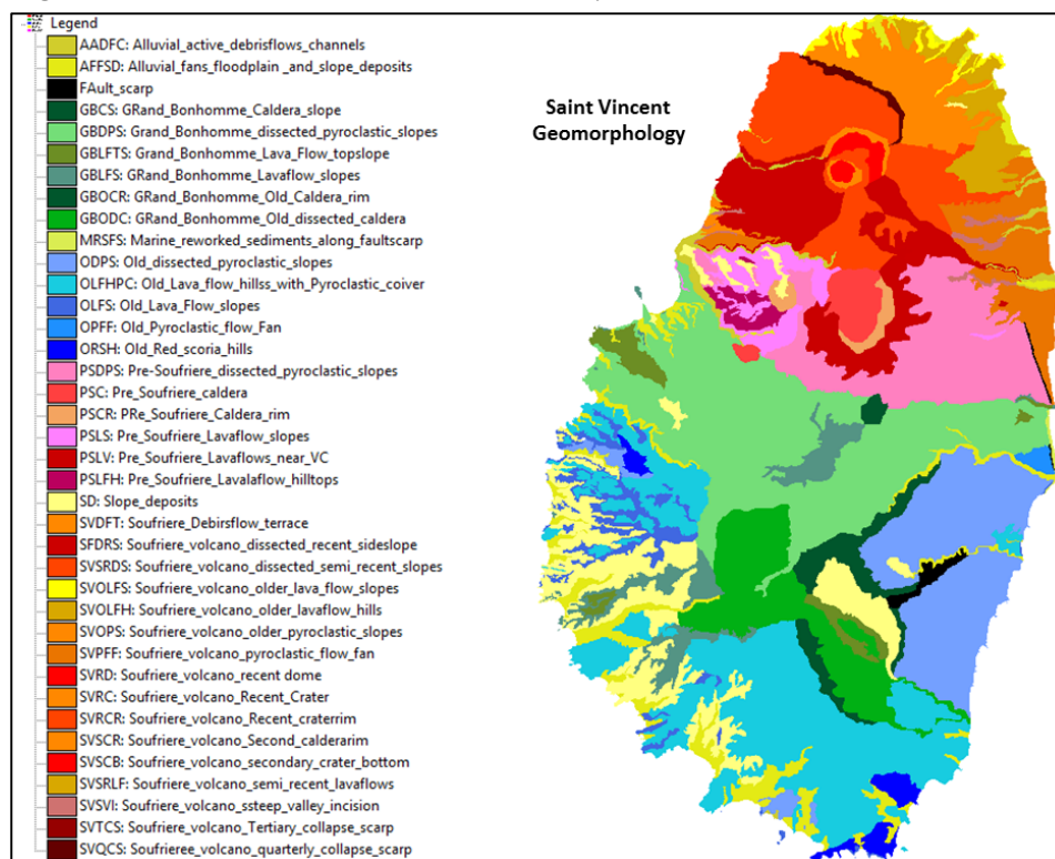
Figure 27. Geomorphological map of Saint Vincent
