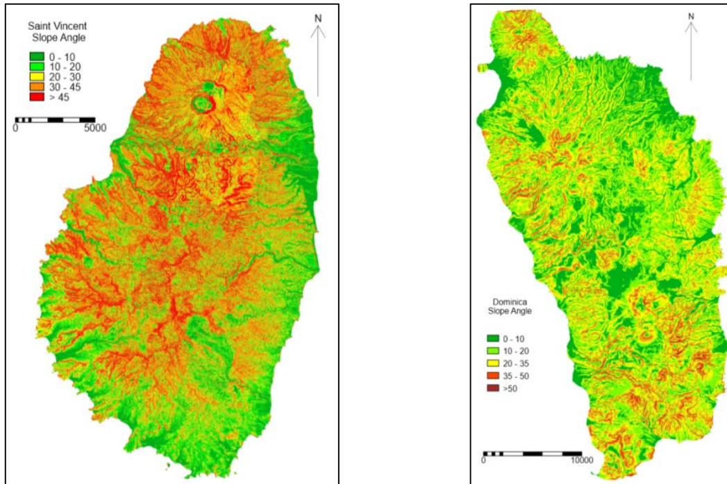
Figure 31. Slope angle map for Saint Vincent (left) and Dominica (Right)
