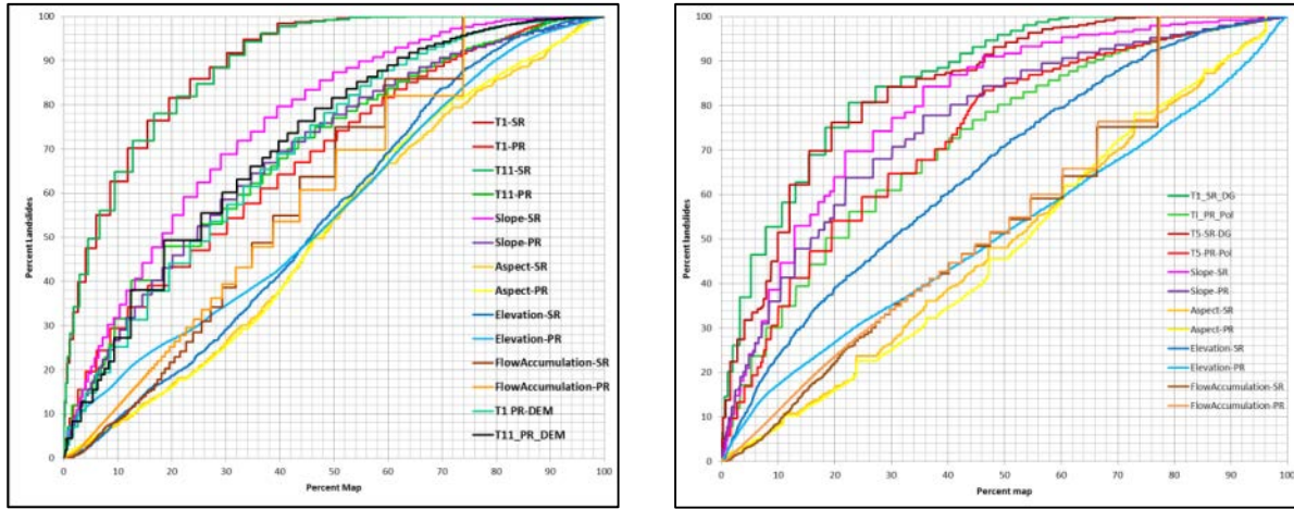
Figure 39. Success and Prediction rate for the initial and final models with standardization method Benefit-Interval, as well as for DEM derivatives for Saint Vincent (left) and Dominica (right).
