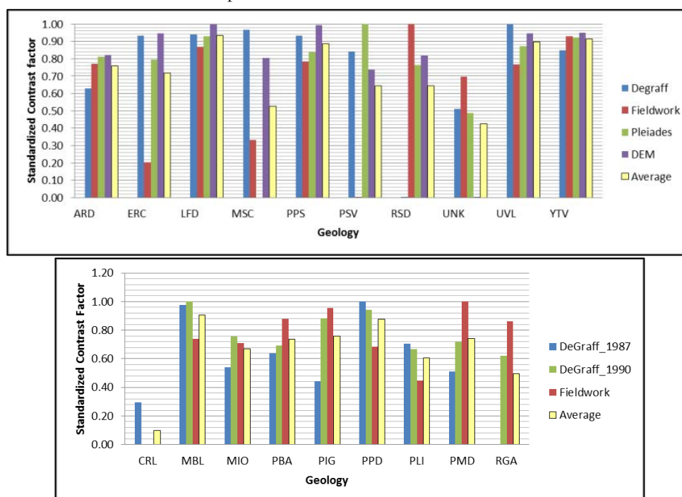
Figure 25. Bar graph showing the contrast factor of each geologic unit for each landslide inventory. And the average contrast factor value. Saint Vincent (Above) and Dominica (Below).
