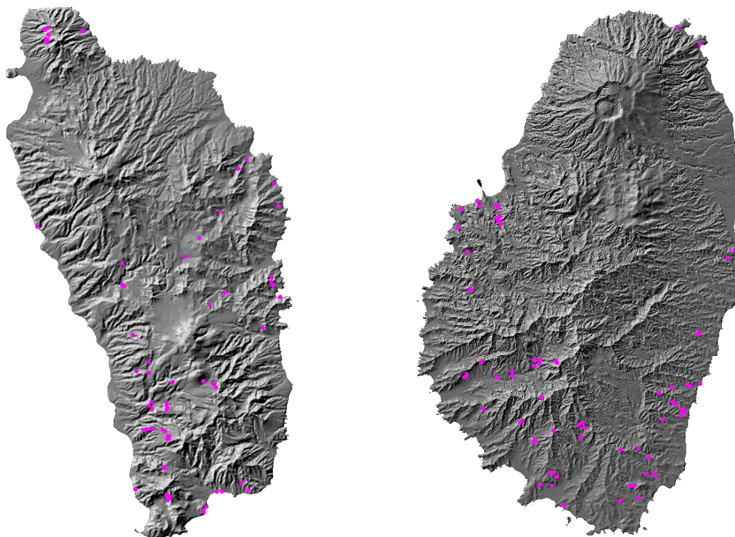
Figure 22. Final landslide inventories collected on fieldwork for Dominica (left) and Saint Vincent (right).
