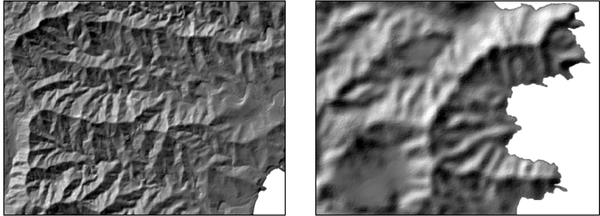
Figure 29. Dem subsets at the same scale, for Saint Vincent (left) and Dominica (right). Notice the differences in detail existing between them.
