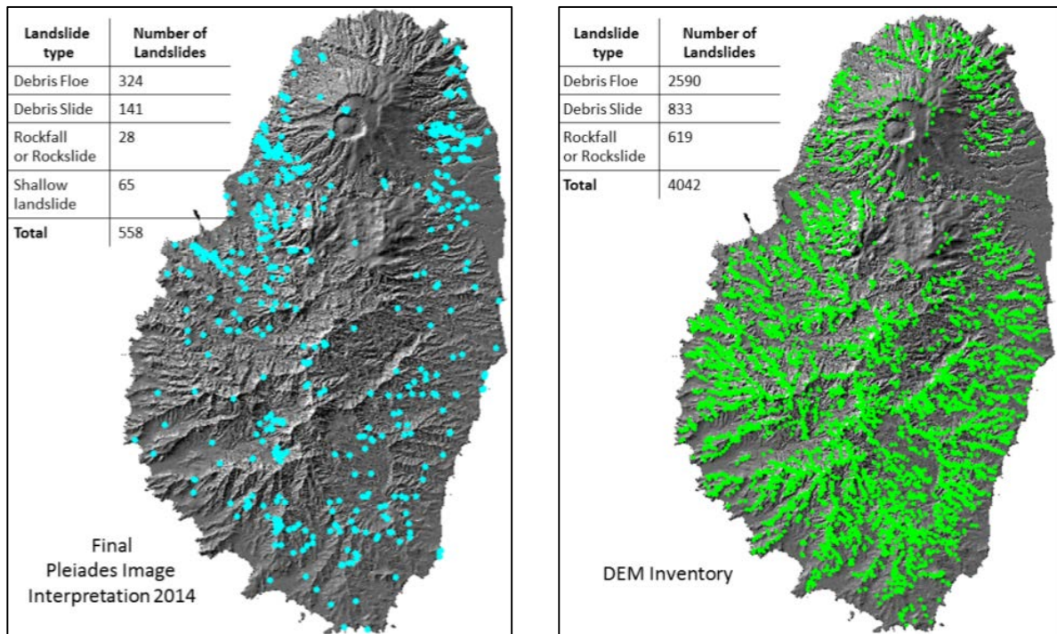
Figure 14. Final landslide inventories based on image interpretation of very high resolution Pleiades images from 2014 and Dem based landslide inventory for Saint Vincent.
