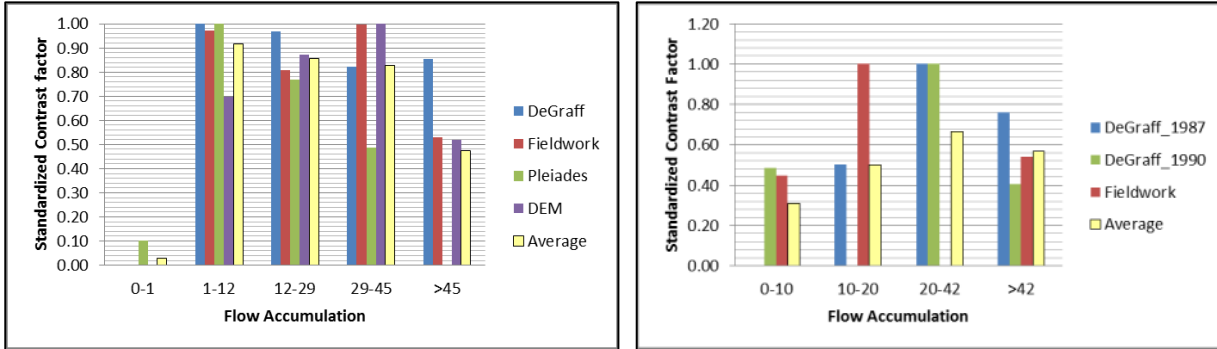
Figure 35. Bar graph showing the contrast factor of each Flow accumulation class for Saint Vincent (left) and Dominica (right)
