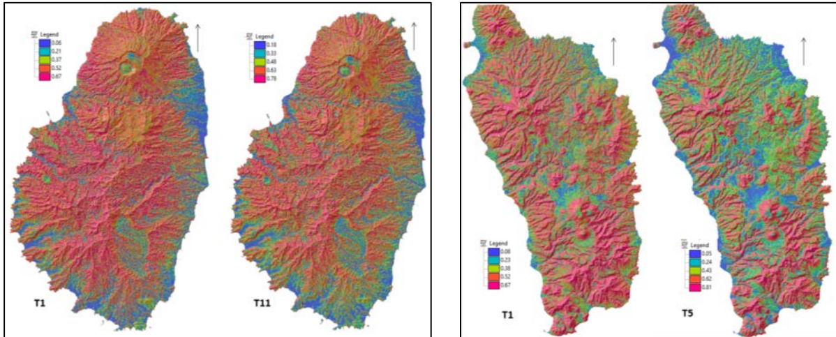
Figure 37. Landslide susceptibility maps obtained on the first and last trials (T1 and T11) for Saint Vincent (left) and (T1 and T5) for Dominica (right).
