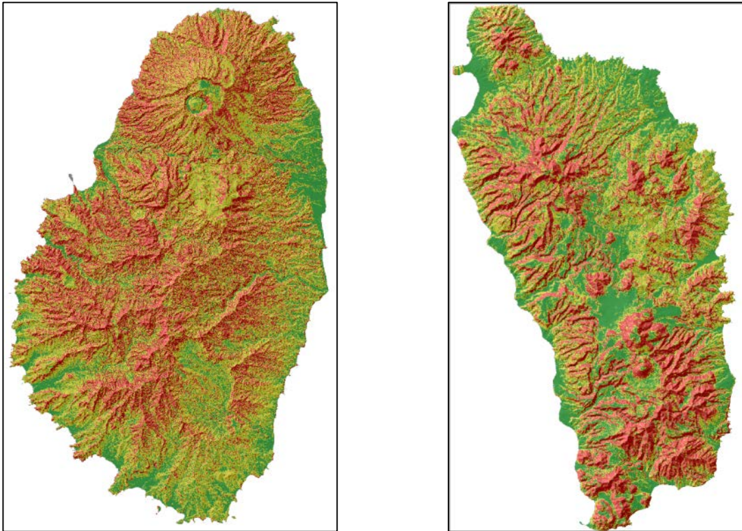
Figure 45. Final landslide susceptibility maps for Saint Vincent (left) and Dominica (right).
