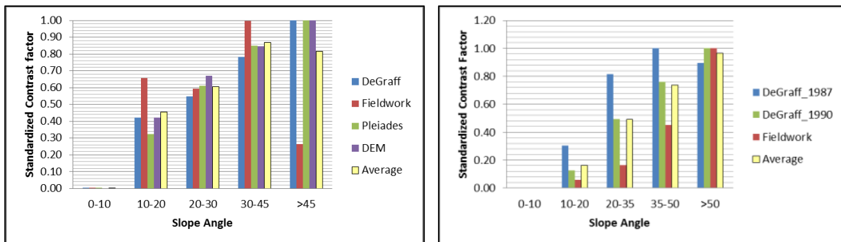
Figure 32. Bar graph showing the contrast factor of each slope angle class for Saint Vincent (left) and Dominica (right)
