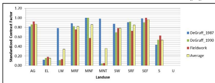
Figure 28. Bar graph showing the contrast factor of each Landuse unit for each landslide inventory in Dominica.
