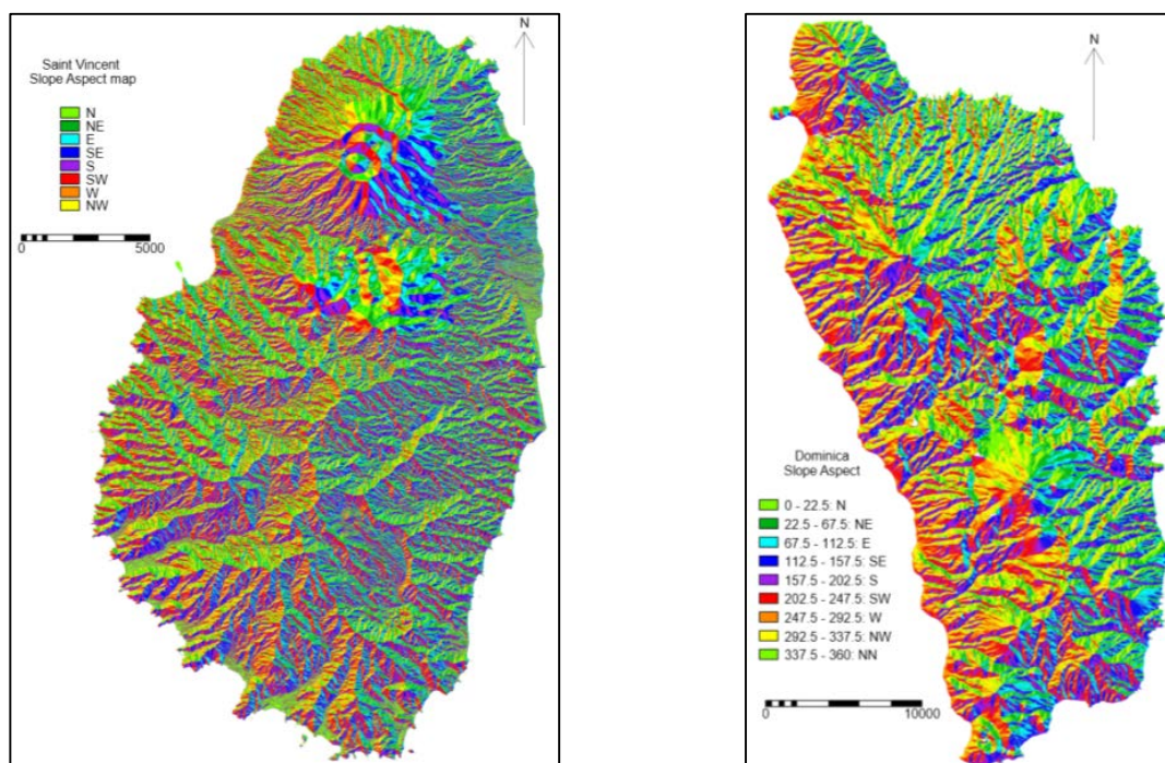
Figure 33. Slope aspect map for Saint Vincent (left) and Dominica (right)
