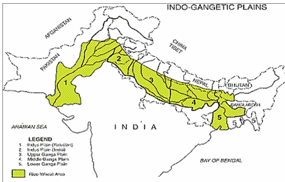
Figure 3-2: Agriculture zone map of Indo-Gangetic Plains (Aggarwal et al., 2004)
