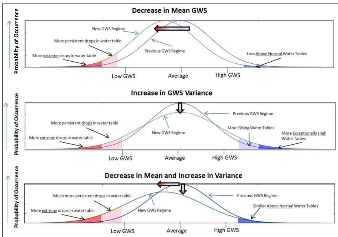
Figure 2-3: Schematic for visualizing effects on extreme GWS events in different scenarios
