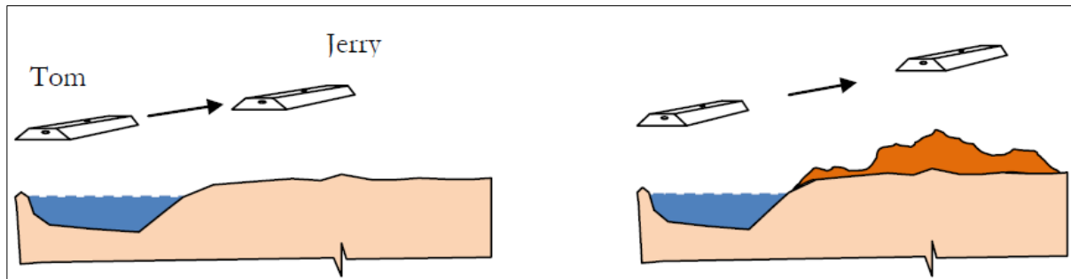
Figure 2-1: The inter-satellite distance varies according to the local gravitational anomaly. When the leading satellite encounters a land/sea interface (left), it decelerates due to the higher gravitational pull because of the denser oceanic crust. On (right), mountainous regions have lower gravitational strength due to isostasy so the inter-satellite distance increases as the leading satellite accelerates (Haile, 2011).
