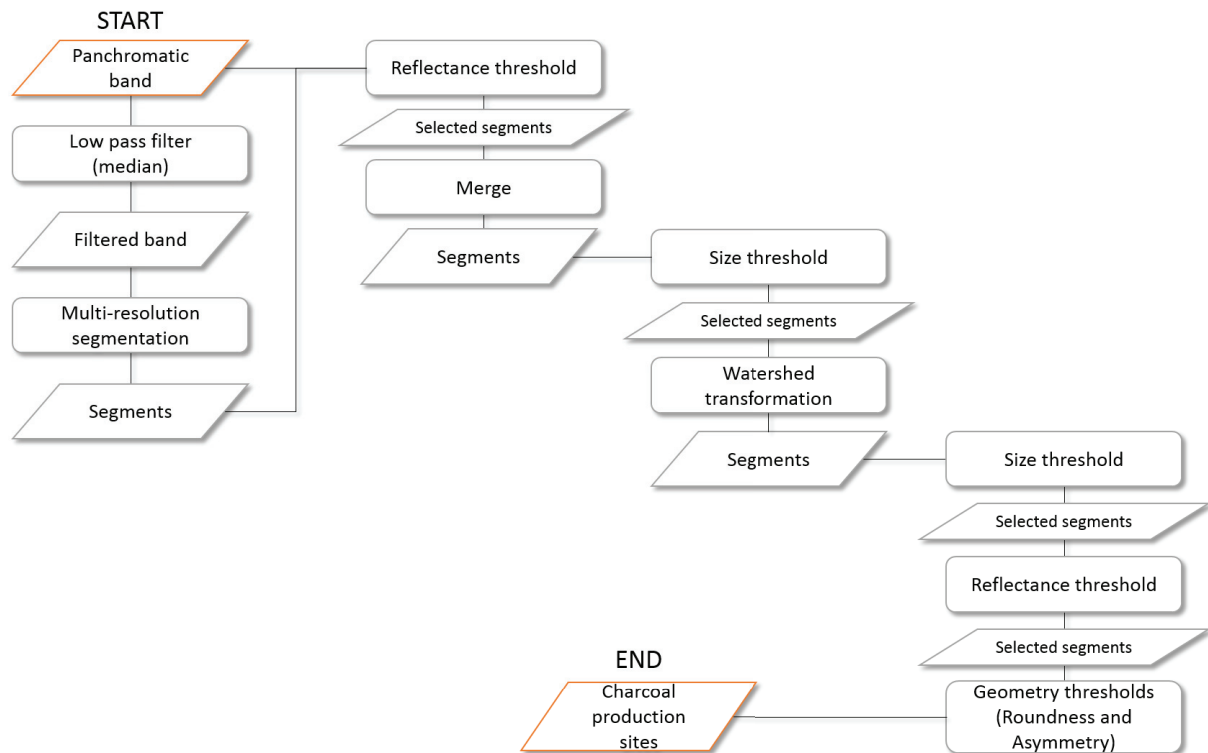
Figure 5 - Object Bases Image Analysis workflow. Once segments are created, a progressive selection is executed based on specified thresholds. While the Threshold-based rules produce a selection of the segments as outputs, the Merge and Watershed processes create new segments requiring new selection, which is obtained by applying new Threshold rules (reflectance and size rules). The final output consists of the objects target of the analysis, charcoal production sites.
