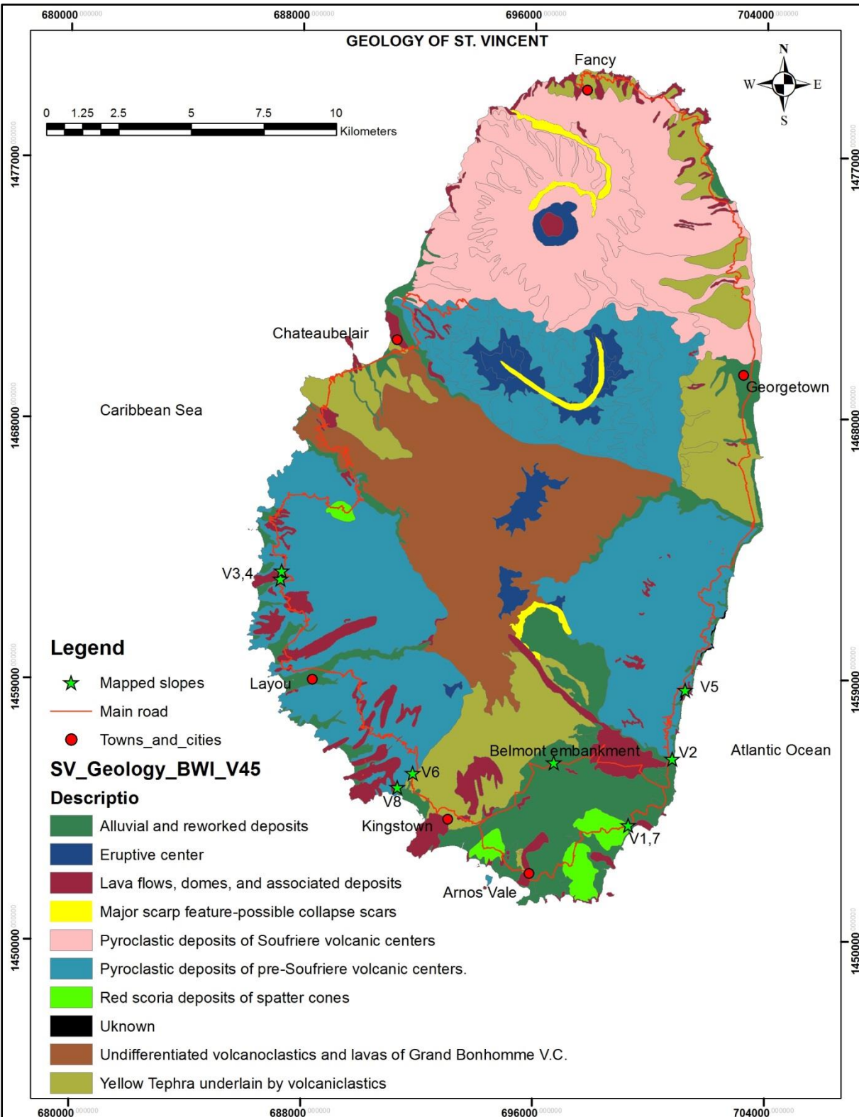
Figure 6: Geology of volcanic centres (after Robertson, 2003)
