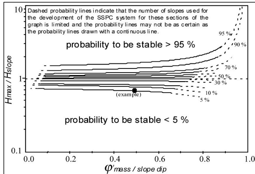
Figure 11: Stability probability as determined in SSPC system
