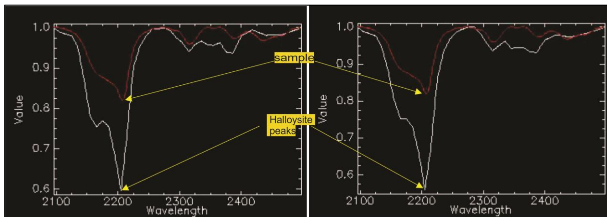
Figure 32: Analytical spectral analysis of rock sample for halloysite
