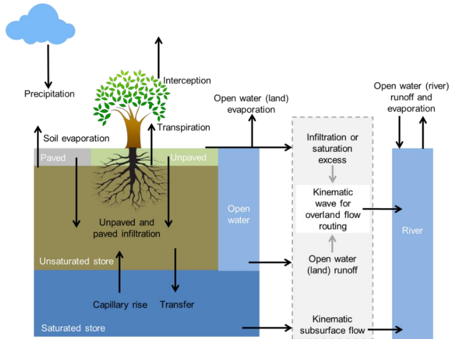
Figure 5 - overview of the wflow-SBM concept (Schellekens, 2019)
