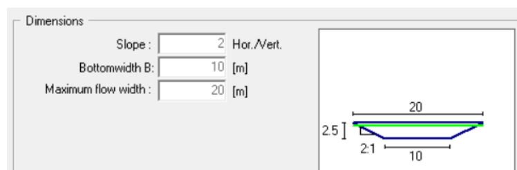
Figure C- 1 – estimated channel dimensions
