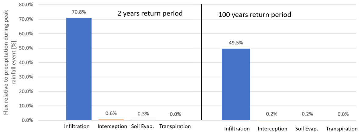
Figure 15 - comparison of average fluxes during the peak rainfall event for different return periods
