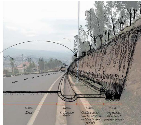
Figure C- 10 - green integrated drain (D5) (World Bank, 2021)
