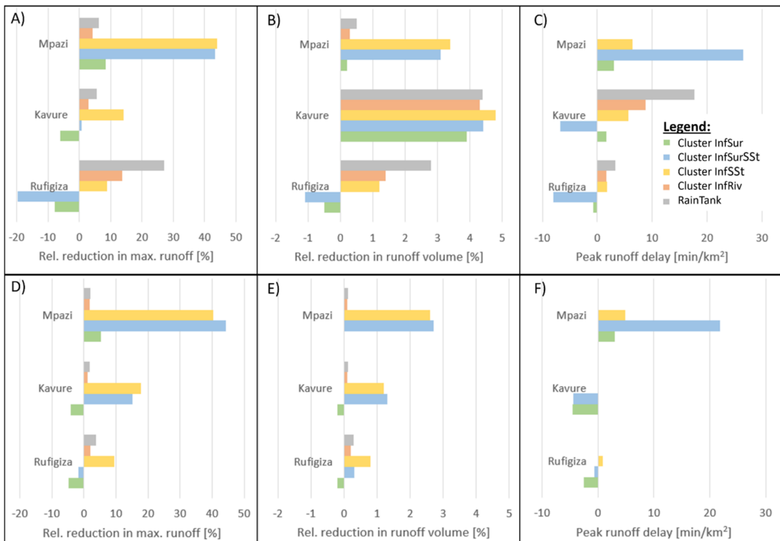
Figure 18 – average individual NBS effects in terms of A, D) relative reduction in maximum runoff, B, E) relative reduction in peak runoff volume, C, F) peak runoff delay. A-C is for a 2-year return period and D-F for a 100-year return period
