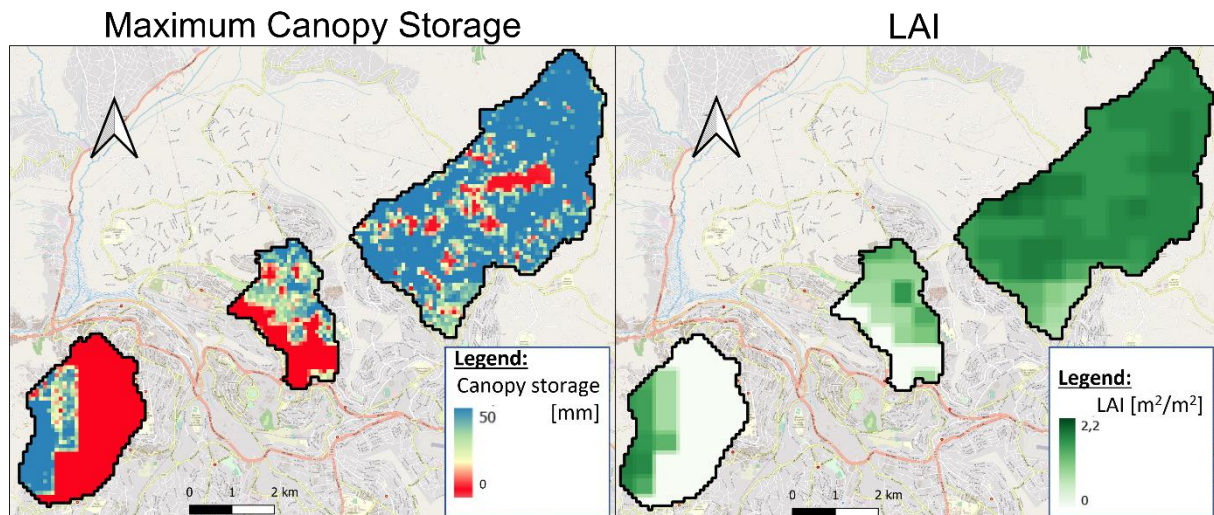
Figure 17 – the maximum storage capacity of Swood (50 mm) is not used when LAI is low
