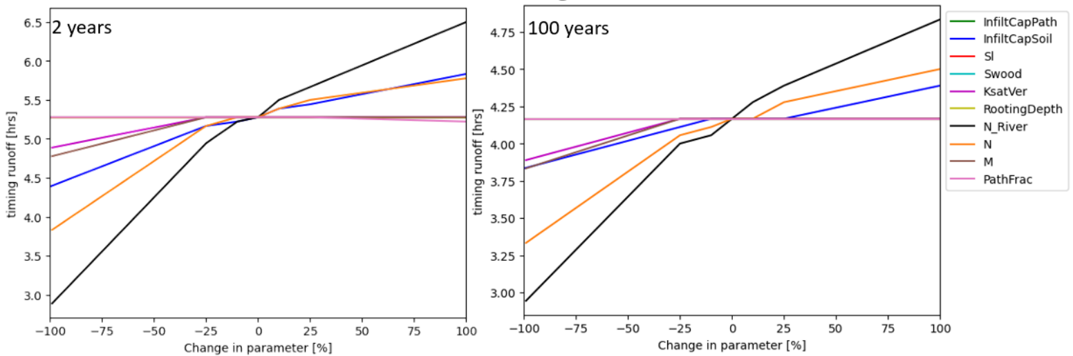
Figure 14 - the average sensitivity of the time between the start of the rainfall event and the maximum runoff for different wflow parameters for return periods of rainfall of 2 and 100 years
