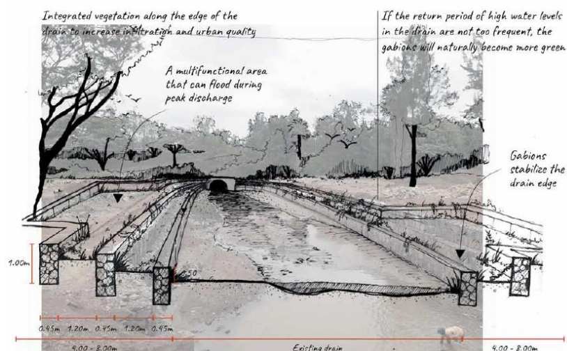
Figure C- 12 - stepped drain (F4) (World Bank, 2021)
