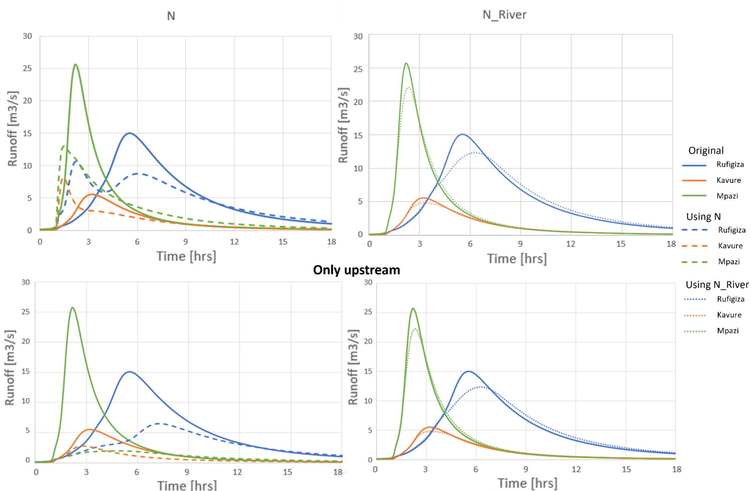
Figure H- 2 - changes in flood waves after increasing the roughness upstream and decreasing it downstream (top), and only increasing the upstream roughness (bottom) for a return period of two years
