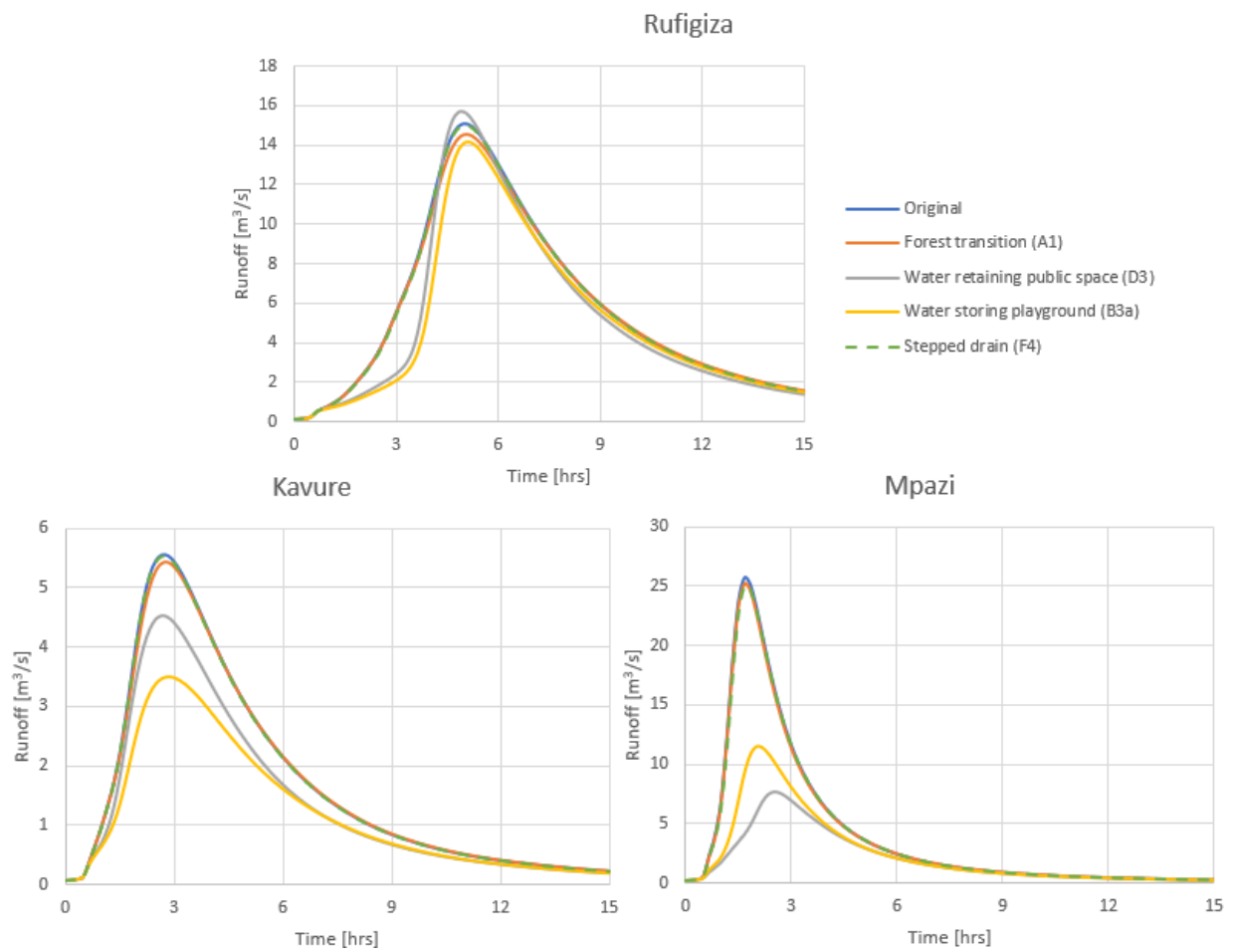
Figure 24 – hydrographs after implementing individual NBSs in all sub-catchments. One NBS is selected from each sub-catchment.
