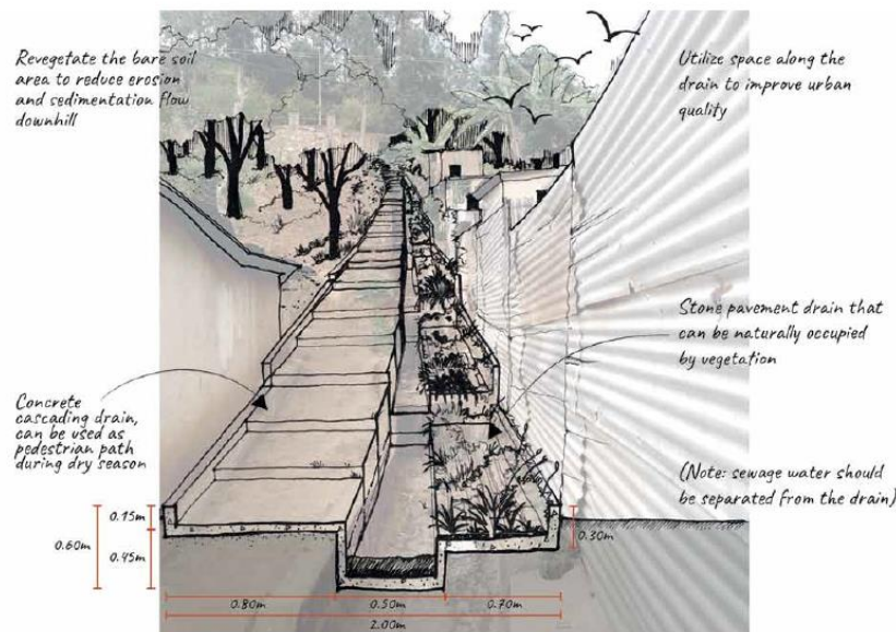
Figure C- 9 - integrated neighbourhood drain (B2) (World Bank, 2021)
