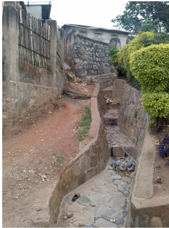
Figure I- 1 – stepped drain in Mpazi
