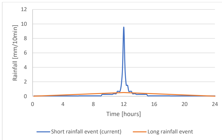
Figure 10 - plotted time series of long and short rainfall events which volume has a return period of two years
