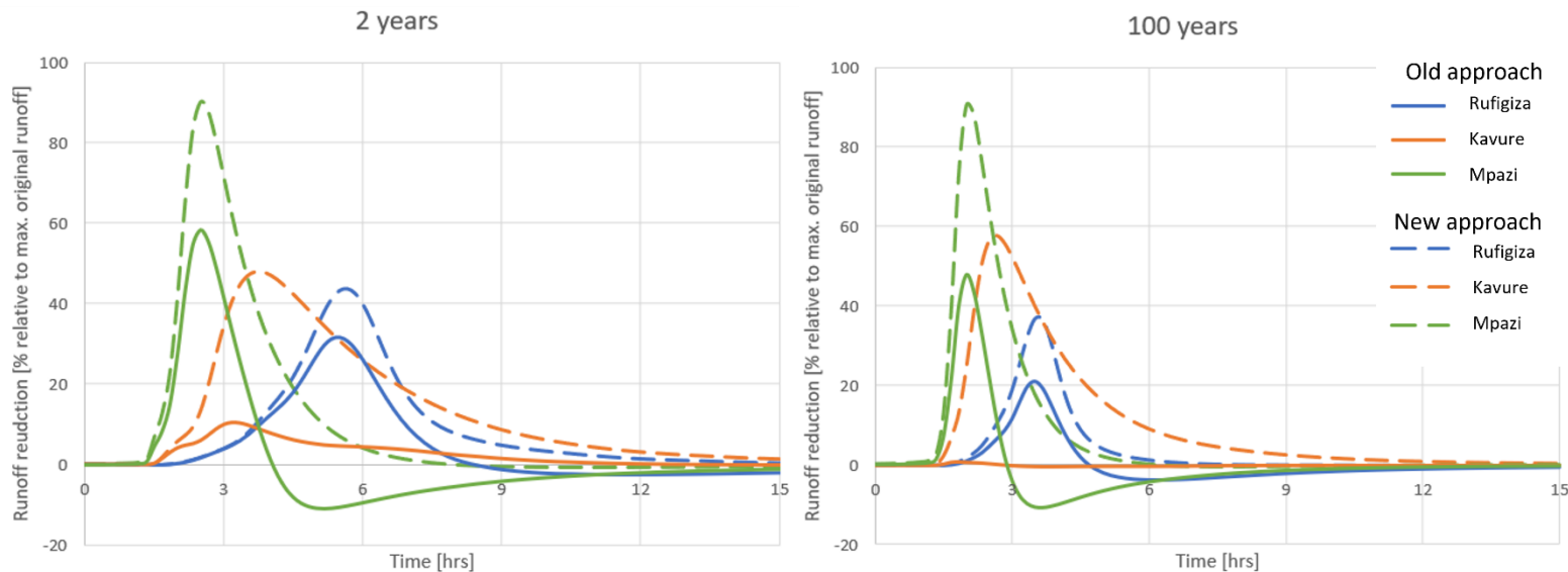
Figure 23 - comparison of combined effects of NBSs for the old and new approach for different sub-catchments and return periods
