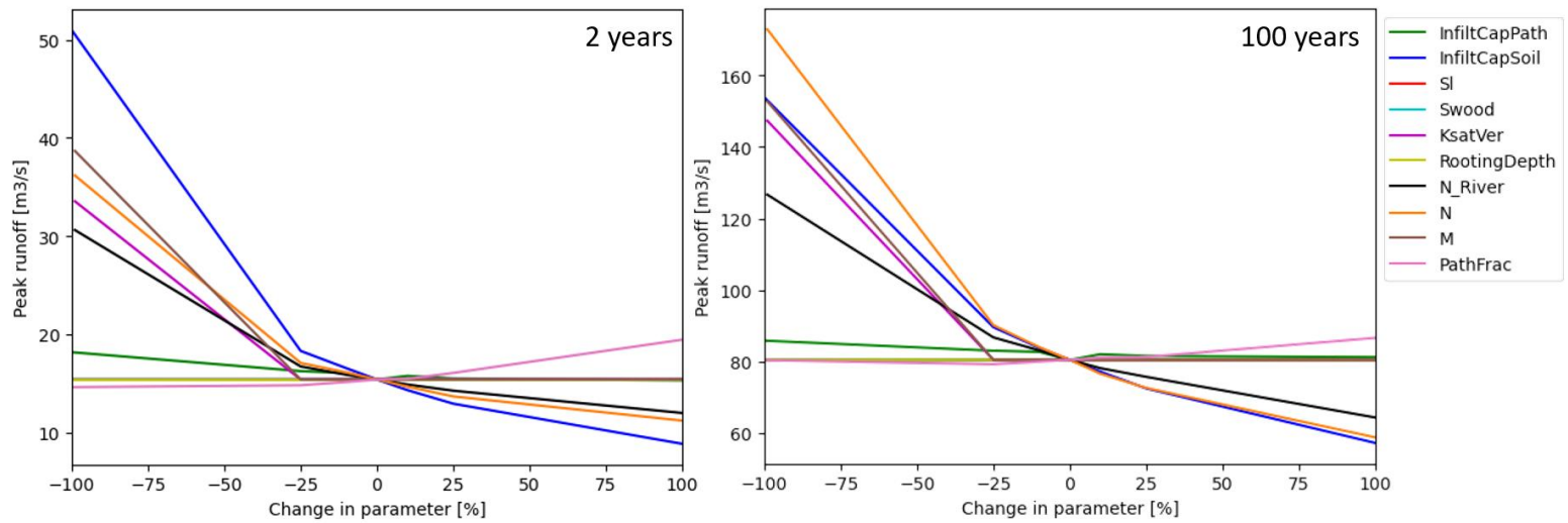
Figure 12 – the average sensitivity of the maximum runoff for different wflow parameters for return periods of rainfall of 2 and 100 years
