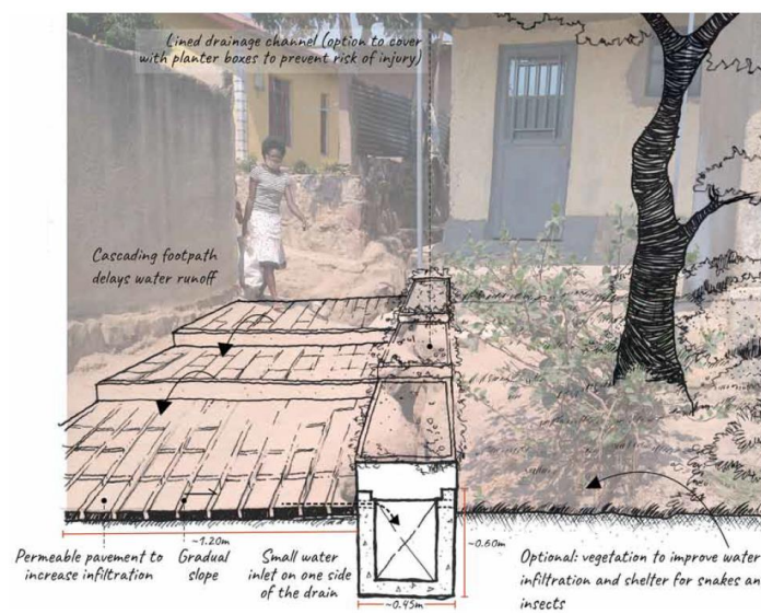
Figure C- 11 - Stepped footpath with planters (F3a) (World Bank, 2021)
