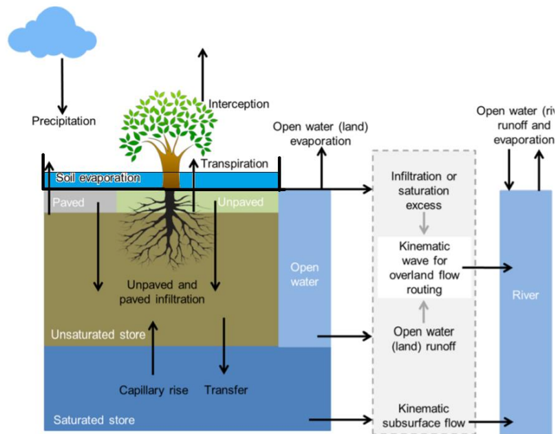
Figure B- 10 - SBM concept including the additional storage bucket
