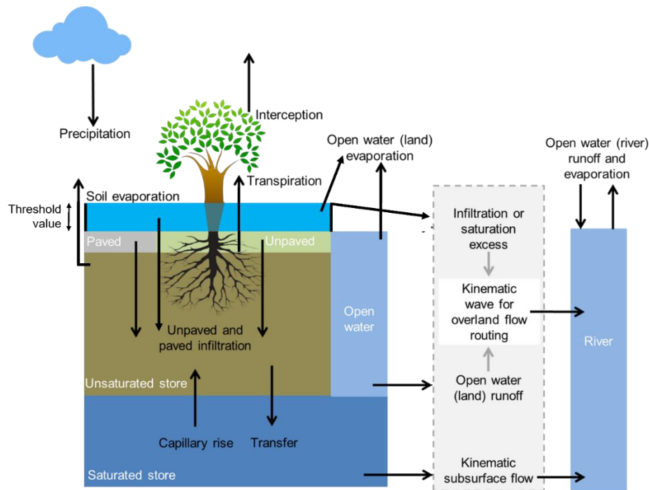
Figure D- 1 – wflow-SBM concept including additional storage layer
