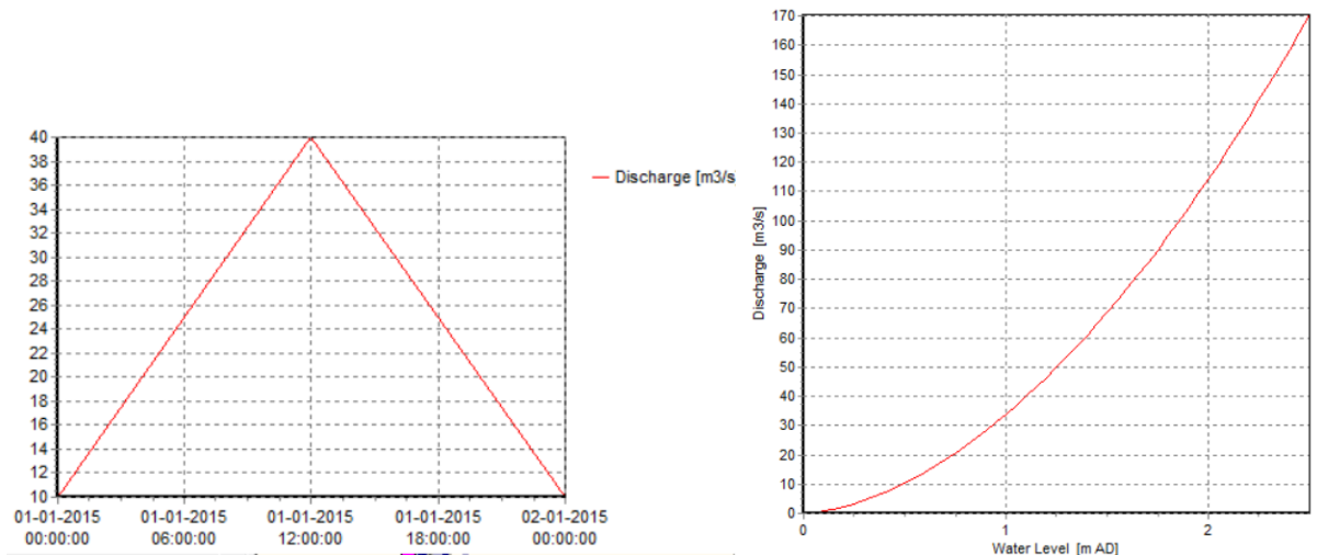
Figure C-2 - left: incoming flood wave; right: Q-h relation
