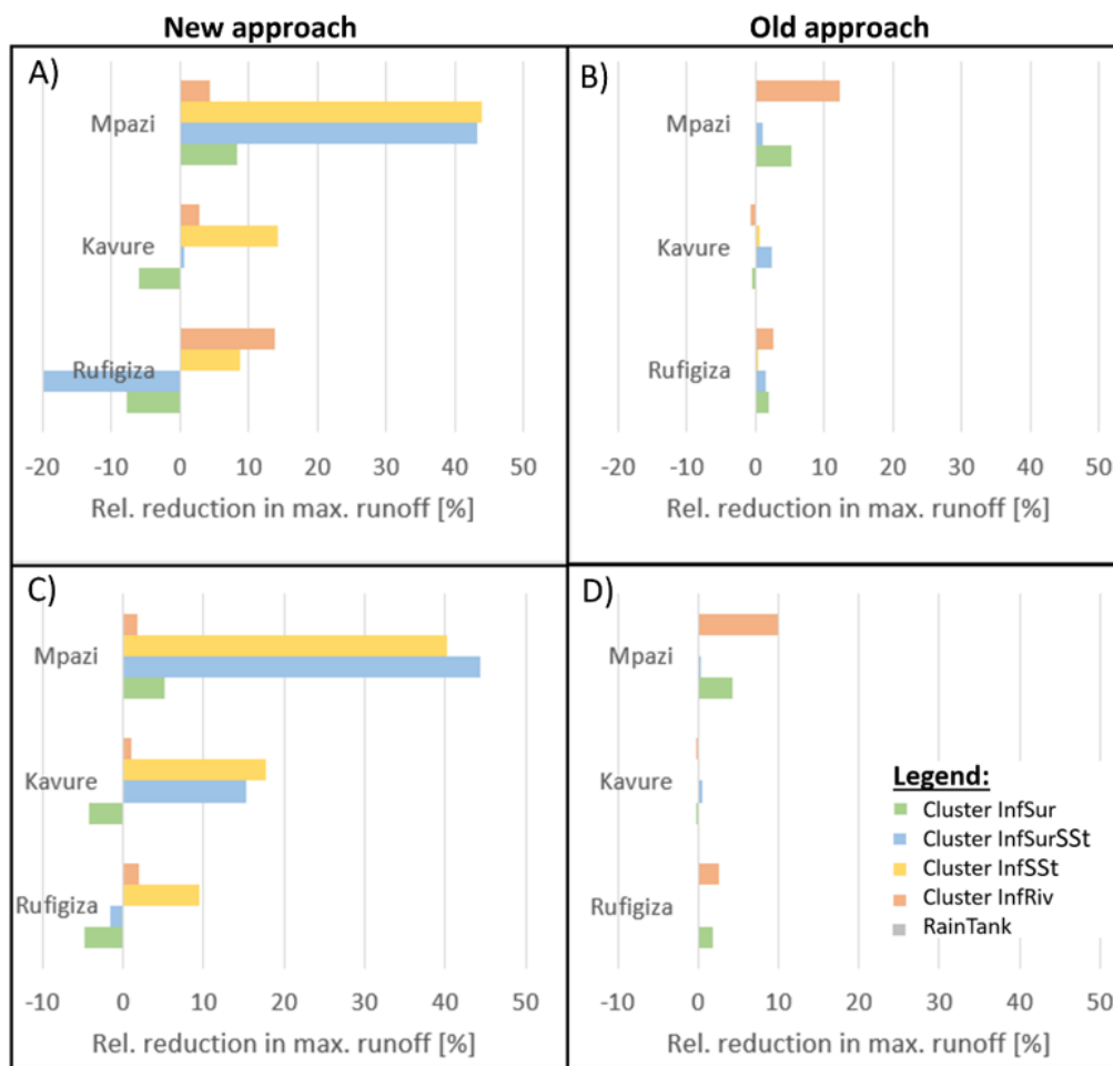
Figure 22 - average individual effects of NBSs for the new (A, C) and old approach (B, D) for return periods of two years (A, B) and 100 years (C, D)
