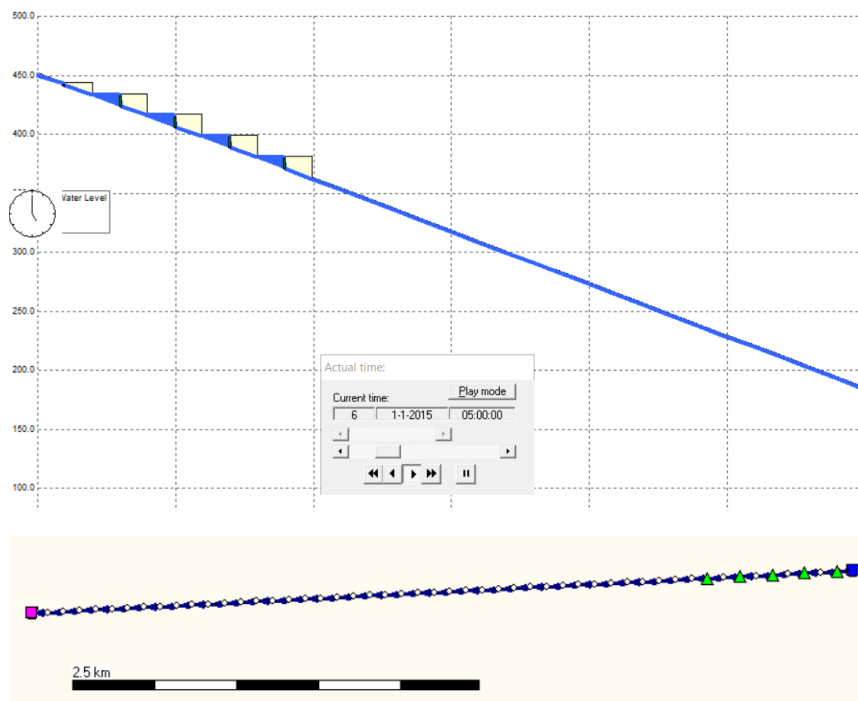
Figure C-3 - placement of Gabions. Top: side view; bottom: top view
