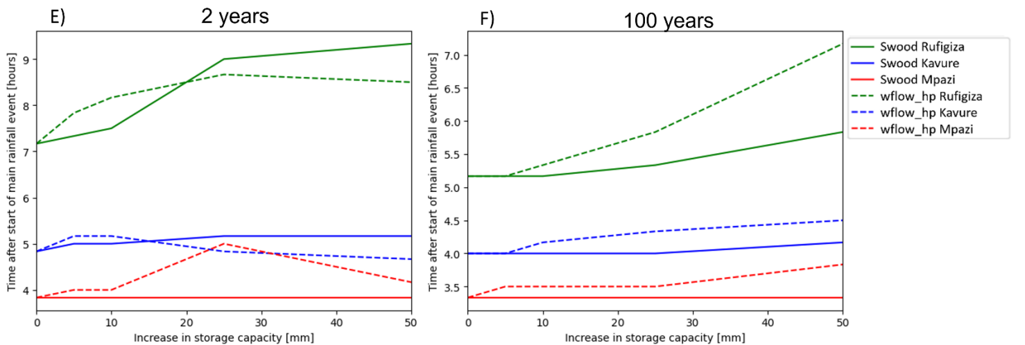
Figure 16 - Sensitivity of the maximum runoff (fig. A & B), runoff volume (fig. C & D) and timing (fig. E & F) when using Swood (tree trunk interception parameter) and wflow_hp (new additional storage layer)
