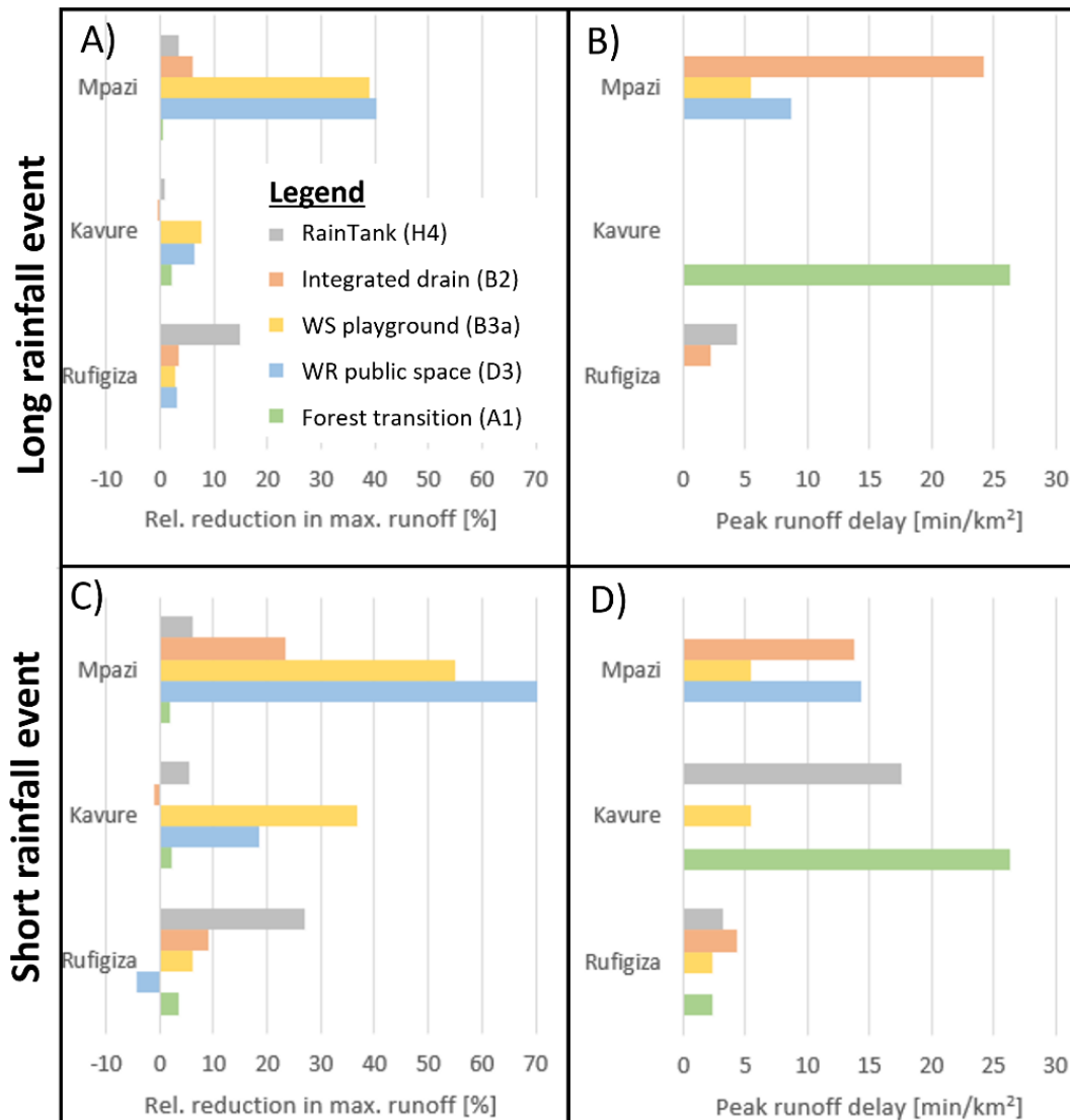
Figure 21 - NBS effects for a long (A, B) and short rainfall event (C, D) in terms of relative reduction in maximum runoff (A, C) and peak runoff delay (B, D) for a two-year return period
