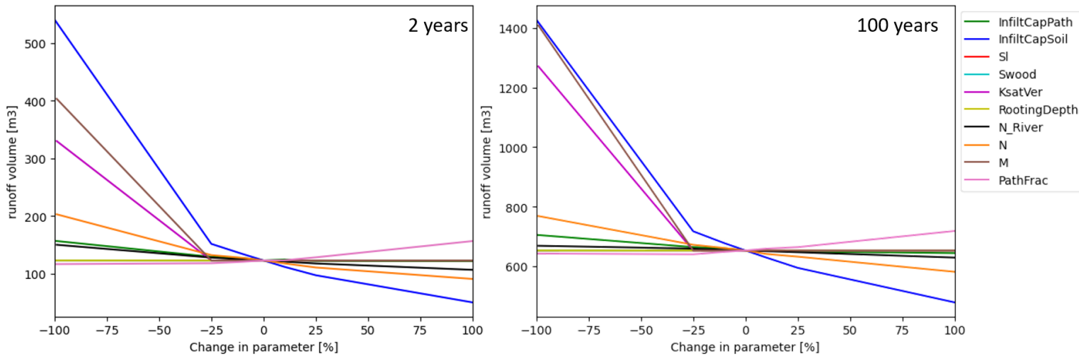
Figure 13 - the average sensitivity of the runoff volume for different wflow parameters for return periods of rainfall of 2 and 100 years
