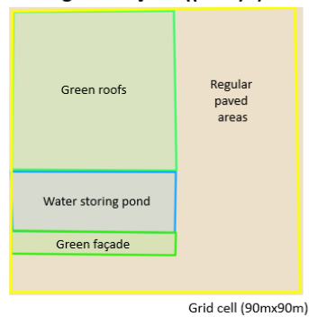
Figure C- 6 - schematisation of a water storing pond, green roofs and green facade in a grid cell in AST
