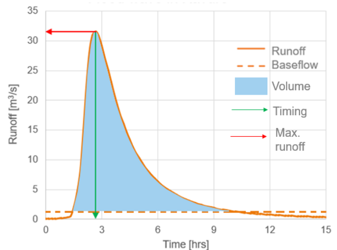
Figure 9 - illustration of baseflow, maximum runoff, peak runoff volume and timing for a flood wave in Kavure
