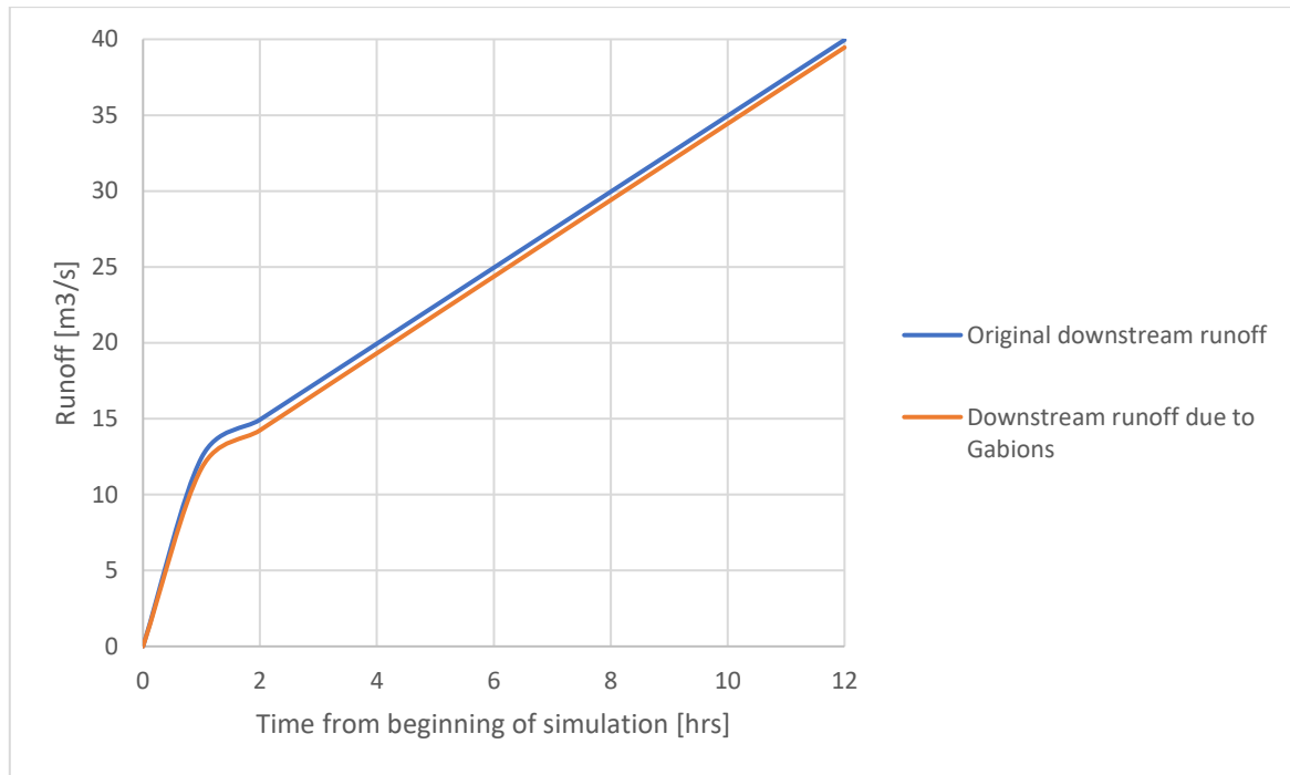
Figure C- 4 - change in runoff due to the gabions over time during the rising limb of the flood wave
