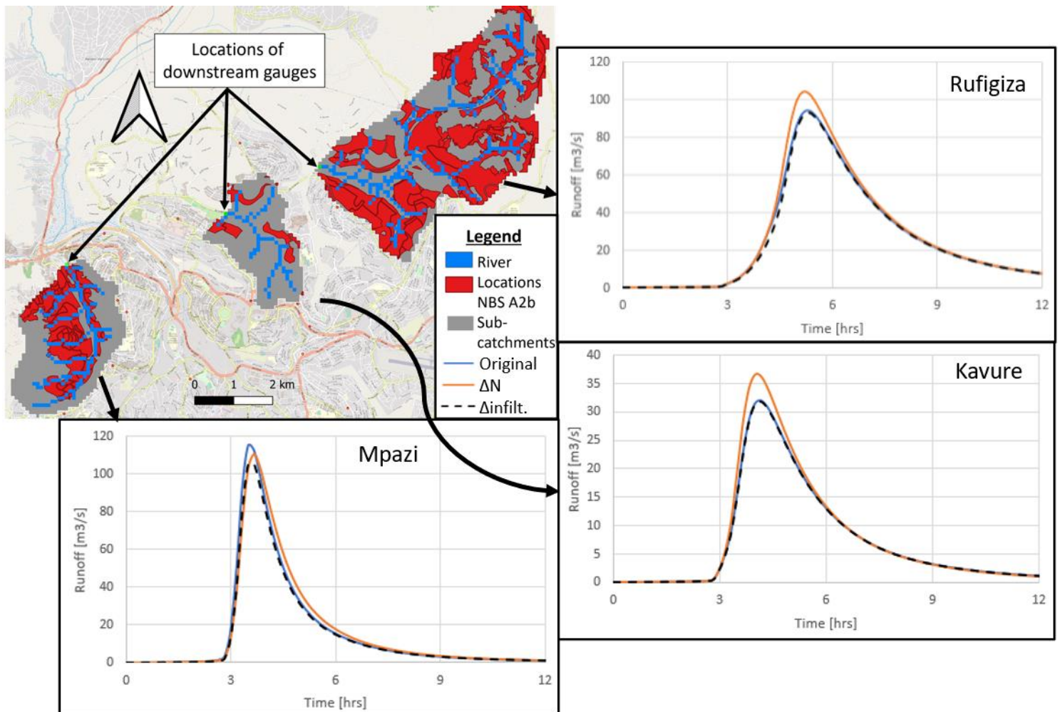
Figure 19 - downstream runoff for the three sub-catchments when changes in the infiltration rate and surface roughness of NBS A2b (contour planting) are compared to the original runoff when the return period is 100 years
