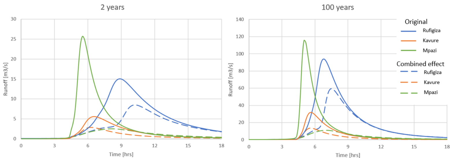
Figure 20 - combined effects of NBSs per sub-catchment for different return periods
