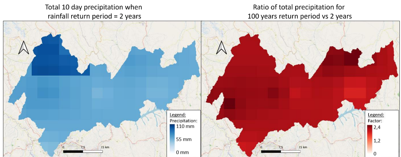
Figure 6 – cumulative precipitation sum in Nyabugogo catchment for a return period of two years (left) and the corresponding ratio of cumulative rainfall when the return period is 100 years to when it is two years
