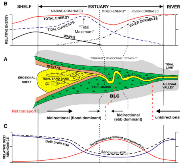
Figure 1: Distribution of the energy and sediment transport over the length of the estuary (Dalrymple and Choi, 2007)
