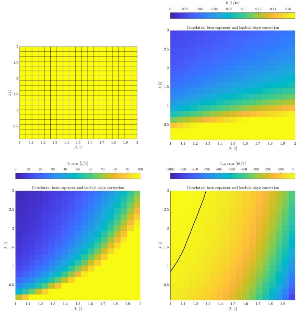
Figure 19: The combined effect of the bed load exponent \beta_b on the x-axis and slope correction factor \lambda on the y-axis and their effect on FGM. The top left figure represents the accuracy of the calculation, with yellow all accurate calculated perturbed flows. Top right the wave number, bottom left the growth rate and bottom right migration rate.
