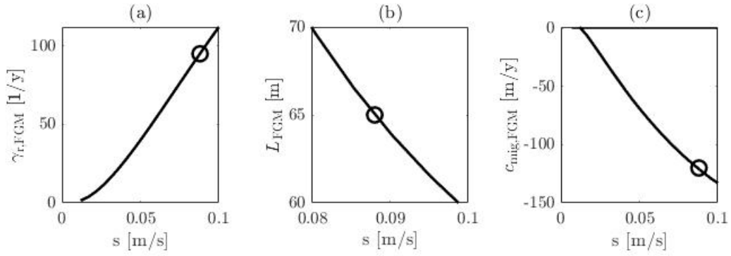
Figure 23: The calibration of the slip parameter for the Scheldt estuary at Terneuzen. a) The corresponding growth rate, b) The wave length limited around the mean wave length c) the corresponding migration rate
