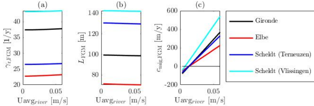
Figure 20: The validation of the model based on 4 different sets of input parameters, of which the Gironde is the calibrated set and the other 3 locations are for validation
