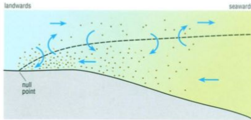
Figure 2: Schematization of the density-driven estuarine circulation. The flow represented on top part of the watercolumn is the freshwater flow and the saltwater flow is represented by the lower part of the water-column. (Colling et al., 1999)
