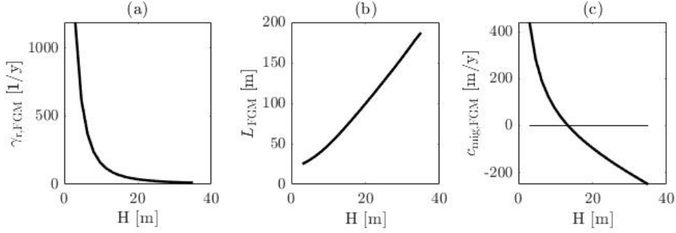
Figure 5: Sensitivity of the FGM to changes in the water depth range 3-35 (m) a: Growth rate of FGM b: wave length of FGM c: migration speed of FGM
