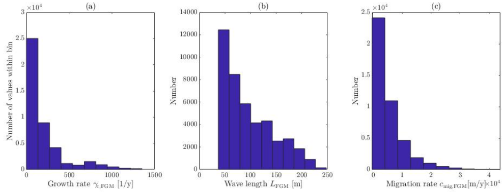
Figure 15: The environmental parameter dependency variation based on the a: the growth rate, b: wave length, c: migration rate.
