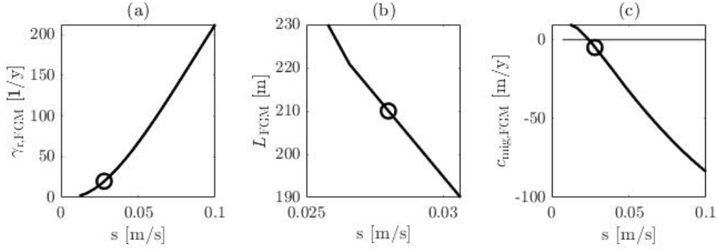
Figure 22: The calibration of the slip parameter for the Scheldt estuary at Vlissingen. a) The corresponding growth rate, b) The wave length limited around the mean wave length c) the corresponding migration rate
