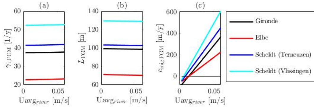
Figure 27: The validation of the model based on 4 different sets of input parameters with the same water depth of 20 meters, of which the Gironde Estuary is the calibrated set and the other 3 locations are for validation
