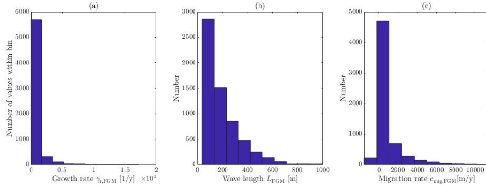
Figure 16: The empirical model parameter dependency variation based on the a: the growth rate, b: wave length, c: migration rate.
