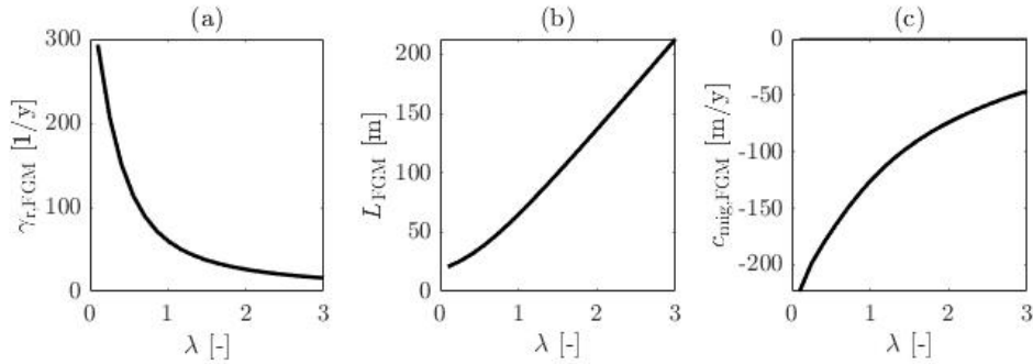
Figure 14: Sensitivity slope gradient range 0.1-3.0, a: Growth rate of FGM b:wave length of FGM c: migration speed based of FGM
