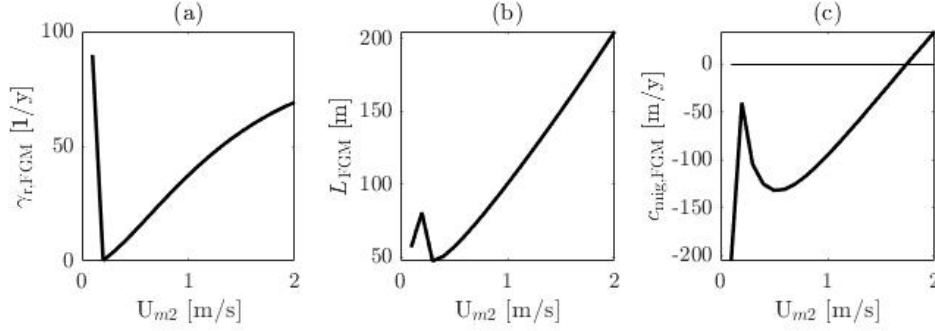
Figure 6: Sensitivity of the FGM to changes in the depth averaged M2 velocity amplitude range 0.1-2.0 (m/s), a: Growth rate of FGM b: wave length of FGM c: migration speed of FGM. The range 0.1 to 0.3m/s inaccurately calculated which causes the jumps in the graph
