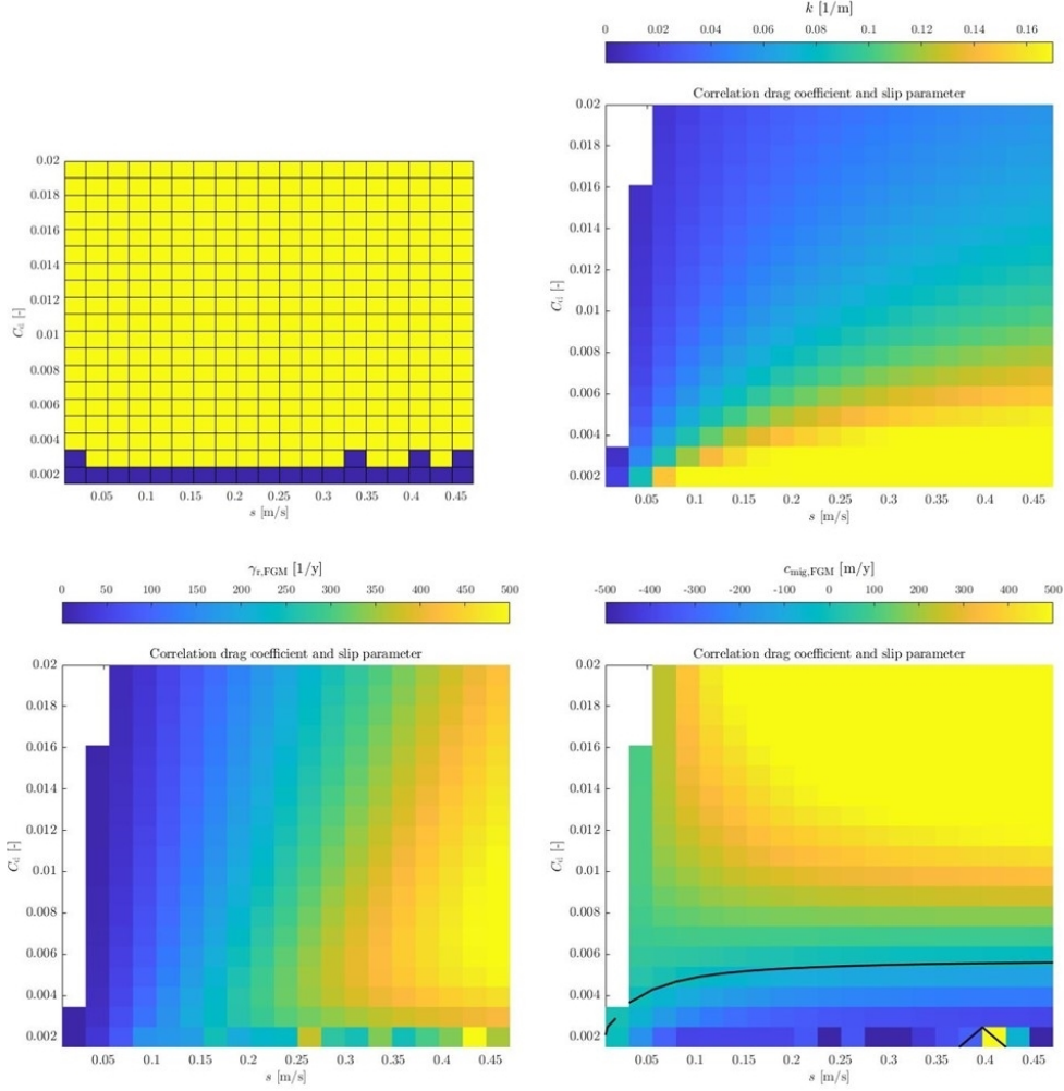
Figure 18: The combined effect of the slip parameter on the x-axis and the drag coefficient on the y-axis and their effect on FGM. The top left figure represents the accuracy of the calculation, with blue inaccurate. Top right the wave number, bottom left growth rate and bottom right migration rate.
