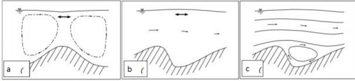
Figure 3: Schematization of the flow patterns and shapes of three different bed forms. a marine sand waves, which are driven by the tidal current. b estuarine sand dunes, which are affected by the tidal current and the river flow. However, this interaction is still not understood. c sketch of a river dune effected by the river flow including flow separation in the trough (van der Sande et al., 2019) inspired by Hulscher and Dohmen-Janssen (2005)
