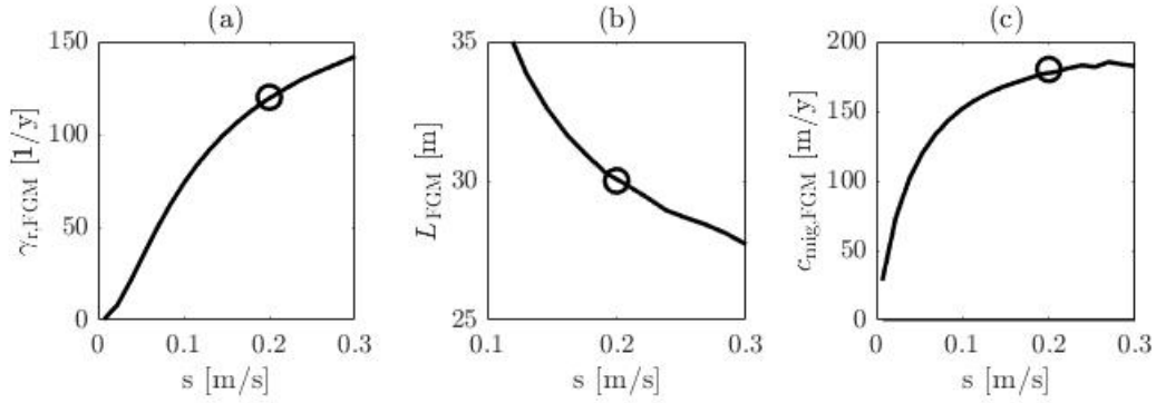
Figure 21: The calibration of the slip parameter for the Elbe estuary at Grauerort. a) The corresponding growth rate, b) The wave length limited around the mean wave length c) the corresponding migration rate
