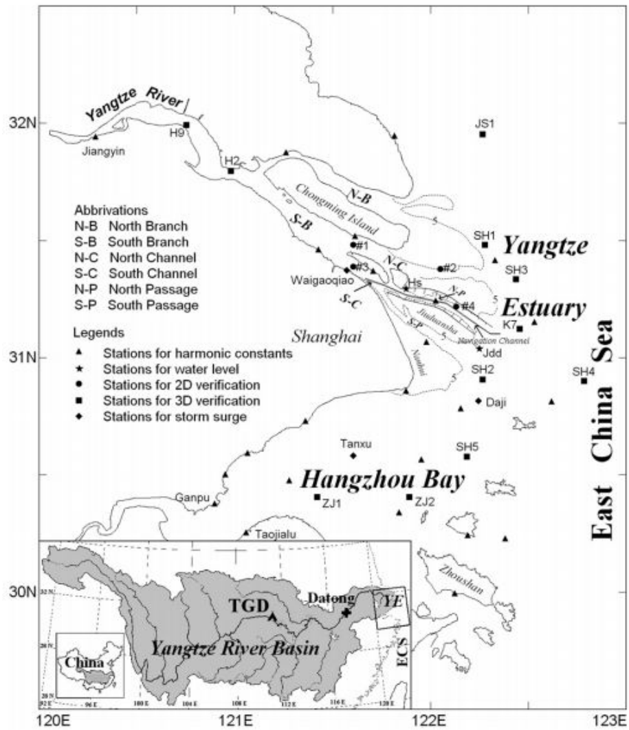
Figure 28: Overview of Yangtze Estuary Hu et al. (2009)
