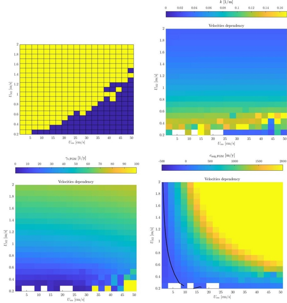
Figure 17: The combined effect of the depth averaged river flow velocity on the x-axis and the depth averaged tidal velocity amplitude on the y-axis and their effect on FGM. The top left figure represents the accuracy of the calculation, with blue inaccurate. Top right the wave number, bottom left growth rate and bottom right migration rate.
