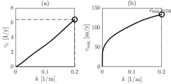
Figure 24: Example of a growth rate and migration curve where there is no maximum calculated growth rate. ( H=10.83m, U_{M2}=0.2m/s, U_{res}=0.17m/s, \phi=1.16 \text{ psu/km}, D_{50}=634\mu m )
