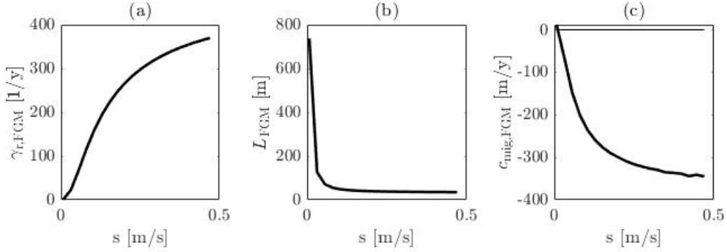
Figure 12: Sensitivity slip parameter range 0.007-0.47 (m/s), a: Growth rate of FGM b: wavelength of FGM c: migration speed based on FGM
