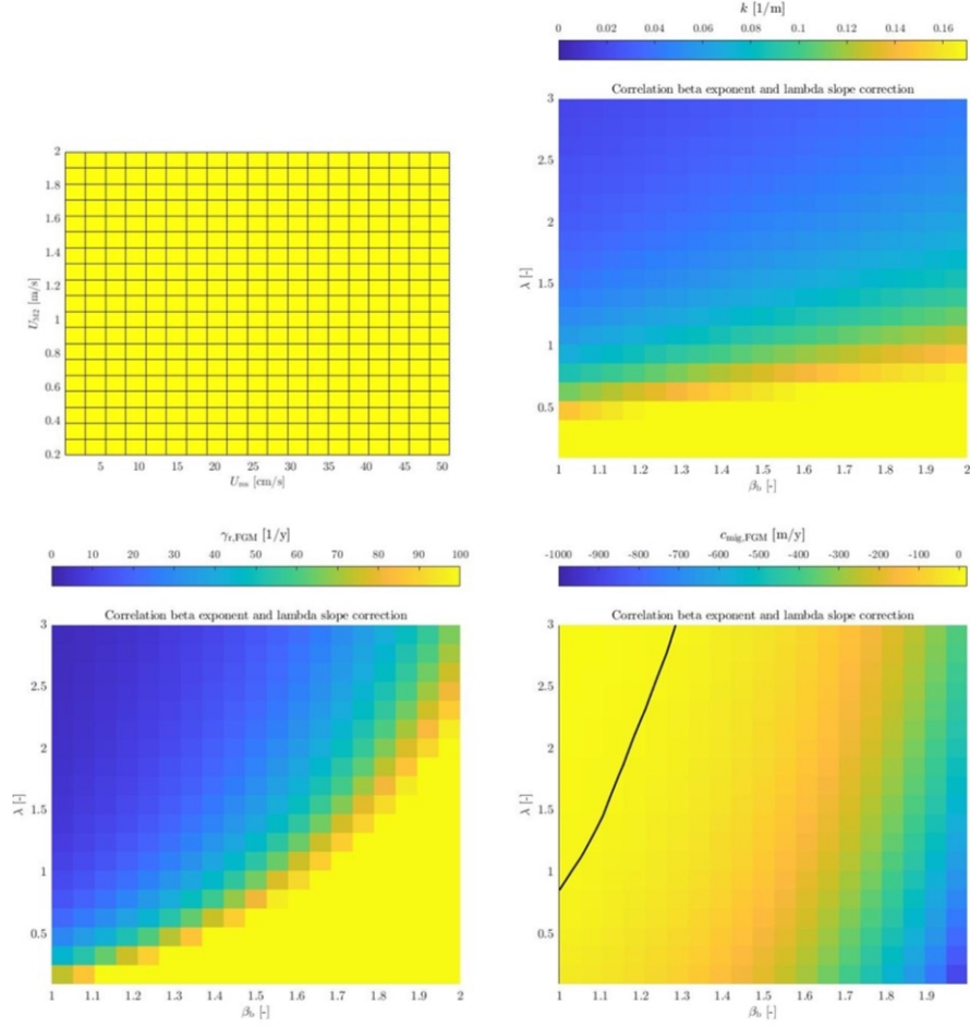
Figure 25: Solution 2 (sum of the velocities): The combined effect of the depth averaged river flow velocity on the x-axis and the depth-averaged tidal velocity amplitude on the y-axis and their effect on FGM. The top left figure represents the accuracy of the calculation, with blue inaccurate. Top right the wave number, bottom left growth rate and bottom right migration rate.
