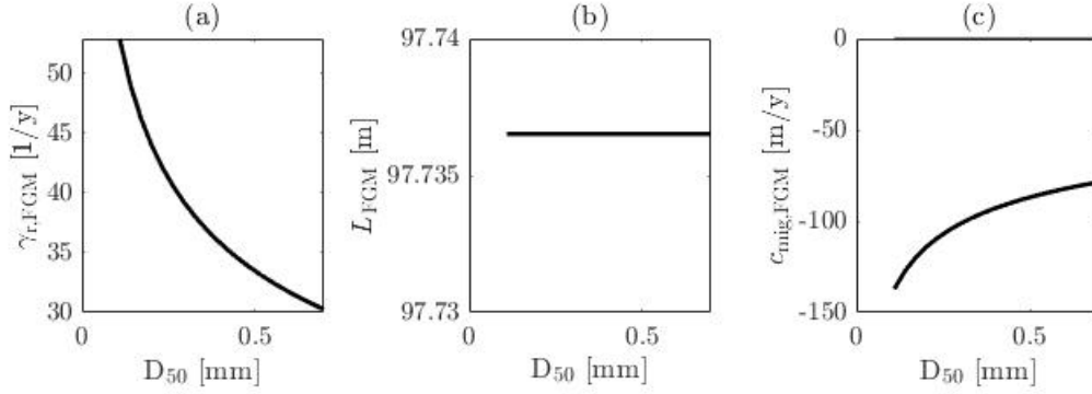
Figure 9: Sensitivity of the FGM to changes in the sediment size 108-700 ( \mu\text{m} ) , a: Growth rate of FGM b:wave length of FGM c: migration speed based of FGM
