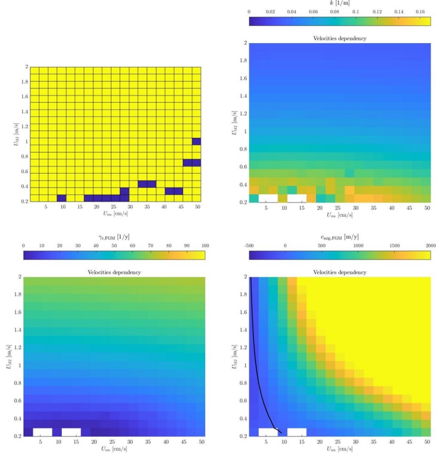
Figure 26: Solution 3 (Pythagoras with the velocities) :The combined effect of the depth-averaged river flow velocity on the x-axis and the depth-averaged tidal velocity amplitude on the y-axis and their effect on FGM. The top left figure represents the accuracy of the calculation, with blue inaccurate. Top right the wave number, bottom left growth rate and bottom-right migration rate.
