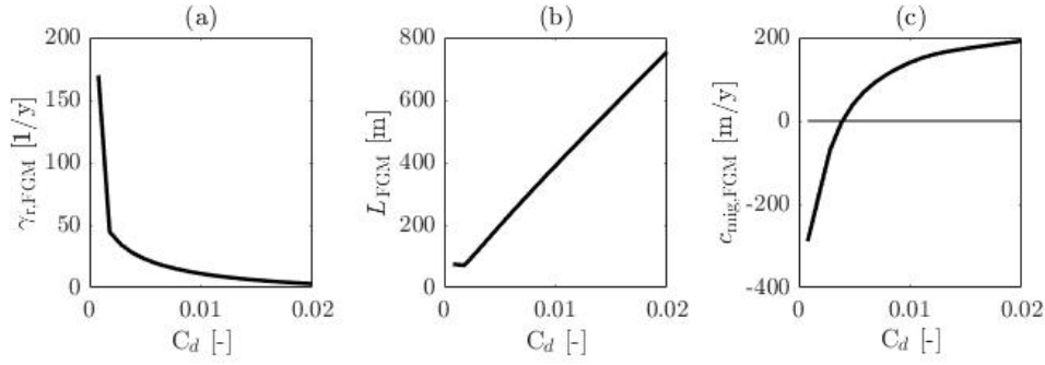
Figure 11: Sensitivity drag coefficient parameter range 8 \cdot 10^{-4} - 2 \cdot 10^{-2} (-), a: Growth rate of FGM b: wavelength of FGM c: migration speed of FGM. Point c_d = 0.008 has an inaccurately calculated perturbed flow and therefore presents an inaccurate calculation of this FGM
