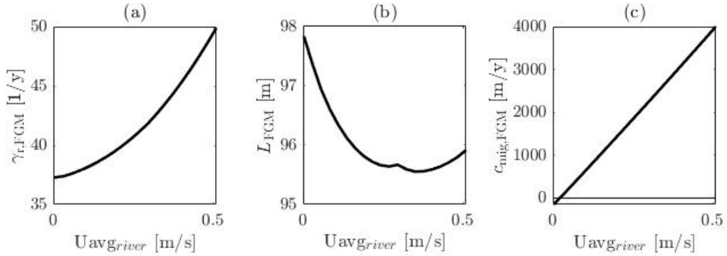
Figure 7: Sensitivity of the FGM based to changes in the river current range 0.002-0.51 (m/s) , a: Growth rate of FGM b: wave length of FGM c: migration speed of FGM
