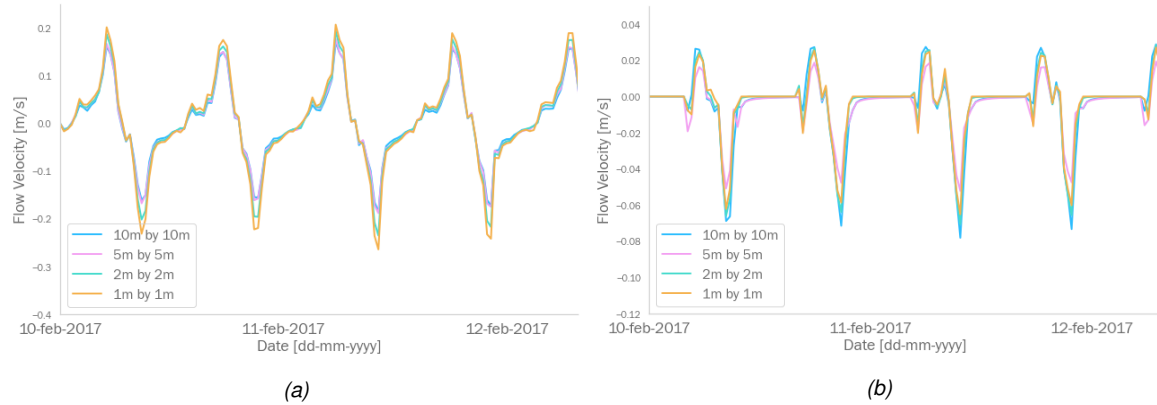
Figure 5.7: Sensitivity analysis of the flow velocities on varying grid sizes. (a) Location 3 and (b) Location 4 in figure 5.4
