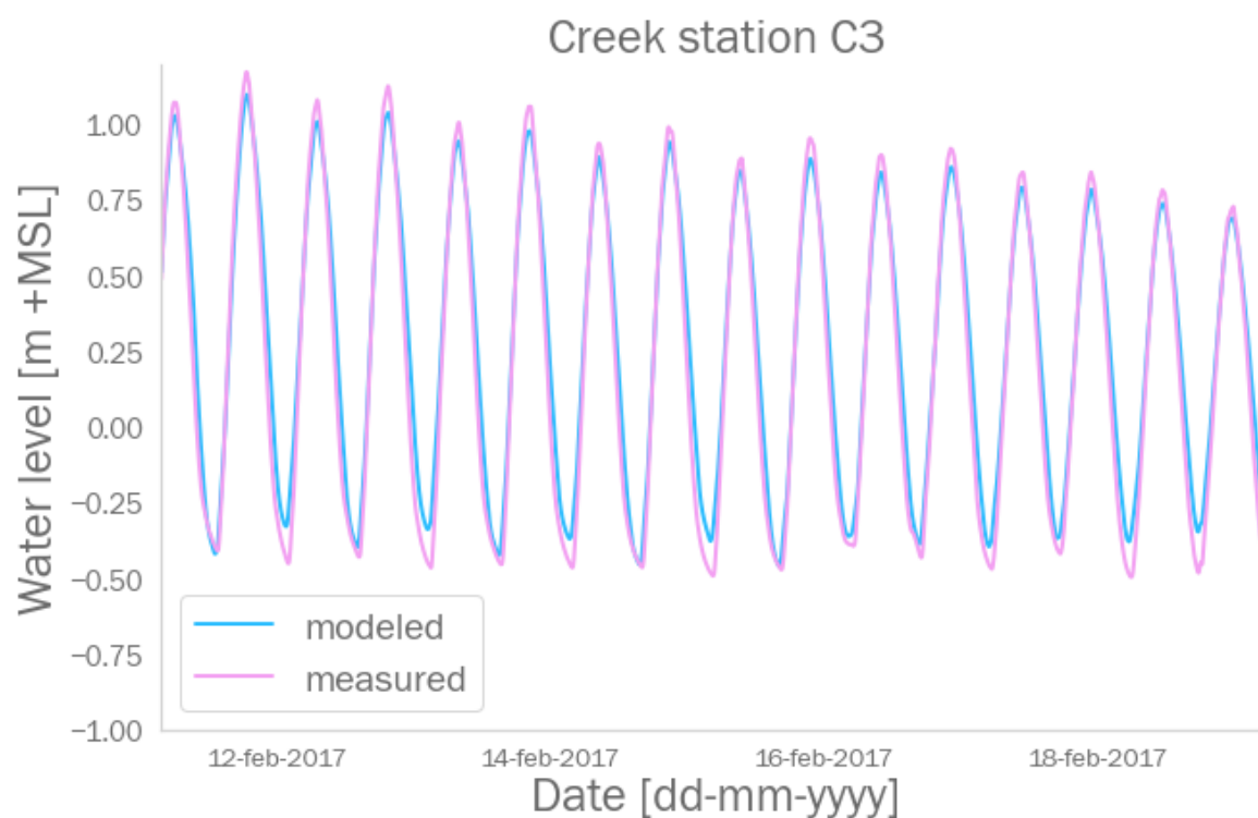
Figure A.11: Comparison between modeled and measured water levels at creek station C3
