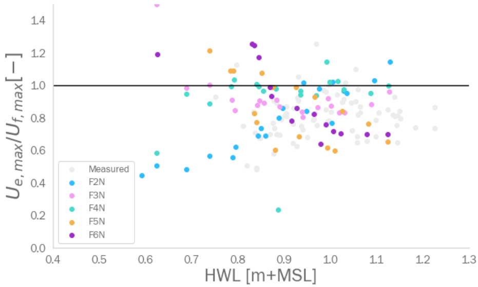
Figure 6.6: Ratio between simulated maximum ebb and flood flow velocity at the forest stations using a roughness raster
