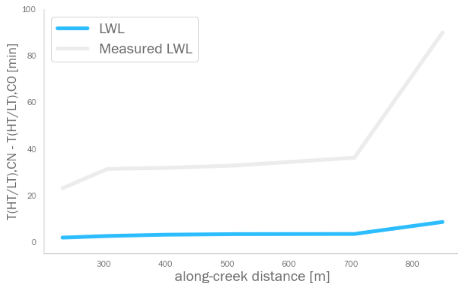
Figure 6.10: Along creek delay of tidal low- water levels using an interflow layer
