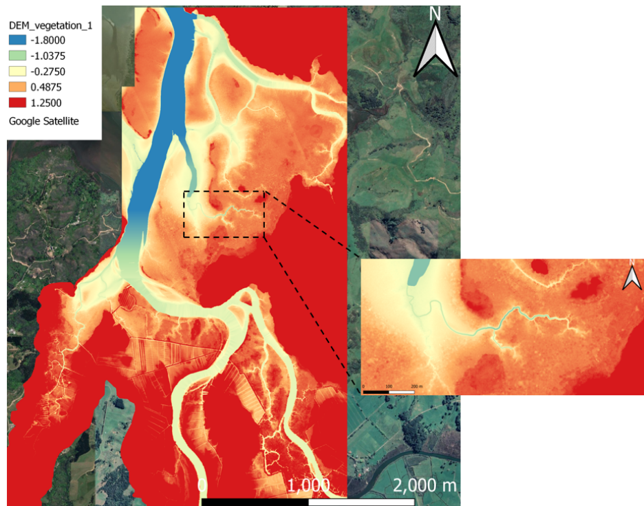
Figure 5.3: DEM after reconstructing lower elevations, elevation given in m+MSL
