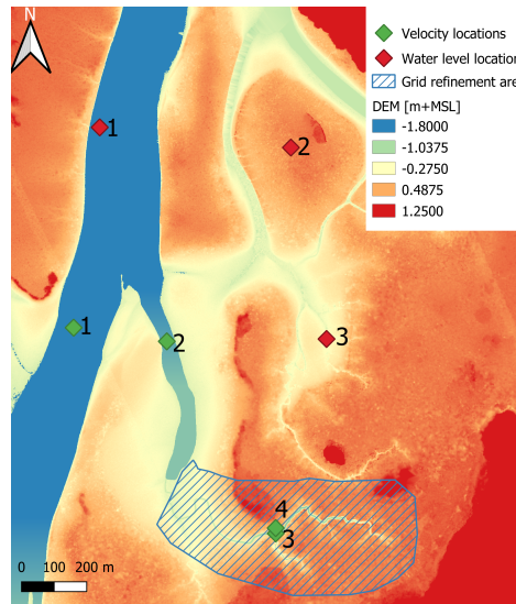
Figure 5.4: Locations where water levels and flow velocities will be compared in a sensitivity analysis on the effects of varying grid sizes on model predictions. In the blue shaded area, the smaller computational grid will be applied.
