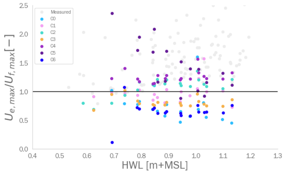
Figure 6.12: Ratio between maximum ebb and flood flow velocity at the creek stations, modeled using an interflow layer
