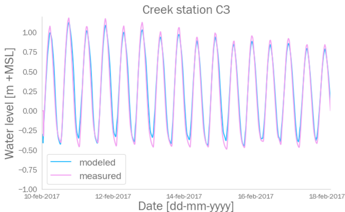
Figure A.4: Comparison between modeled and measured water levels at creek station C3
