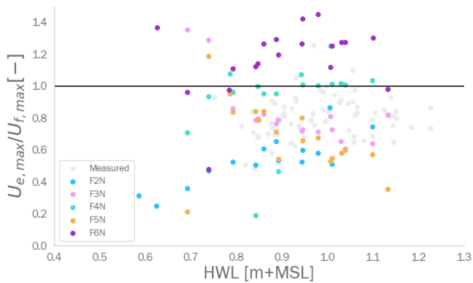
Figure 6.13: Ratio between maximum ebb and flood flow velocities at the forest stations, modeled using an interflow layer
