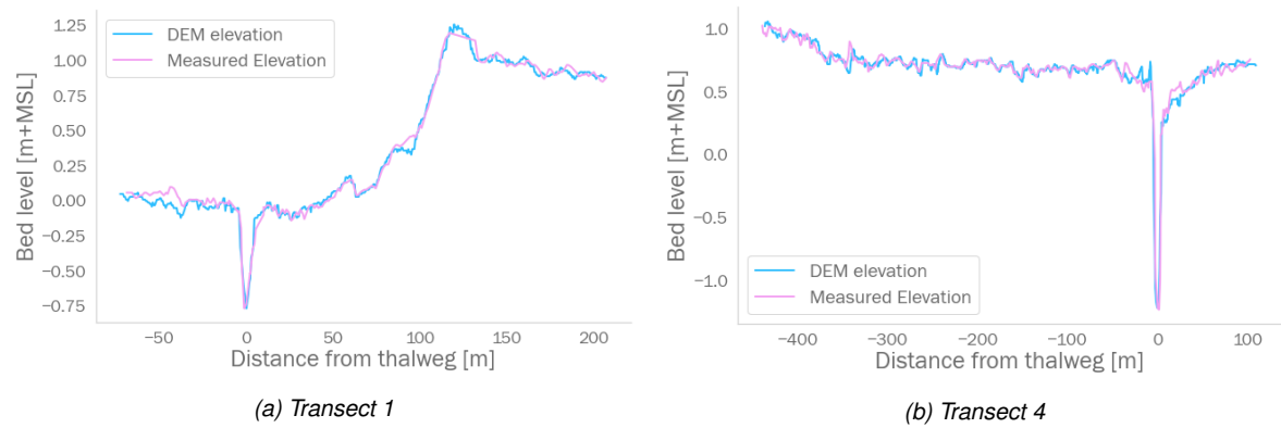
Figure 5.2: Comparison of the measured and the constructed elevation, as used in the DEM. Along two transects
