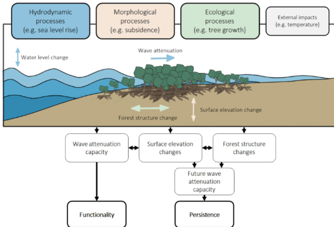
Figure 2.2: Interaction between hydrodynamic, morphological and ecological processes in mangroves (Gijssman et al., 2021)
