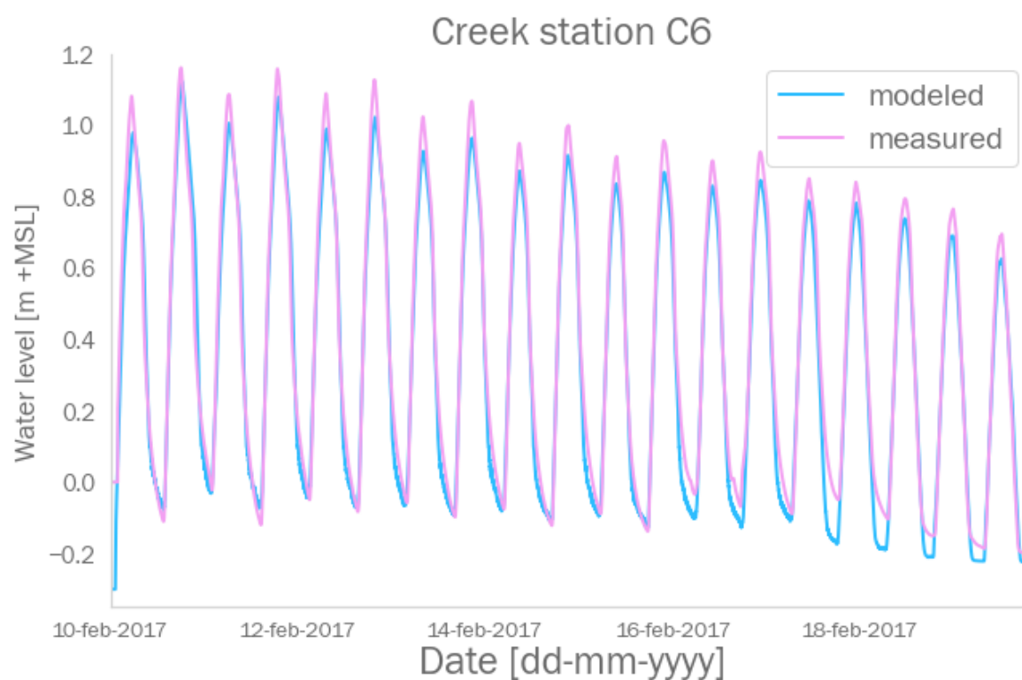
Figure A.7: Comparison between modeled and measured water levels at creek station C6
