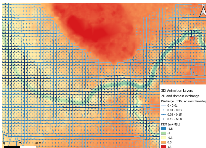
Figure 7.2: Flow routing using a calibrated roughness raster during ebb-tide on 14 February 2017
