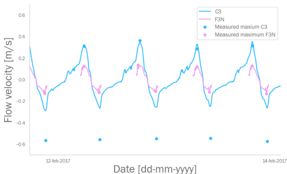
Figure 6.11: Modeled flow velocities at stations C3 and F3N, using an interflow layer
