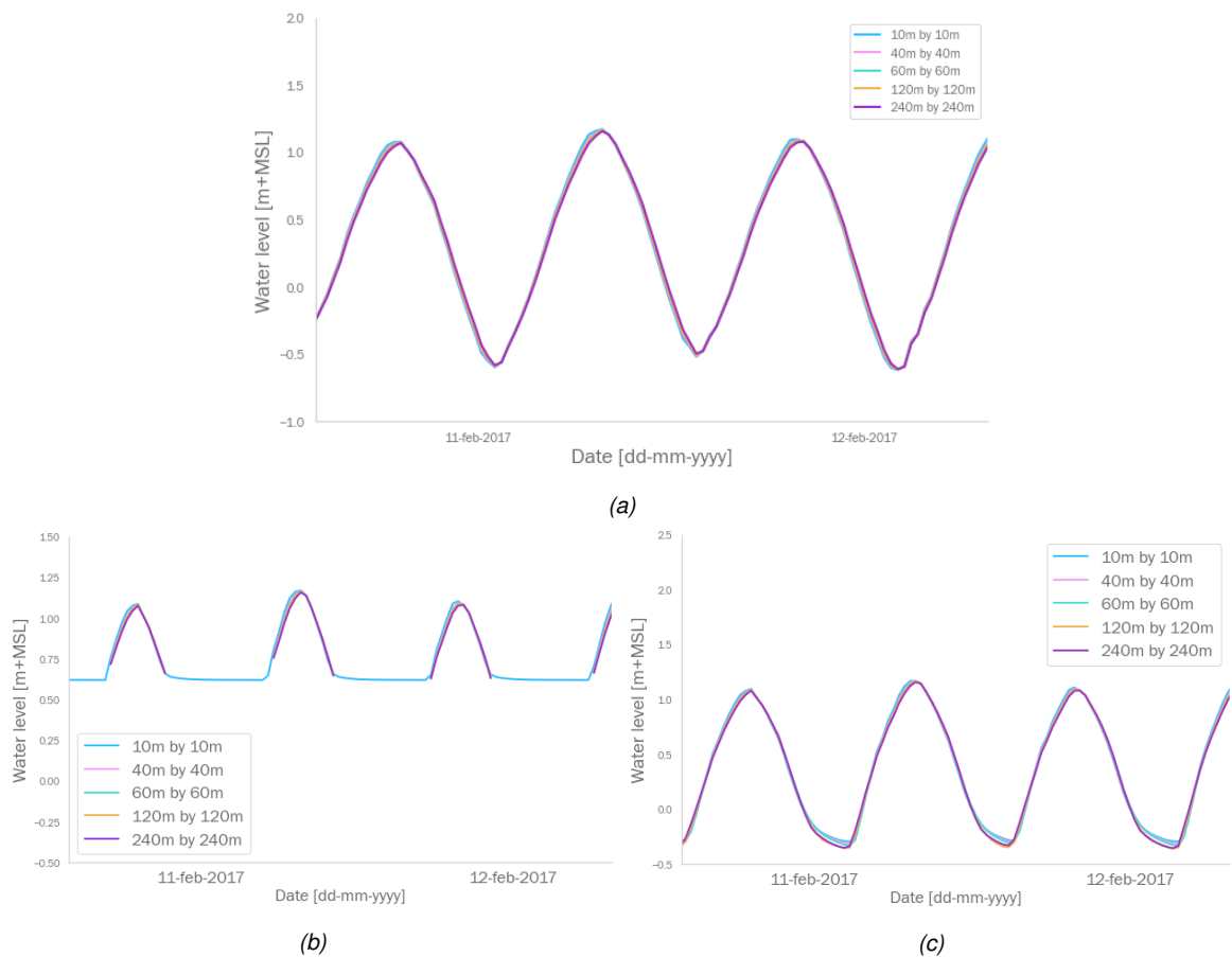
Figure 5.5: Sensitivity analysis of the water levels on varying grid sizes. (a) Location 1 (b) Location 2 and (c) Location 3 in figure 5.4
