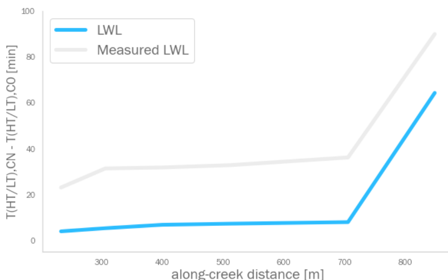
Figure 6.4: Along creek delay of the LWL, modeled using a roughness raster
