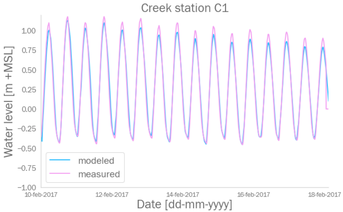
Figure A.2: Comparison between modeled and measured water levels at creek station C1
