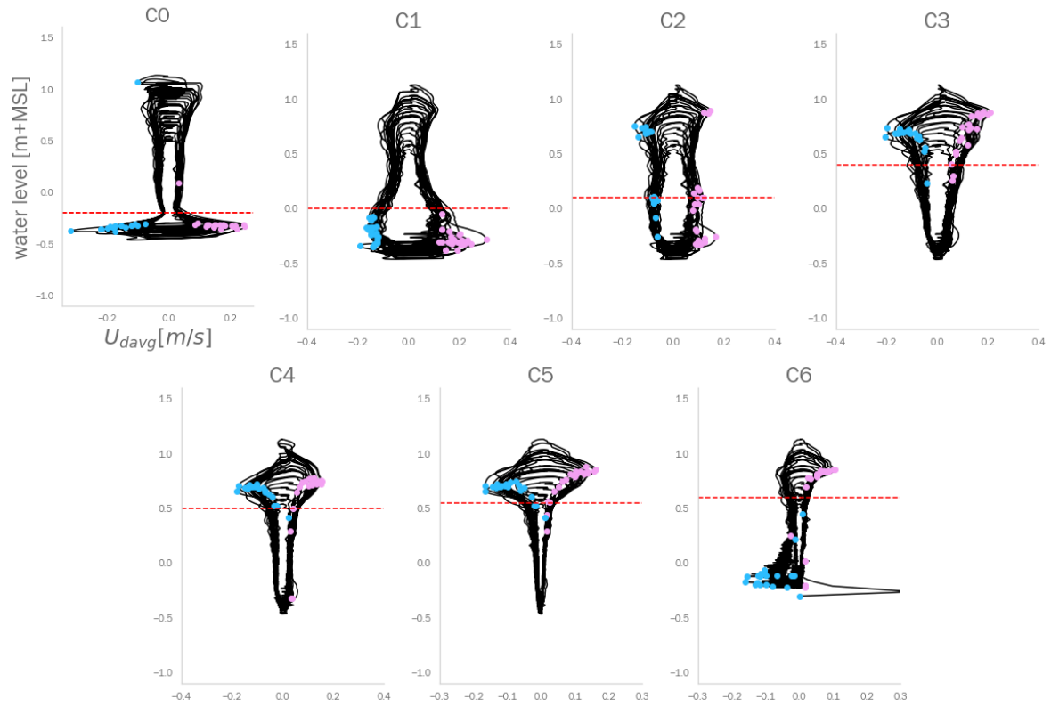
Figure B.6: Simulated tidal flow-stage velocity curves for all creek stations, blue and pink dots indicate maximum ebb and flood tidal velocities during each individual tide. Modeled using the base-case model
