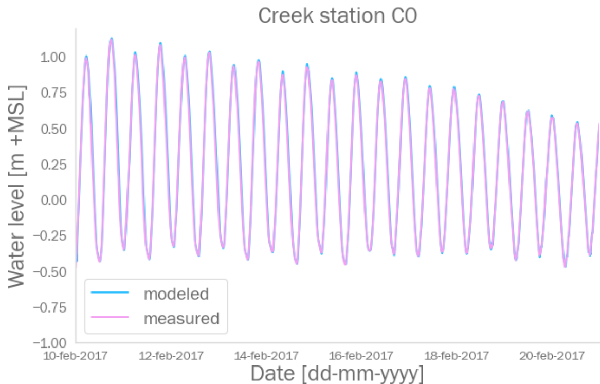
Figure A.1: Comparison between modeled and measured water levels at creek station C0
