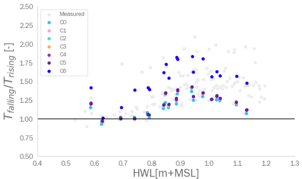
Figure B.1: Duration asymmetry at the creek stations modeled with the base-case model
