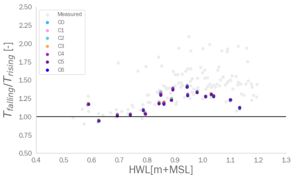
Figure 6.9: Duration asymmetry at the creek stations using an interflow layer
