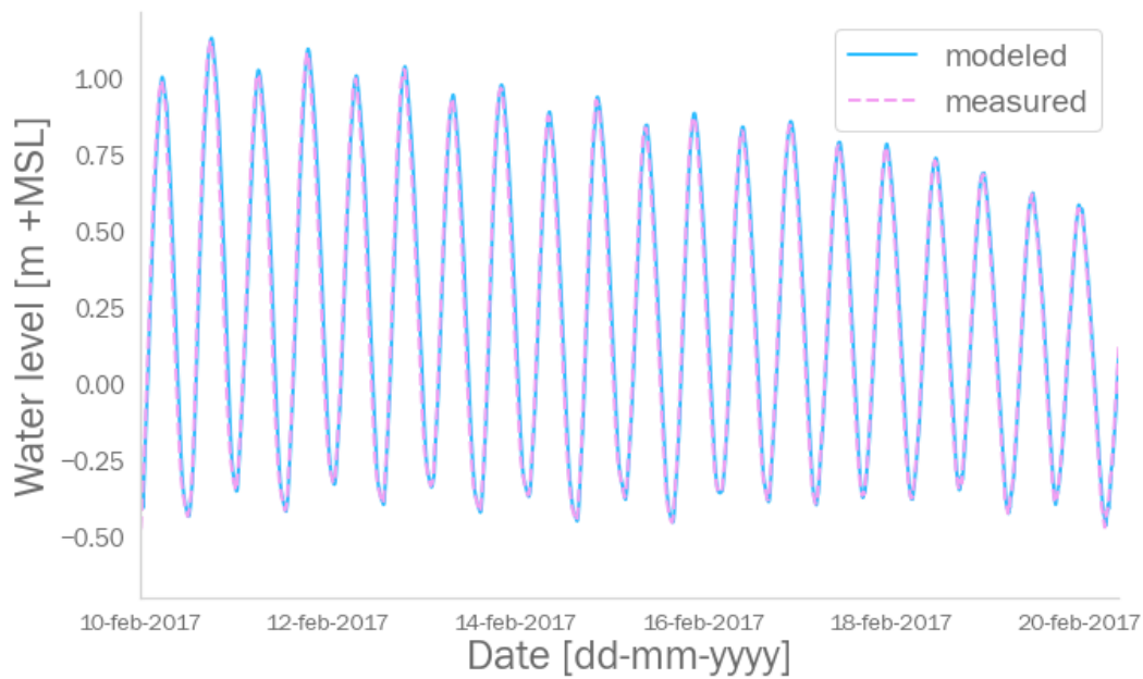
Figure 5.9: Modeled and measured water level time series after calibration of the boundary condition, retrieved at creek station C0
