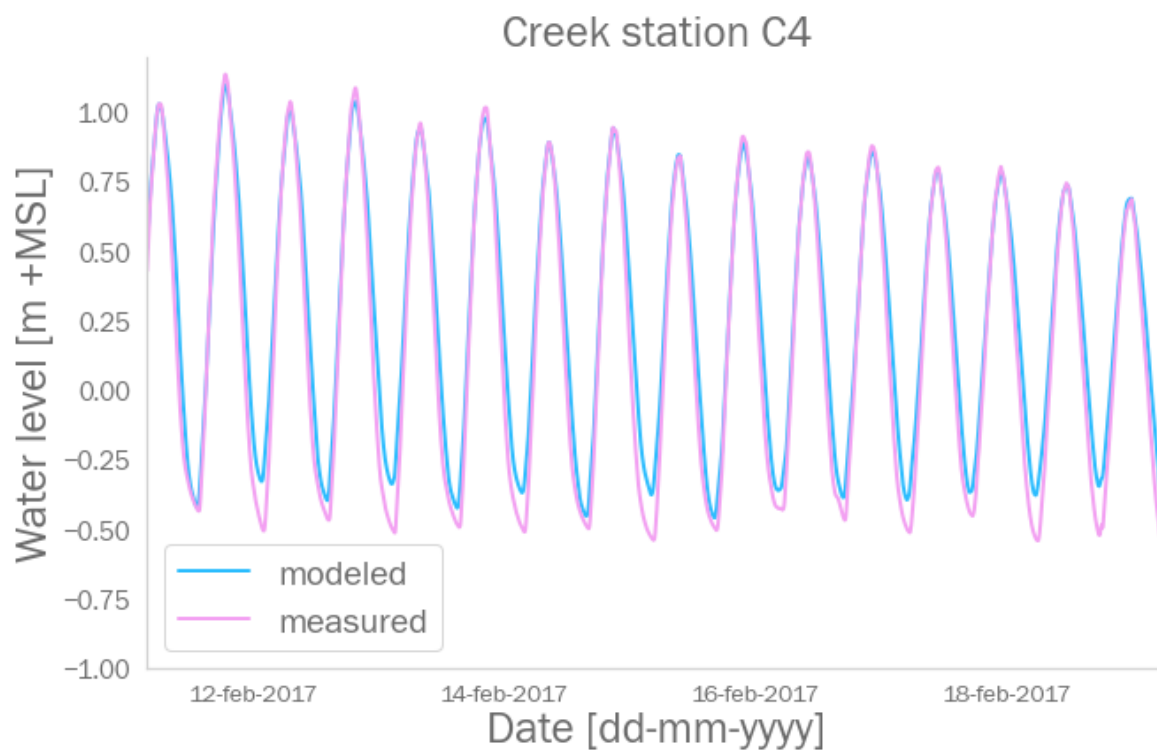
Figure A.12: Comparison between modeled and measured water levels at creek station C4
