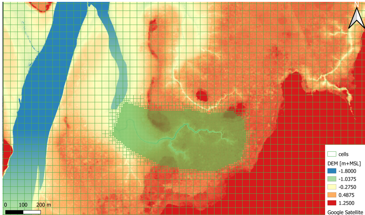
Figure 5.8: Computational grid used in the hydrodynamic model of the Whitianga estuary.
