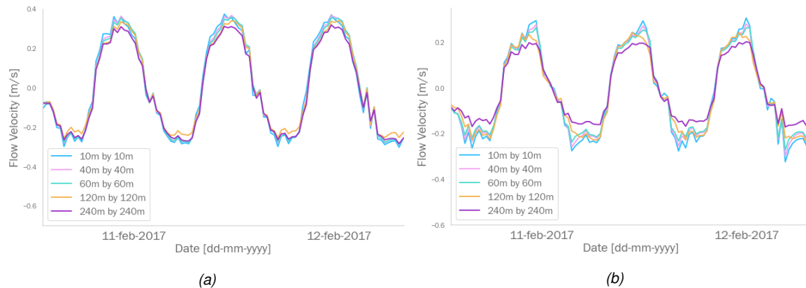
Figure 5.6: Sensitivity analysis of the flow velocities on varying grid sizes. (a) Location 1 and (b) Location 2 in figure 5.4
