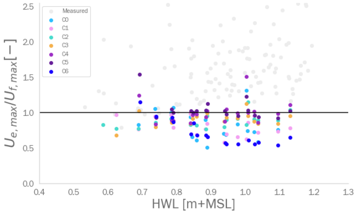
Figure B.5: Ratio between maximum ebb and flood flow velocities at the creek stations, modeled using the base-case model
