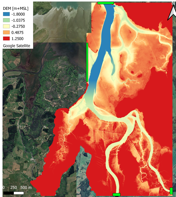
Figure 5.1: Model domain of the Whitianga Estuary. The green line on the north of the model domain is representing the location of the tidal boundary condition. The boundary on the west of the model domain is representing the location of the assumed natural flow boundary. On the south and southeast of the model domain the closed boundary upstream of the river is shown with the green lines
