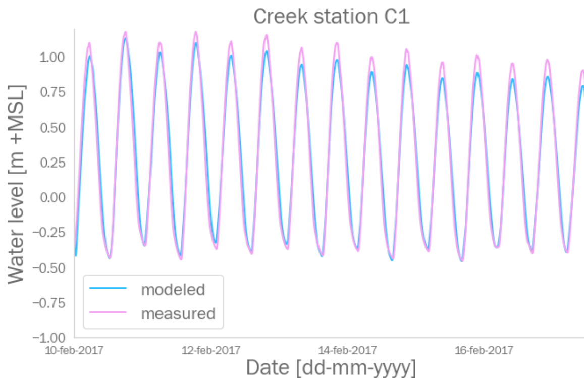
Figure A.9: Comparison between modeled and measured water levels at creek station C1
