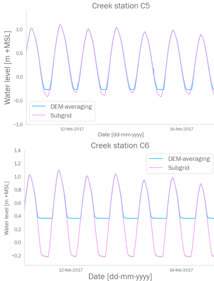
Figure 5.10: Comparison of the water level at creek stations C5 and C6 between a simulation including subgrid and a simulation excluding subgrid
