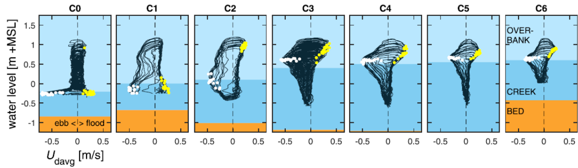
Figure 3.6: Tidal flow-stage curves for the different creek stations from Horstman et al. (2021). With the white dots being the maximum ebb flow velocities and the yellow dots being the maximum flood flow velocities during each tide
