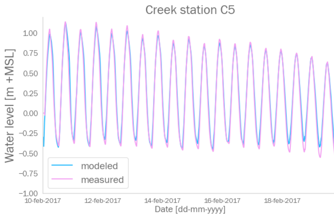
Figure A.6: Comparison between modeled and measured water levels at creek station C5
