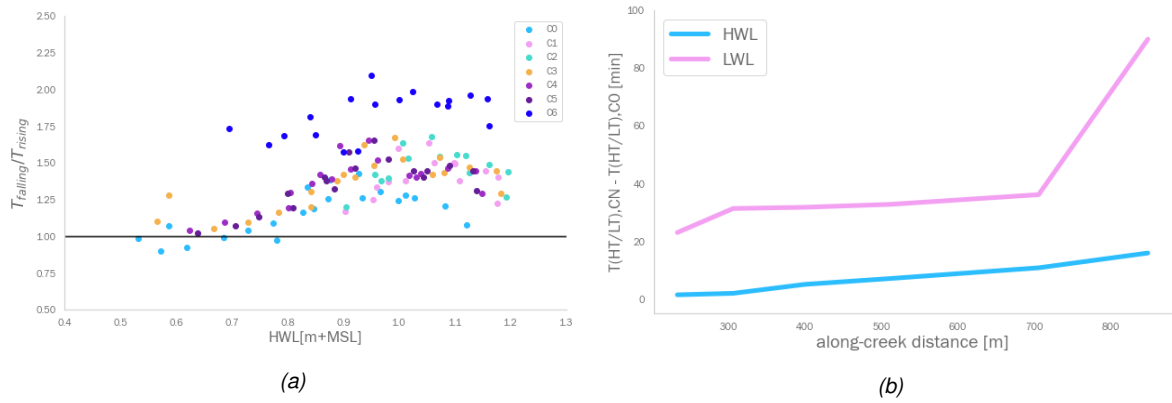
Figure 3.4: (a) Measured duration asymmetry at the creek stations (b) Measured along creek delay of the HWL and LWL in relation to creek station C0
