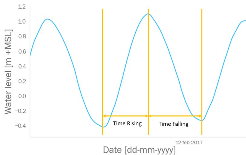
Figure 4.1: Schematization of the duration asymmetry
