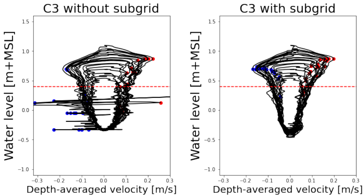
Figure 5.11: Comparison of the tidal flow-stage curves of a simulation including subgrid and a simulation excluding subgrid
