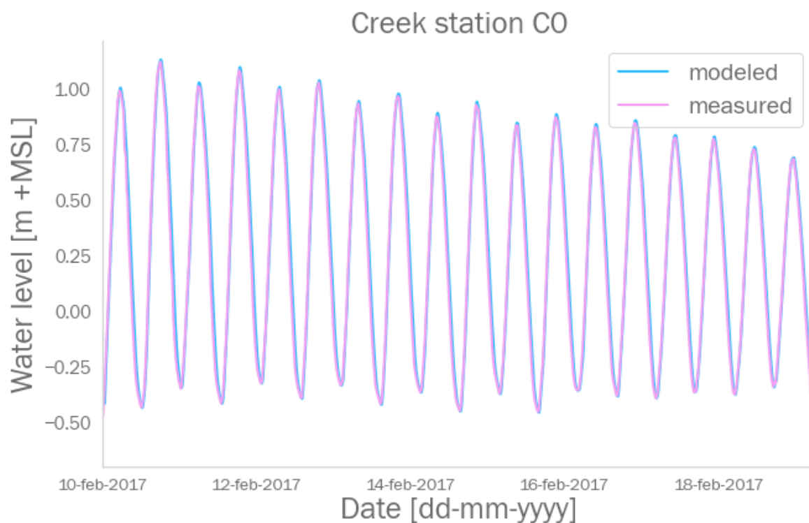
Figure A.8: Comparison between modeled and measured water levels at creek station C0
