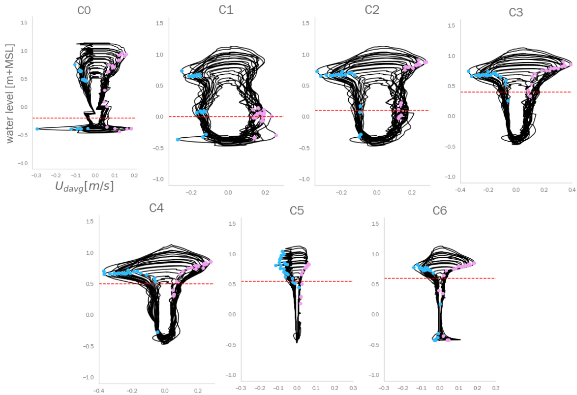
Figure 6.8: Simulated tidal flow-stage velocity curves for all creek stations, blue and pink dots indicate maximum ebb and flood tidal velocities during each individual tide. Modeled using an interflow layer
