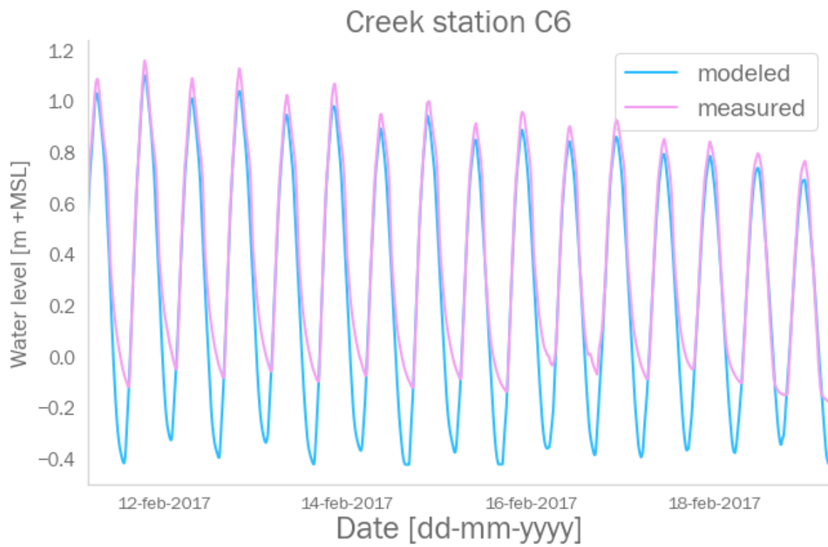
Figure A.14: Comparison between modeled and measured water levels at creek station C6
