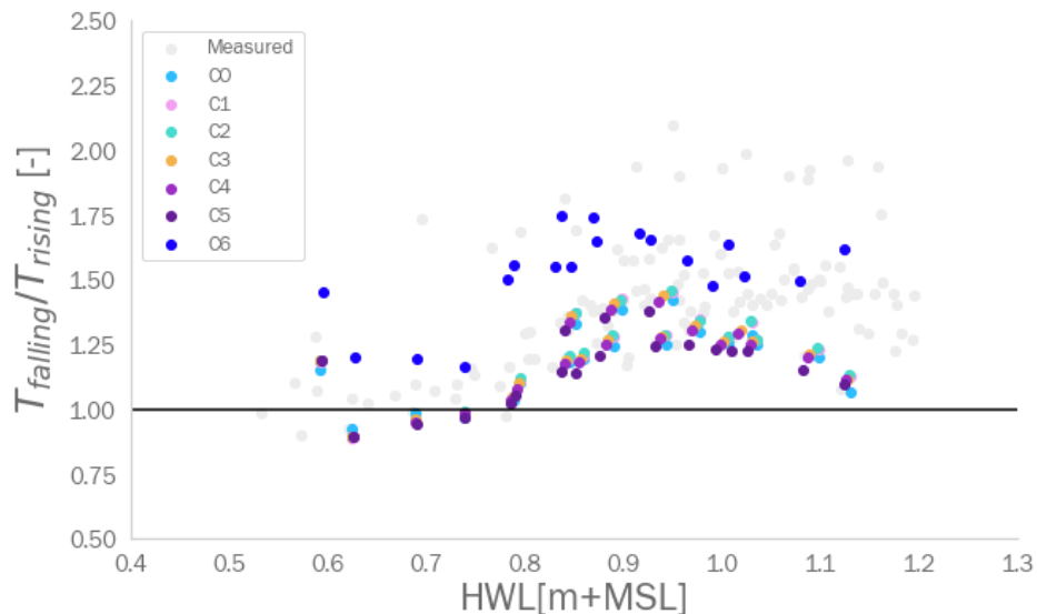
Figure 6.3: Duration asymmetry of the simulated tidal dynamics at the creek stations. Modeled using a roughness raster
