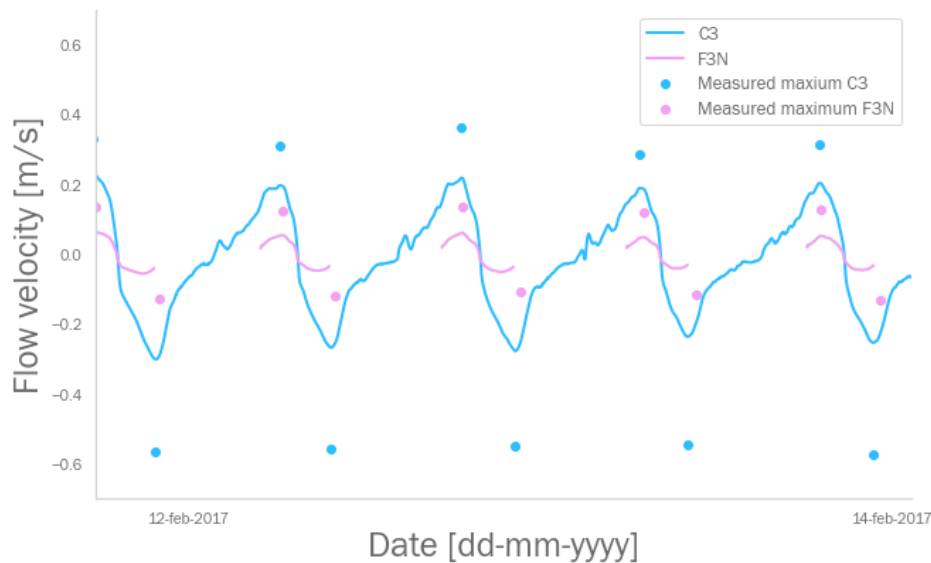
Figure 6.5: Flow velocity in creek station C3 and concurring forest station F3N, modeled using a roughness raster
