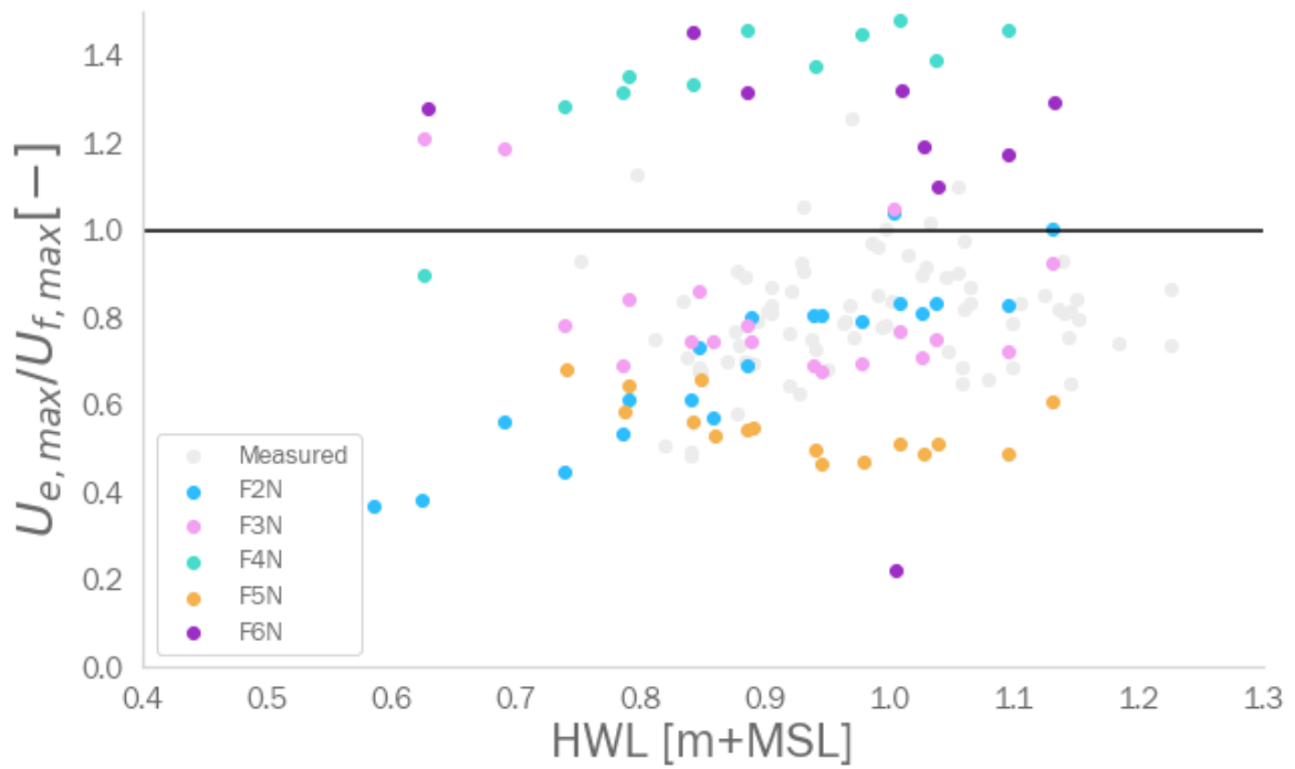
Figure B.4: Ratio between maximum ebb and flood flow velocities at the forest stations, modeled using the base-case model
