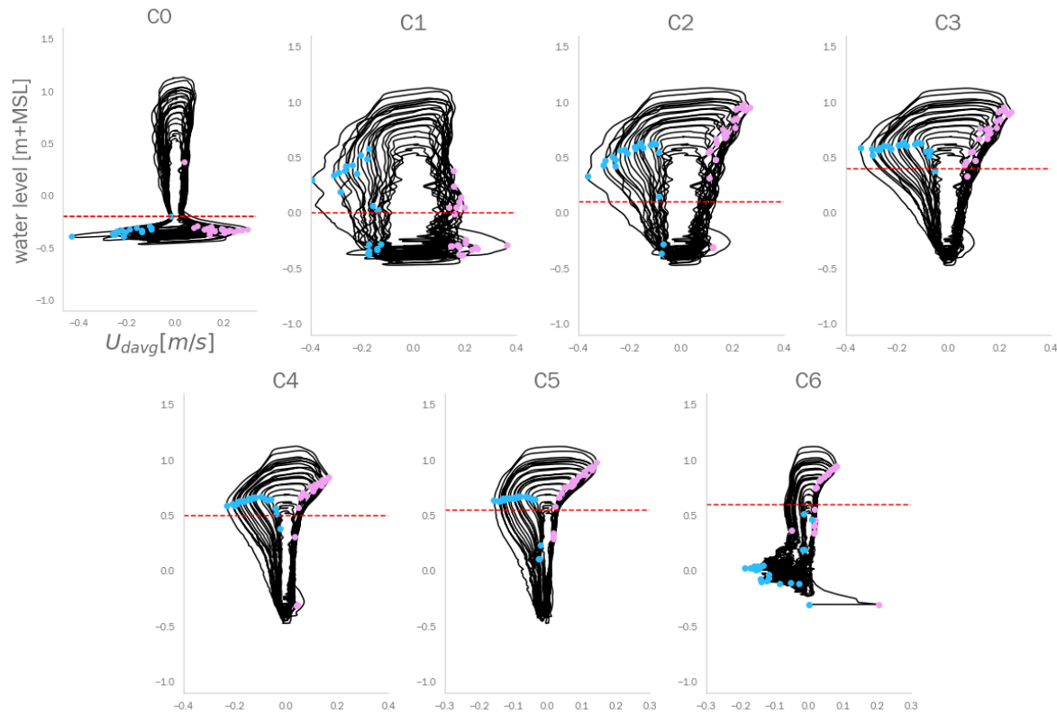
Figure 6.2: Simulated tidal flow-stage velocity curves for all creek stations, blue and pink dots indicate maximum ebb and flood tidal velocities during each individual tide. Modeled using a roughness raster.
