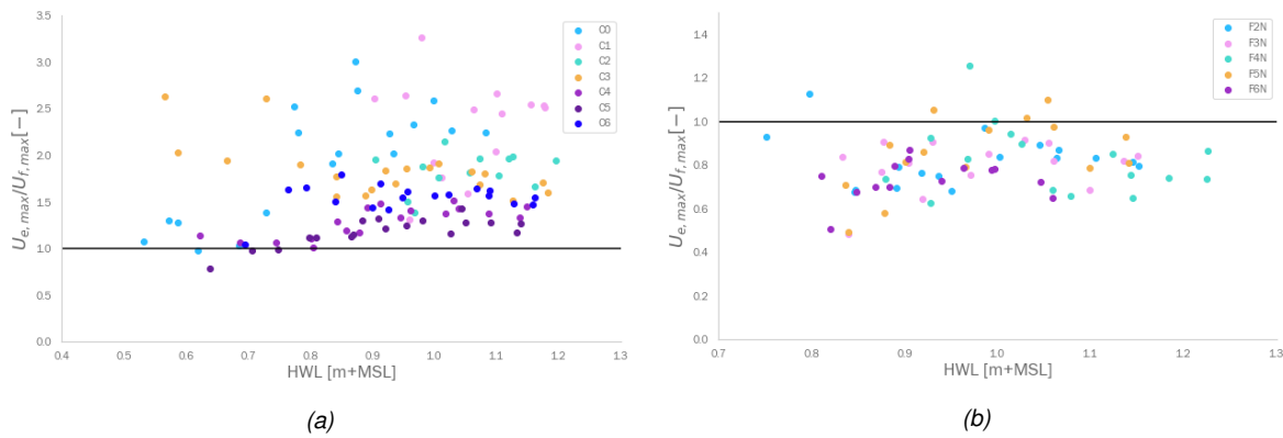
Figure 3.5: Measured tidal velocity asymmetry at (a) the creek stations and (b) the forest stations
