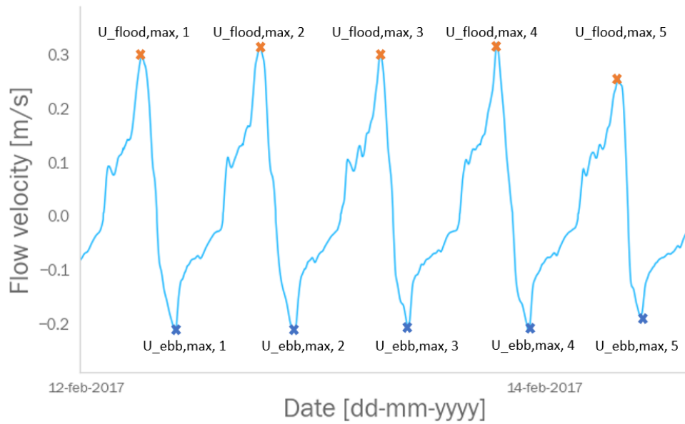
Figure 4.2: Schematization of the velocity asymmetry
