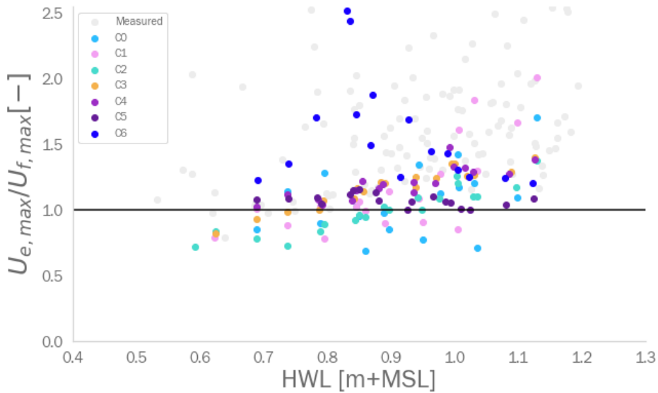
Figure 6.7: Ratio between simulated maximum ebb and flood flow velocities at the creek stations using a roughness raster
