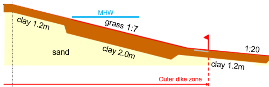
Figure 12. Wide green dike design (adapted from van Loon-Steensma & Schelfhout (2013))
