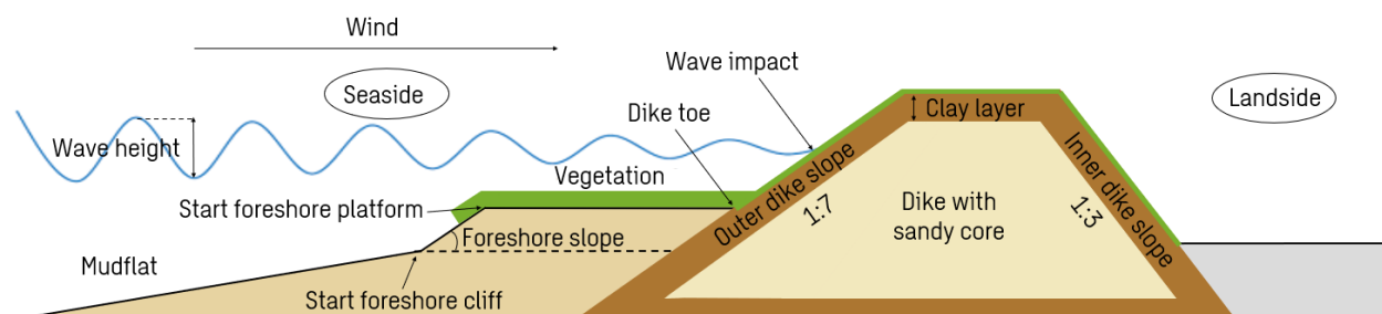
Figure 7. Dike geometry with vegetated foreshore under storm conditions
