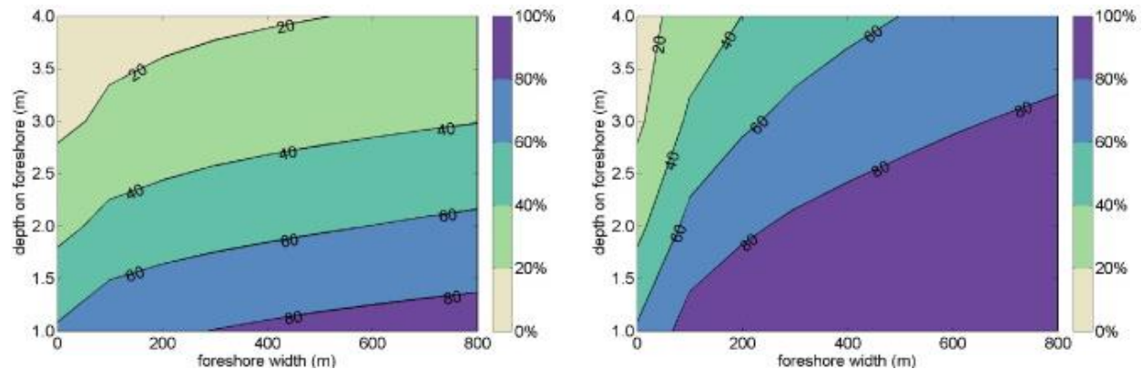
Figure 27. Reduction of significant wave height in case of water depth and width on/off the foreshore. Left panel; foreshore without vegetation, right panel; foreshore with vegetation (Vuik et al., 2016)
