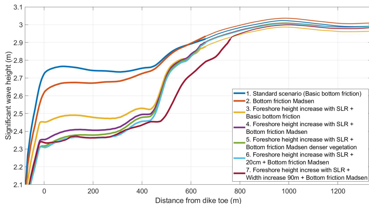
Figure 31. Results scenario analysis erosion
