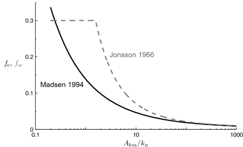
Figure 37. Madsen vs Jonsson bottom friction (Humbyrd & Madsen, 2011)
