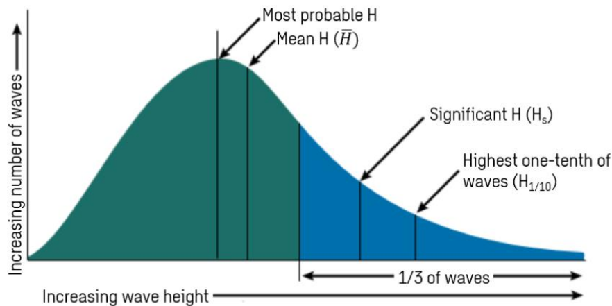
Figure 13. Significant wave height distribution (Collins, 2014)
