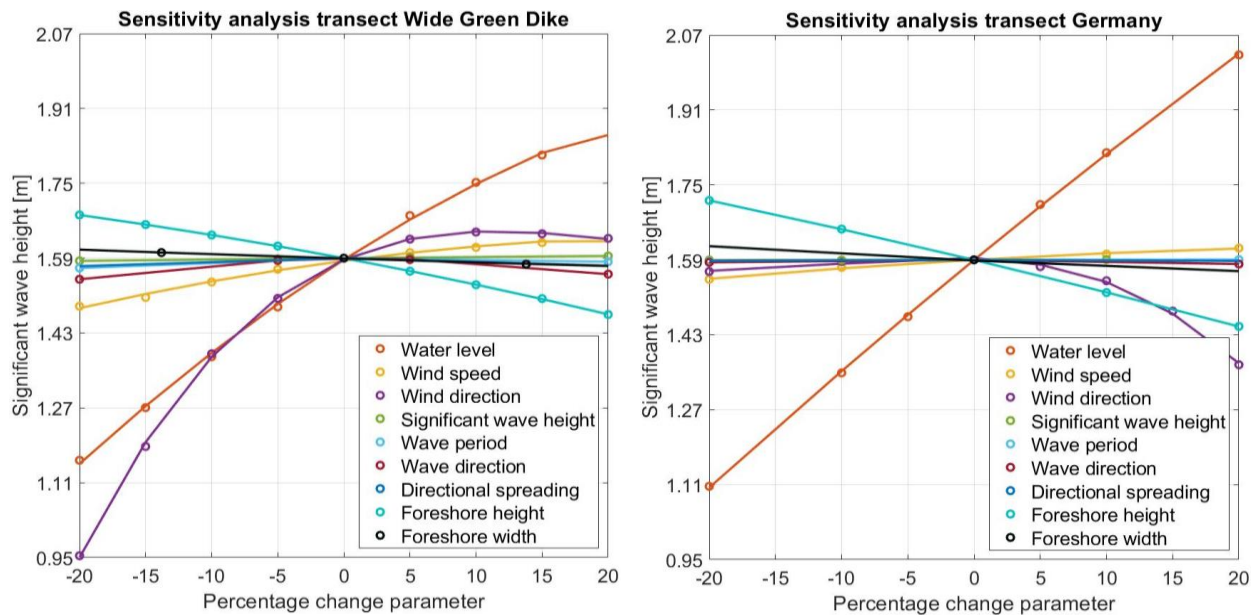
Figure 21. Results sensitivity analysis
