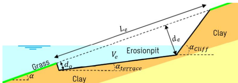
Figure 29. Erosion profile with dimensions (adapted from van Steijn & Klein Breteler (2021))
