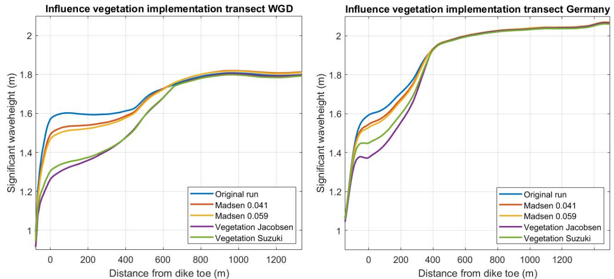
Figure 24. Results sensitivity analysis with implementation influence vegetation
