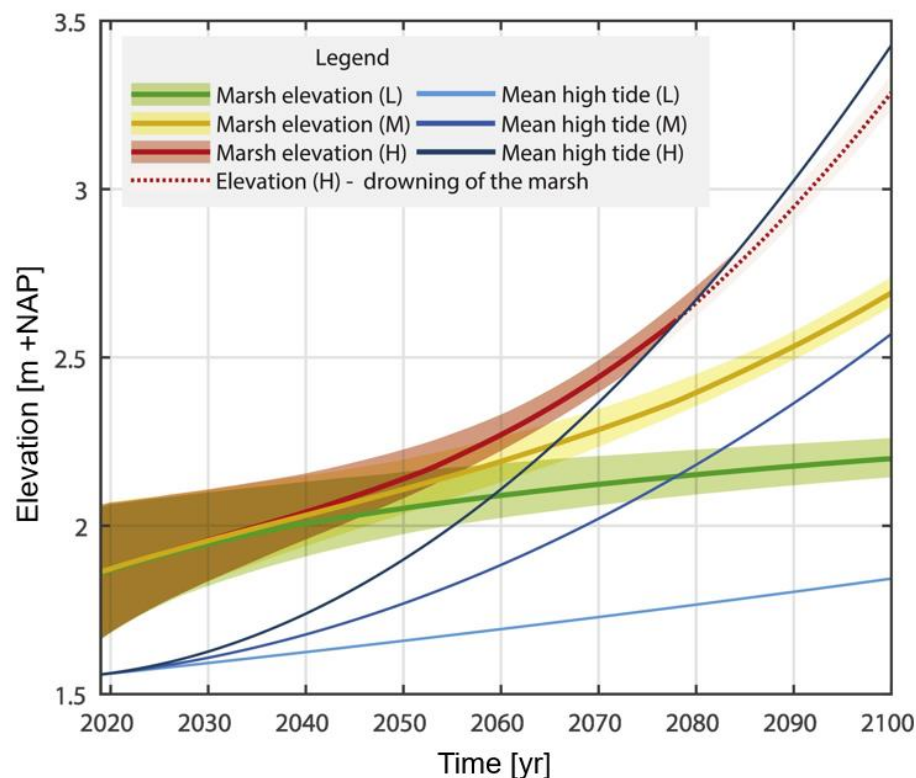
Figure 38. Development of the marsh elevation over time for different SLR scenarios (Marijnissen et al., 2020)
