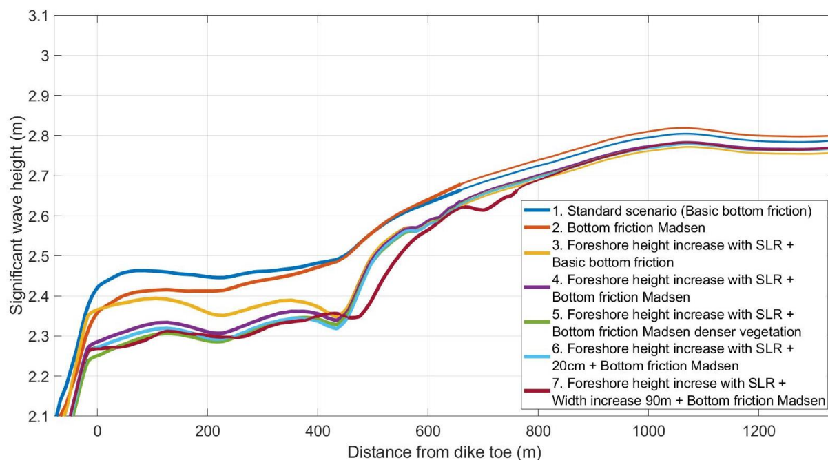
Figure 30. Results scenario analysis wave overtopping
