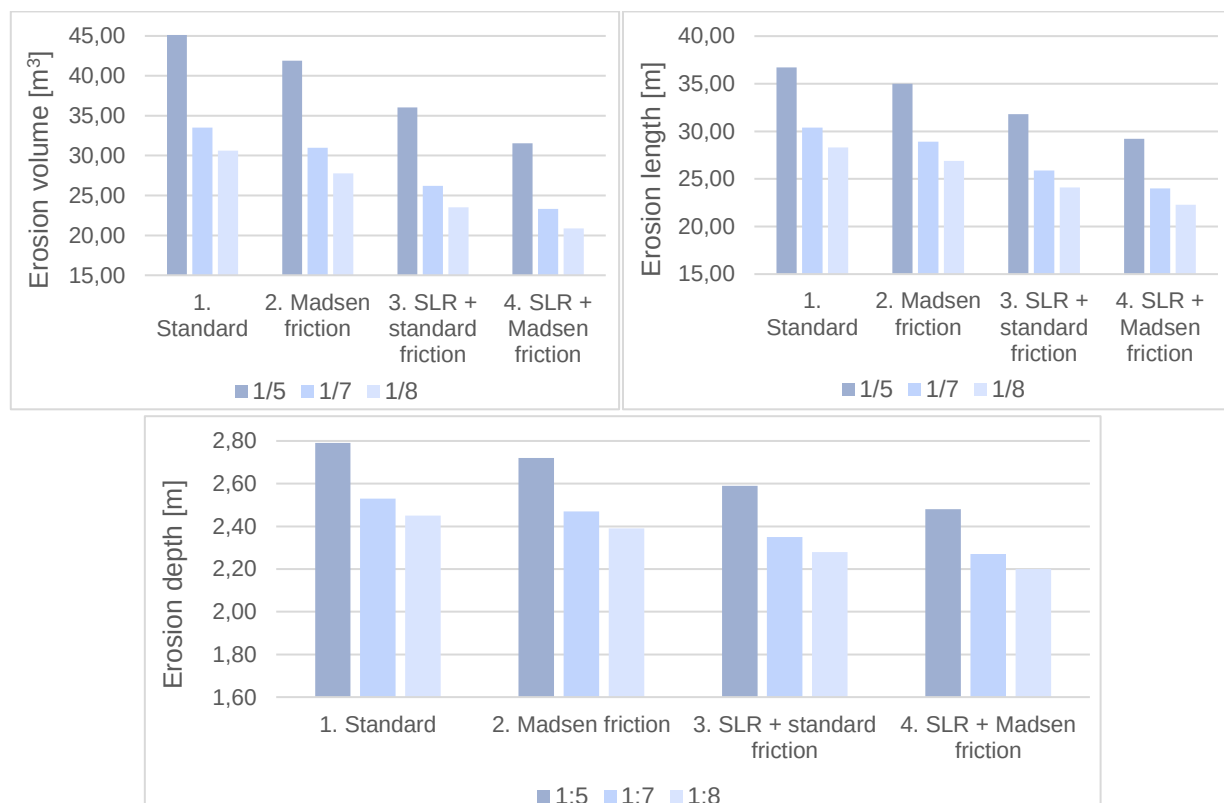
Figure 33. Results erosion hole and clay layer thickness for the different scenarios and dike slope
