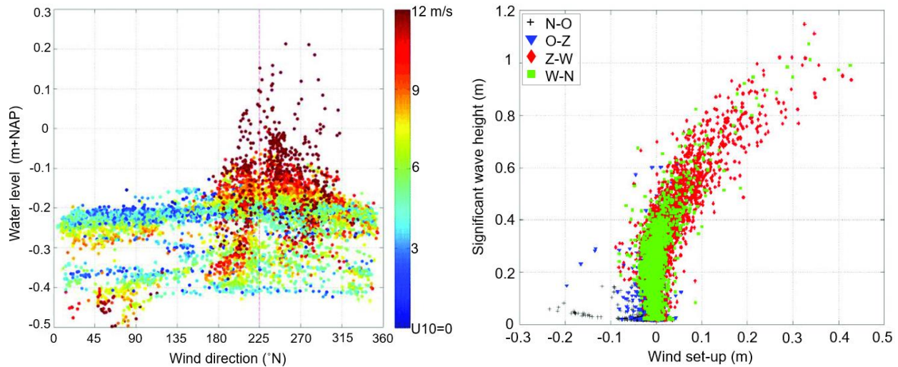
Figure 23. Relationship between wind speed and water level (left) and wind set-up and significant wave height (right) (Penning et al., 2016)
