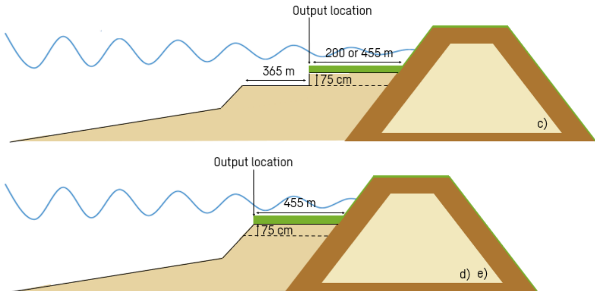
Figure 35. Visualisation of the different implementation methods; no inclusion of foreshore vegetation or increased height (a), use DaF module current approach (b), fictively increase foreshore width (c), replace output location in Hydra-NL whereafter implement the DaF module or a use separate SWAN model (d and e).
