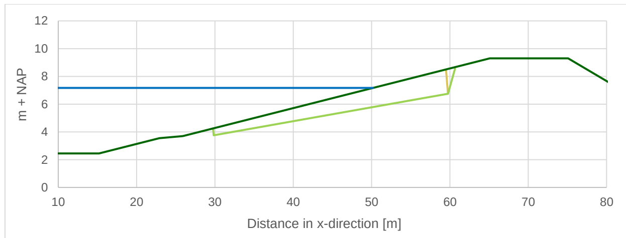
Figure 34. Erosion hole standard scenario and outer dike slope of 1:7
