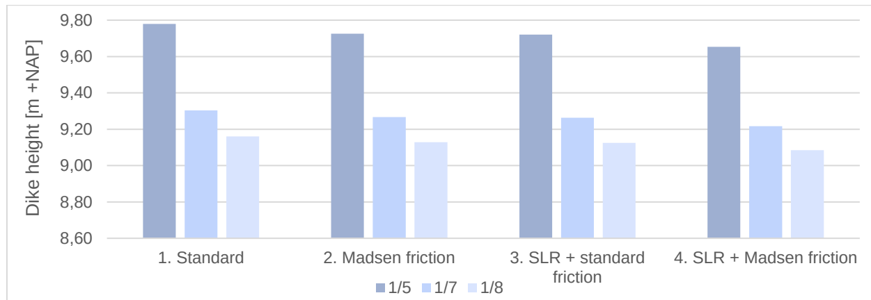
Figure 32. Dike height for wave overtopping for the different scenarios and dike slope
