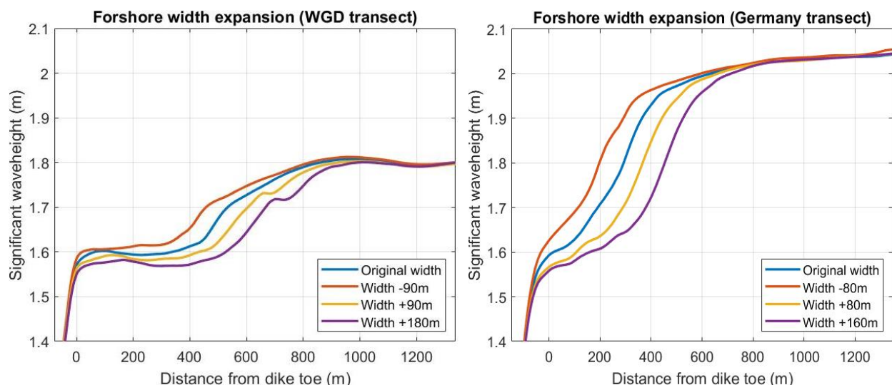
Figure 28. Significant wave height course for the two transects when including foreshore width expansion
