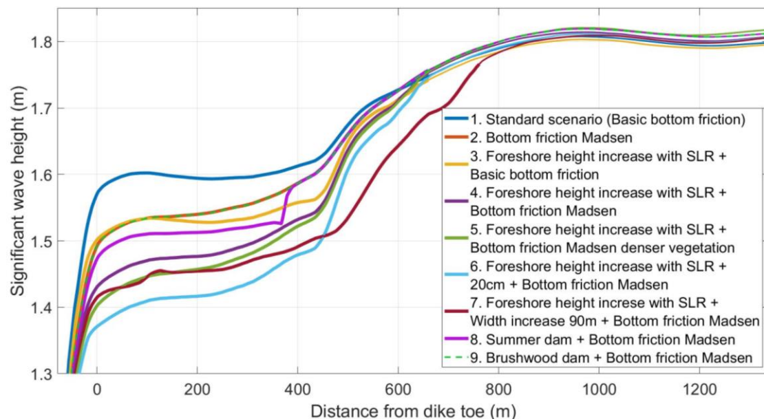
Figure 25. Results scenario analysis WGD transect for a normative storm of 1/3.000 year
