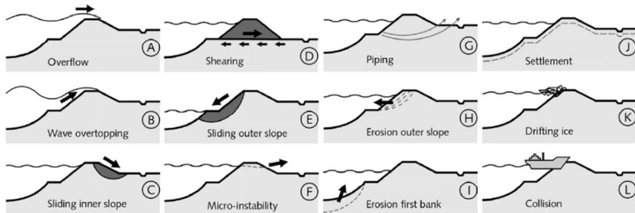
Figure 3. Failure mechanisms of soil structures (TAW, 1998)
