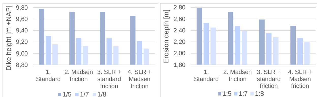
Figure 2. Required dike dimensions for different scenarios
