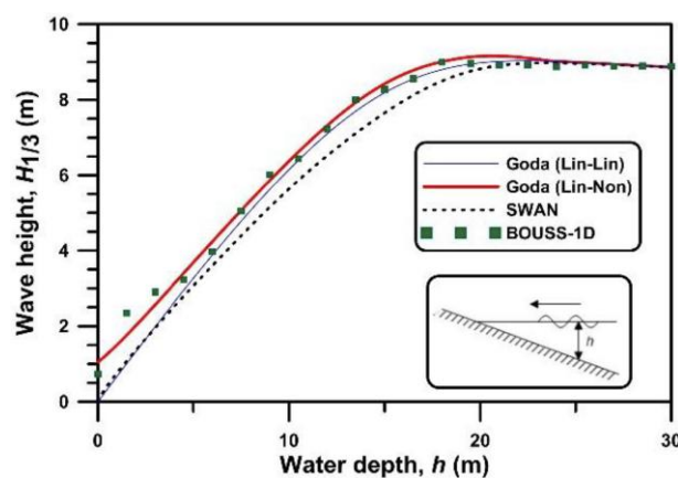
Figure 22. Water depth vs significant wave height (Kang et al., 2020)
