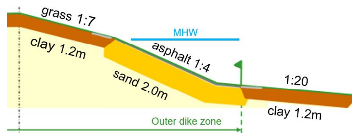
Figure 11. Current (traditional) dike design (adapted from van Loon-Steensma & Schelfhout (2013))
