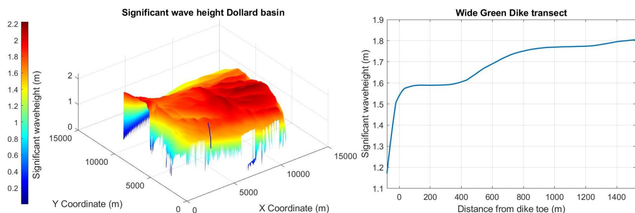
Figure 15. Significant wave height over Dollard basin (left) and cross-section WGD (right) for a 1/3.000 year storm
