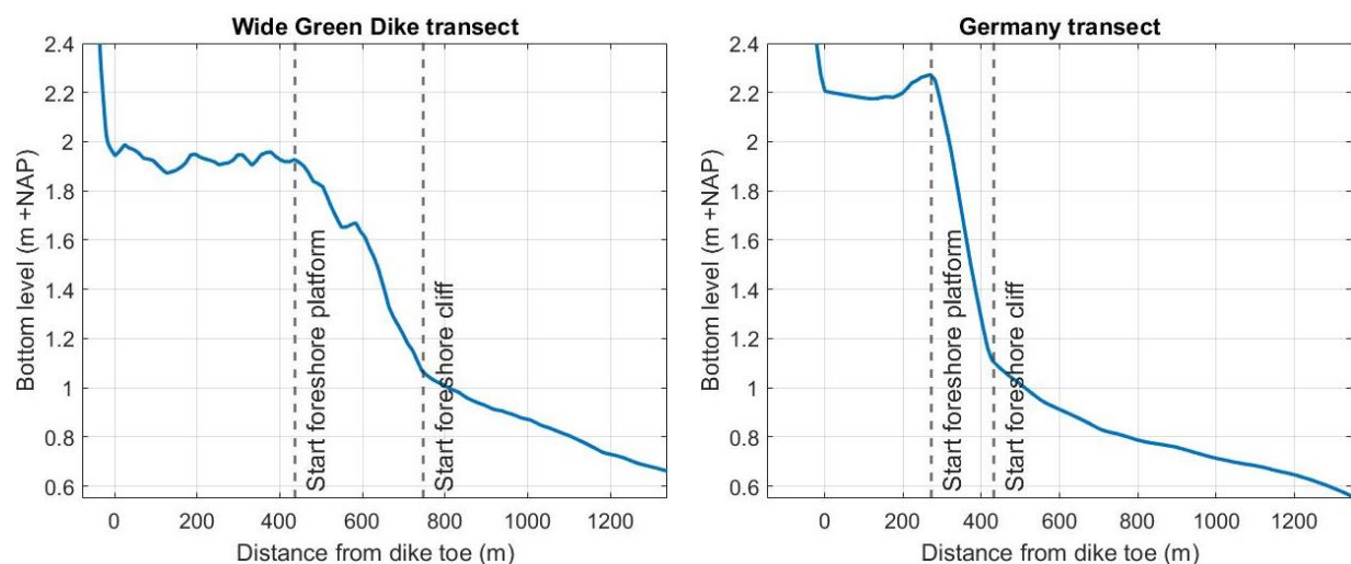
Figure 16. Bottom level different locations
