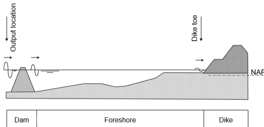
Figure 36. Schematisation Dam and Foreshore module Hydra-NL (Rijkswaterstaat, 2019)
