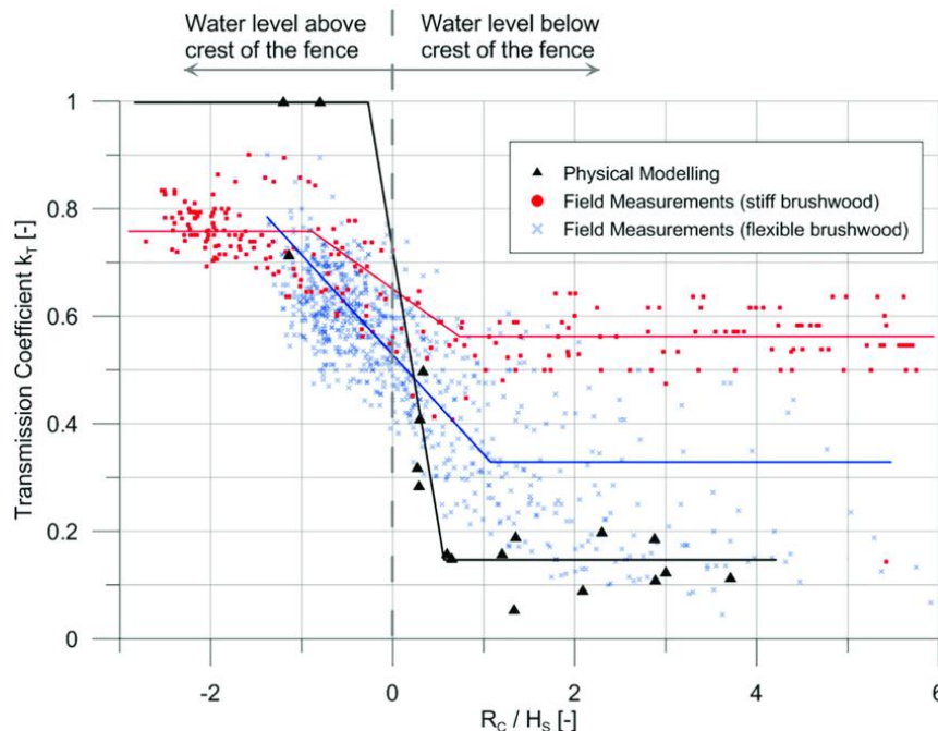
Figure 19. Wave transmission coefficients of bamboo fences under various hydrological conditions (Winterwerp et al. (2020) modified after Schmitt et al. (2013))
