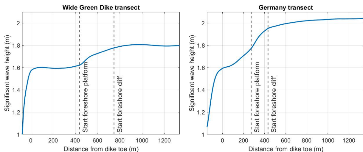
Figure 20. Significant wave height different locations
