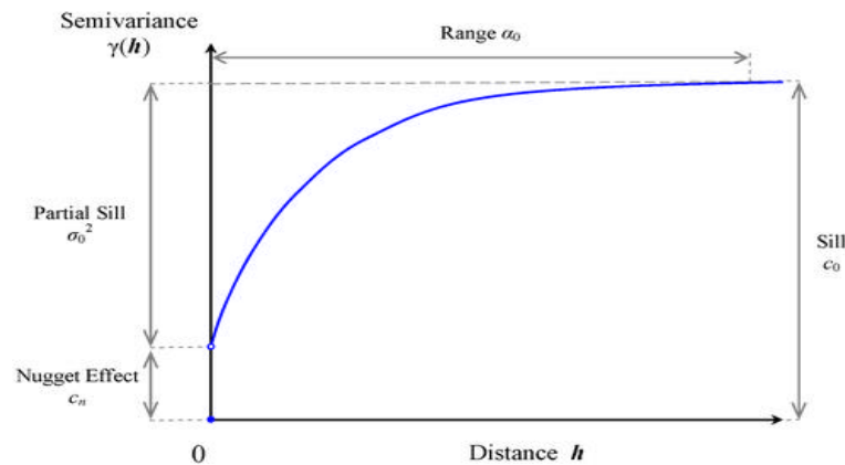
Figure 5: Variogram along with Lag distance (h)
