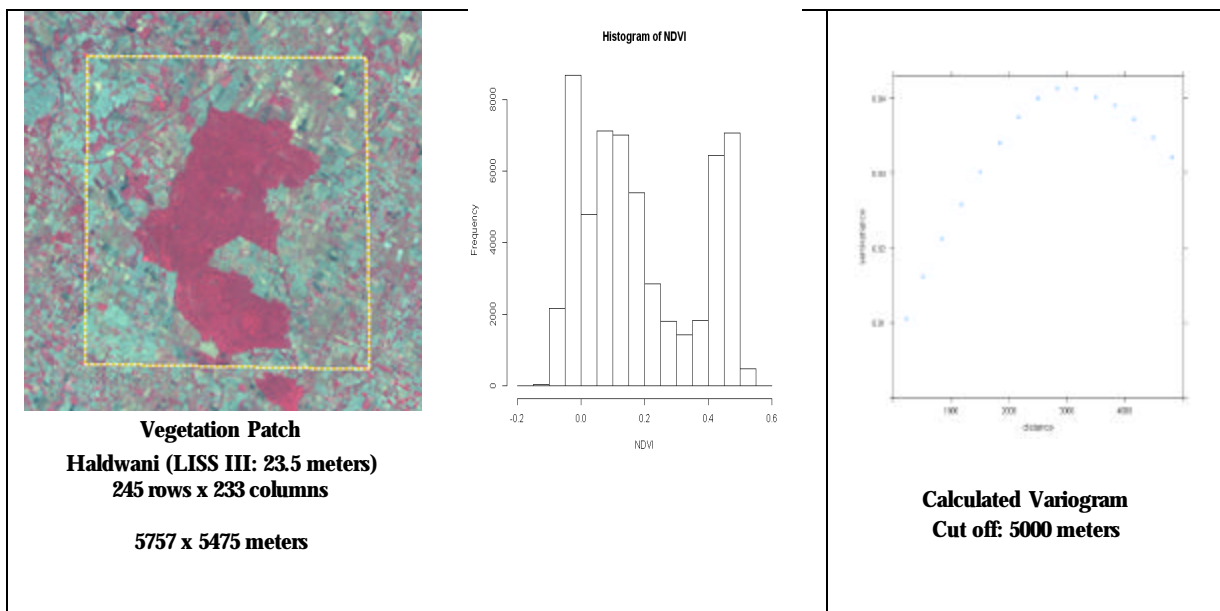
Figure 16 Variogram analysis of a vegetation patch on including non vegetation areas (Case B)
