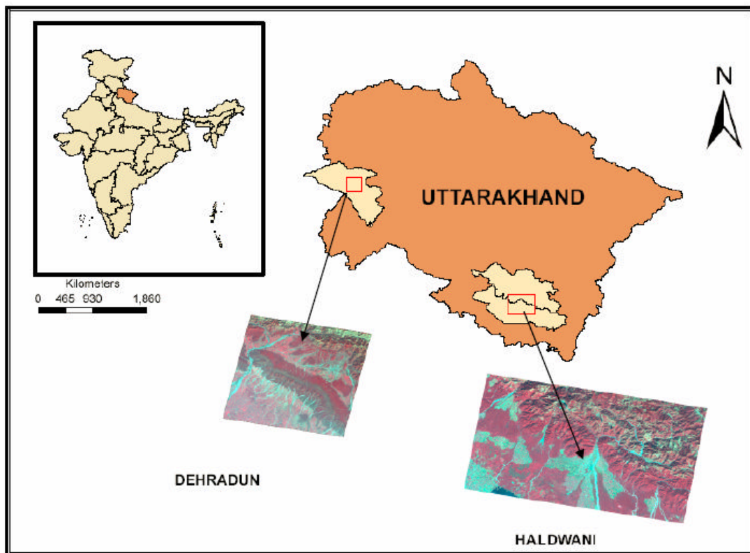
Figure 8: Study area: Dehradun and Haldwani
