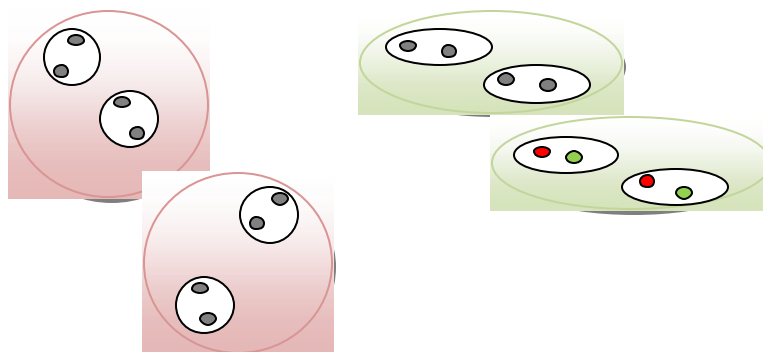
Figure 3: spatial correlation using variogram
