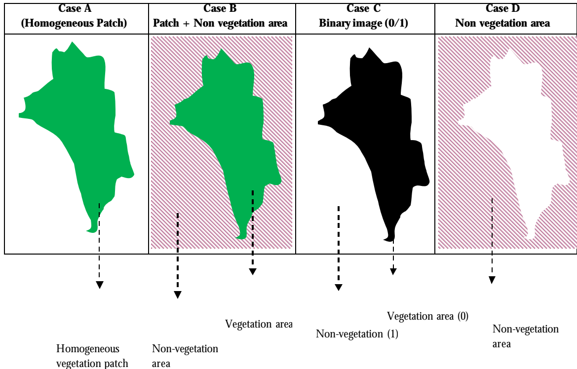
Figure 13: Explanation of different scenarios (Case A, B, C and D)
