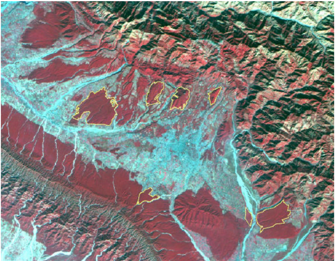
Figure 12: Selected vegetation patches in Dehradun area
