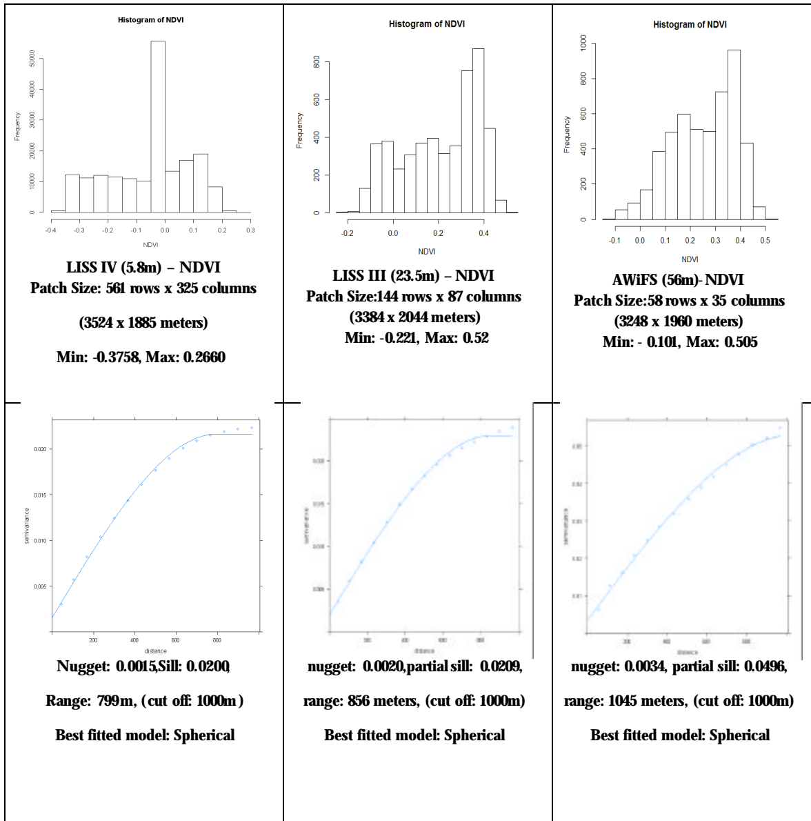
Figure 18 Histogram and Variogram estimation for a non-homogeneous patch (Case B) across different resolutions
