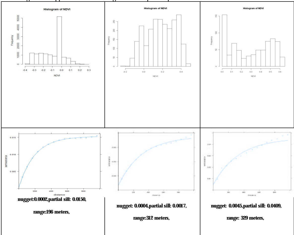
Figure 21: Histogram and Variogram estimations after excluding vegetation patch from NDVI image CaseD
