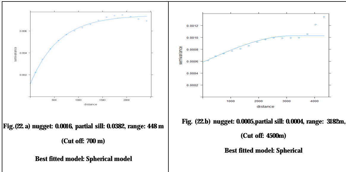
Figure 22: Comparison of variogram parameters for small and large size homogeneous vegetation patch (Case A)
