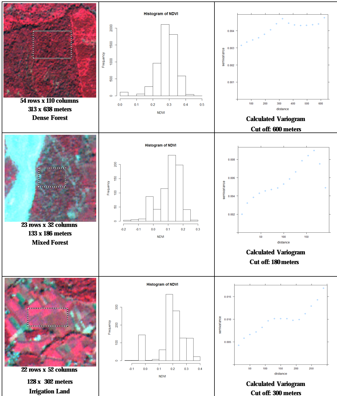
Figure 26 Variogram calculations for selected subsets of different vegetation types present in LISS IV, Haldwani area
