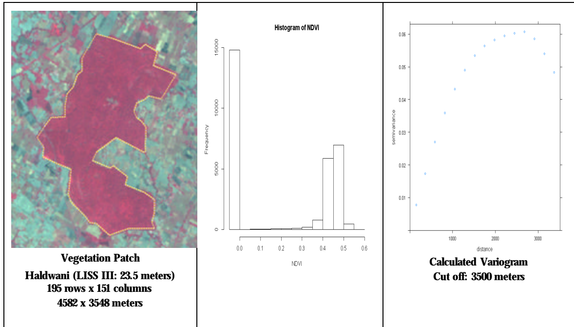
Figure 14: Spatial Structure of a vegetation patch using variogram analysis (Case A)
