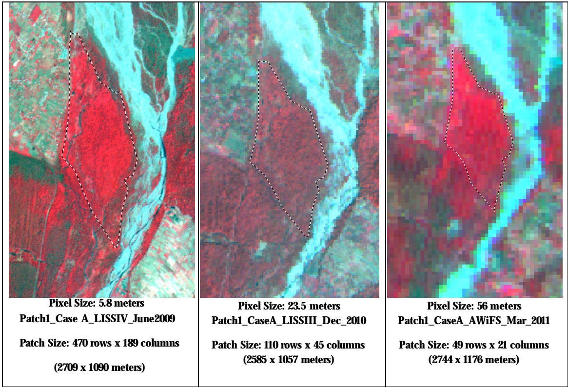
Figure15: Selected homogeneous vegetation patch (Case A) across different resolutions
