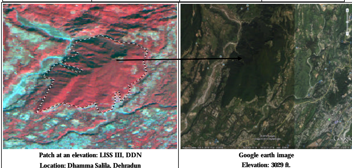
Figure 23 and Figure 24 representing variogram analysis for a patch located at an elevation of 3029 ft. in Dehradun area
