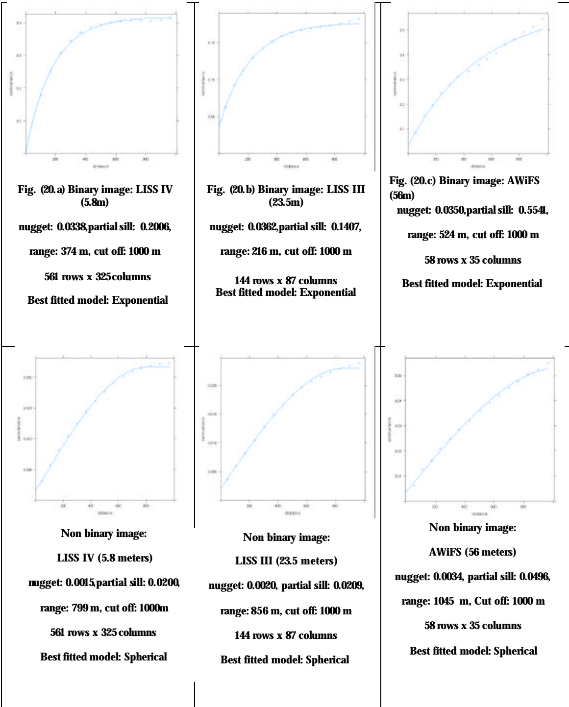
Figure 20 Comparison of variogram estimation for binary (Case C) and non binary images (Case B) at different resolutions
