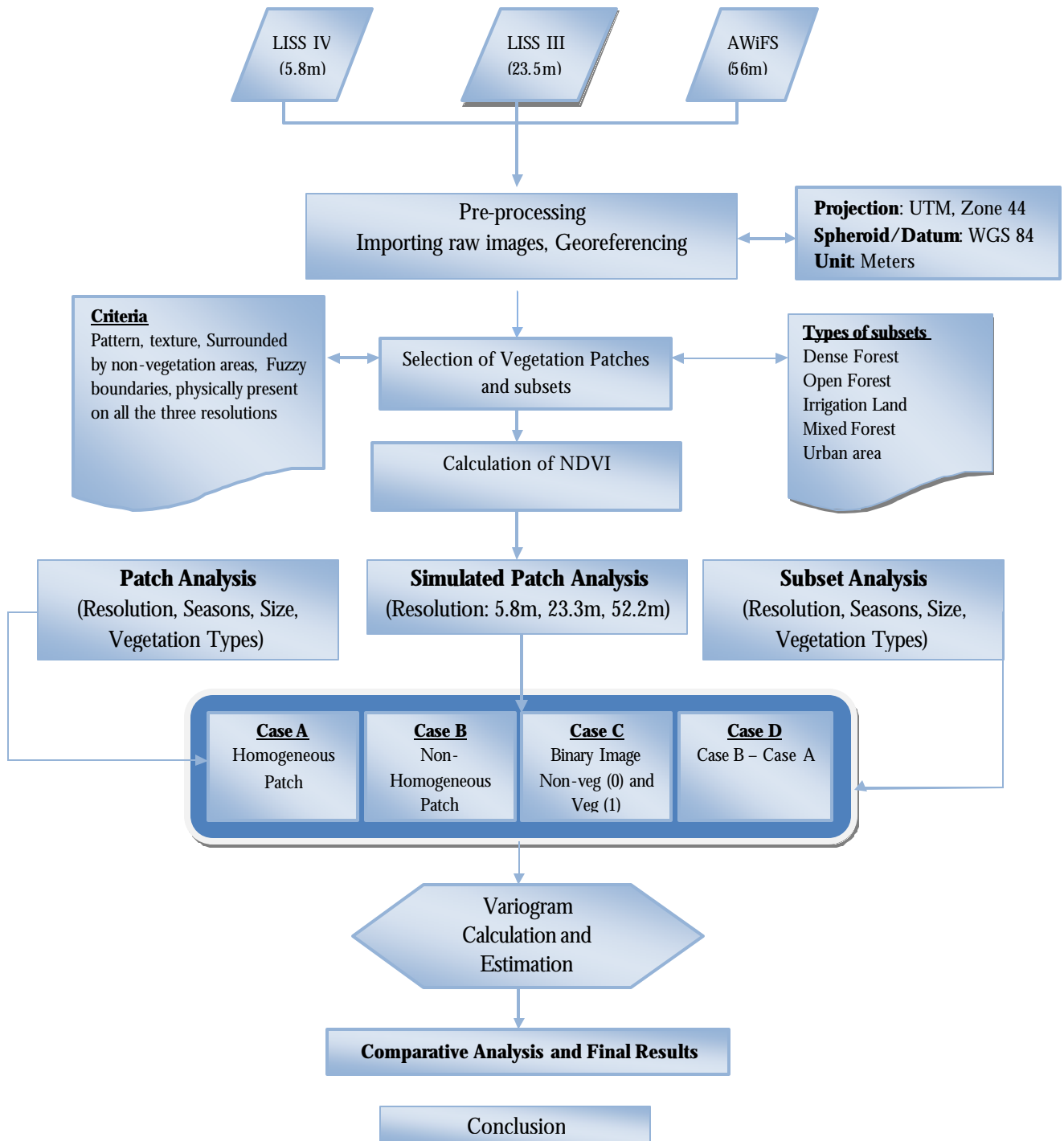
Figure 11 Methodology flow chart
