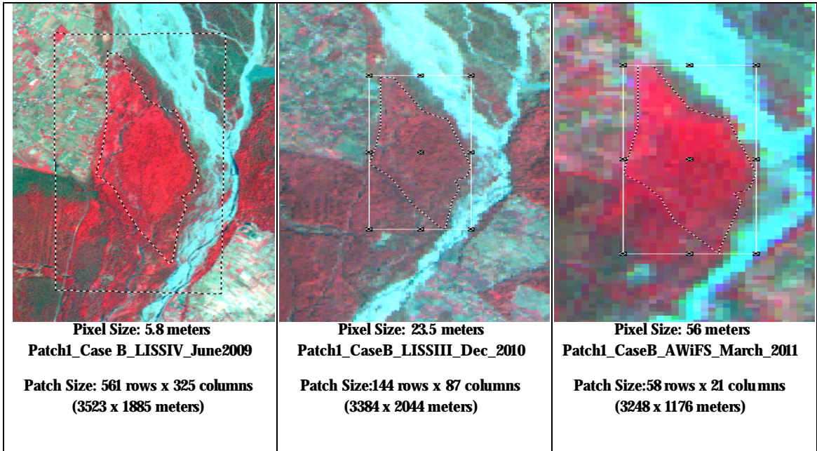
Figure 17: Selected vegetation patches with non vegetation areas along the boundaries across different spatial resolutions (Case B)
