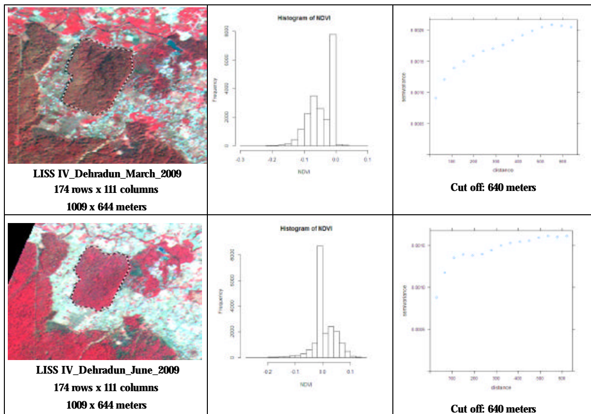
Figure 27 Variogram calculations for same vegetation patch during two different seasons (March and June)
