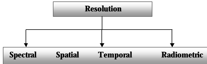
Figure 7: Types of Resolutions
