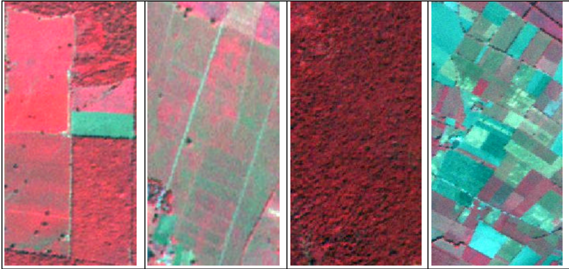
Figure 2: Spatial structure of vegetation
