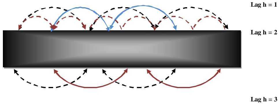
Figure 4 Lags long a transect of pixels
