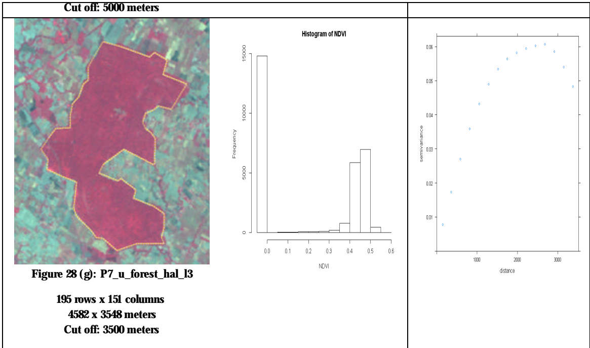
Figure 28: Variogram calculation for different types of subsets selected in Haldwani: LISS III (October, 2009)
