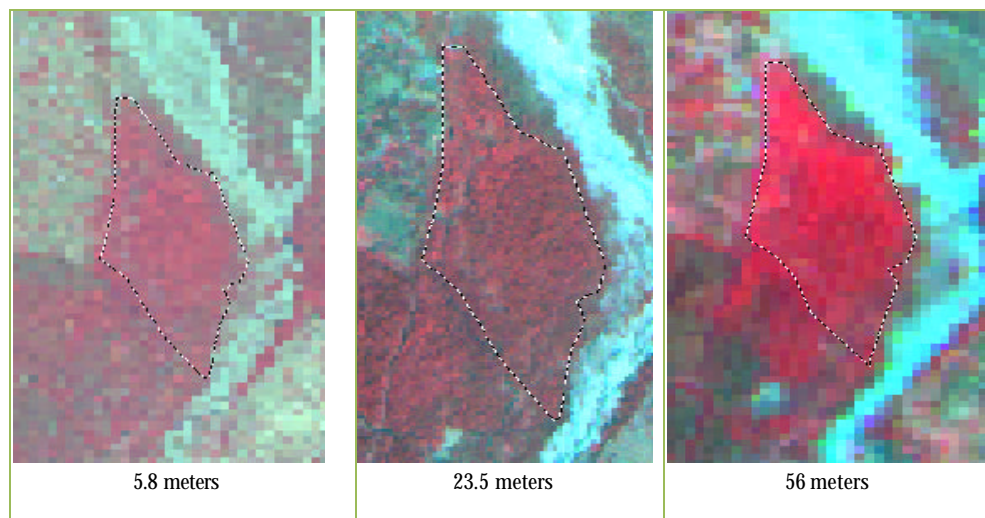
Figure 6: Change in Boundary at different resolutions
