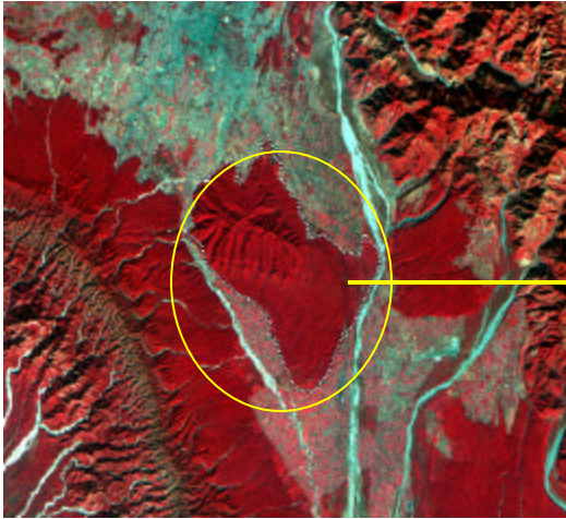
Figure 10(a): Vegetation Patch LISS III Image, DDN Earth
