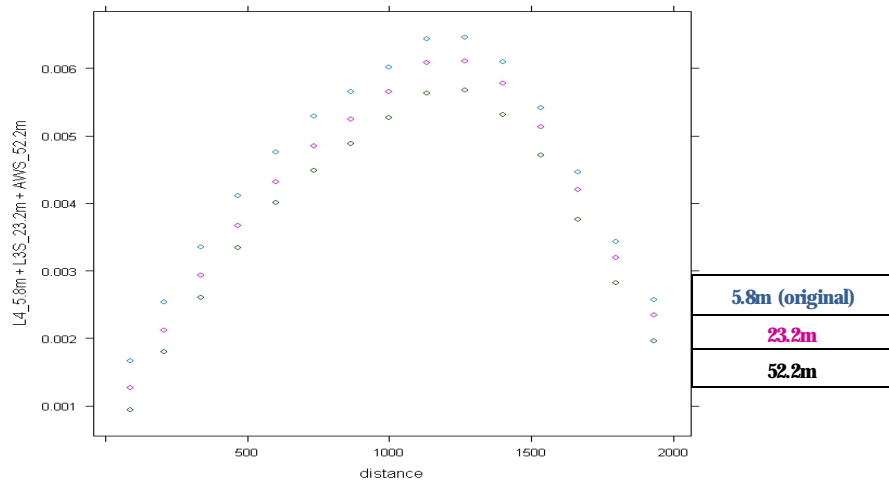
Figure 28 Variogram calculation s for LISS IV (5.8m) and two simulated images (52.2m and 23.2m)
