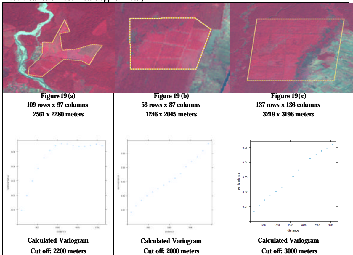
Figure 19 Variogram analysis for vegetation patches having fuzzy and crisp boundaries (Haldwani, LISS III image)
